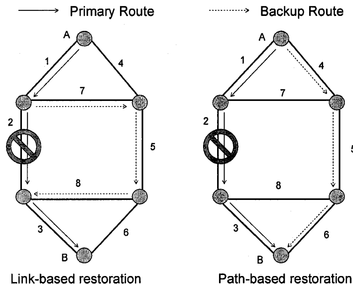
Figure 2-1 Re-establishment mechanisms
