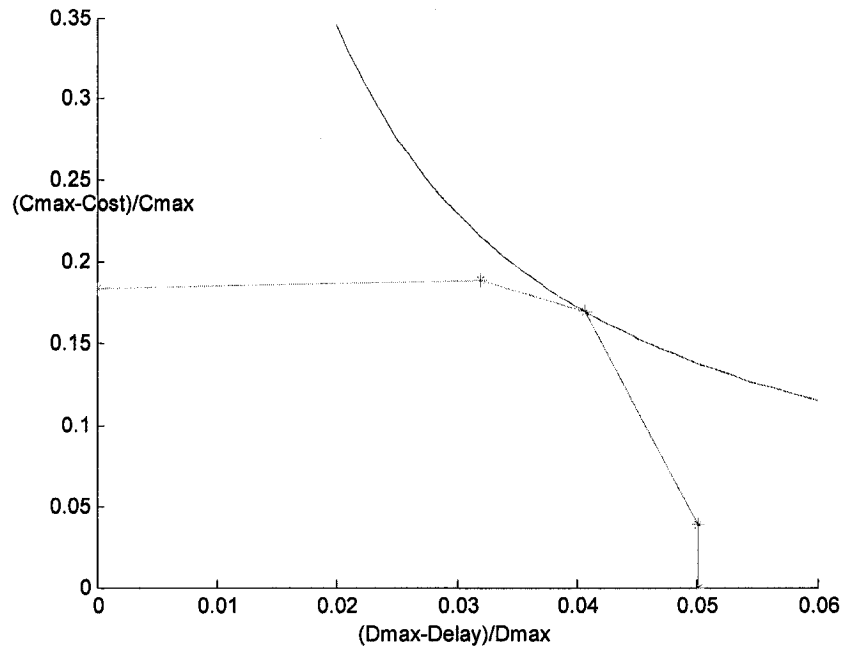
Figure 4-17 Pareto Boundary of delay vs. cost
