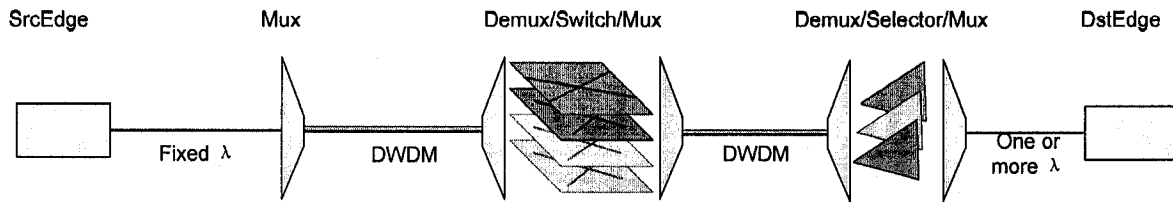
Figure 4-11 Asymmetric Architecture
