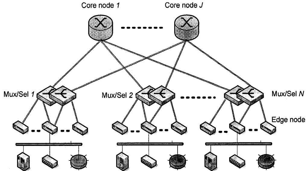
Figure 4-1 AAPN network model: three-layer overlaid tree topology
