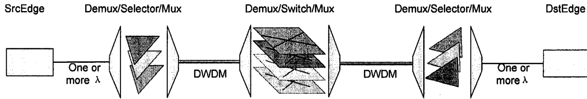
Figure 4-9 Symmetric Architecture
