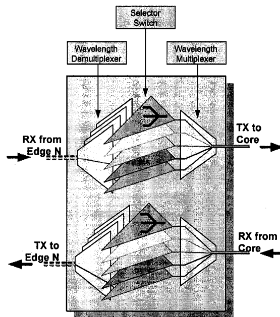
Figure 4-6 Mux/Sel: Symmetric
