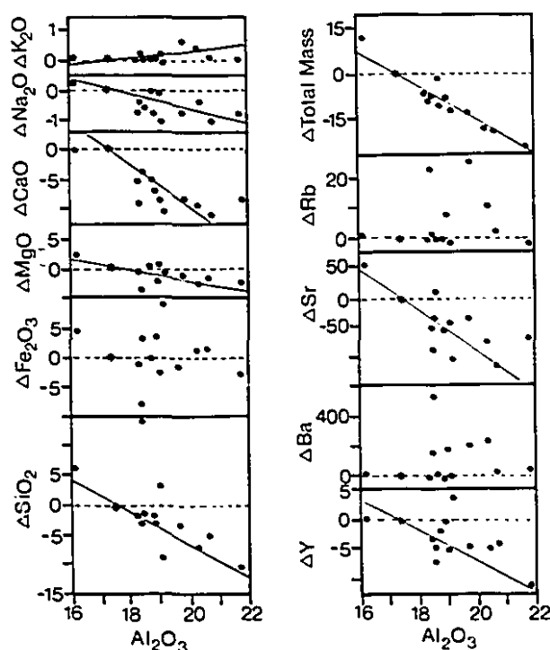
FIG. 10. Element mass changes for pipe 1 (constant TiO 2 , Table 4; major elements in grams, trace elements in parts per million). Al 2 O 3 is used as the alteration index; it is either concentrated by mass losses or diluted by mass gains. *, Least-altered basalt U22.
