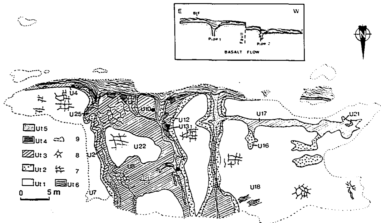
FIG. 6. Outcrop map of pipe 1. U1, least-altered glomeroporphyritic basalt; U2, bleached zone; U3, condrite-gedrite-garnet zone; U4, andalusite-rich zone; U5, pipe conduits filled with chert and disseminated sulfides; U6, silicate-oxide BIF, showing deposition of BIF into the conduits; 7 and 8, fracture patterns; 9, outcrop limit. ●, Mg-tourmaline. Samples numbers as in Tables 2, 3, 4, and 6. The inset is a schematic diagram showing the relation between pipe 1, pipe 2, stratiform alteration (hatched symbol), and BIF.
