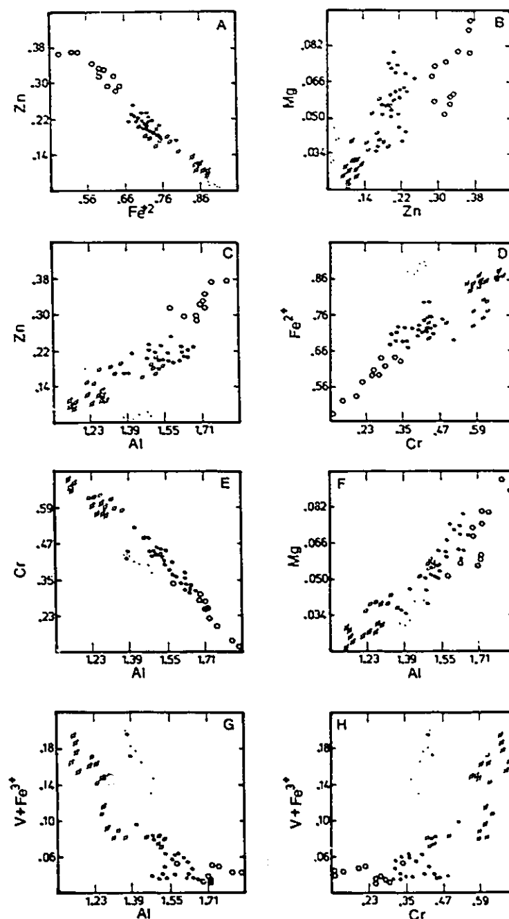
FIG. 7. Binary diagrams showing compositional ranges of hercynite from Atik Lake. Symbols: half-filled circle: U10A, small circle with cross-line: U10B, open circle: U4, filled circle: U8, small dots: U12, open circle with arrow: U17. Correlation coefficients as in Table 5. Concentrations in number of cations.
