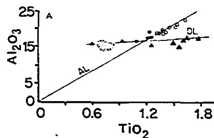
FIG. 9. \text{Al}_2\text{O}_3 - \text{TiO}_2 diagram for pipe 1. Symbols as in Fig. 8. AL, alteration line. Hatched field is for 10 analyses from Hargreaves (1978).
