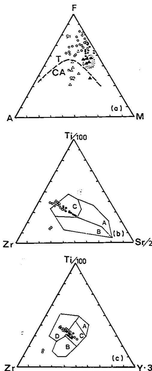
FIG. 5. (a) AFM diagram. T, tholeiitic; CA, calc-alkaline. Closed symbols represent least-altered rocks: ●, porphyritic basalt; ▲, aphyric basalts. Open symbols represent altered basalts: ○, pipes 1 and 2 (g1 = group 1); △, stratiform alteration (g2 = group 2). Hatched field is for 10 analyses from Hargreaves (1978). (b, c) Discriminant diagrams used to distinguish basalt types (Pearce and Cann 1973). A, low-K tholeiite; B, calc-alkaline basalt; C, ocean-floor basalt; D, intraplate basalt.
