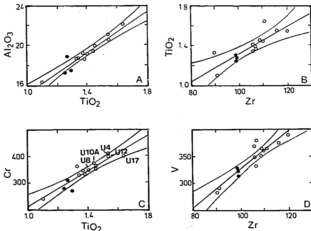
FIG. 4. Plots of element concentrations in rock from pipe 1 (major elements plotted as oxides, expressed in wt. % A. \text{Al}_2\text{O}_3 - \text{TiO}_2 , B. \text{TiO}_2 - Zr, C. Cr - \text{TiO}_2 (the numbers indicate the hercynite-bearing samples of altered basalt), D. V-Zr. Solid lines through data points are derived by linear regression, and the curves reflect a 95% confidence interval. Filled circle: fresh basalt, open circle: altered basalt.
