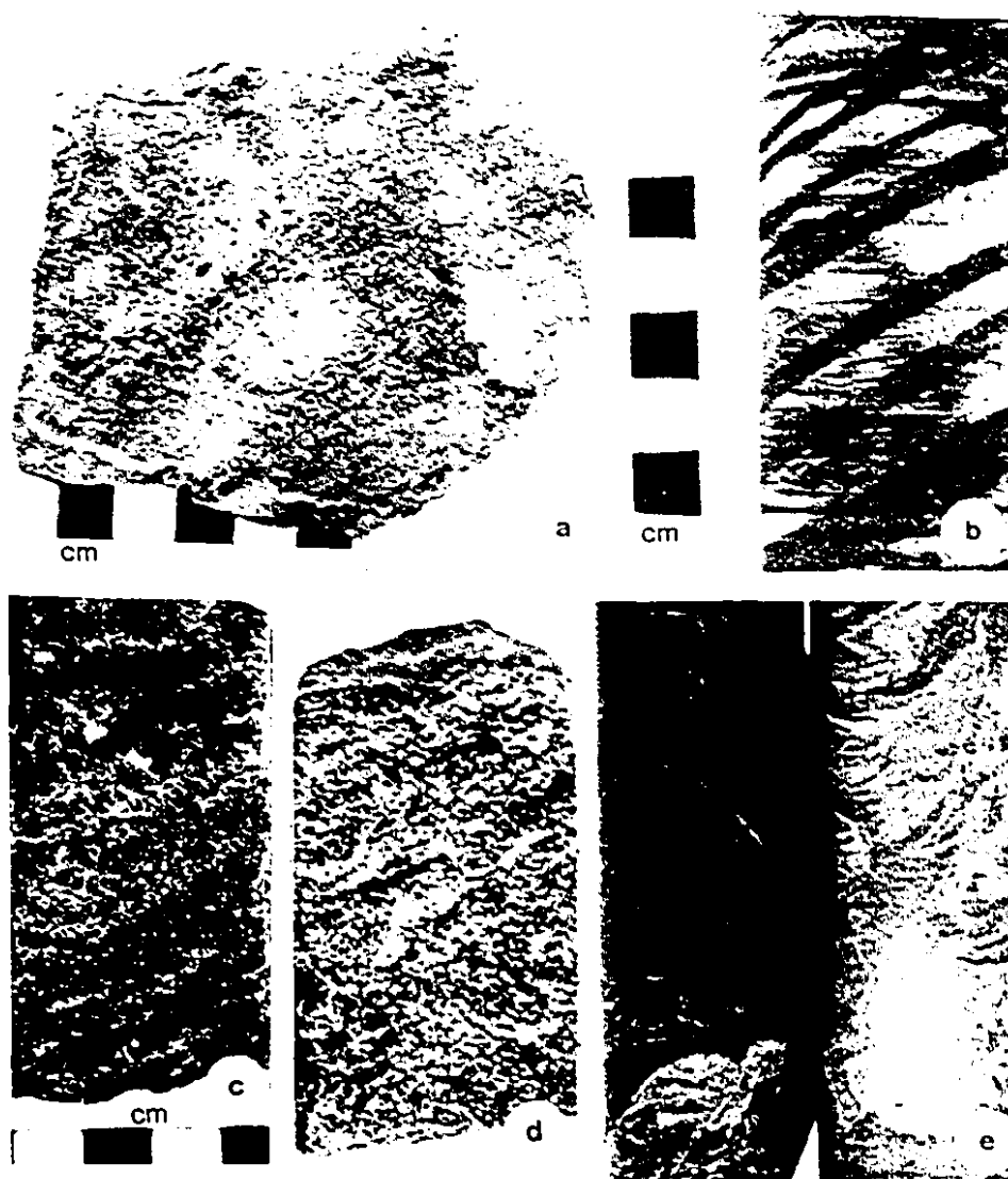
FIG. 4. Photographs of hand specimens. (a) Massive sulfides containing chert and schist fragments (durchbewerget texture; Gilligan and Marshall 1987). (b) Oxide BIF. (c) Silicate-oxide BIF. (d) Auriferous chert. (e) Graphitic argillite.
