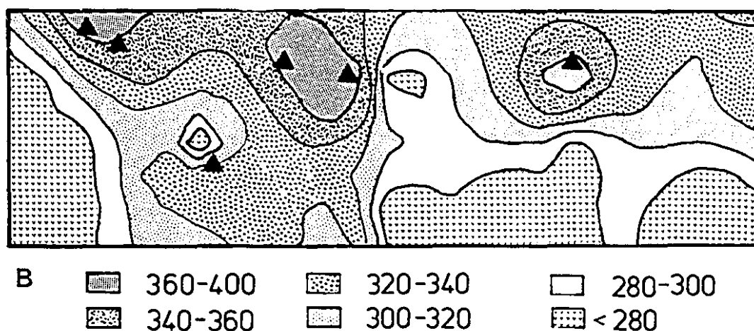
FIG. 2. A. Outcrop map of pipe 1. Symbols: Ut1: least altered glomeroporphyritic basalt, Ut2: bleached zone, Ut3: cordierite-gedrite-garnet zone, Ut4: andalusite-rich zone, Ut5: pipe conduits filled with chert and disseminated sulfides, Ut6: silicate-oxide BIF, showing deposition of BIF into the conduits, 7 and 8: fracture patterns, 9: limit of outcrop. Black dots: magnesian tourmaline. B. Contour map showing chromium concentrations in the alteration pipe. Symbols: triangles: location of samples containing vanadiferous zincian-chromian hercynite.
