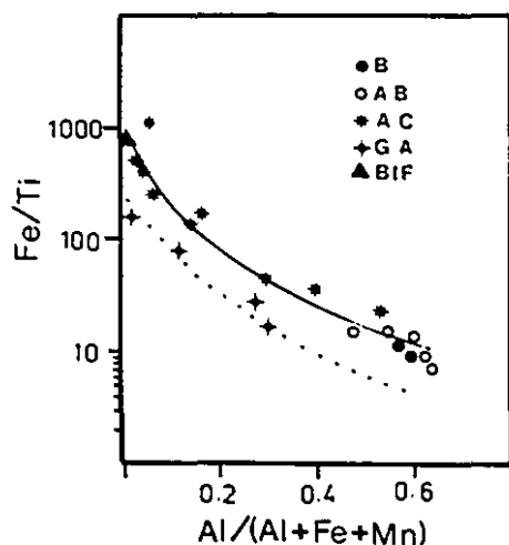
FIG. 13. Fe/Ti vs. Al/(Al + Fe + Mn) diagram (after Boström 1983) illustrating mixing between a pure hydrothermal component (low-Al/(Al + Fe + Mn)) and a detrital or basaltic component (high-Al/(Al + Fe + Mn)). Abbreviations as in Figs. 11 and 12.
