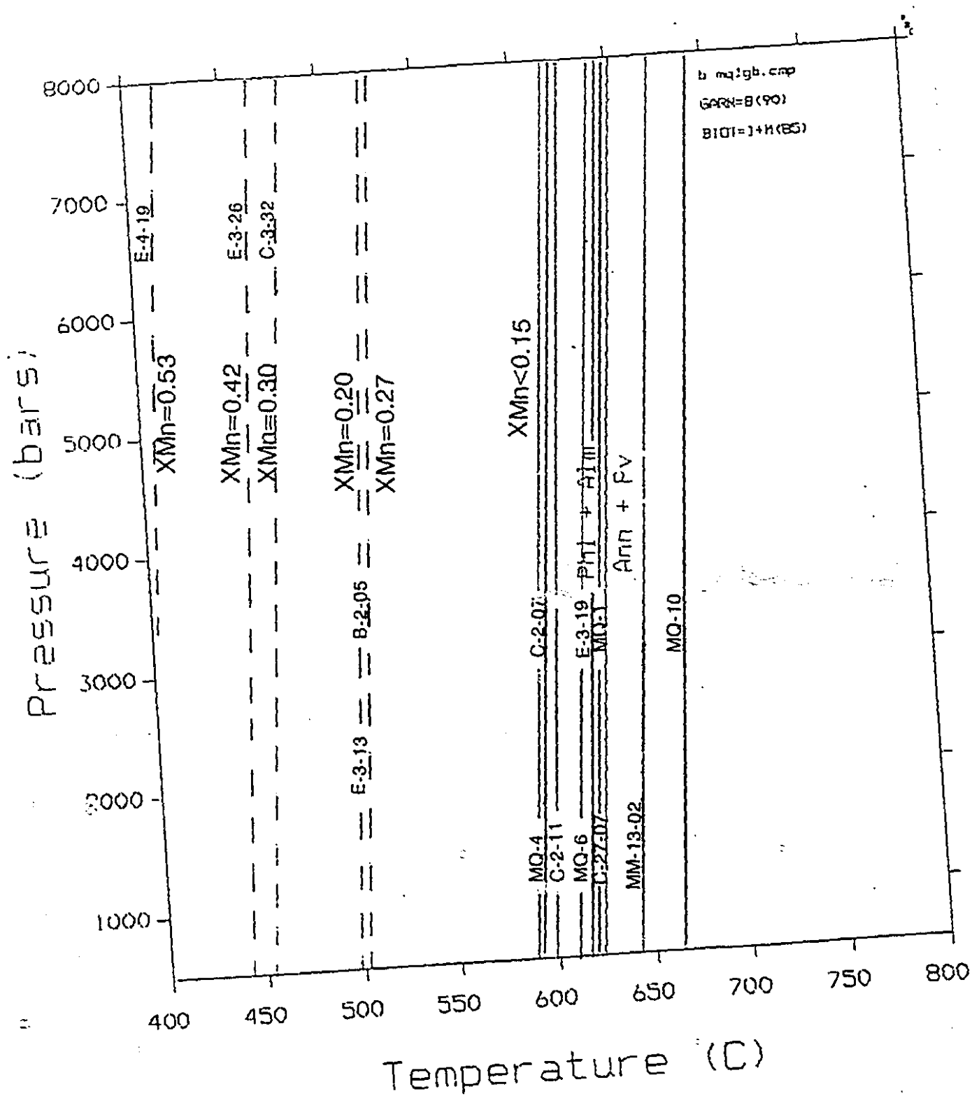
Fig. 4.14. Pressure-temperature diagram showing the garnet-biotite equilibria calculated for the Montauban rocks using GEO-CALC and Berman's (1991) garnet activity model. The equilibrium boundary is displaced toward lower T with increasing mole fraction of spessartine ( X_{Mn} ) in garnet.
