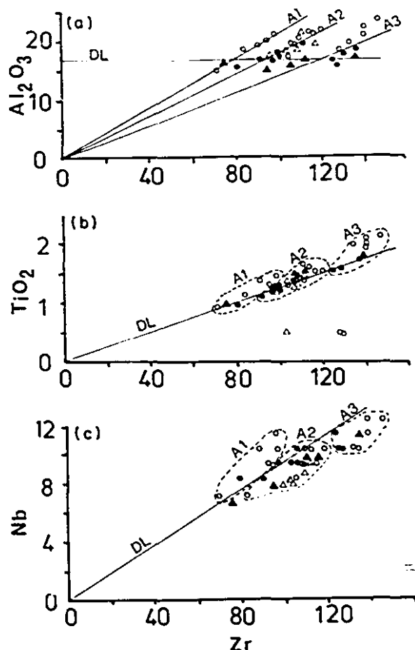
FIG. 8. (a) \text{Al}_2\text{O}_3 -Zr diagram. DL, differentiation line; A2, alteration line for pipes 1 and 2 and stratiform alteration; A1 and A3, alteration lines for other flows. (b) \text{TiO}_2 -Zr diagram. Alteration lines A1-A3 coincide with the differentiation line (DL) for all basalt compositions. (c) Nb-Zr diagram. Nb shows a distribution similar to that of \text{TiO}_2 . ●, Glomeroporphyritic basalt; ▲, aphyric basalts; ○, altered basalts; △, stratiform alteration.
