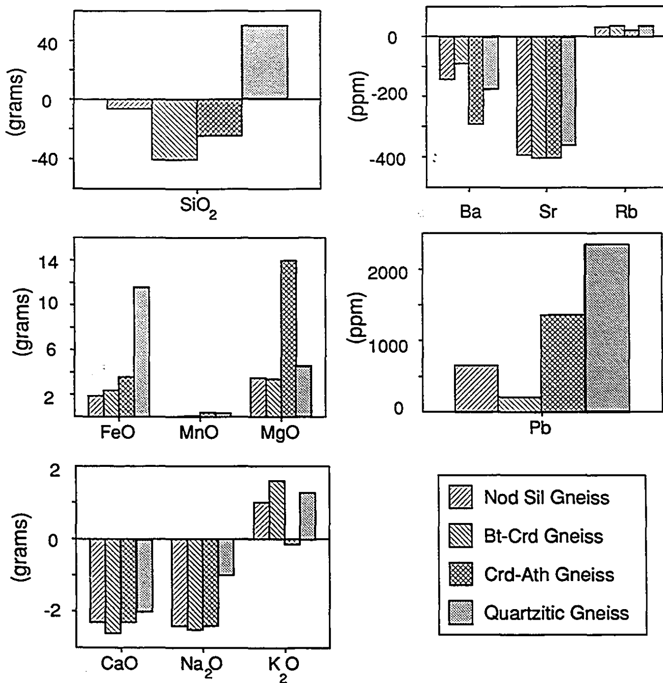
Fig. 10. Bar diagrams illustrating average mass changes for the North Gold Zone altered rocks.
