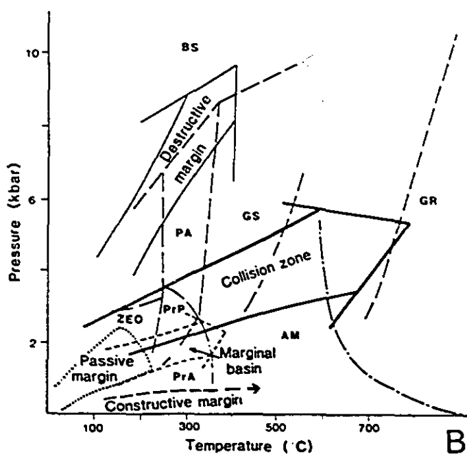
Fig. 4.33. Schematic diagrams of P-T ranges for the metamorphic facies series (A) from Best (1982), and for major tectonic settings (B) from Robinson (1987). The range of peak P-T conditions estimated for the Atik Lake, Némiscau and Montauban terranes are outlined on these P-T diagrams. A) Geotherms are drawn for 10, 30, 50, 100°C/Km. B) ZEO=zeolite facies, PrA=prehnite-actinolite facies, BS=blueschist facies, GS=greenschist facies; AM=amphibolite facies, GR=granulite facies.
