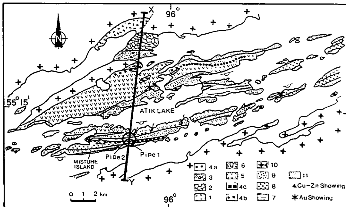
Fig. 2. Geology of the Atik Lake greenstone belt (modified from Weber 1974). (1) Amphibolite; (2) felsic agglomerate and tuff; (3) mafic pyroclastics; (4a) sulfide iron formation (auriferous chert where gold bearing); (4b) oxide BIF; (4c) silicate BIF; (5) basalt; (6) conglomerate; (7) cordierite-biotite gneiss; (8) glomeroporphyritic basalt; (9) gabbro; (10) granitic gneiss (north) and tonalitic gneiss (south); and (11) altered basalt. X-Y, section in Fig. 3.
