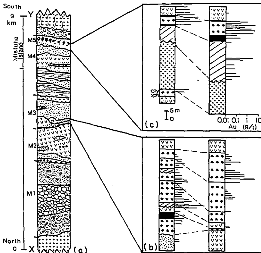
FIG. 3. (a) Stratigraphic section (X-Y, Fig. 2). M1-M5 mafic sequences. (b, c) Detailed sections of the BIF and auriferous cherts. Gold contents are on a logarithmic scale. The hatched symbol in c is the stratiform alteration zone. Black areas in b and c are graphitic argillite; cpy, chalcopyrite; sph, sphalerite. Other symbols as in Fig. 2.
