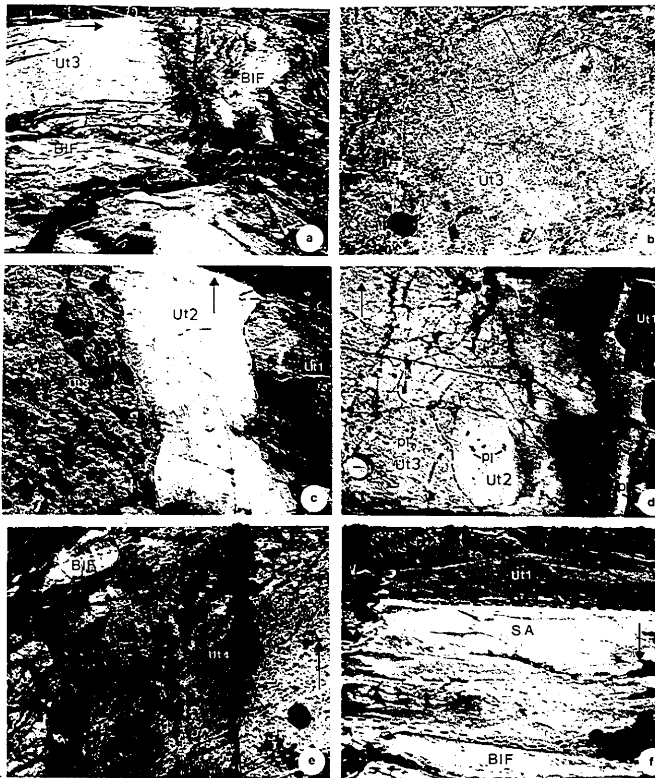
FIG. 7. Photographs of alteration zoning at pipe 1. (a) BIF within conduit. (b) Polygonal joints in basalt (Ut3, Fig. 6), with concentrations of gedrite needles. (c) Alteration zoning from least-altered basalt (Ut1) to bleached basalt (Ut2) and cordierite-gedrite-garnet altered basalt (Ut3). (d) Transition from Ut1 to Ut3; pl, plagioclase phenocrysts. (e) Andalusite-rich patches (Ut4). (f) Stratiform alteration (S.A.) in flow-top breccia overlying Ut1 and capped by silicate-oxide facies BIF. Arrow indicates stratigraphic top. Lens cap = 5 cm.
