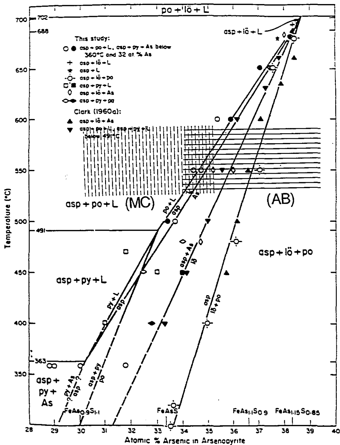
Fig. 4.21. Temperature-composition diagram with arsenopyrite-buffered boundaries, from Kretchmar and Scott (1976). The ranges of arsenopyrite compositions in the mineralized chert (MC) and the altered basalt (AB) are shown in the two hatched boxes.
