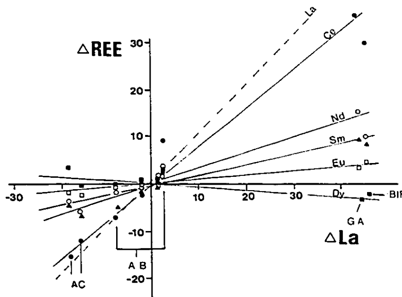
FIG. 12. Changes in chondrite-normalized REE values vs. changes in La. Abbreviations as in Fig. 11. The increase in mobility is indicated by the increase in slope values: Dy = -0.04 (■); Eu = 0.09 (□); Sm = 0.19 (▲); Nd = 0.32 (○); and Ce = 0.70 (●).
