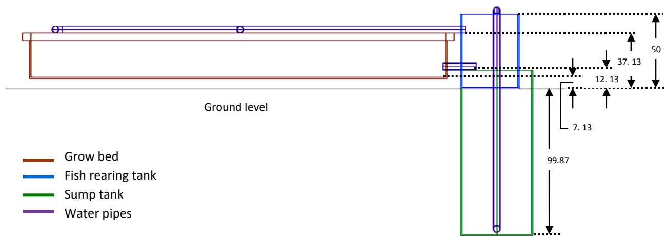
Figure 20: Aquaponic system side view (grow bed, fish rearing tank, sump tank and water distribution pipes) with heights in centimetres.
