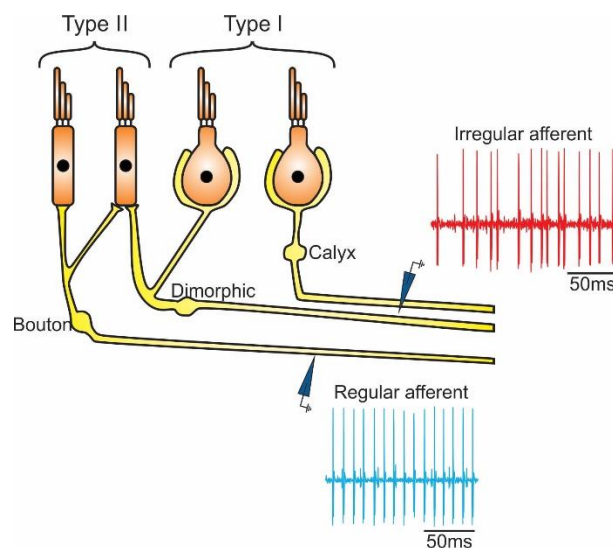
Figure 1.3: Vestibular hair cells and primary vestibular afferents
