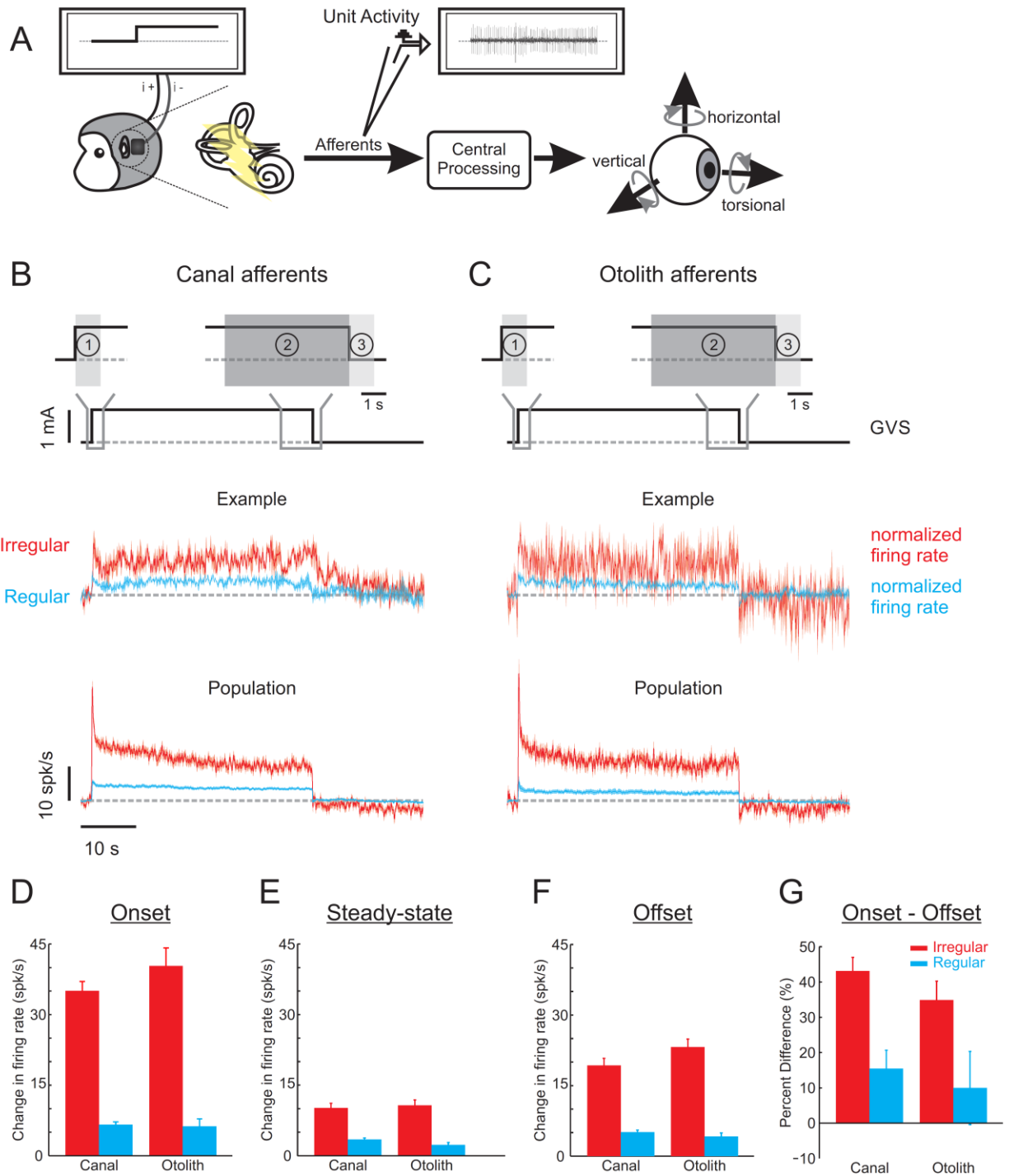
Figure 3.2. Response characteristics of vestibular afferents to constant cathodal current GVS. (A) We recorded extracellular single-unit activity from vestibular afferents using tungsten electrodes during constant current GVS. (B) The top row shows the constant cathodal current stimulation and the zoomed-in schematic of the three phases: (1) onset, (2) steady-state, and (3) offset. The middle row shows the average firing rate across three constant current pulses of an example regular (blue) and irregular (red) canal afferents relative to a 2 second baseline prior to the onset of the
