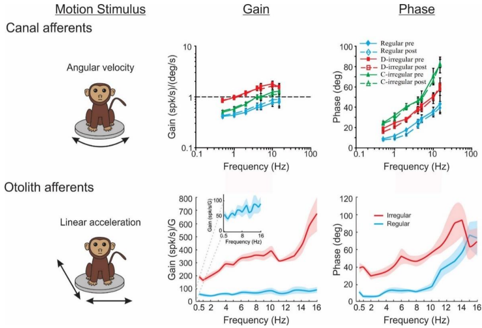
Figure 1.4: Linear response dynamics of vestibular afferents to motion
