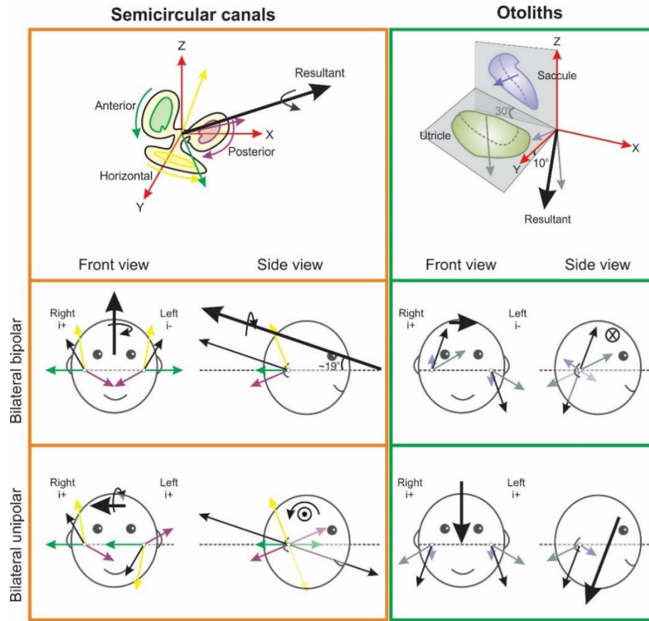
Figure 1.6: Model of GVS activation of the peripheral vestibular system
