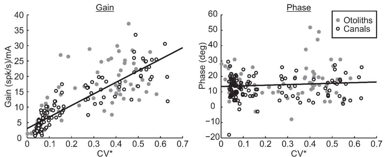
Figure 2.3. Comparison of canal and otolith afferent responses to sinusoidal GVS (A) Gain (left) and phase (right) of canal (open black circles, N = 118 ) and otolith (filled grey circle, N = 81 ) to 1 Hz sinusoidal as a function of the resting discharged variability, quantified as CV*.
