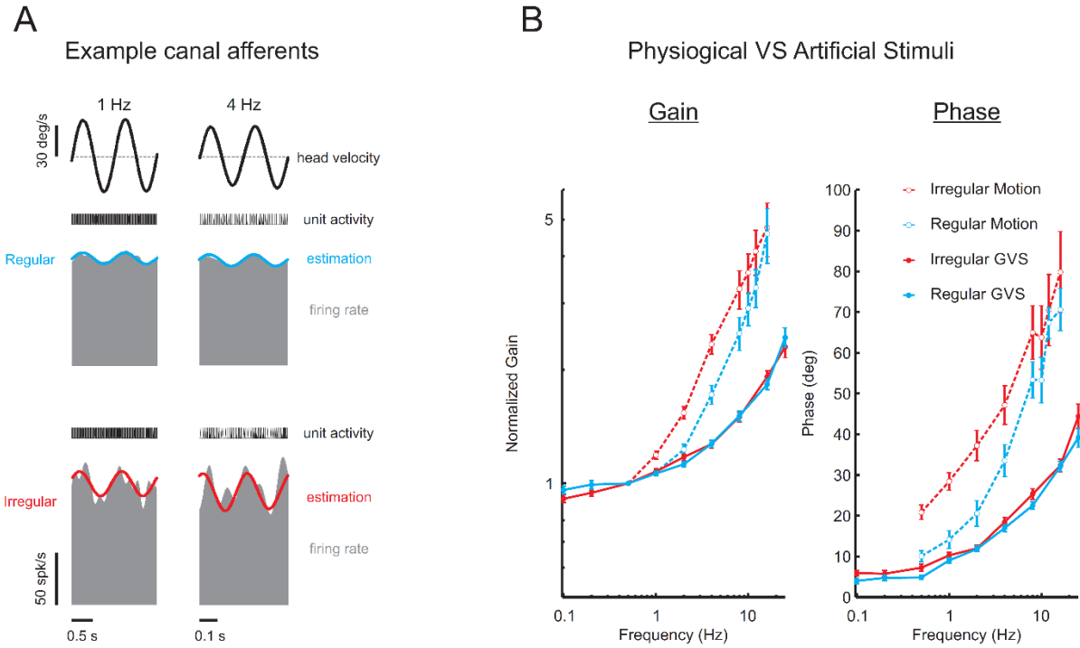
Figure 2.4. Comparison of motion and GVS for canal afferents. (A) Firing rate (gray) of example regular (blue) and irregular (red) canal afferents to 1 Hz (left) and 4 Hz (right) head velocity. Firing rate estimates (solid blue and red line) are found using eq. 2.2. (B) Comparison of canal afferent responses to physiological (yaw rotation) and artificial (GVS) stimuli. Population normalized gain (left) and phase (right) to motion for regular (blue dashed line and open circles, N = 21-26 ) and irregular (red dashed line open circles, N = 17-21 ) canal afferents. Population normalized gain (left) and phase (right) to sinusoidal GVS for regular (solid blue line) and irregular (solid red line) canal afferents.
