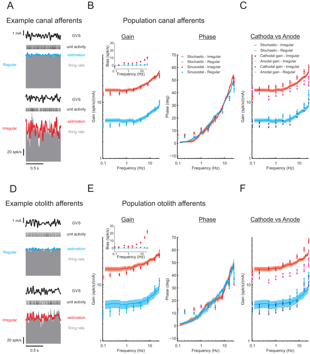
Figure 3.4. Response dynamics of vestibular afferents to broadband stochastic GVS. (A) Response of canal afferents. The right panel shows firing rate (gray) of example regular (blue) and irregular (red) canal afferents to segments of broadband stochastic GVS. (B) Population averaged gain (left), and phase (right) for regular (blue, N = 58 ) and irregular (red, N = 48 ) canal afferents. Superimposed gain and phase (dots) are the population response dynamics to sinusoidal GVS from Chapter 2. Inset shows estimated bias using eq. 2.1 as a function of frequency for regular (blue) and irregular (red) afferents. (C) The gains using the cathodal (red filled circles) and anodal (pink
