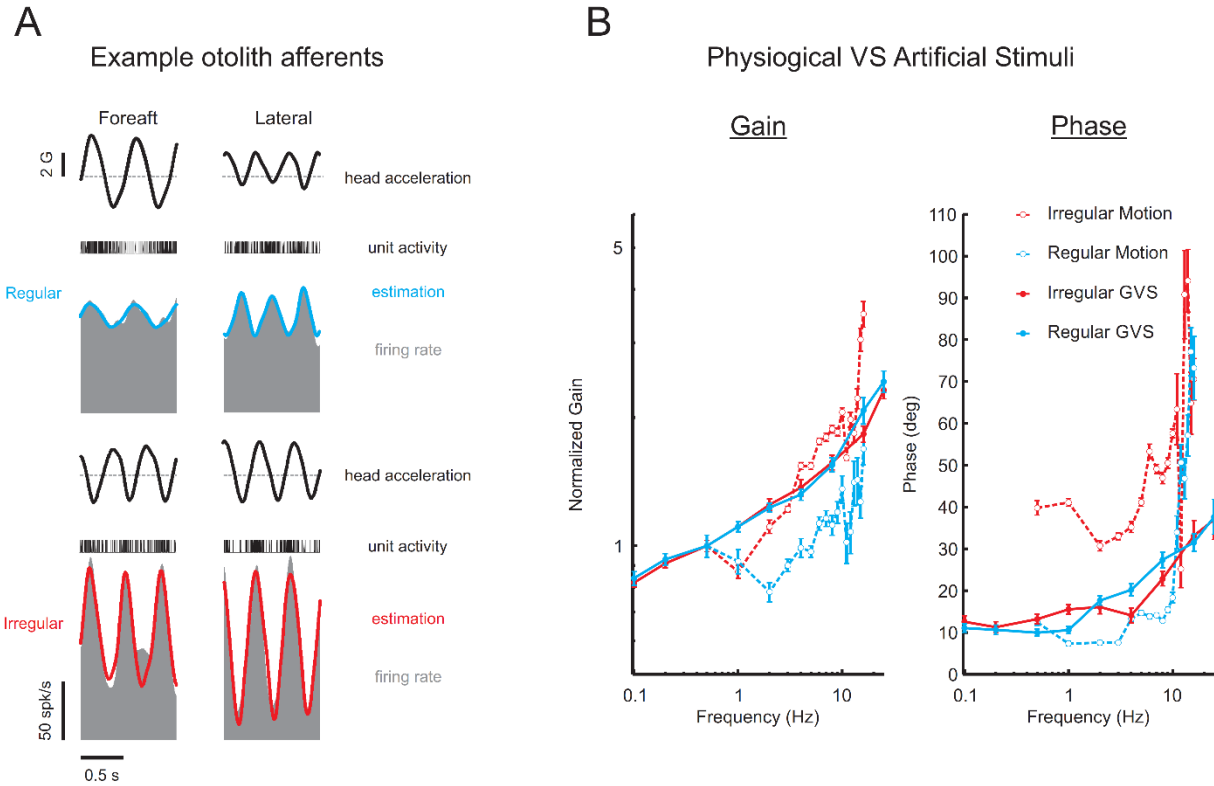
Figure 2.5. Comparison of motion and GVS for otolith afferents. (A) Firing rate (gray) of example regular (blue) and irregular (red) otolith afferents to \sim 2 Hz foreaft (left) and lateral (right) head acceleration. Firing rate estimates (solid blue and red line) are found using eq. 2.3. (B) Comparison of otolith afferent responses to physiological (translation motion) and artificial (GVS) stimuli. Population normalized gain (left) and phase (right) to motion (Jamali et al. , 2013) for regular (blue dashed line and open circles, N = 6-30 ) and irregular (red dashed line open circles, N = 4-26 ) otolith afferents. Population normalized gain (left) and phase (right) to sinusoidal GVS for regular (solid blue line) and irregular (solid red line) otolith afferents.
