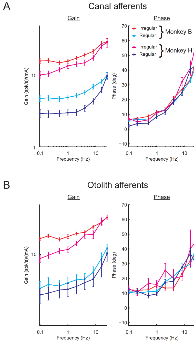
Figure S2.1. Comparison of vestibular afferents recorded from two animals. (A) Population averaged gain and phase of regular (Monkey B: light blue, N = 21-36; Monkey H: dark blue, N = 6-27) and irregular (Monkey B: red, N = 21-40; Monkey H: pink, N = 6-16) canal afferents to sinusoidal GVS. (A) Population averaged gain and phase of regular (Monkey B: light blue, N = 8-18; Monkey H: dark blue, N = 3-12) and irregular (Monkey B: red, N = 17-41; Monkey H: pink, N = 1-13) otolith afferents to sinusoidal GVS.
