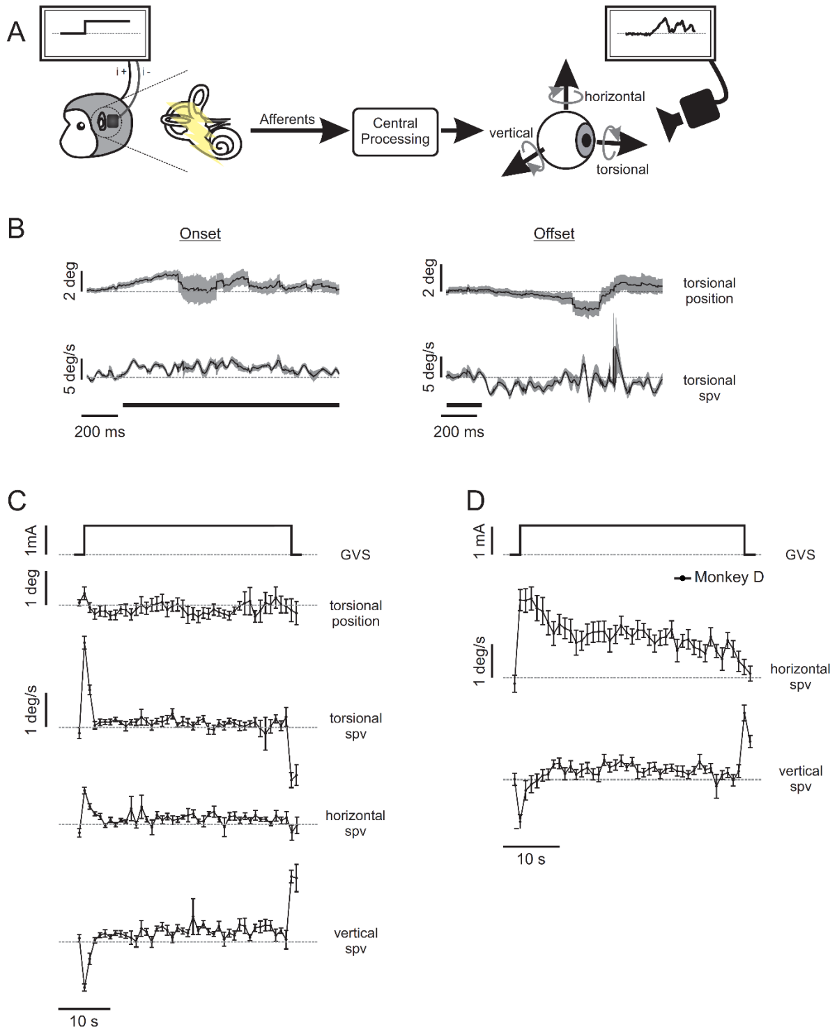
Figure 3.1. Eye movements in response to constant current GVS. (A) While we applied constant current GVS between surface electrodes placed on the mastoid processes behind the ears, we recorded the animal's eye movements in the presence or absence of a fixation target. (B) GVS-evoked torsional eye movements with a fixation target. Average torsional eye position and slow
