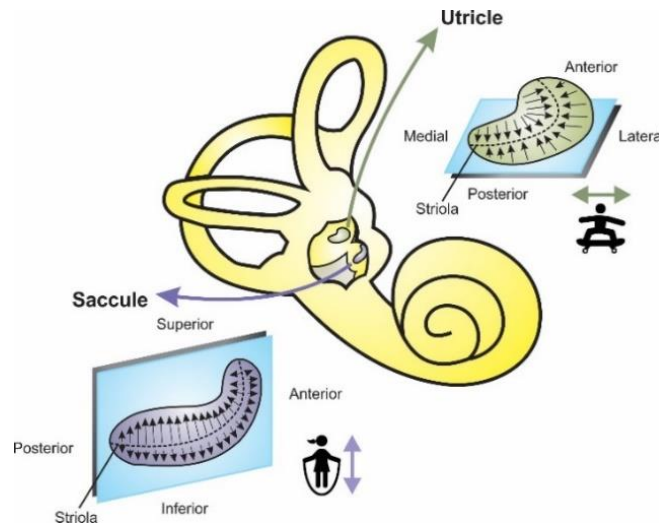
Figure 1.2: Diagram of the utricle and saccule
