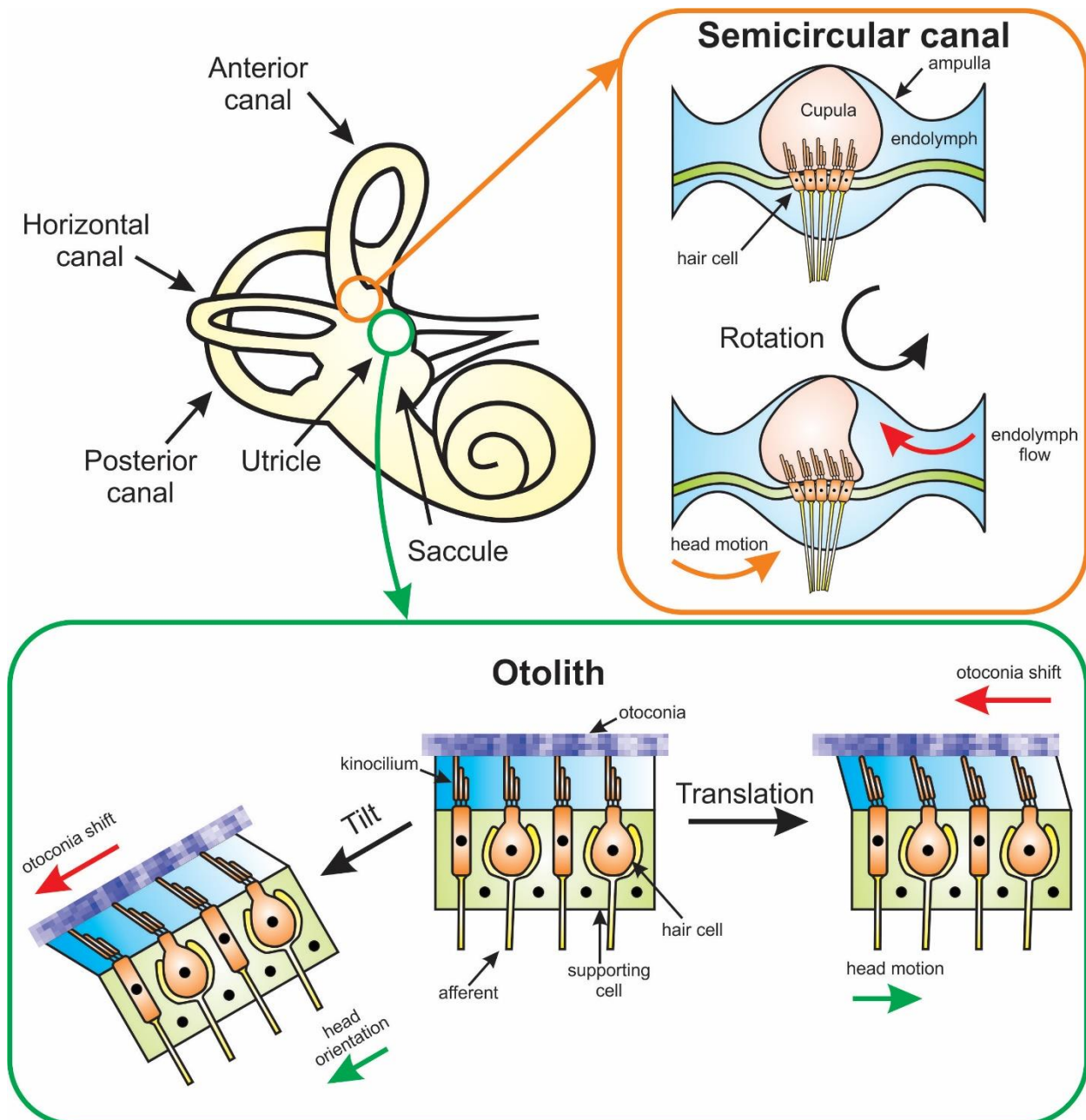
Figure 1.1: Diagram of the vestibular sensory organs and mechanism of hair cell activation Semicircular canals detect rotation. Orange inset shows the organization of the hair cells within the semicircular canals. During head rotation, the endolymph lags behind and pushes on the cupula, deflecting the hair cells in the process. Otolith organs sense translation as well as head tilt relative to gravity. Green inset shows the organization of the hair cells within the otolith organs. During head translation (right), the otoconia lags behind and causes a shift between the otolithic membrane and the macula, deflecting the hair cells in the process. During head tilt (left), the force of gravity pulls the otoconia downward and causes a shift between the otolithic membrane, deflecting the hair cells in the process.
