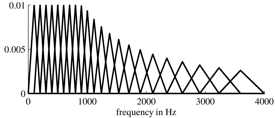
Fig. 2.4 A Typical Mel filter bank
