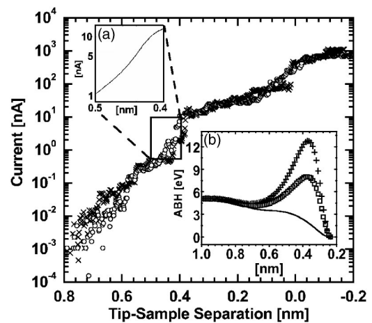
FIG. 2. Current-distance characteristics. Inset plots are theoretically calculated (a) current (from Ref. 13) and (b) work functions (ABH) vs tip-sample separation. Relaxation effects are more pronounced over top site (cross, b) than hollow site (square, b). The calculated work functions (without relaxation) do collapse (solid line, b).
