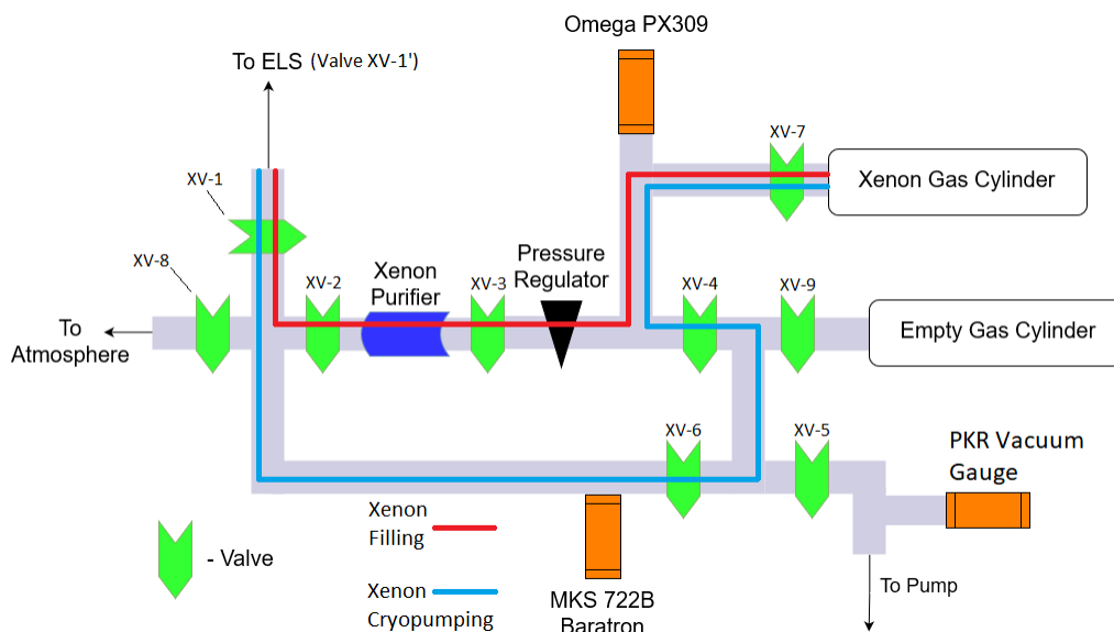
Figure 20: Diagram for the ELS gas handling system, along with main components and outlets. Labelled valves (in green) are located throughout the system to close off different areas depending on whether the system is used for filling the chamber with xenon or for cryopumping the gas back into the cylinder; the gas xenon paths for both filling and cryopumping are shown in red and blue, respectively. The Baratron is used to measure the gas pressure in a volume which includes the chamber, whereas the Omega is used to monitor the gas pressure in the xenon bottle (at a level of 2900 Torr when all the gas is in the bottle). Also shown is the secondary gas cylinder usually pumped to vacuum that can be used to reduce the pressure in the chamber without having to cryopump and refill.
