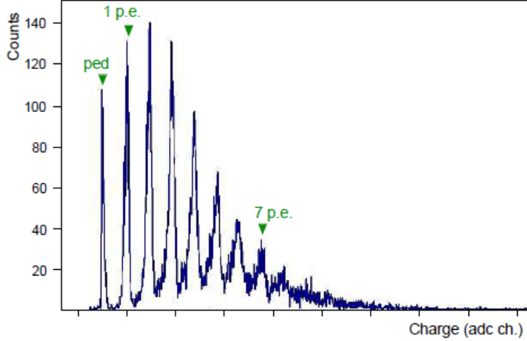
Figure 10: Integrated charge signal histogram for a typical low photon count SiPM signal. The left-most peak is referred to as the “pedestal” and represents the integrated signal for 0 pixels firing, every subsequent peak corresponds to the integrated signal from one more photoelectron avalanche [58].
