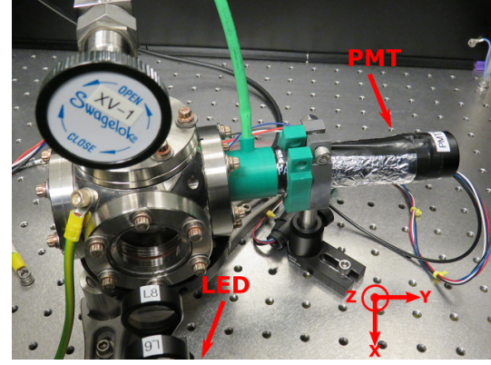
(b) PMT Positioned for Light Collection.
