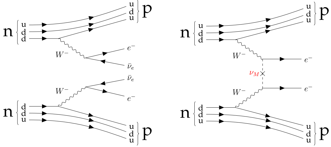
Figure 2: On the left: Feynman diagram of a regular double beta decay in which two neutrons decay into two protons and release 2 e^- \bar{\nu}_e pairs. On the right: A neutrinoless double beta decay where only 2 e^- are present in the final state.
