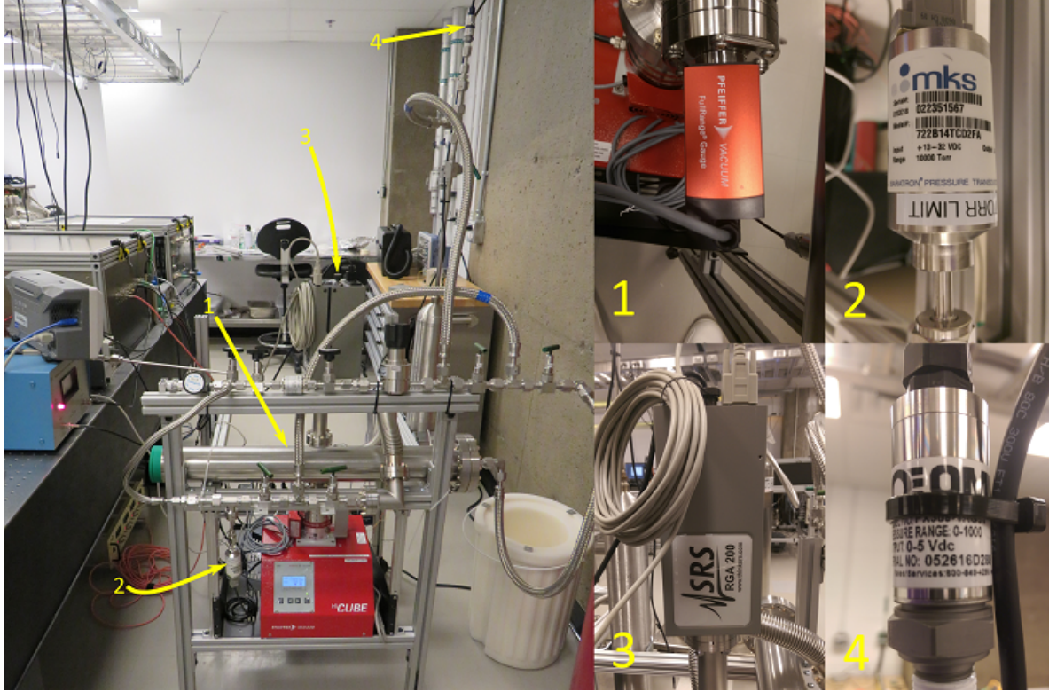
Figure 19: The gas handling system used for the pumping, filling and recovery of the xenon gas used in the ELS. In red is a Pfeiffer HighCube Eco pump stand coupled with a Pfeiffer PKR361 full range pressure gauge (gauge labelled as 1) used to reach vacuums of 10^{-10} Torr. The system is also equipped with an Omega PX309 [98] (4) gauge to measure the gas pressure in the xenon tank and an MKS 722B Baratron [99] (2) used to determine the pressure inside the chamber. To recover the xenon gas from the system, the white dewar is filled with liquid nitrogen and the vertical cylinder containing the xenon is lowered into it. A residual gas analyzer (3) is also attached to the system to perform leak checking and ensure good vacuum quality before any xenon is allowed to flow.
