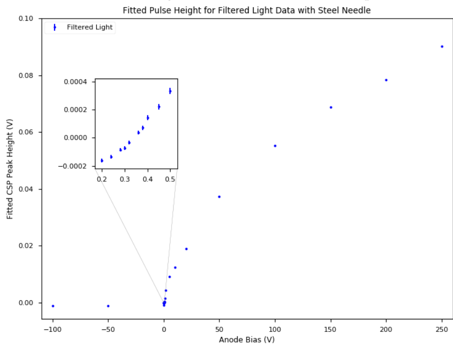
(b) Pulse height vs. anode bias with Xe lamp + 265 nm filter.
