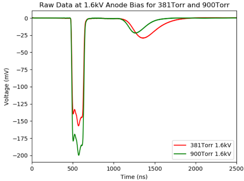
Figure 43: Example of different leakage amplitudes for two different pressures at the same anode bias. The data sets for 381 Torr and 900 Torr were taken on Oct. 11 th 2019 and Oct. 14 th 2019, respectively.
