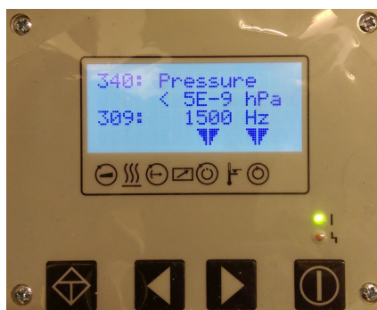
Figure 23: Pfeiffer pump stand display control unit. The display can output the state of two parameters at once. In this case the pressure measured by the PKR361 and the rotation frequency of the turbo pump are displayed. The buttons on the DCU can be used to navigate, monitor and change the different parameters of the pump stand, such as the drive current, turbo pump power, backing pump operation mode and more.
