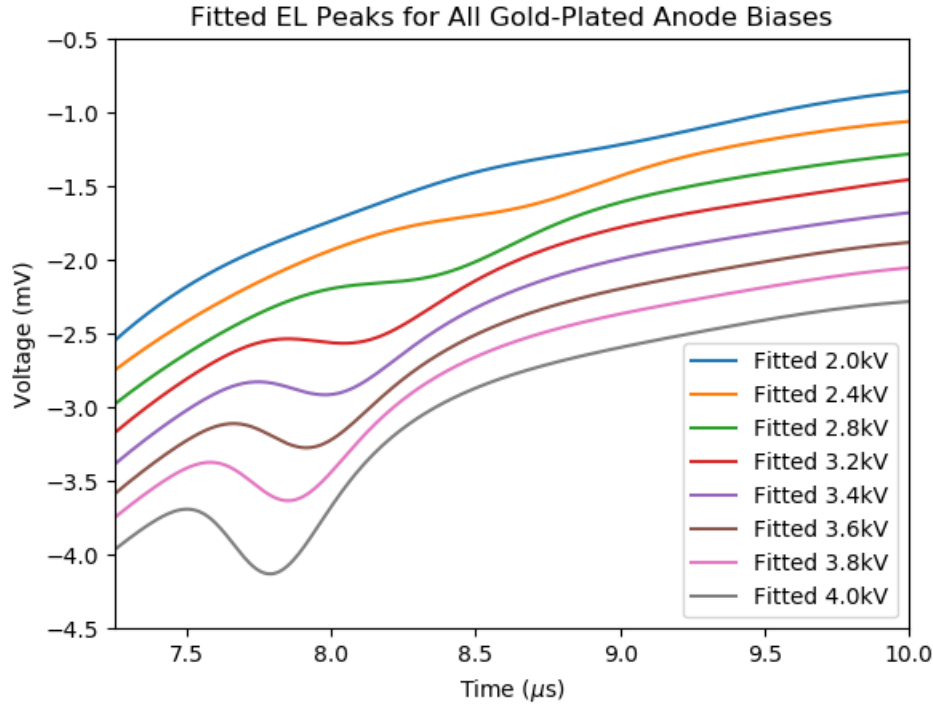
Figure 39: Fits for all EL pulses at various gold-plated anode biases between 2 kV and 4 kV. A clear trend can be seen both in the height, position and width of the peaks. Note that the fits are vertically offset by 0.1 mV each for clarity; however, there is no horizontal offset.
