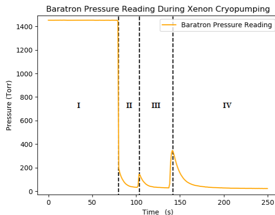
(b) Pressure Reading During Cryopumping.
