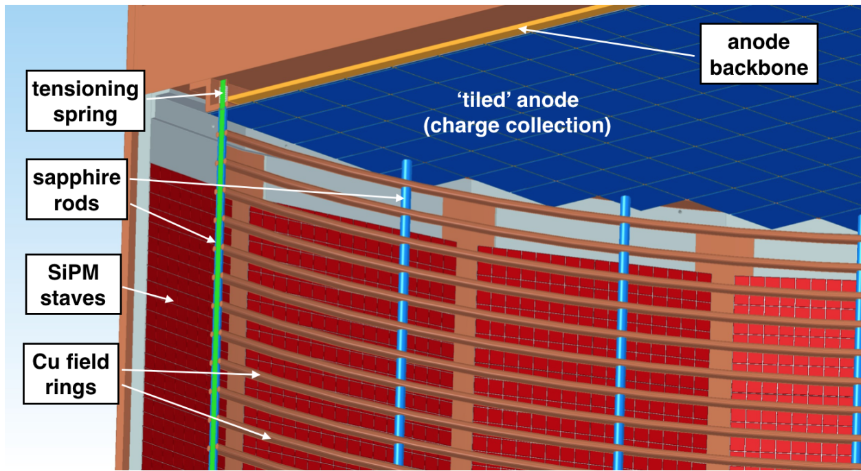
Figure 7: Artist's drawing of the inner view of the TPC near the anode. The field shaping rings will be spaced apart 1.6 cm and held together by long sapphire rods, tensioning springs at each end of the TPC hold the sapphire rods straight. Illustrated is the tiled nature of the anode and the placement of the light detecting Silicon Photomultiplier staves behind the field shaping rings [33].
