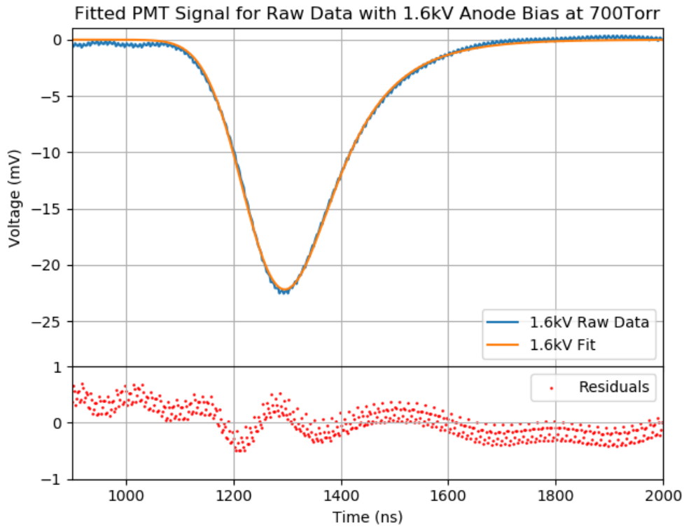
Figure 42: Fit of approximately 10^6 averaged raw data traces of electroluminescent light at 700 Torr and 1.6 kV bias. This wavy behavior of the residuals is common for basically all EL pulses with the steel needle. The small ripples before the peak in the raw data might be due to noise from the digitizer or the PMT. The uncertainties on the residuals have been omitted for clarity and are on the order of 0.2 mV. As in previous plots with residuals, their units are the same as those of the main y-axis.
