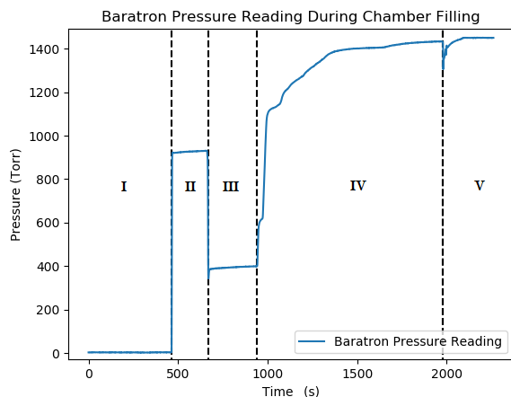
(a) Pressure Reading During Filling.
