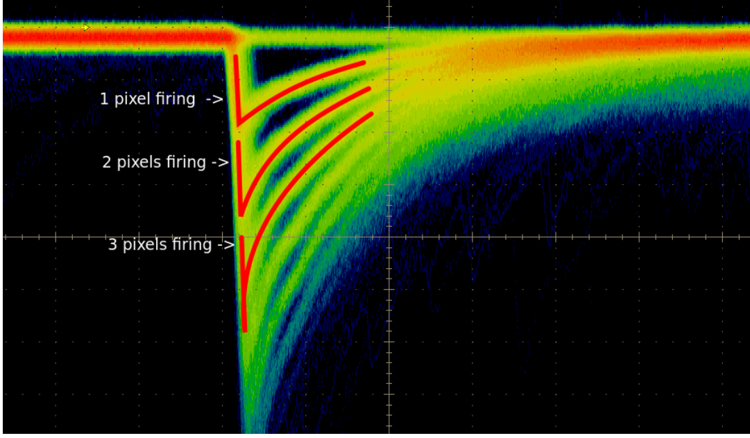
Figure 11: Examples of SiPM time trace signals. The increase in amplitude with increasing photoelectron number is clear. Peaks with crosstalk contributions are indistinguishable as they remain in phase. Afterpulsing is represented by secondary peaks (in dark blue here) following the signal from the main avalanche [60].
