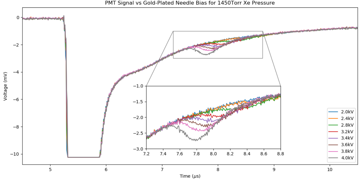
Figure 37: Averaged sets of 200 raw light data traces with the Xe flash lamp showing the emergence of electroluminescent light emission at around 8 \mu s. The bias was varied from 2 kV where no EL is noticeable to 4 kV where a very visible peak is present. The PMT bias was held at 2.4 V for these measurements to prevent the intense lamp signal from damaging the PMT.
