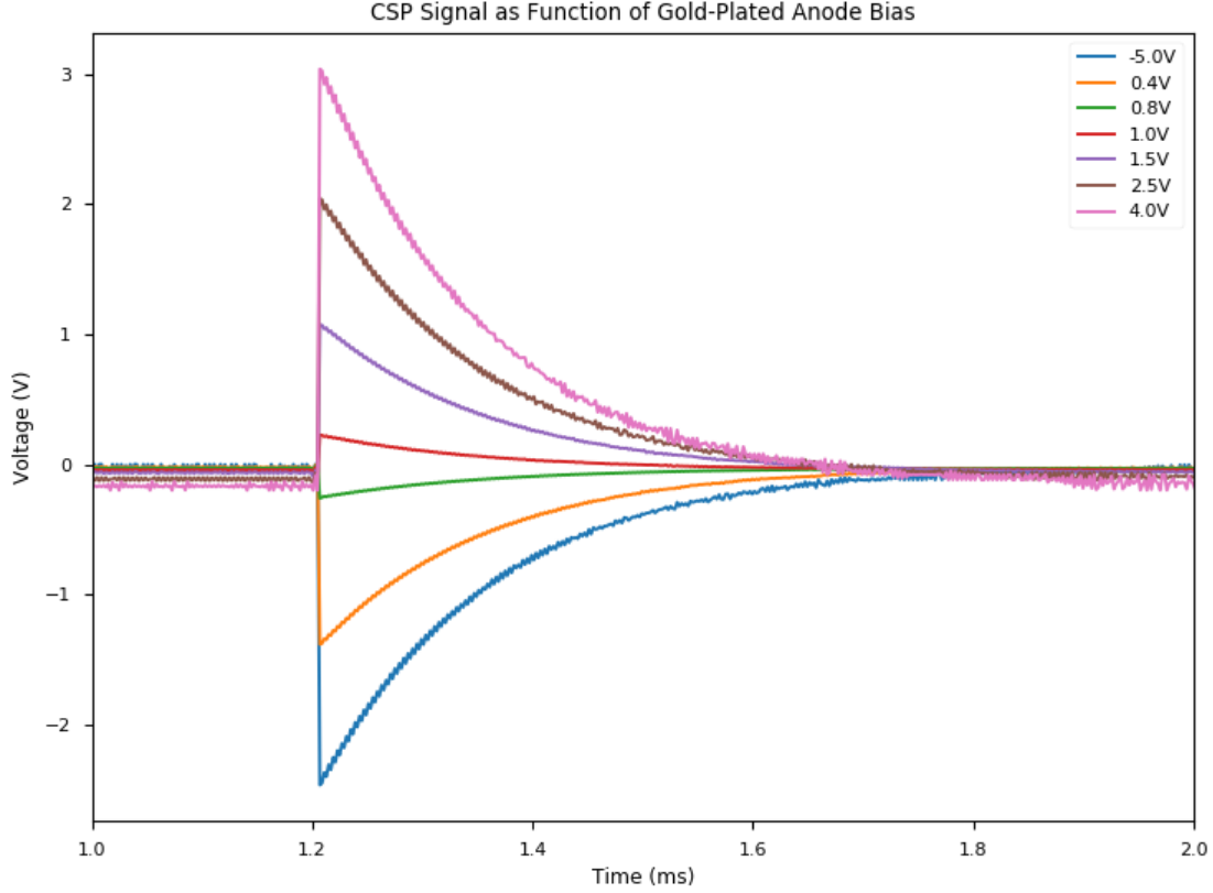
Figure 32: Averaged 200 raw data pulses per bias from the CSP for a variety of biases with the Xe flash lamp and no filter. Note how the amplitude at 0.4 V bias is negative despite the positive polarity of the applied bias. This is a sign of net photoelectron emission from the anode which is overcome by applying higher voltages.
