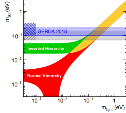
(b) Mass hierarchy regions as functions of \langle m_{\beta\beta} \rangle and the lightest neutrino mass.
