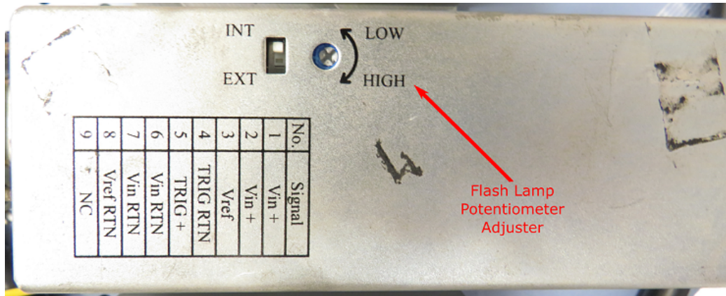
Figure 25: Labeled is the trimmer potentiometer used to adjust the charge stored in the lamp capacitor and therefore the intensity of the light pulses when the lamp is set to internal discharge mode. Next to it is the switch used to change between the discharge modes as well as a table for the required connections to each pin on the lamp's connector.
