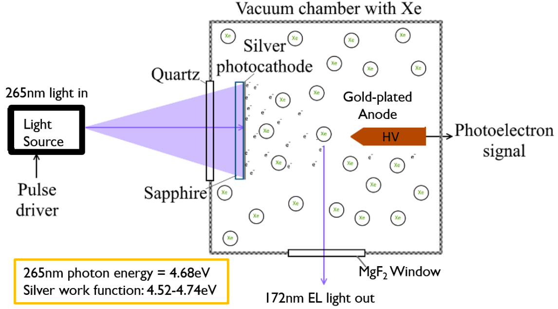
Figure 12: Diagram for the working principle of the ELS. An external UV light source is used to produce photoelectrons from a silver photocathode. Those are drifted in a gas xenon volume, exciting the xenon atoms which produce 172 nm electroluminescent light. The charge signal is collected at an anode, biased with a high voltage (HV), that also generates the drift field, while the light signal is measured with a PMT placed at the MgF 2 window of the vacuum chamber. Figure modified from [79].
