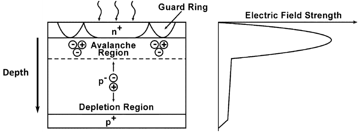
Figure 8: Structure of a single photon avalanche photodiode on the left. When photons create electron-hole pairs, the electric field in the depletion region accelerates electrons creating more pairs, resulting in a charge avalanche. The electric field strength in the p-n junction is demonstrated on the right [55].
