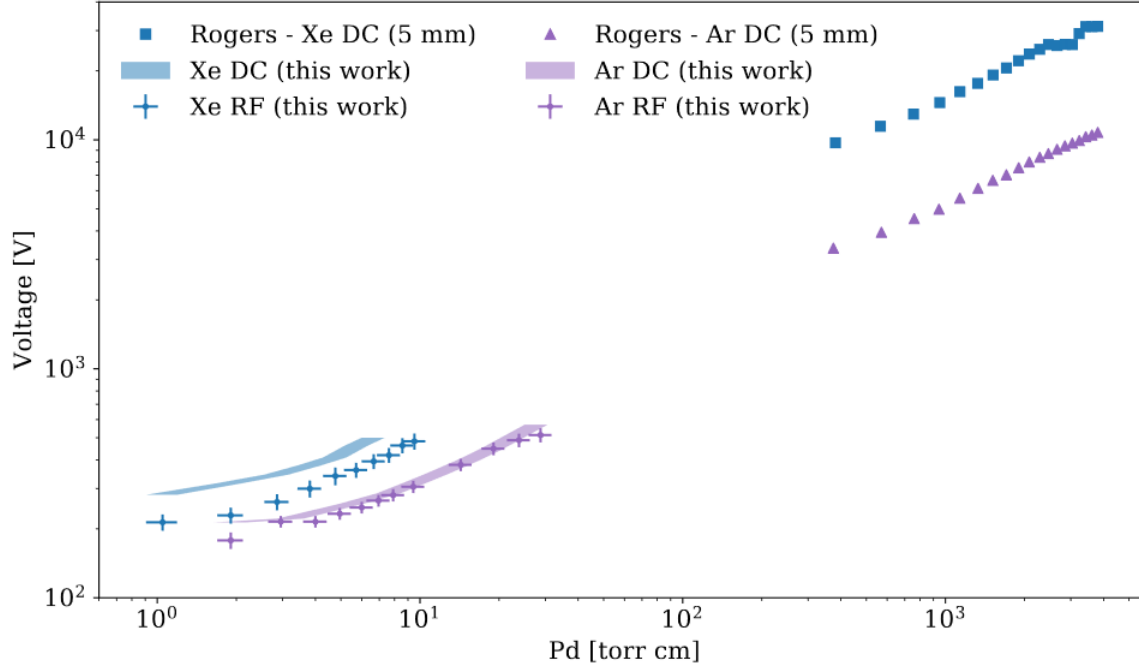
Figure 18: Breakdown voltage threshold in gas xenon as a function of pressure multiplied by distance between electrodes. This plot and the data for Pd < 10^2 Torr are from [95] while the data for Pd > 10^2 is from [96].
