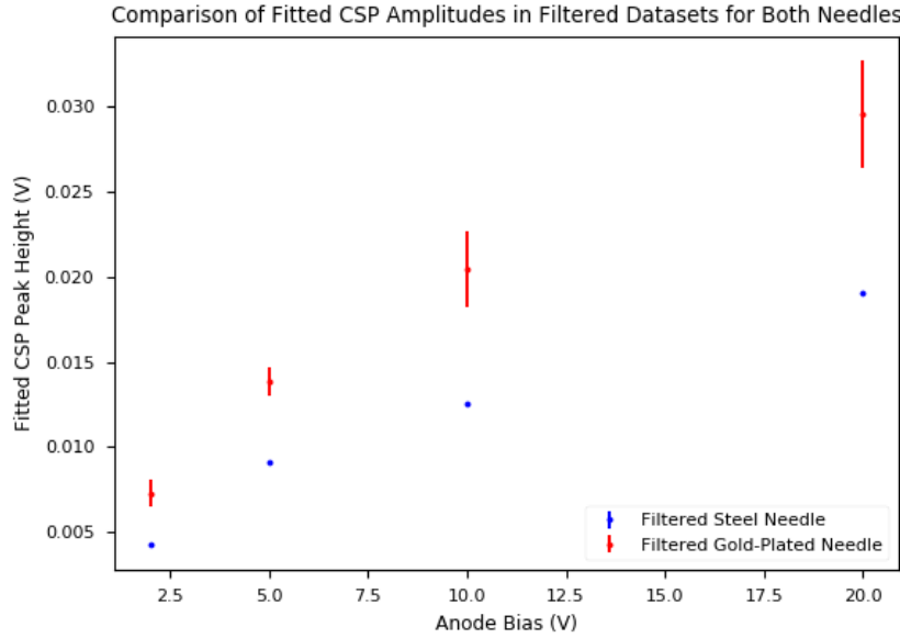
Figure 36: Comparison of charge signals for both needle geometries at various biases. The output for the gold-plated needle measurements was 50 \Omega terminated (to reduce noise in that dataset) unlike for the steel needle, which results in the output being halved. This is a good example of the steel needle’s very short range field. The Xe flash lamp was kept at the same distance relative to the photocathode for both datasets so the difference is not attributed to difference in incident light flux.
