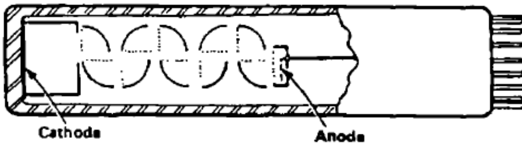
Figure 29: Schematic of the box and grid geometry for a PMT. Photoelectrons are emitted when a photon strikes the cathode and are attracted to a series of dynodes, each at progressively higher bias than the previous one. When an electron strikes a dynode, the energy transfer liberates secondary electrons creating a cascade, a process which greatly multiplies the e^- to form a measurable current collected at the anode. This electron multiplication process allows PMTs to commonly reach gains of 10^5 - 10^6 [56].
