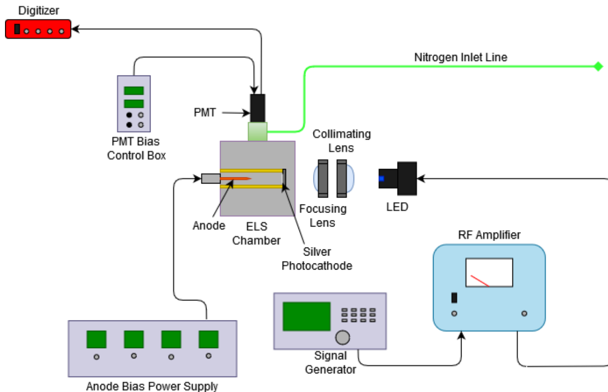
Figure 31: A diagram of all the components involved in producing and measuring electro-luminescent light pulses. Illustrated are also all the signals involved in the measurement as well as the nitrogen inlet line to purge the volume of air between the \text{MgF}_2 window and the face of the PMT.
