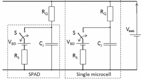
Figure 9: Circuit schematic for a silicon photomultiplier. Multiple SPAD cells in parallel represent the individual pixels of a SiPM. The bias voltage V_{BIAS} is set to be above the SPAD's breakdown voltage. C_J and R_S represent the capacitance and resistance of the SPAD p-n junction, respectively. R_Q is a quenching resistor in charge of stopping the avalanche process [57].
