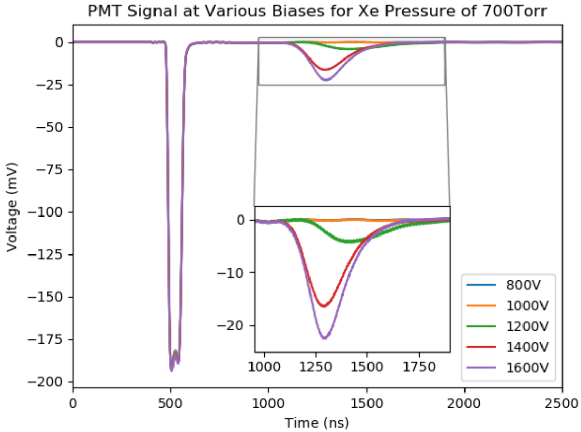
Figure 41: Raw data traces from Root imported in Python for various biases. Notice the digitizer's ability to fit both the full leakage pulse and the EL pulse without losing resolution. Data points are taken every 2 ns and a full trigger window lasts for 2.5 \mu s.
