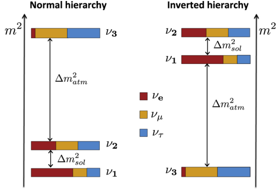
(a) Neutrino mass hierarchy scale with relative contributions from each flavour.
