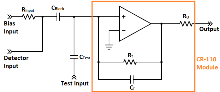
(b) Simplified circuit diagram of the CSP.
