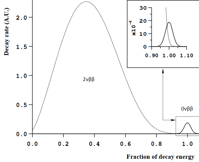
Figure 5: Summed electron kinetic energy spectrum normalized to 1 (dotted curve) for 2\nu\beta\beta decays. The secondary smaller peak corresponds to 0\nu\beta\beta decays normalized to 10^{-2} , in the inset this peak is normalized to 10^{-6} . The signal corresponding to 0\nu\beta\beta decays is a distribution rather than a delta function because energy collection is governed by Poisson statistics, where the number of detected photons for a 0\nu\beta\beta is distributed around the Q value [41].
