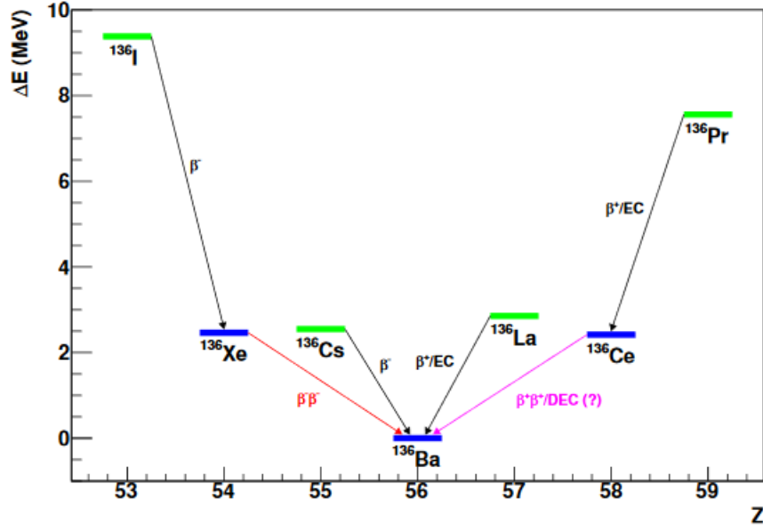
Figure 1: Energy Levels of A=136 isobars. Given ^{136}\text{Xe} cannot reach a lower energy state through a single beta decay, it must undergo double beta decay to ^{136}\text{Ba} . ^{136}\text{Ce} can theoretically decay to the same daughter isotope through double electron capture or double \beta^+ decay but this has not yet been experimentally observed. Figure from [12].
