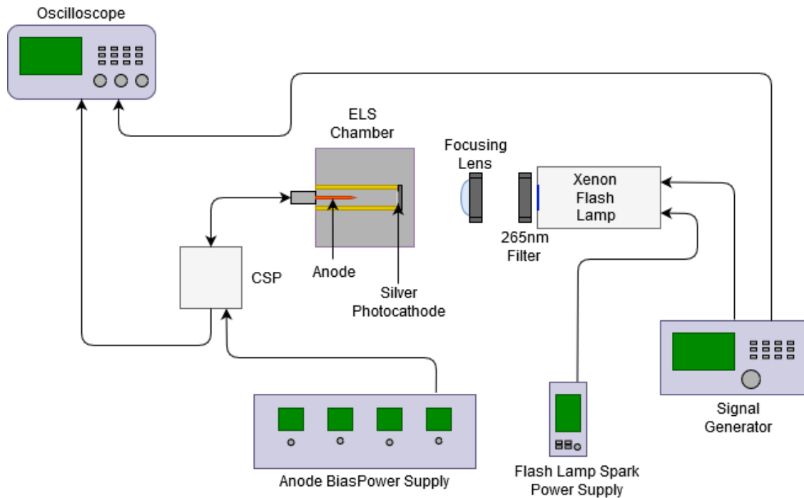
(b) Diagram of the Full Charge Collection Setup.
