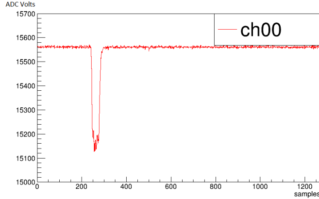
Figure 30: Raw data for a single trigger of an 80 ns LED leakage pulse on the digitizer GUI. The y-axis represents the ADC Voltage and the x-axis the time samples, where the time difference between two time samples is 2 ns.
