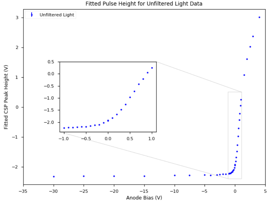
(a) Pulse height vs. anode bias with Xe lamp.
