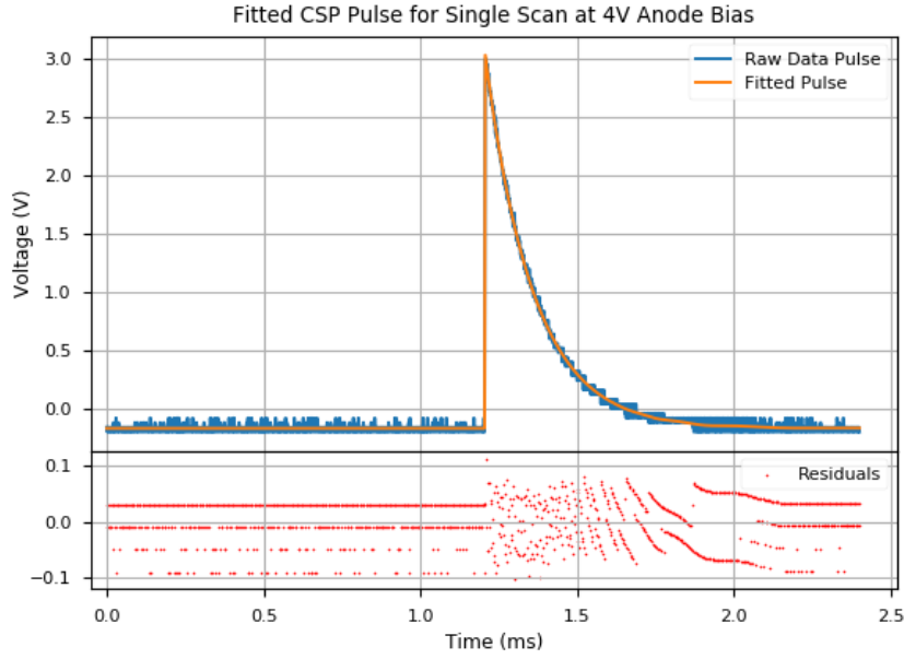
Figure 33: Fit of an individual raw data trace from the charge sensitive preamplifier taken with no filter and +4 V anode bias. The units of the residuals are the same as those for the main plot. Furthermore the residual uncertainties are \sim 0.06 V but were not included as they cause major clutter given the amount of data points.
