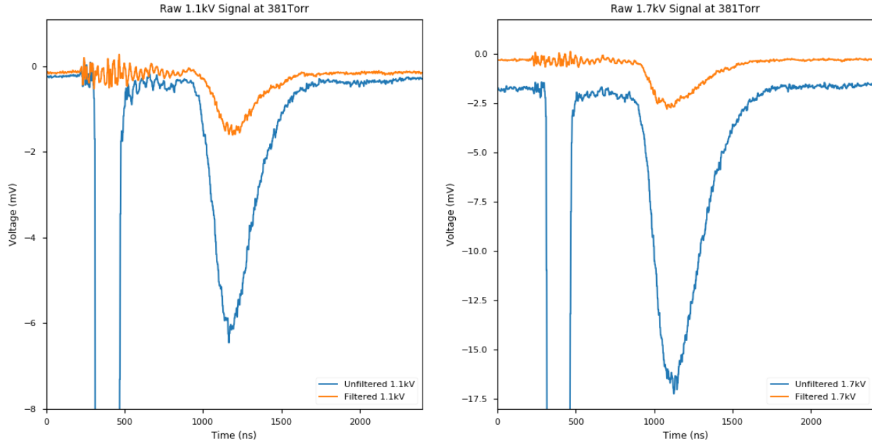
Figure 40: On the left: Raw data with and without 172 nm filter in front of the PMT at 1.1 kV. On the right: same data but at a 1.7 kV bias. When the leakage pulse is attenuated the electronic noise left is due to the signal generator input into the LED.
