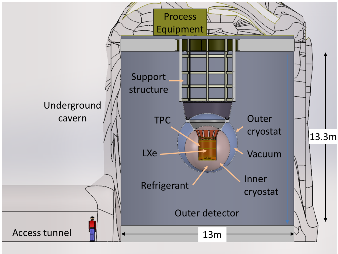
Figure 6: Conceptual design of the nEXO detector, located in an underground cavern. Shown are the LXe TPC surrounded by two layers of cryostats; the HFE-7000 filled cryostat provides the cooling power to keep the xenon liquid and double as a \gamma ray shield. Meanwhile the vacuum cryostat provides thermal insulation. There is an additional outer detector which consists of a large water tank used to reduce cosmogenic, \gamma and muon backgrounds [33].
