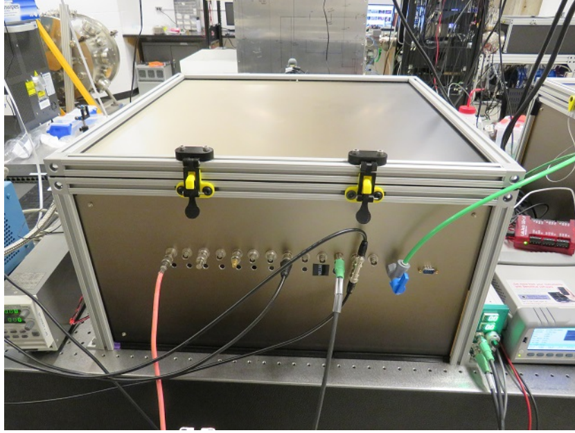
Figure 15: Dark Box to house the electroluminescent light source. The box is fully light-tight to prevent outer light leakage from entering the PMT. The front panel features feedthroughs to power the different electronics inside the box such as the CSP, PMT, the 265 nm light sources and to read the output signals, as well as a feedthrough valve for the nitrogen gas purge. All panels are electrically grounded to the optical table to prevent RF signal pickup from other experiments.
