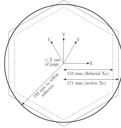
(b) Charge collection wire schematic
