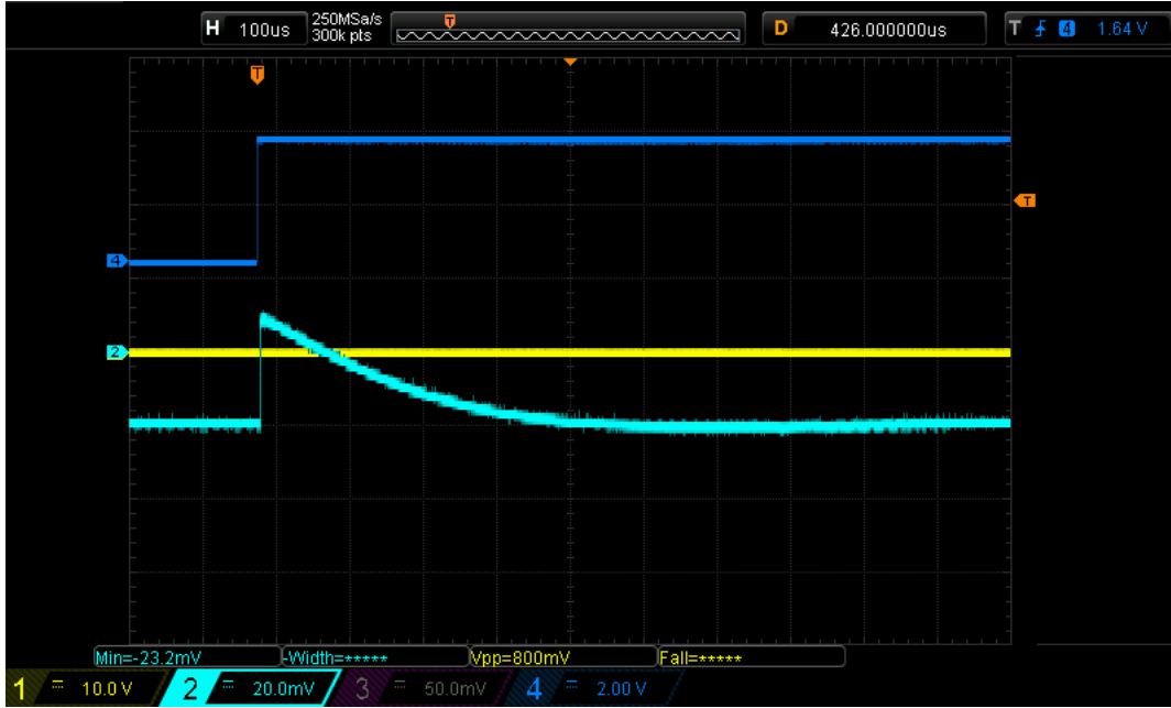
Figure 28: Example of data traces on the oscilloscope for the CSP output pulse (light blue ch. 2) and the Xe Flash Lamp trigger square wave (dark blue ch. 4). In this example, the bias applied to the anode is 50 V which results in a positive peak. For negative biases, where electrons are being emitted from the anode needle rather than collected, the peak has a negative amplitude. This negative amplitude plateaus in magnitude relatively quickly in the negative bias region.
