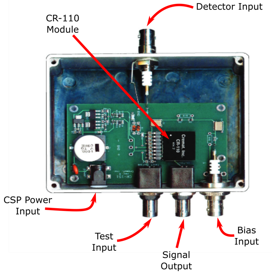
(a) Main input/output ports of the Cremat CSP.
