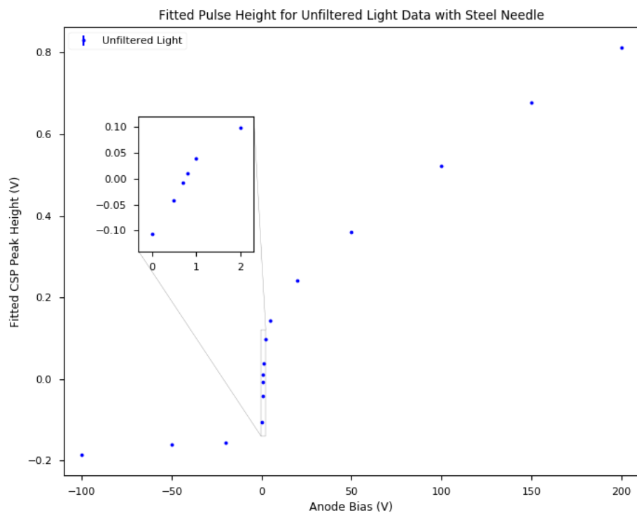
(a) Pulse height vs. anode bias with Xe lamp.
