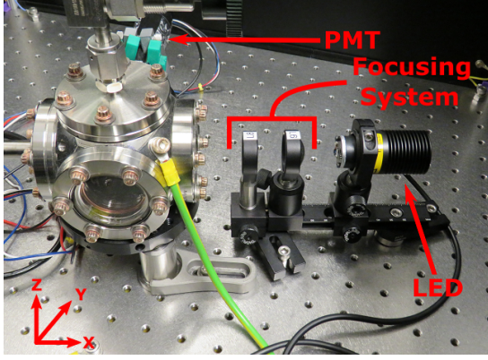
(a) LED and Lens Focusing System.
