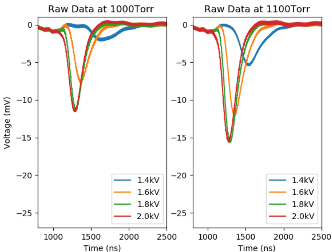
Figure 48: Comparison of 4 biases for pressures of 1000 Torr and 1100 Torr showing systematically smaller EL pulses at 1000 Torr pressure.
