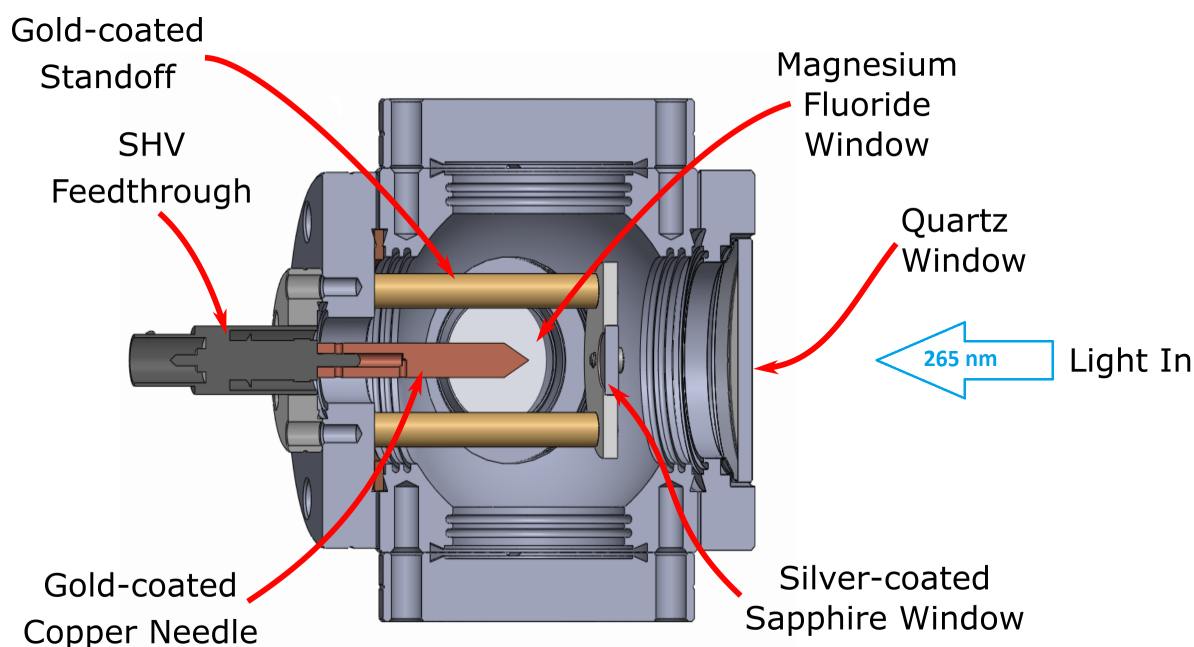
Figure 16: Inner structure of the ELS vacuum chamber. Labelled are the main components of the chamber. The anode makes contact with a push-on SHV feedthrough welded to a CF 1.33" flange. Also shown are the three standoffs holding the sapphire window; they are gold-plated like the copper anode, to reduce their susceptibility to photoelectron emission. The quartz and \text{MgF}_2 viewports for light input and output respectively are also labelled.
