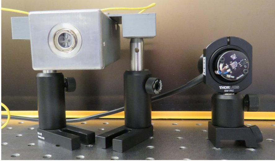
Figure 13: UV light sources used to illuminate the silver photocathode for photoelectron production. On the left is a 5 W Hamamatsu L11035 xenon flash lamp used with a 265 nm bandpass filter (not shown) to limit its normally broad (185-2000 nm) emission spectrum; the filter decreases the lamp's power by about one order of magnitude. On the Right is a 10 mW mounted Thorlabs M265L3 LED with a narrow emission spectrum centered around 265 nm (11 nm FWHM) [85].
