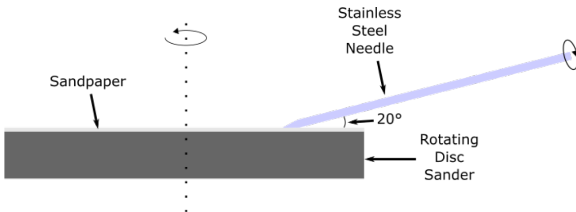
Figure 22: Diagram of the machining process for the stainless steel needle. Shown are the rotating disc sander and thin sandpaper as well as the needle itself and the approximate angle of contact with the sand-paper.
