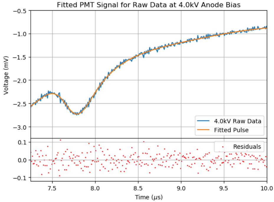
Figure 38: Fit of the 4 kV electroluminescent pulse raw data. Shown are also residuals with uncertainties on the order of 0.1 mV. Even without the inclusion of the afterpulsing contribution there is not any noticeable deviation from the raw data as suggested by the lack of trend on the residuals. The residuals' units are the same as those of the y-axis.
