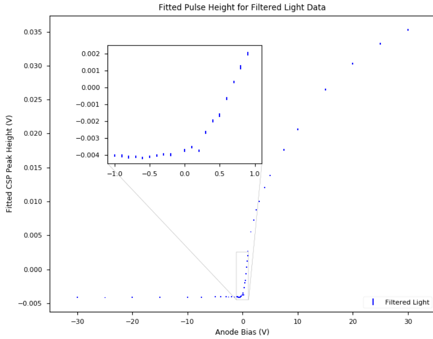
(b) Pulse height vs. anode bias with Xe lamp + 265 nm filter.
