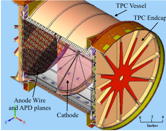
(a) EXO-200 TPC
