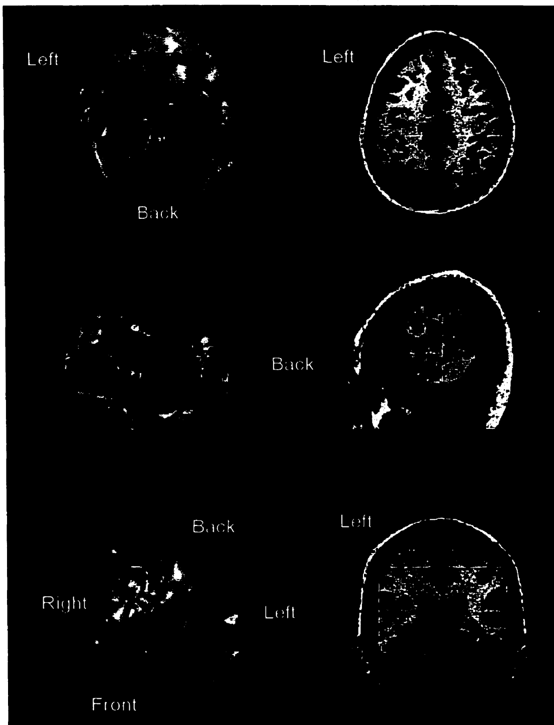
Figure 2.6: Left: 3D statistical parametric maps of local volume increase (red), volume decrease (blue) and structural displacement (yellow) thresholded at the probability 0.025, 0.025, 0.05 (corrected). Right: Statistical parametric maps are superimposed on the axial, sagittal and coronal sections of the atlas brain MRI. The cross-sections are taken at the interior of the largest red cluster inside the purple box (parietal cortex). The white lines indicate where the cross-sections are taken.
