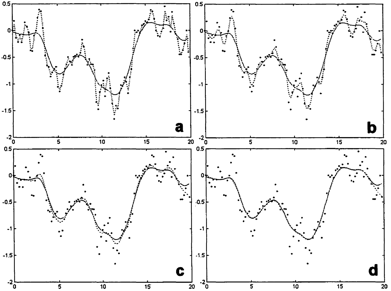
Figure 3.2: Comparison between Gaussian kernel smoothing with the bandwidth parameter h = 1 (solid line) and diffusion smoothing (dotted line). a. before the iteration. b. after 0.05 seconds (5th. iteration). c. after 0.25 seconds (25th. iteration). d. after 0.5 seconds equivalent to h = 1 (50th. iteration).
