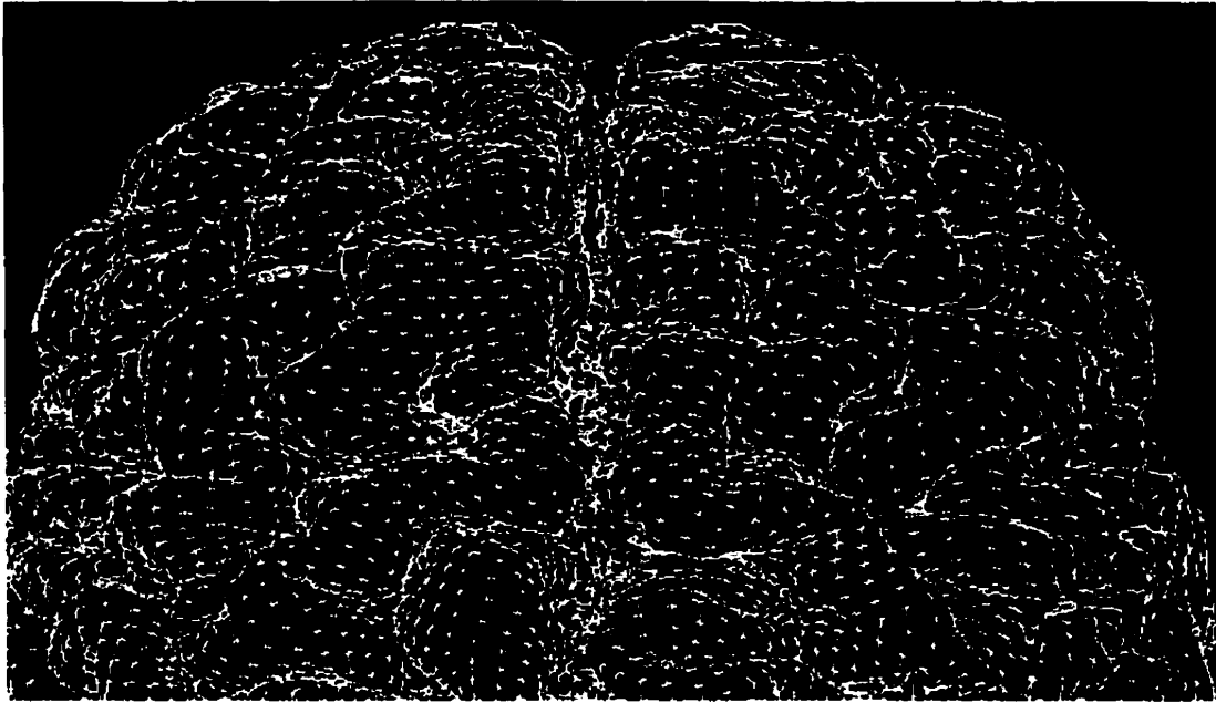
Figure 3.4: A typical triangular mesh of the outer cortical surface consisting of 81,920 triangles and 40,962 vertices.
