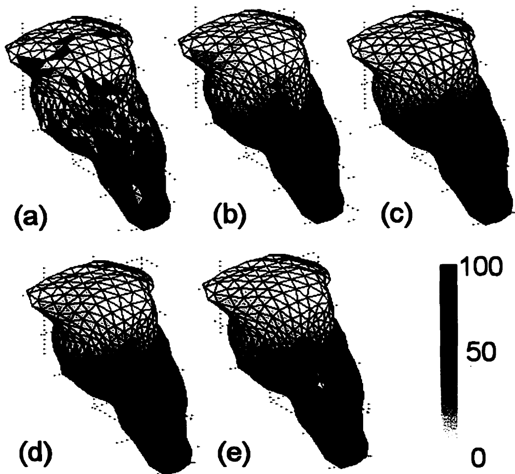
Figure 3.6: Diffusion smoothing of an artificial heat distribution on the triangulated mesh of the brain stem consisting of 1280 triangles. The artificial signal was generated with Gaussian noise to illustrate how the finite difference scheme works with different iteration step sizes. a. The initial heat distribution, b. After 10 iterations with \delta t = 0.5 , c. After 20 iterations with \delta t = 0.5 , d. After 50 iterations with \delta t = 0.2 , e. After 10 iterations with \delta t = 1.5 . Because the iteration step size is large, the iteration breaks down and a singularity (the white spot) begins to appear.
