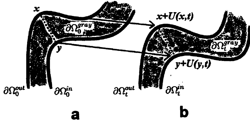
Figure 4.1: Cortical thickness change under the deformation x \rightarrow x + U(x, t) . The linkage between x and y is defined by the ASP algorithm and the cortical thickness is defined as the Euclidian distance \|x - y\| . a. Before the deformation. b. After the deformation.
