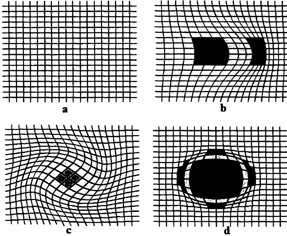
Figure 2.3: Square grid under translation, rotation and volume change. Red: volume increase, Blue: volume decrease, Gray: rotation, Yellow: translation. a. square grid under no deformation. b. Horizontal translation caused by local volume increase on the left side. c. 45 degree clockwise rotation. The rotation induces the outer region of the center of the rotation to translate. d. Volume expansion in the middle causes the grid to radially translate outward.
