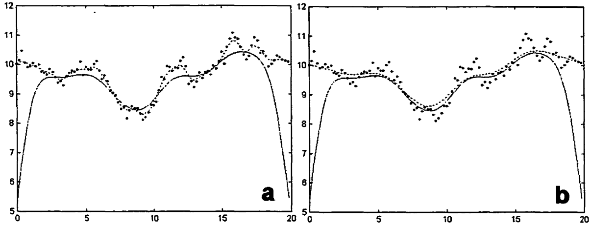
Figure 3.3: Breakdown of Gaussian kernel smoothing with h = 1 at the boundary (red line). Diffusion smoothing solved with the boundary condition (blue dotted line). a. after 0.25 seconds (25th. iteration). b. after 0.5 seconds equivalent to h = 1 (50th. iteration).
