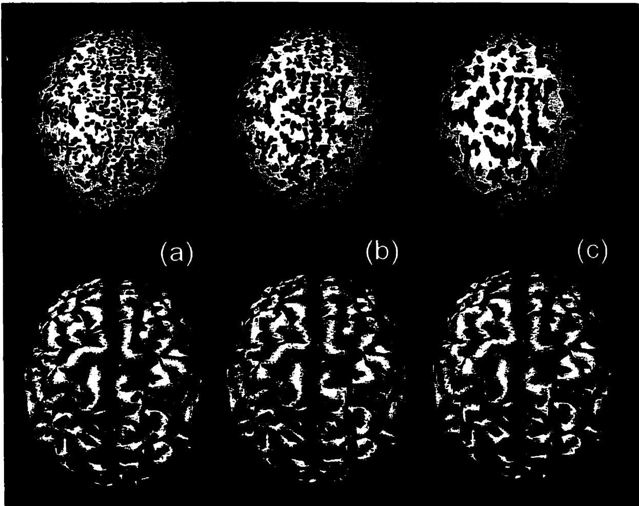
Figure 3.7: The mean curvature of the outer cortex is mapped onto an ellipsoid consisting of 81920 triangles preserving the connectivity. Note that the diffusion was run directly on the cortical surface and mapped onto the ellipsoid later. a. Before the iteration. b. After 40 iterations with \delta t = 0.02 c. After 100 iterations with \delta t = 0.02 . If the smoothing were based on simple internodal averaging, such sulcal pattern can not be obtained.
