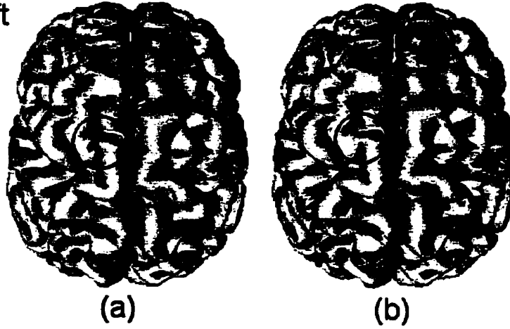
Figure 3.8: Comparison of the parametric method and the finite element method of the diffusion smoothing of the mean curvature in Figure 3.7 c. The extent of smoothing is roughly equivalent to 5mm FWHM Gaussian kernel smoothing in 2D Euclidian space ( \delta t = 0.02 , N = 100 iterations). a. Parametric method. b. The finite element method. The smoothing patterns are slightly different inside the black circle.
