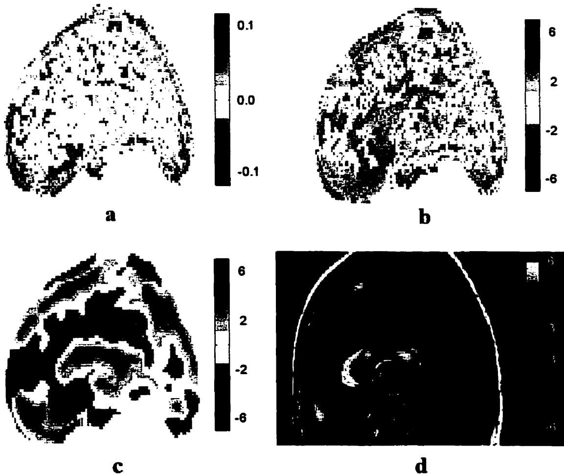
Figure 2.2: The statistical analysis of local volume change data on the mid-sagittal section. a. The sample mean dilatation-rate M_{volume} . It gives an incorrect impression that the local volume change only occurs near the outer cortical boundaries due, perhaps, to registration error. b. t -map of local volume change. Local maxima appear around the corpus callosum. A lot of noise on the cortical boundaries disappears. c. t -map of local volume change after 10mm Gaussian kernel smoothing. The smoothing is applied directly to the displacement fields and the signal-to-noise ratio improves. d. Thresholded t -map superimposed on the mid-sagittal section of the atlas brain. The corpus callosum shows volume increase. When the corrected threshold of t > 6.5 is applied, most of the red regions disappears except the local maximum in the splenium and the isthmus of the corpus callosum.
