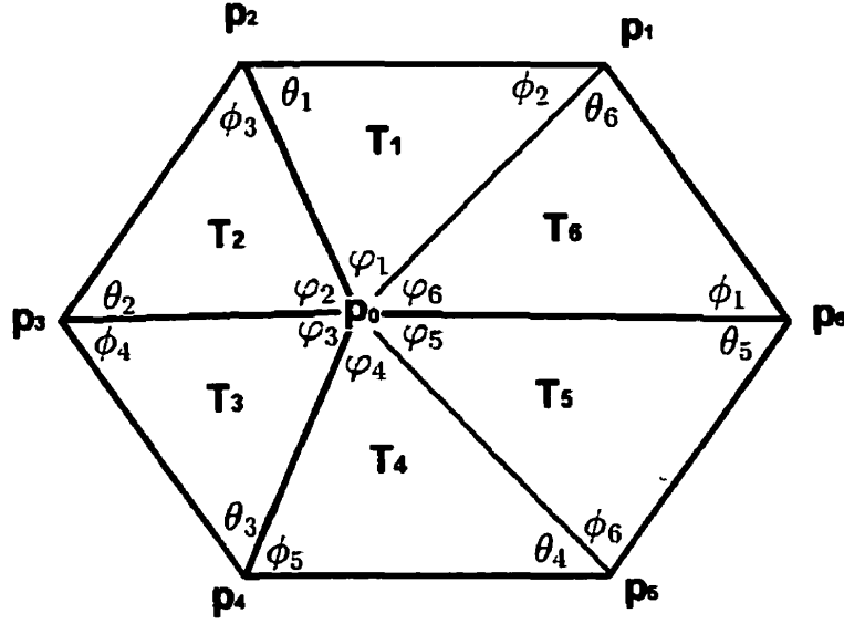
Figure 3.5: A typical triangulation in the neighborhood of \mathbf{p} = \mathbf{p}_0 . The triangulation is either pentagonal or hexagonal in ASP algorithm for 81920 triangles.
