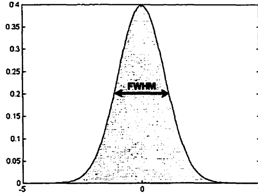
Figure 3.1: FWHM of the Gaussian kernel K(x) .
