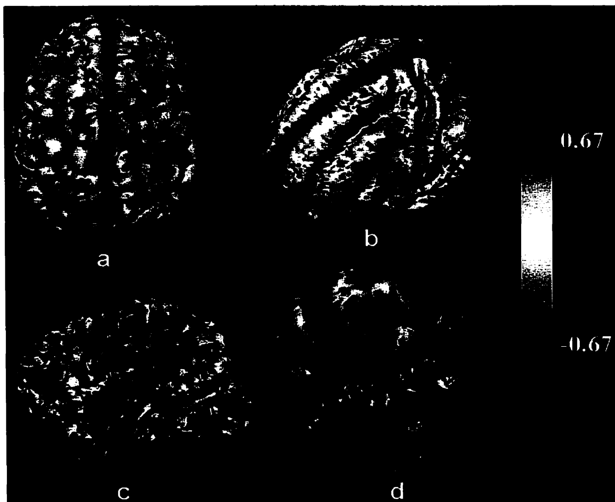
Figure 4.2: Cortical thickness dilatation rate for a single subject. The red (blue) regions show more than 67% thickness increase (decrease). a. The outer cortical surface. b., d. The same data as in a. projected onto the average outer cortical surface of 28 subjects. c. The inner cortical surface. Note the high variabilities of the cortical thickness dilatation rate across the cortex. Due to such large variabilities, surface-based smoothing is required to increase the signal-to-noise ratio.
