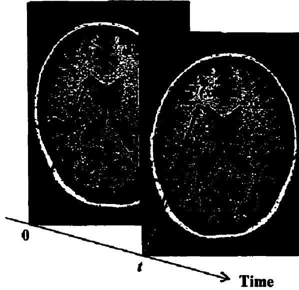
Figure 2.1: The structure at x deforms to the homologous structure at x + U(x, t) after time t .
