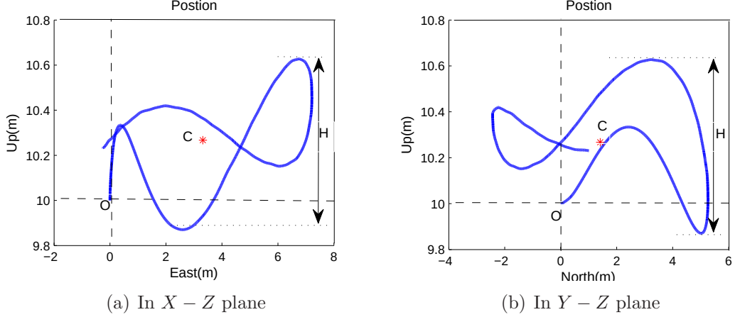
Figure 3–6: ALTAV 360^\circ turning maneuver with present actuator locations
