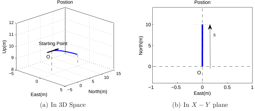
Figure 3-3: ALTAV straight forward maneuver with present actuator locations
