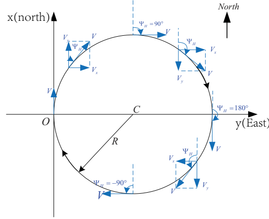
Figure 3–2: Heading angle
