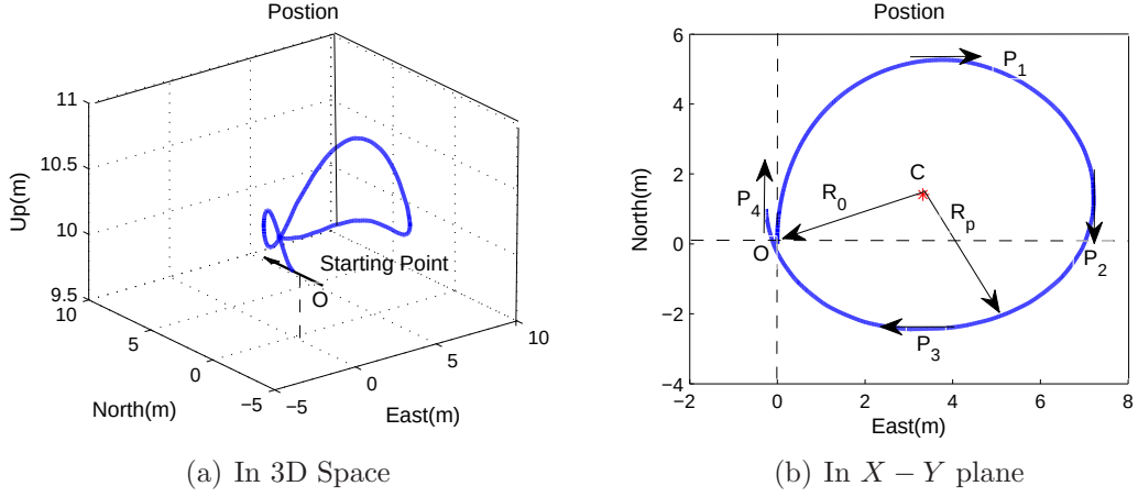
Figure 3–5: ALTAV 360^\circ turning maneuver with present actuator locations
