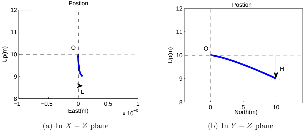
Figure 3-4: ALTAV straight forward maneuver with present actuator locations
