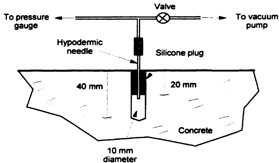
Figure 3-22: Modified Figg air permeability test [27]
