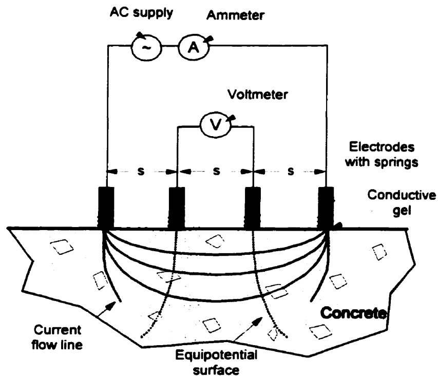
Figure 3-16: Wenner probe set-up [73]
