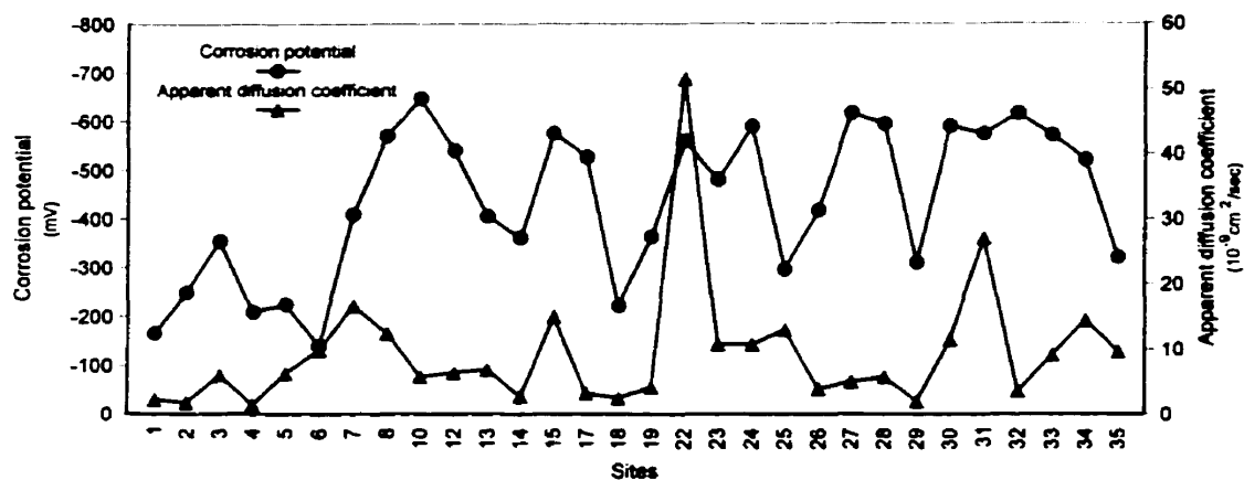
Figure 6-17: Dependence of apparent diffusion coefficient on corrosion potential (entire deck)
