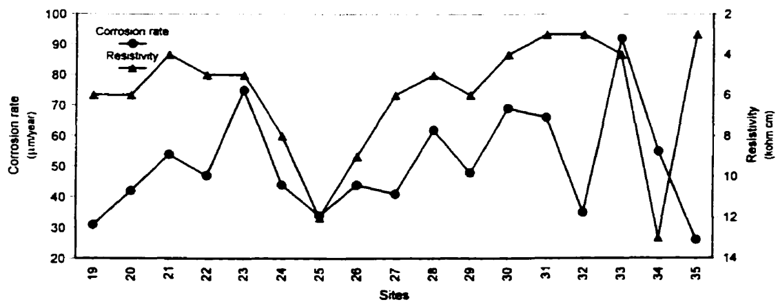
Figure 6-14: Dependence of resistivity of concrete on corrosion rate (west side of deck)
