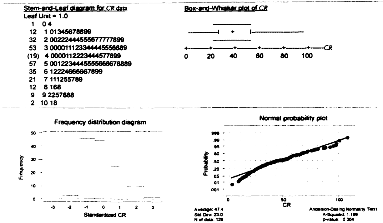
Figure G-3: Analysis 2 for corrosion rate (entire deck)
