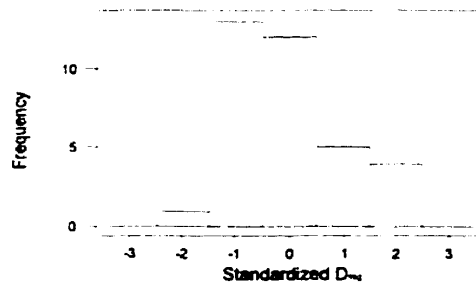
Figure G-12: Analysis 1 for in-situ chloride migration coefficient (entire deck)
