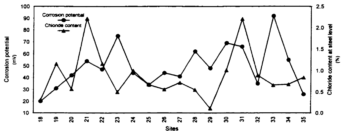
Figure 6-8: Dependence of chloride content at steel level on corrosion potential (west side of deck)
