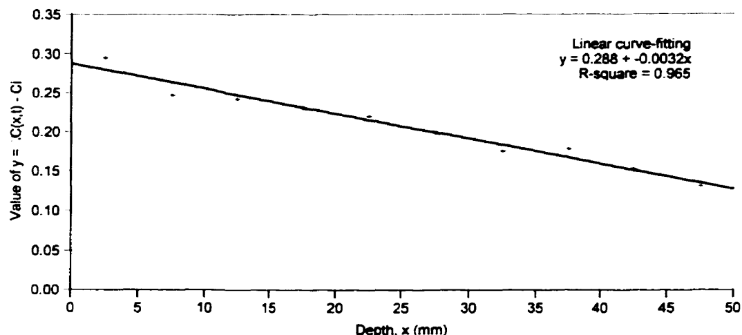
Figure 4-22: Linear regression analysis of the transformed variables (Site 3)
