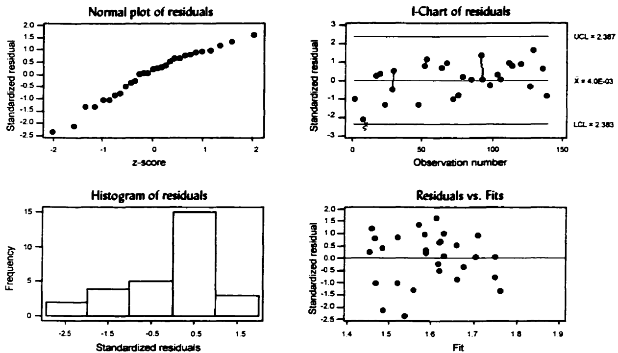
Figure H-4: Standardized residual model diagnostics for '%CI' (entire deck)
