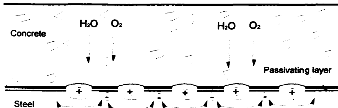
Figure 2-9: General corrosion [33]
