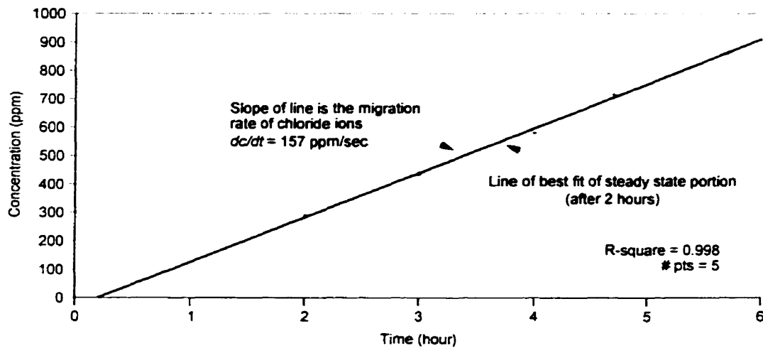
Figure 4-15: Typical concentration vs. time graph for Site 15 (6-hour test duration)
