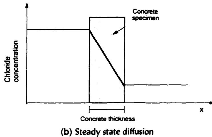
Figure 3-17: Schematic diagram of standard diffusion cell [76, 77] .
