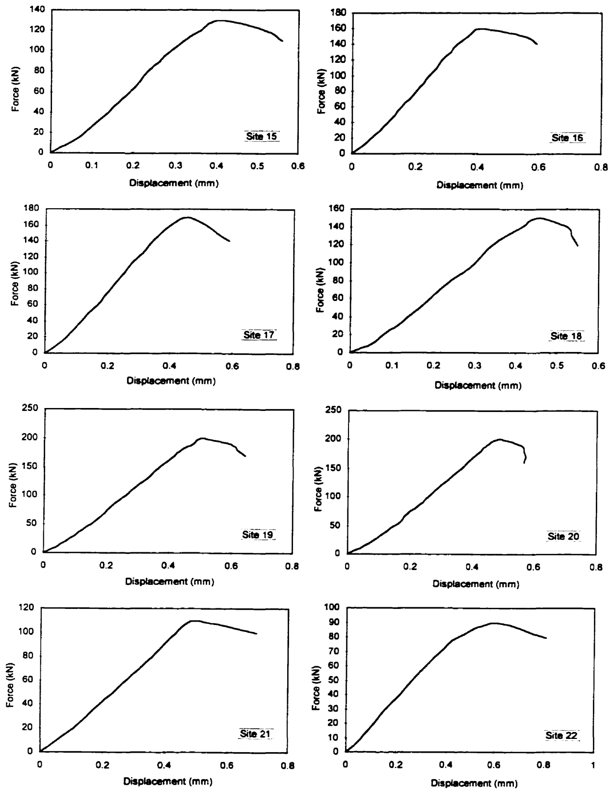
Figure F-3: Force versus displacement plot (Sites 15-22)
