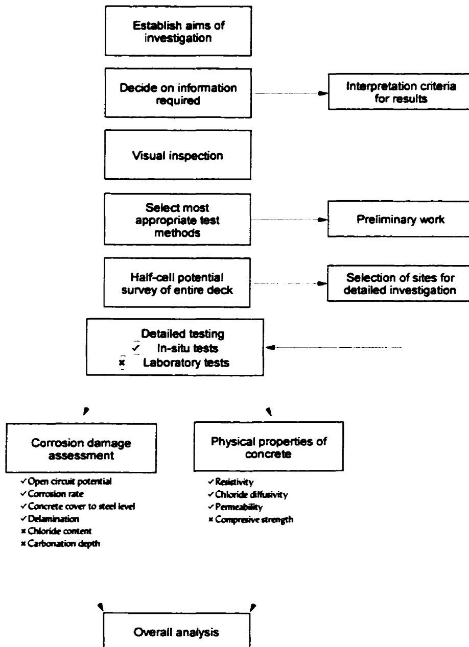
Figure 4-1: Scheme of test program
