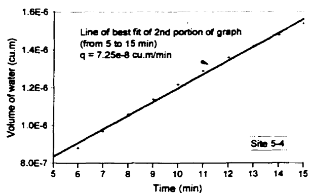
Figure E-1: Steady state slope of volume of water vs. time graphs for Sites 4 and 5
