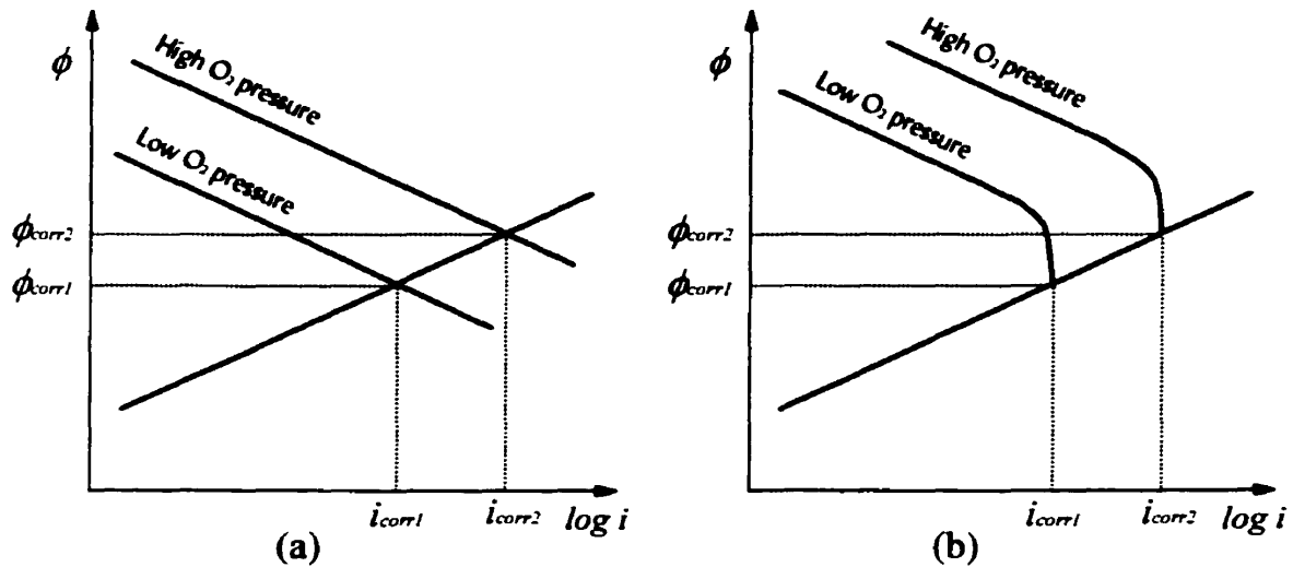
Figure 3-7: Influence of oxygen pressure in activation and concentration polarization [55, 56]
