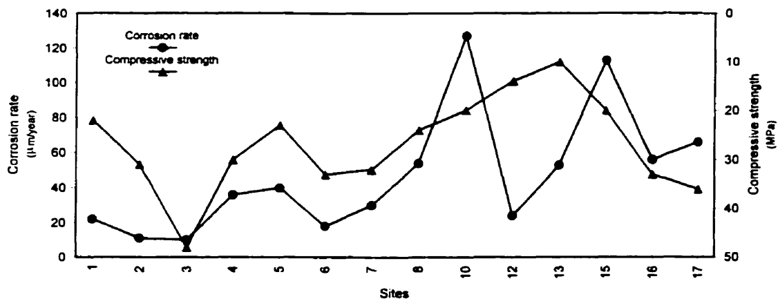
Figure 6-15: Dependence of concrete compressive strength on corrosion rate (east side of deck)
