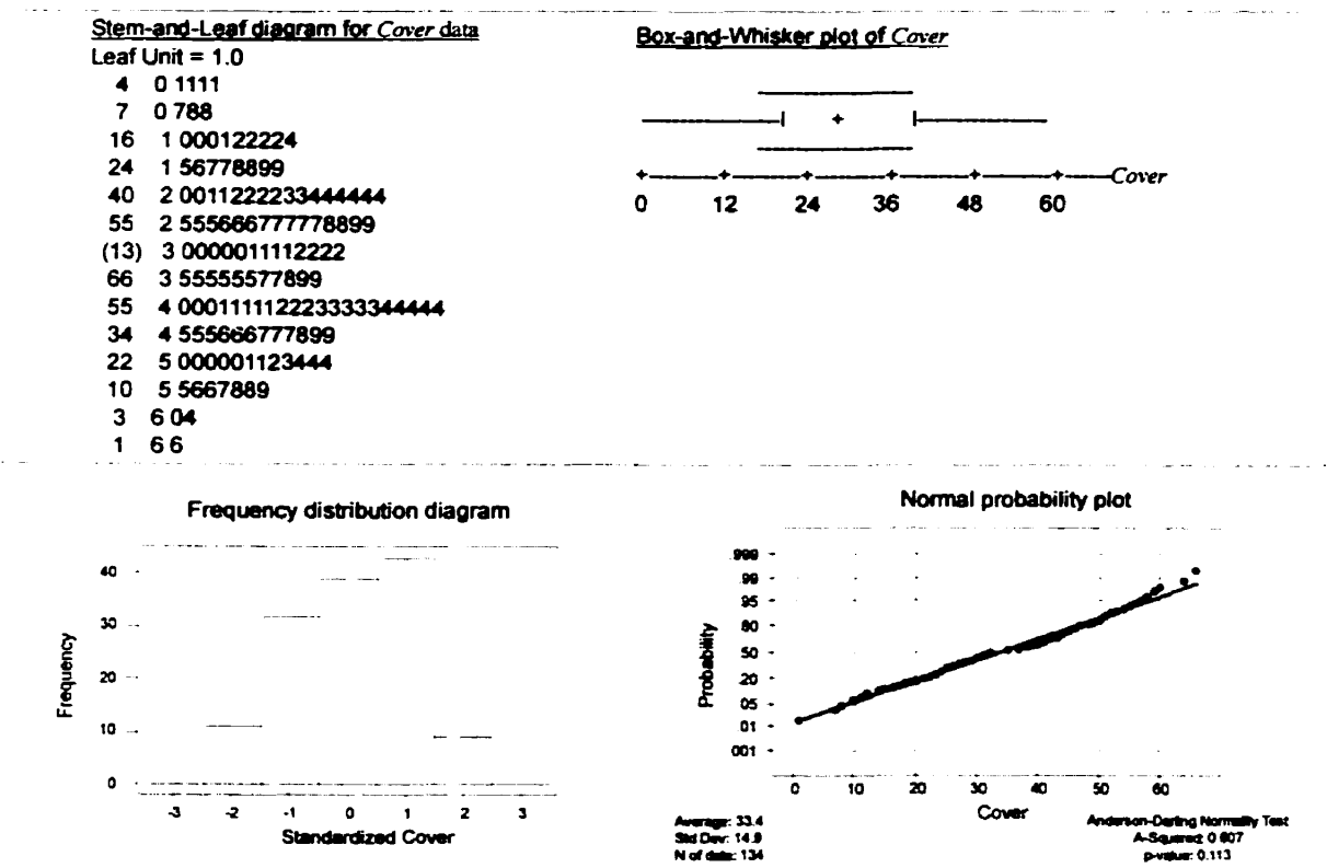
Figure G-6: Analysis 2 for concrete cover thickness (entire deck)
