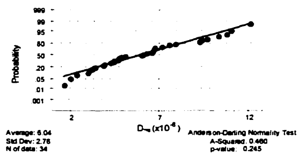
Figure G-13: Analysis 2 for in-situ chloride migration coefficient (entire deck)
