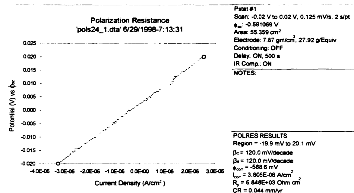
Figure B-1: Polarization resistance plot (Site 24, location 1)
