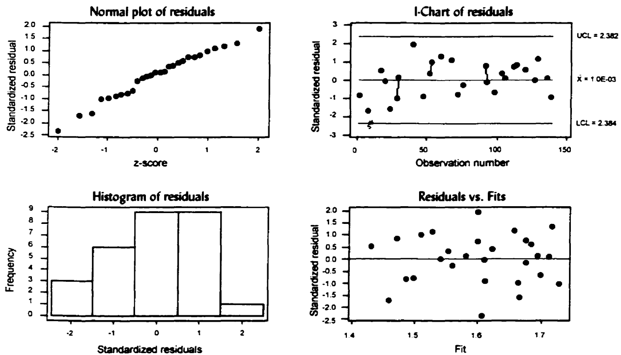
Figure H-5: Standardized residual model diagnostics for 'LogDa' (entire deck)
