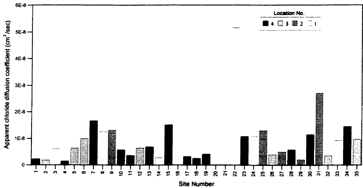
Figure A-8: Apparent chloride diffusion coefficient values
