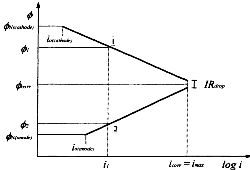
Figure 3-2: Electropotential vs. Current density [56]
