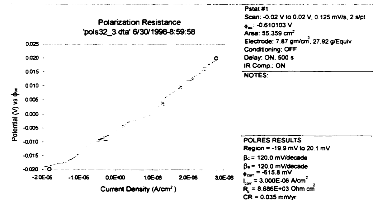
Figure B-15: Polarization resistance plot (Site 32, location 3)
