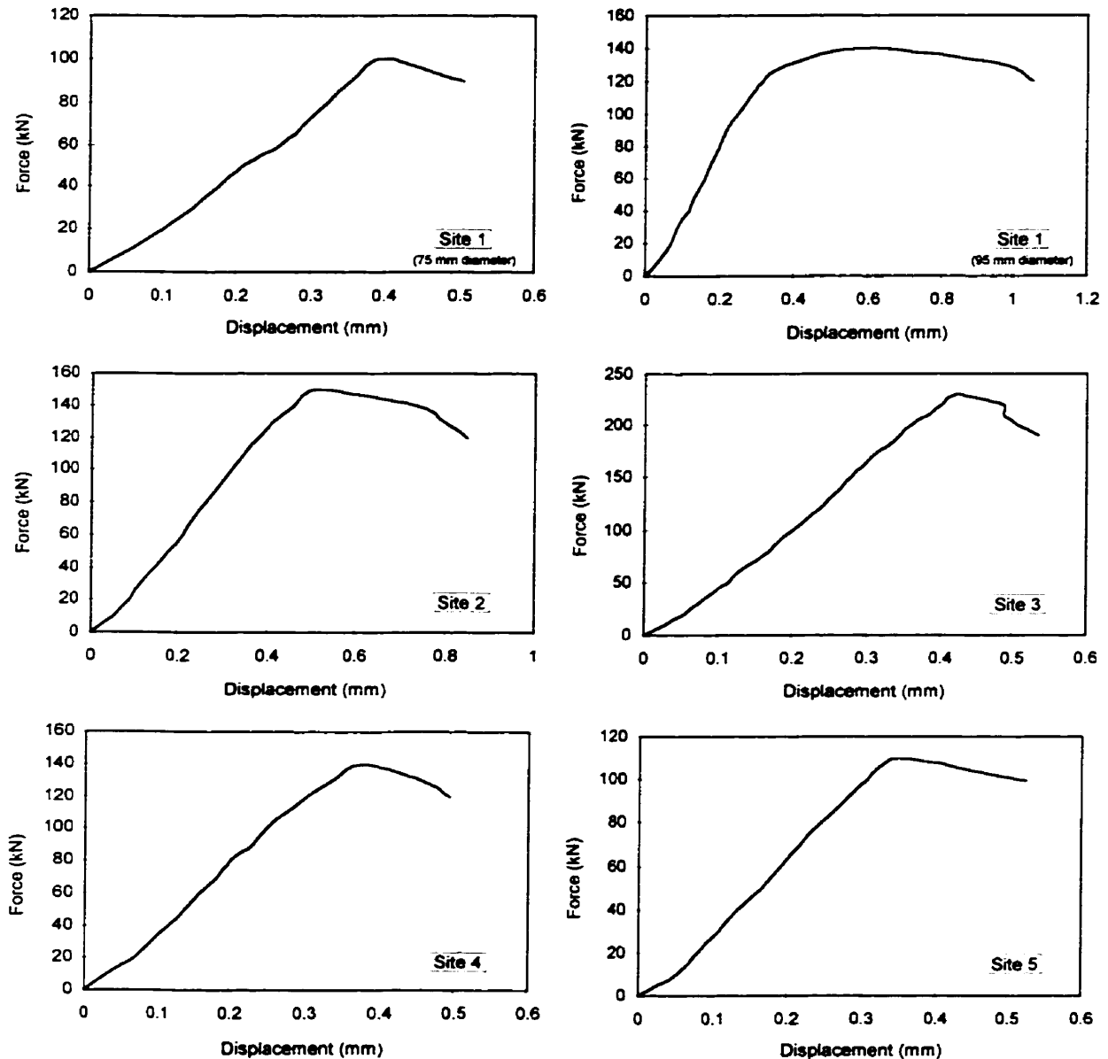
Figure F-1: Force versus displacement plot (Sites 1-5)
