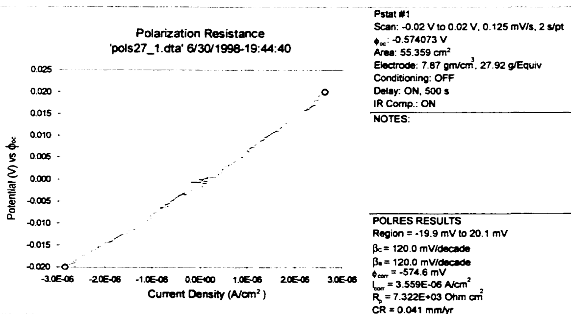
Figure B-9: Polarization resistance plot (Site 27, location 1)
