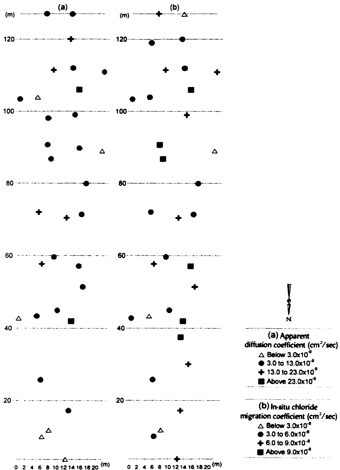
Figure 5-12: Chloride diffusivity results
