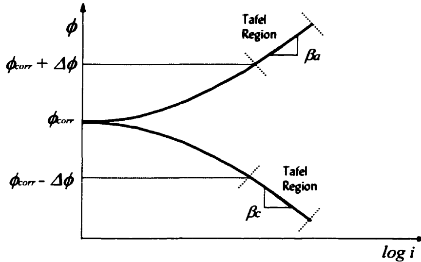
Figure 3-13: Tafel regions [66]
