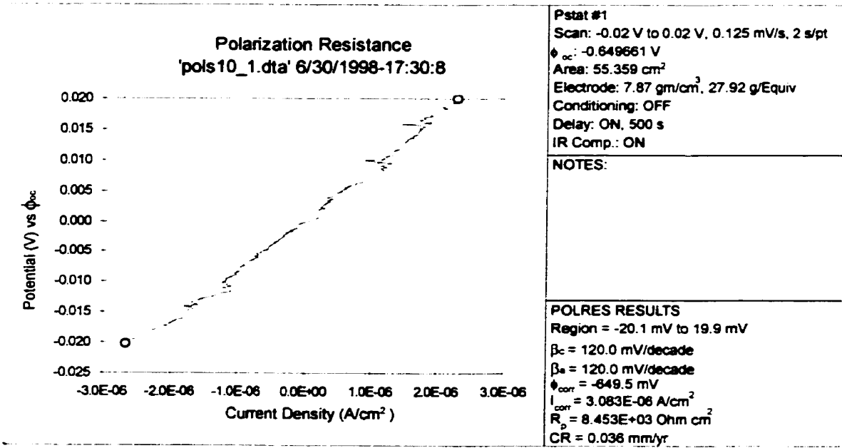
Figure 4-11: Typical polarization resistance plot (Site 10, location 1)
