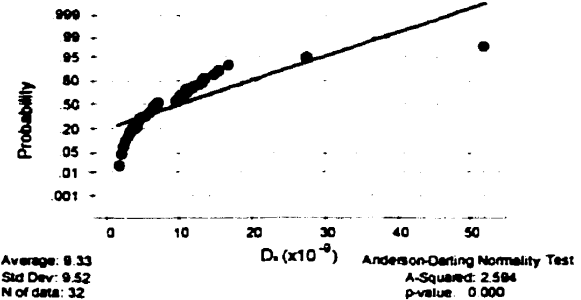
Figure G-9: Analysis 1 for apparent chloride diffusion coefficient (entire deck)
