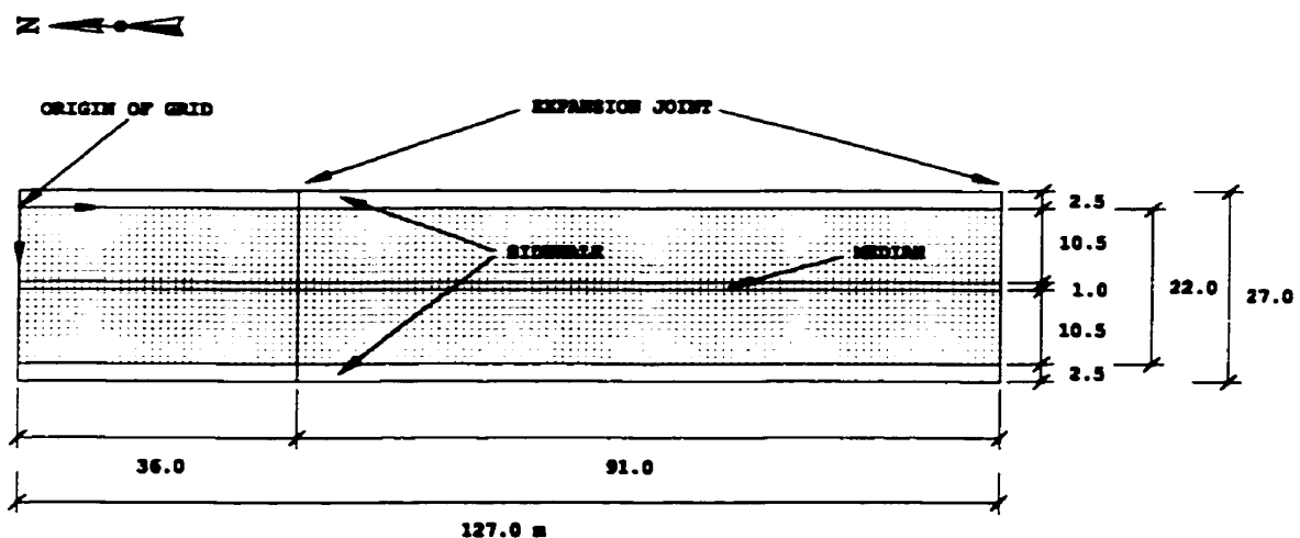
Figure 4-2: North section of bridge deck (detail from Figure 1-3)
