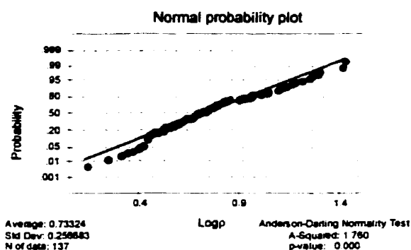
Figure G-17: Analysis 3 for resistivity of concrete (entire deck)
