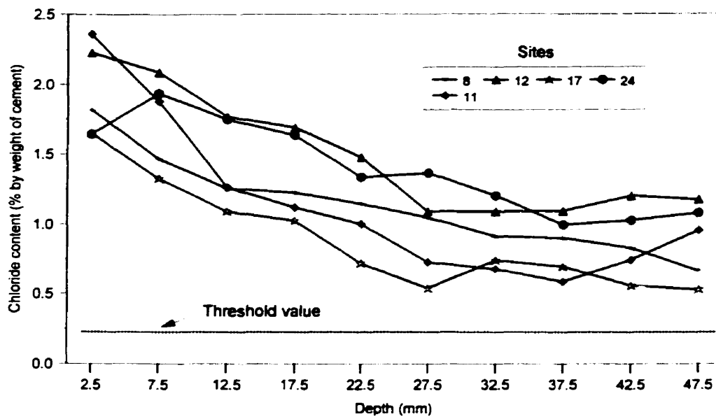
Figure 4-20: Concentration chloride profiles through concrete (Sites 8, 11, 12, 17 and 24)
