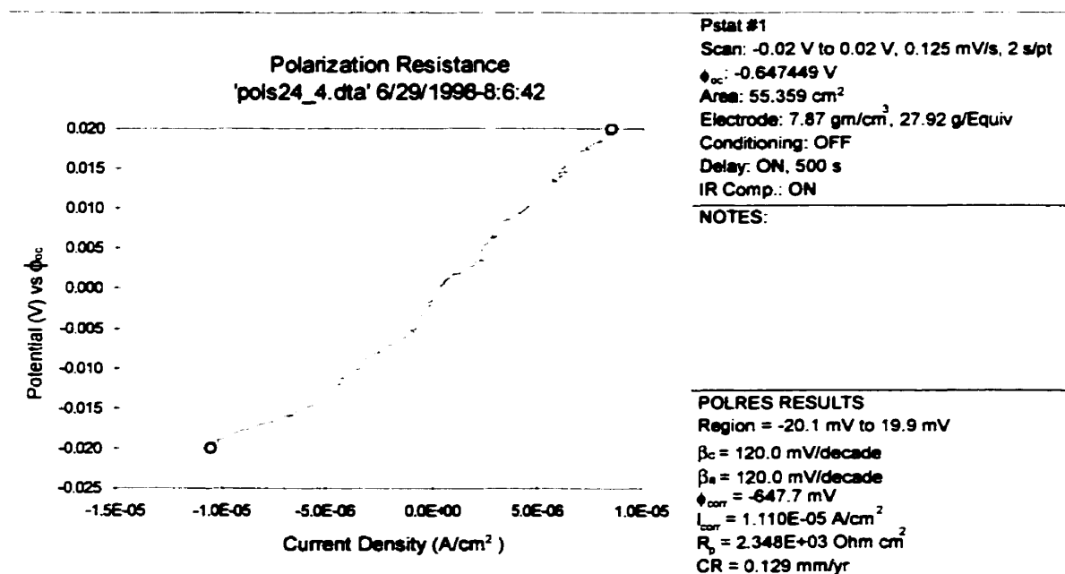
Figure B-4: Polarization resistance plot (Site 24, location 4)
