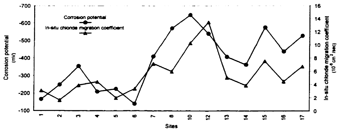
Figure 6-3: Dependence of in-situ chloride migration coefficient on corrosion potential (east side of deck)
