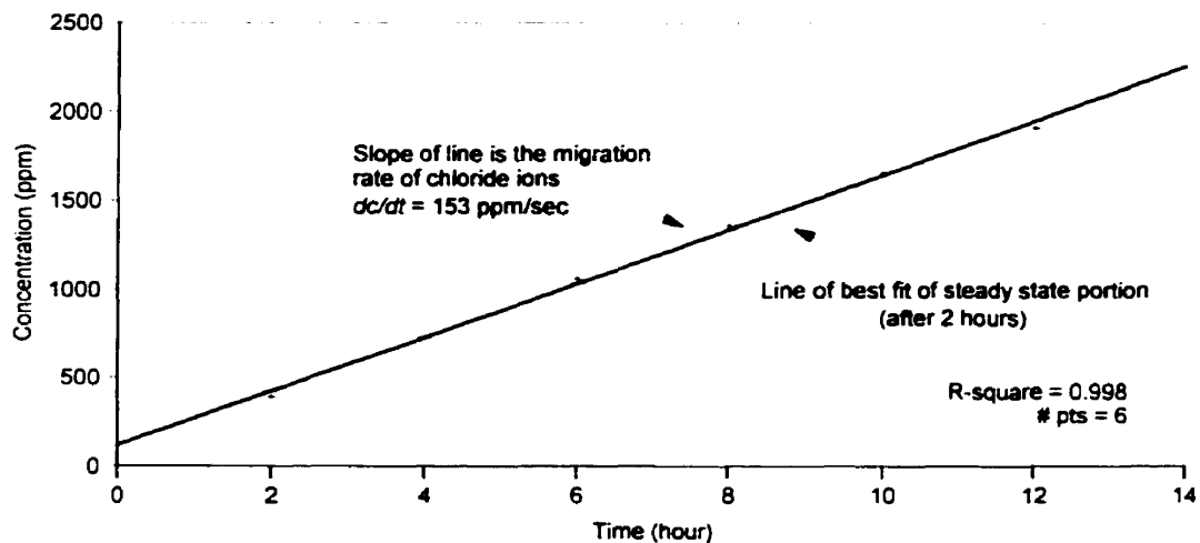
Figure 4-16: Concentration vs. time plot for Site 15 (12-hour test duration)
