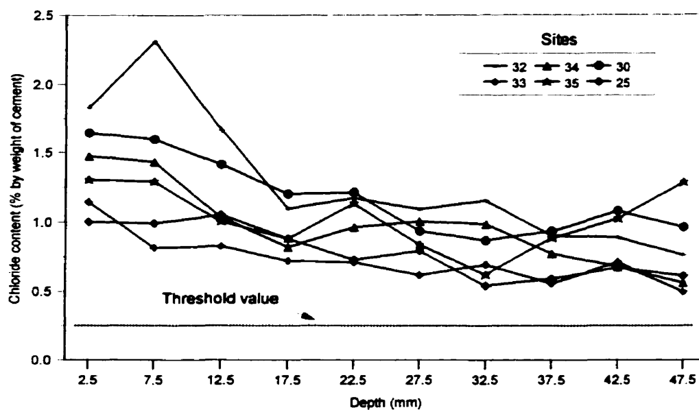
Figure D-2: Chloride profiles (Sites 25,30 and 32-35)
