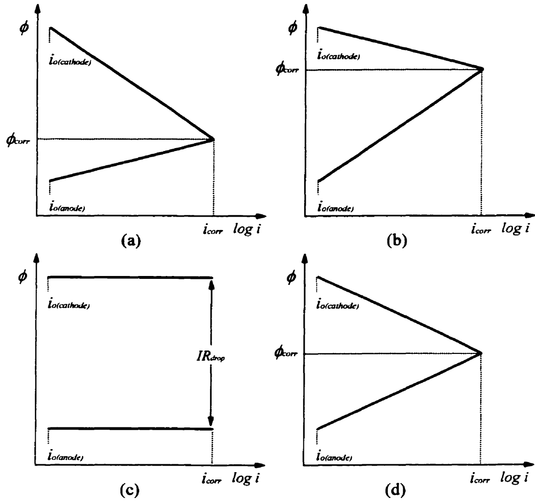
Figure 3-6: Types of corrosion control [55]
