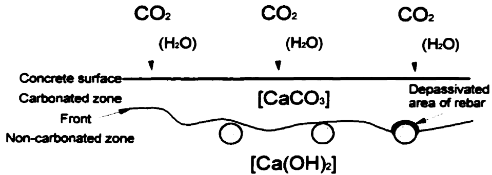
Figure 2-3: Schematic representation of the carbonation process [45]
