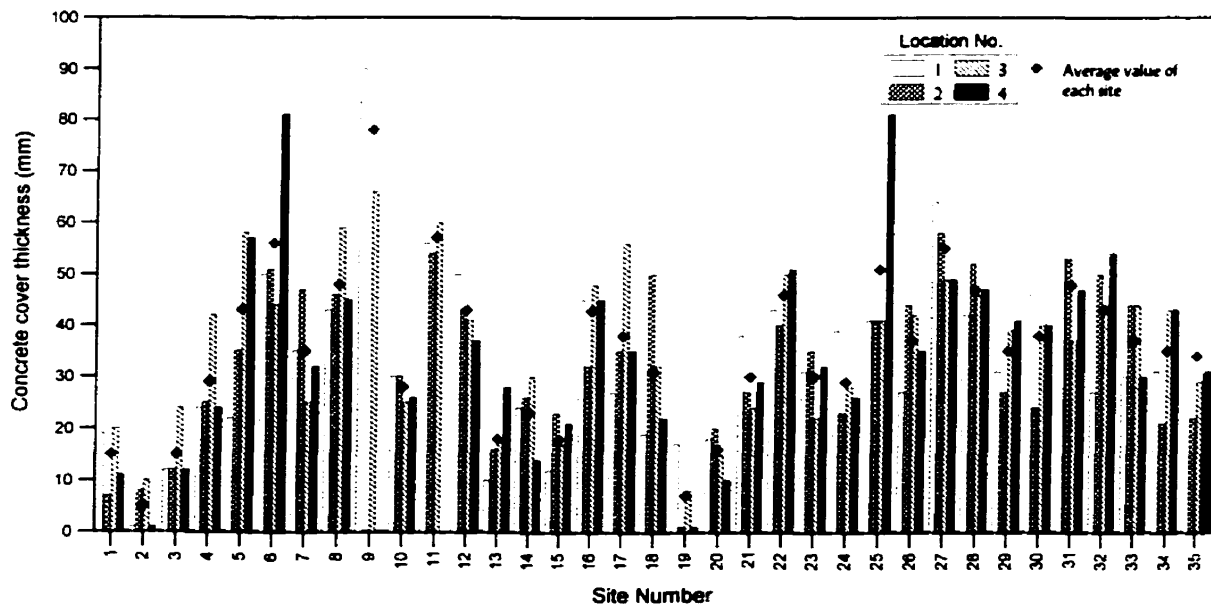
Figure A-1: Concrete cover thickness survey
