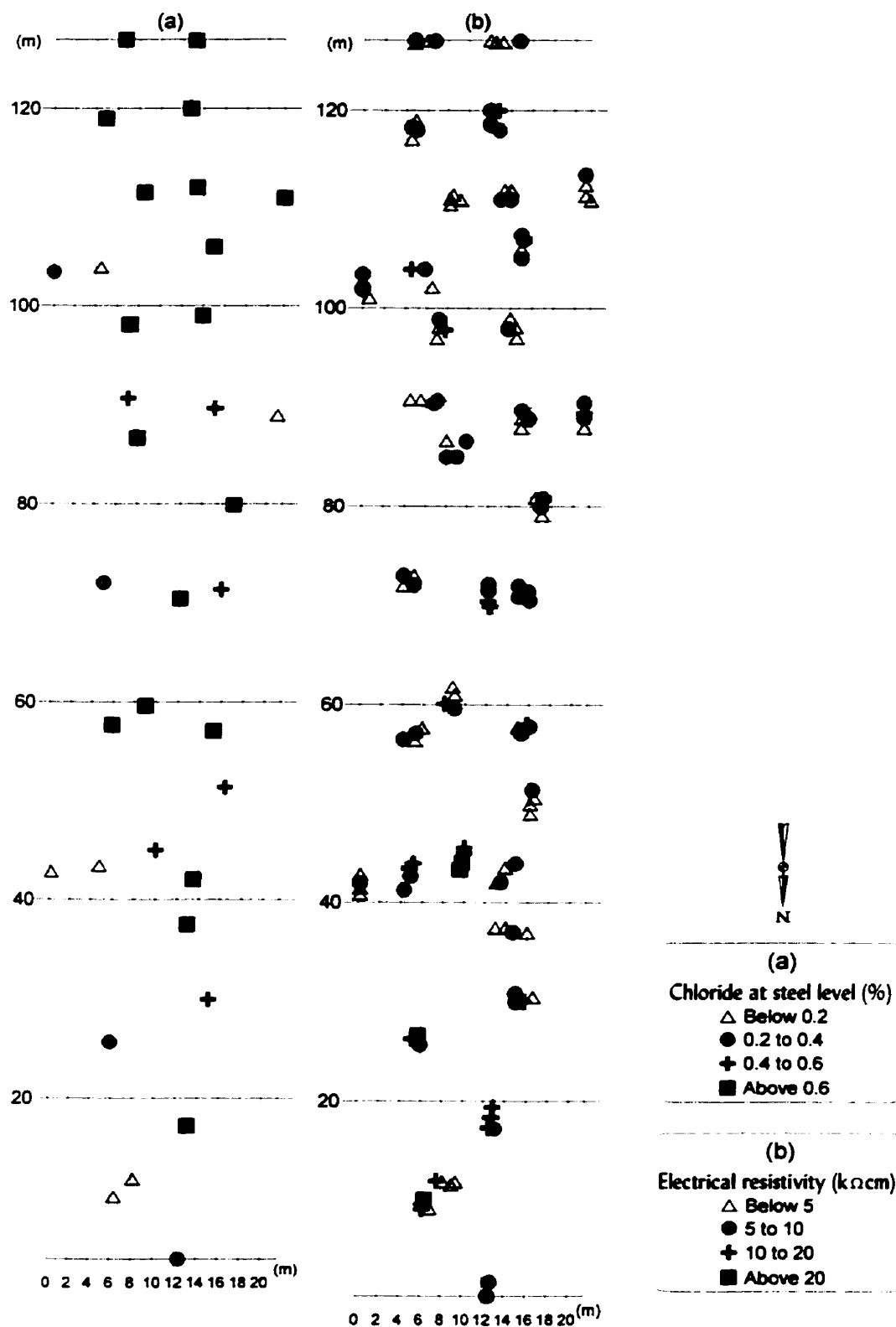
Figure 5-11: Chloride percentage at steel level and resistivity results
