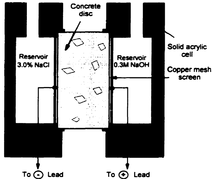
Figure 3-19: Applied voltage cell for core specimens [80, 81]
