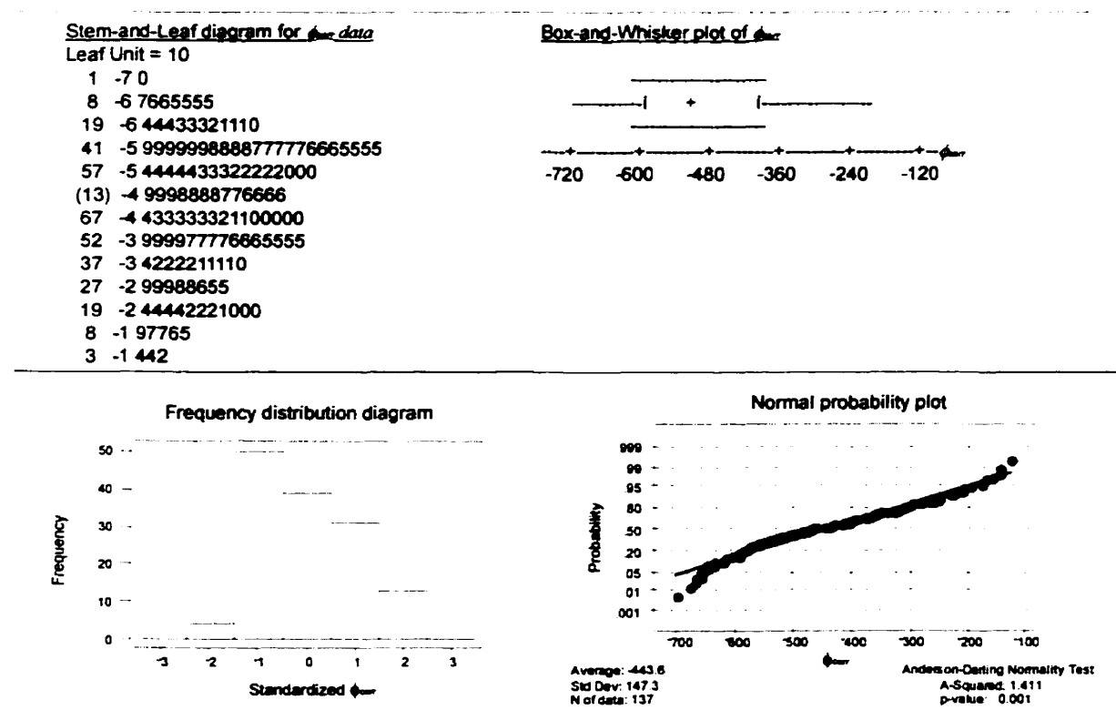
Figure G-1: Analysis 1 for corrosion potential (entire deck)
