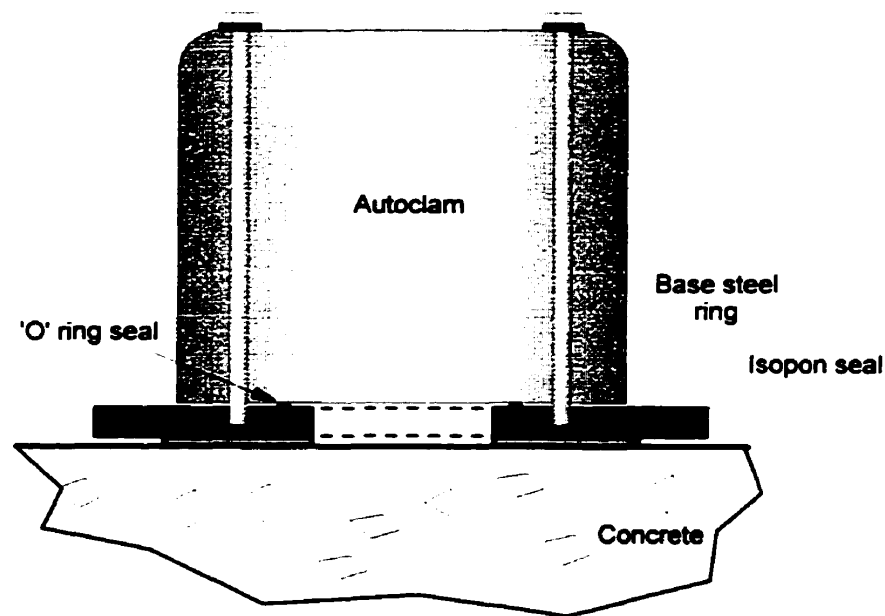
Figure 3-23: Clamping the base plate of the Autoclam to the concrete surface
