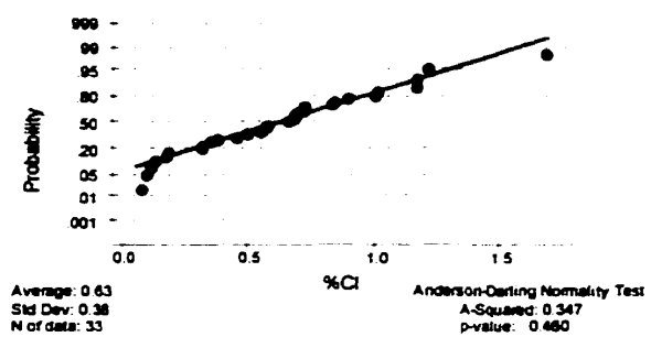
Figure G-8: Analysis 2 for percentage chloride at steel level (entire deck)
