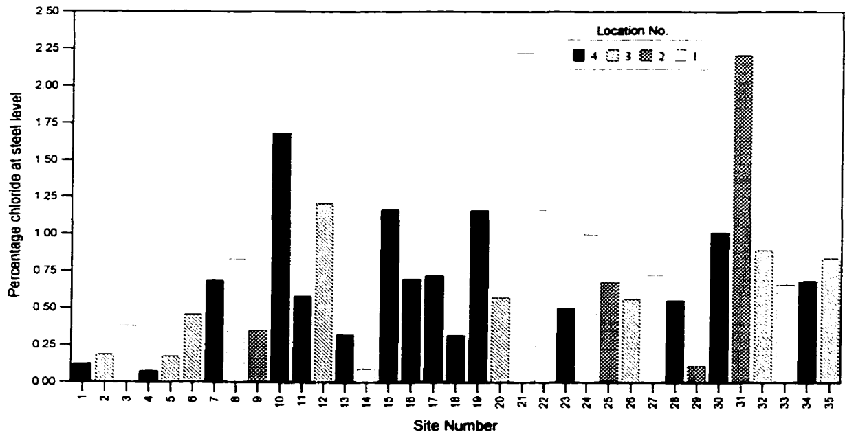
Figure A-7: Percentage chloride at steel level
