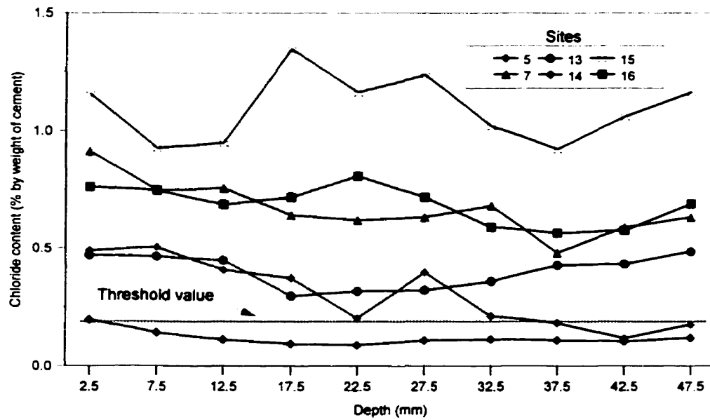
Figure D-5: Chloride profiles (Sites 5, 7 and 13-16)
