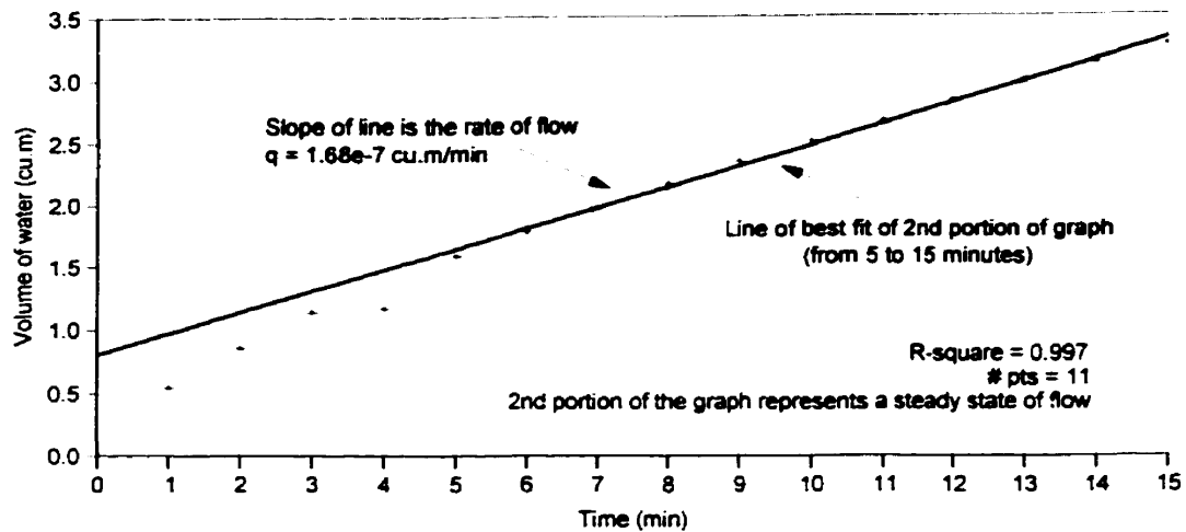
Figure 4-25: Calculation of rate of flow for the steady state (Site 6, location 1)
