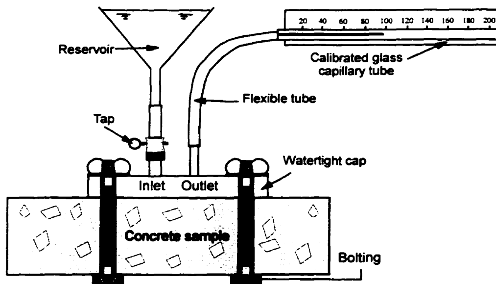
Figure 3-21: Initial Surface Absorption Test (ISAT) [27]
