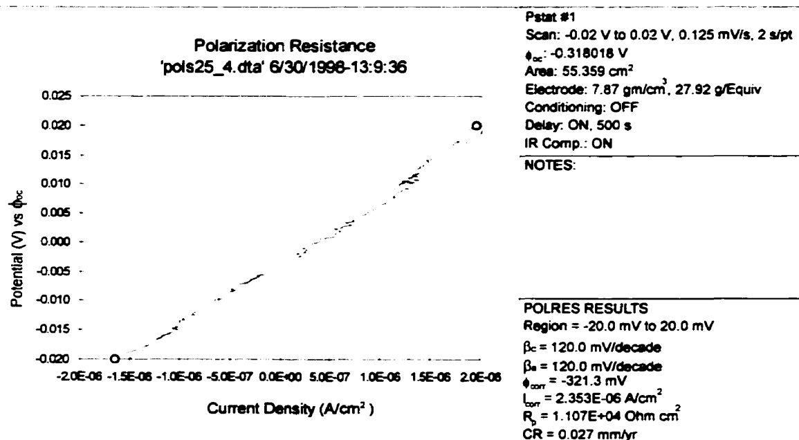
Figure B-8: Polarization resistance plot (Site 25, location 4)
