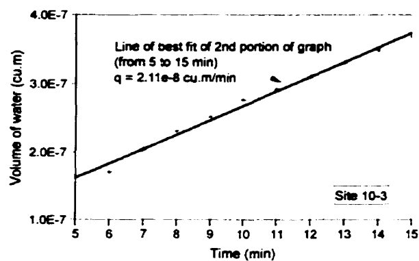
Figure E-2: Steady state slope of volume of water vs. time graphs for Site 10
