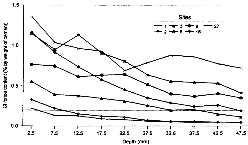
Figure 4-21: Concentration chloride profiles through concrete (Sites 1-3, 6, 9, 18 and 27)
