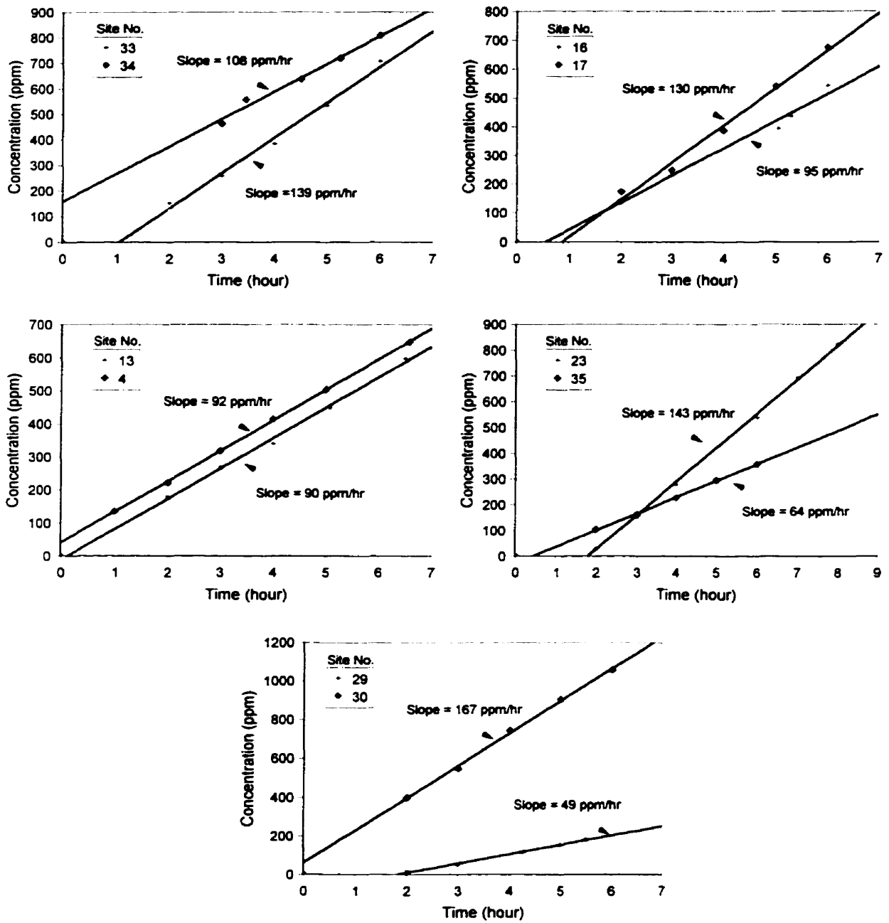
Figure C-3: Steady state slope of concentration vs. time graphs (Sites 4, 13, 16, 17, 23, 29, 30 and 33-35)
