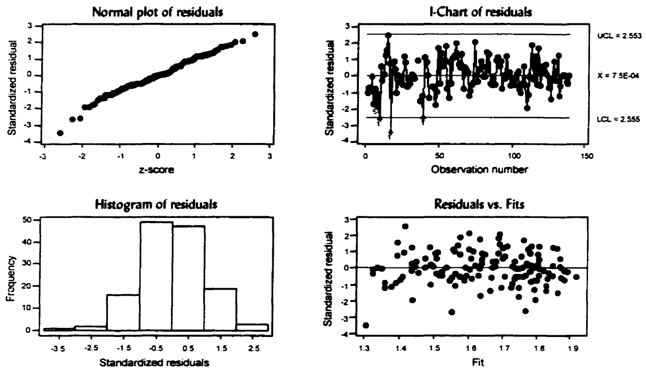
Figure H-1: Standardized residual model diagnostics for ' \phi_{corr} ' (entire deck)
