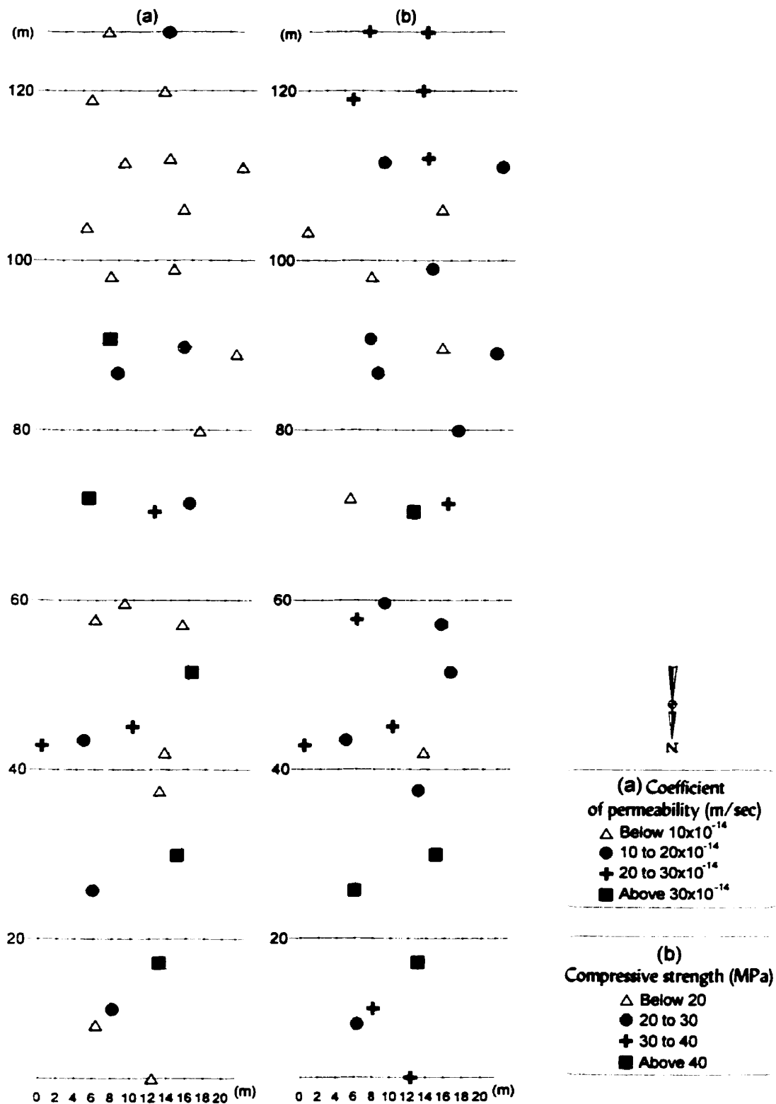
Figure 5-13: Coefficient of permeability and compressive strength results
