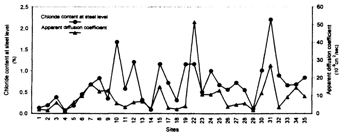
Figure 6-20: Dependence of chloride content at steel level on apparent diffusion coefficient (entire deck)
