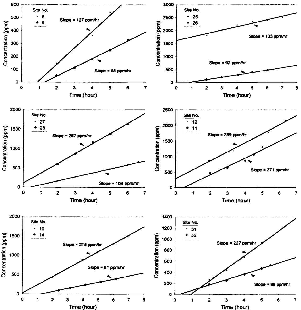
Figure C-2: Steady state slope of concentration vs. time graphs (Sites 8-12, 14, 25-28, 31 and 32)
