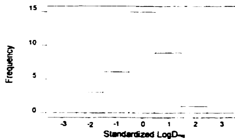
Figure G-14: Analysis 3 for in-situ chloride migration coefficient (entire deck)
