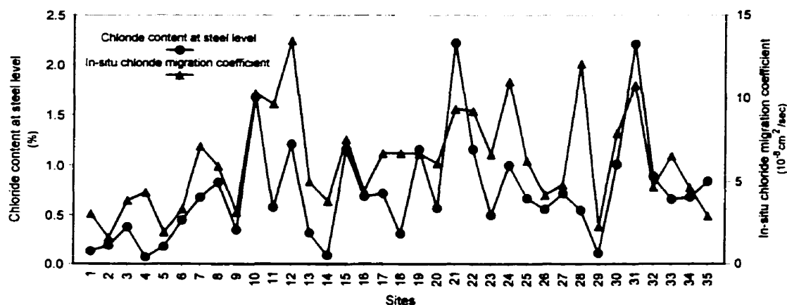
Figure 6-21: Dependence of chloride content at steel level on in-situ migration coefficient (entire deck)
