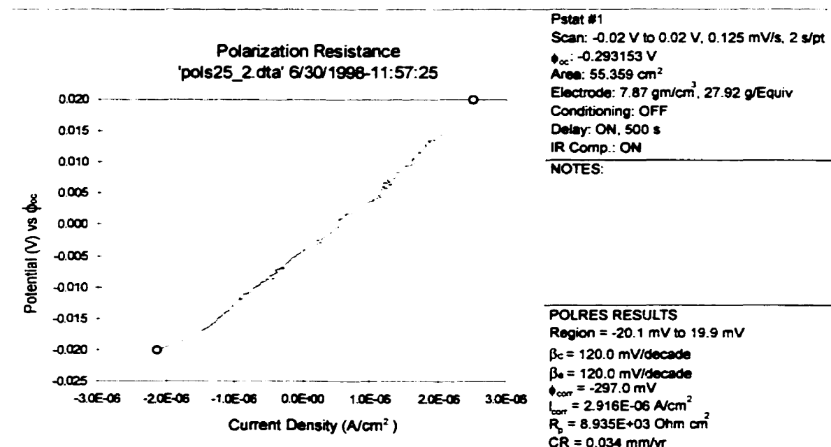
Figure B-6: Polarization resistance plot (Site 25, location 2)
