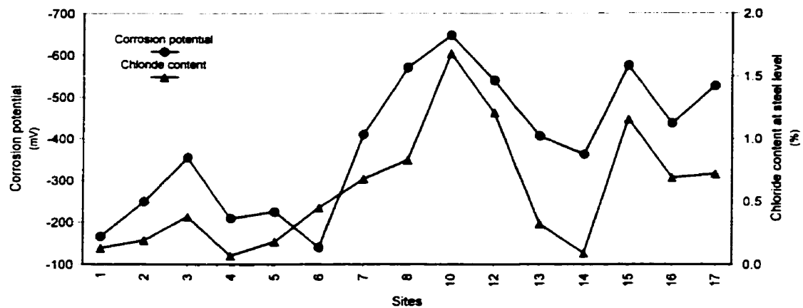
Figure 6-7: Dependence of chloride content at steel level on corrosion potential (east side of deck)
