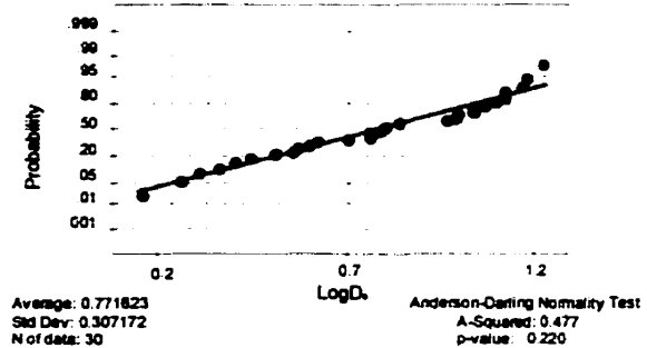
Figure G-11: Analysis 3 for apparent chloride diffusion coefficient (entire deck)
