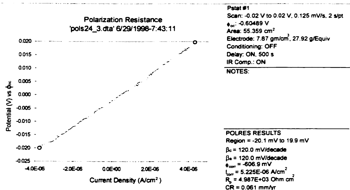
Figure B-3: Polarization resistance plot (Site 24, location 3)
