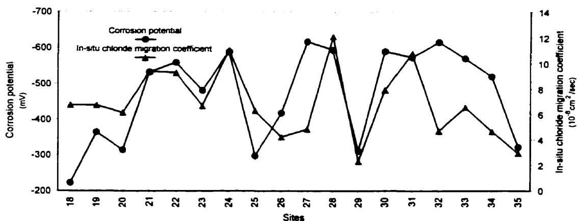
Figure 6-4: Dependence of in-situ chloride migration coefficient on corrosion potential (west side of deck)
