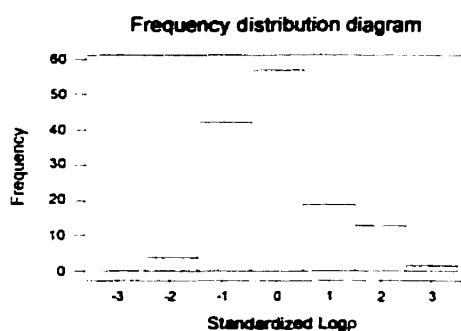
Figure G-17: Analysis 3 for resistivity of concrete (entire deck)
