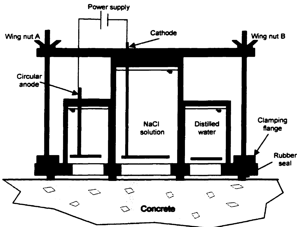
Figure 3-20: In-situ chloride migration test [86]
