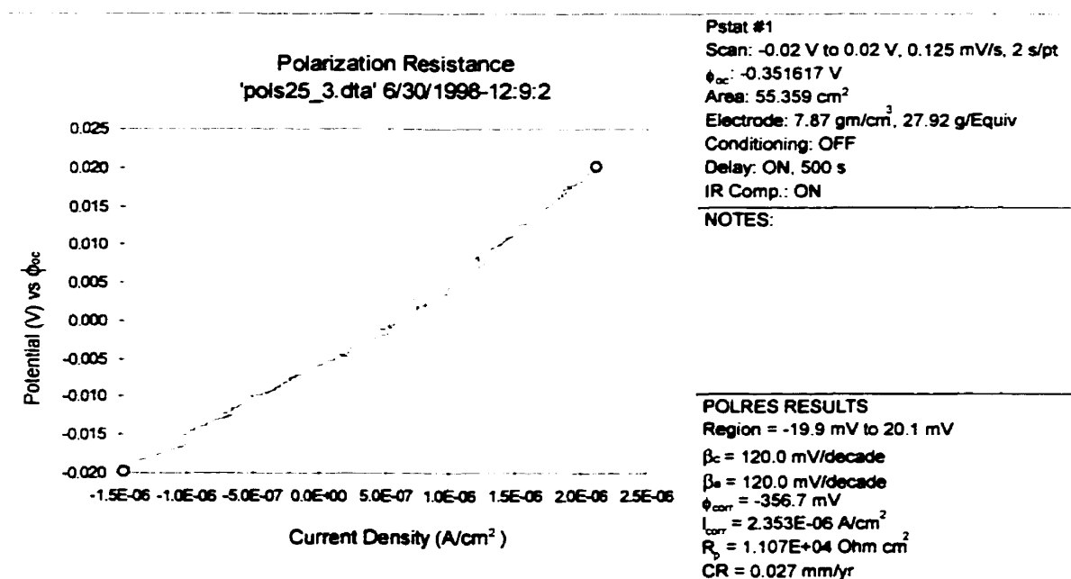
Figure B-7: Polarization resistance plot (Site 25, location 3)
