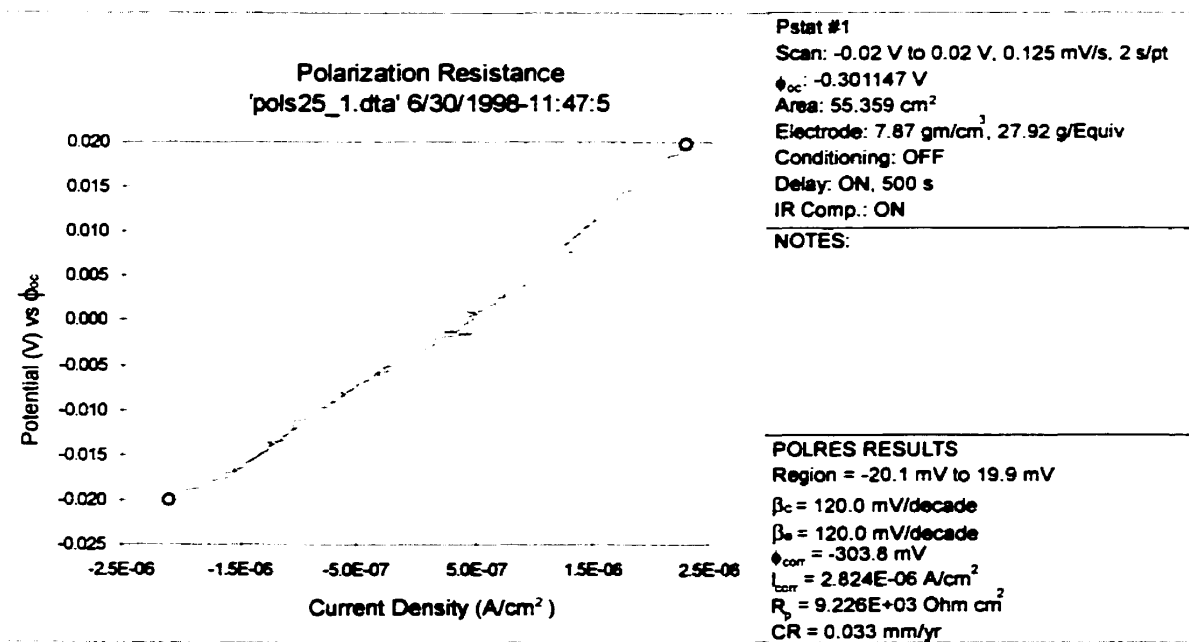
Figure B-5: Polarization resistance plot (Site 25, location 1)
