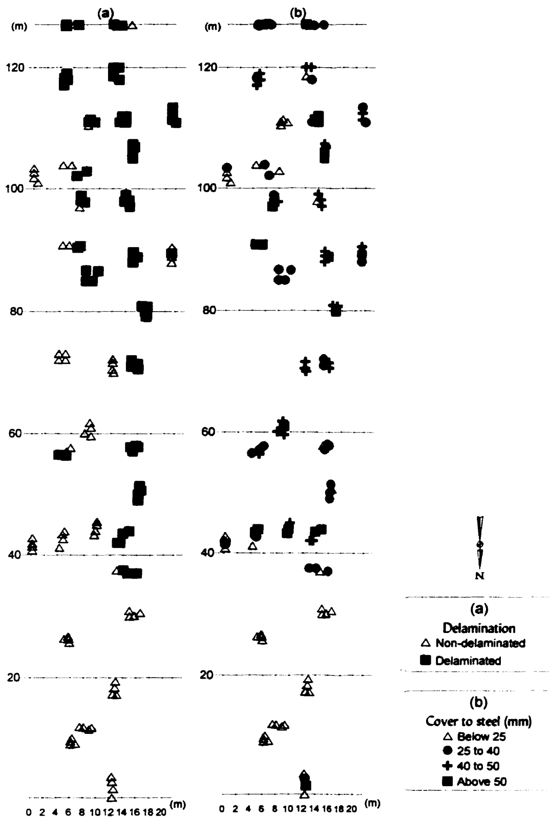
Figure 5-10: Results of delamination and concrete cover surveys
