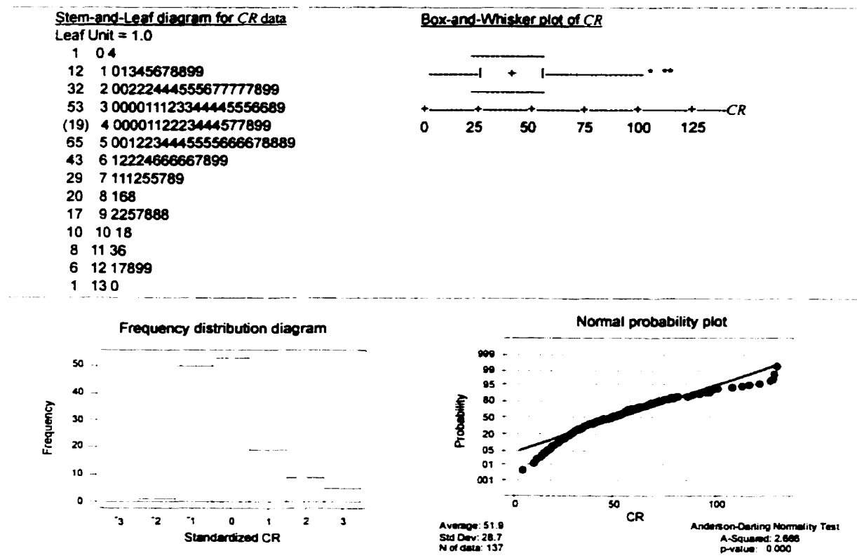
Figure G-2: Analysis 1 for corrosion rate (entire deck)
