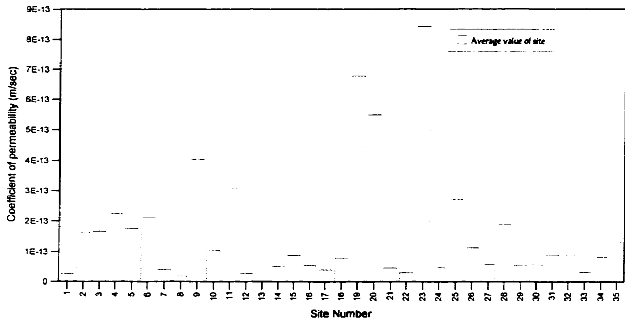
Figure A-10: Coefficient of permeability values
