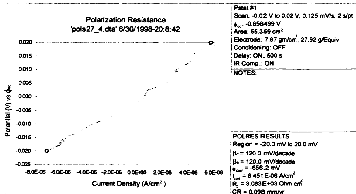
Figure B-12: Polarization resistance plot (Site 27, location 4)
