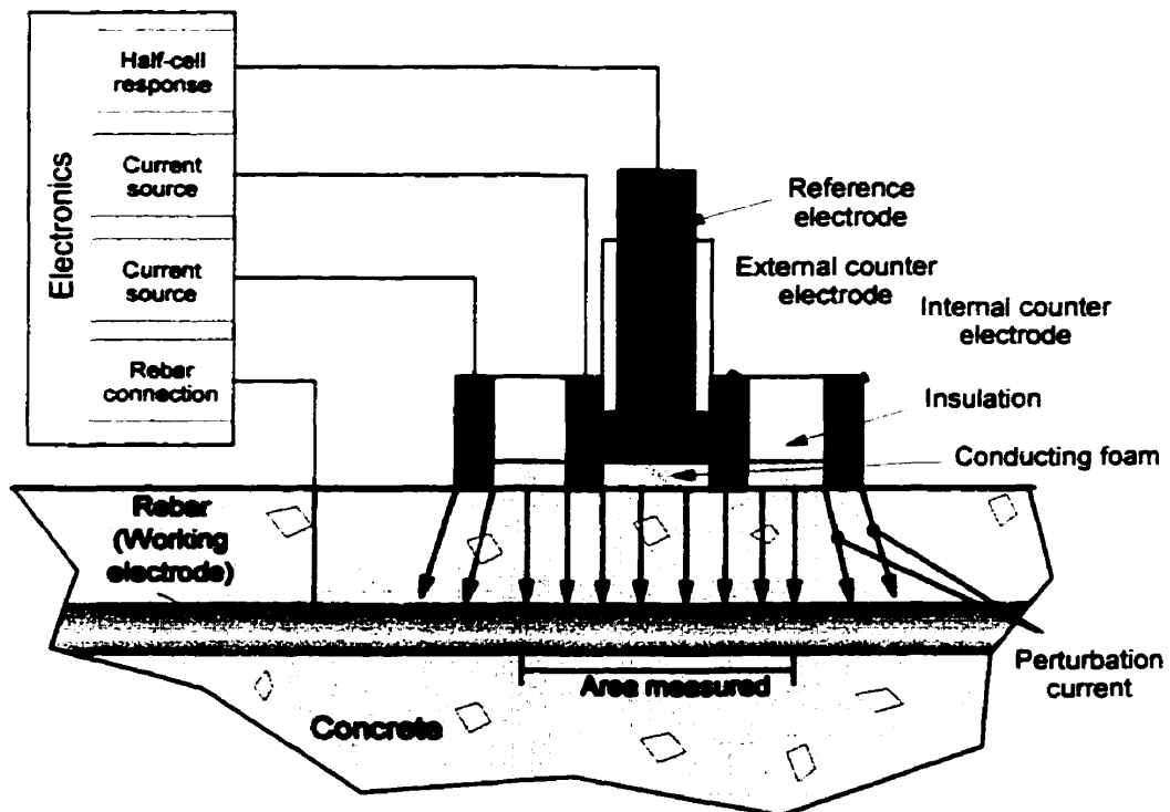
Figure 3-15: Schematic of linear polarization device with controlled guard ring [33, 68]
