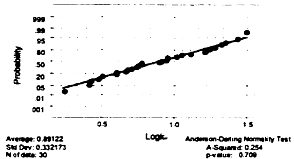
Figure G-20: Analysis 3 for coefficient of permeability (entire deck)
