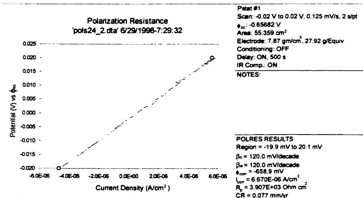
Figure B-2: Polarization resistance plot (Site 24, location 2)
