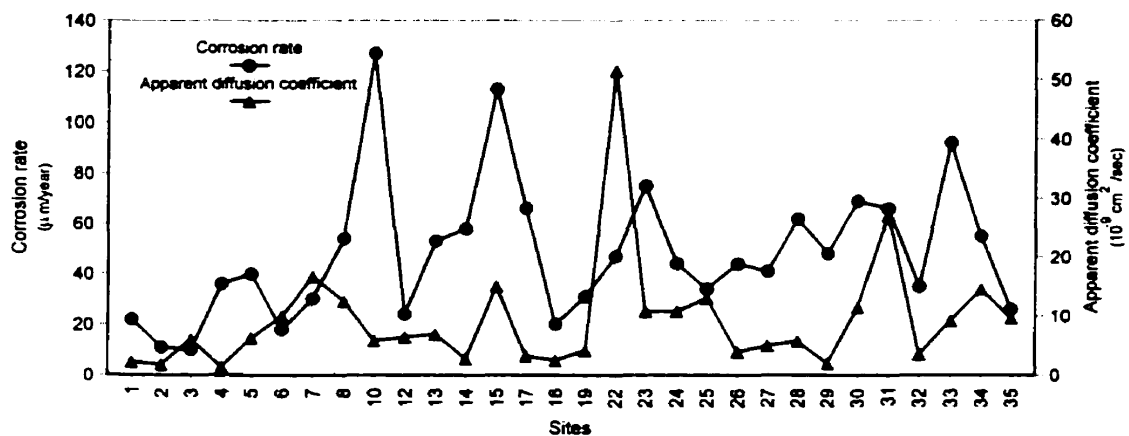
Figure 6-18: Dependence of apparent diffusion coefficient on corrosion rate (entire deck)
