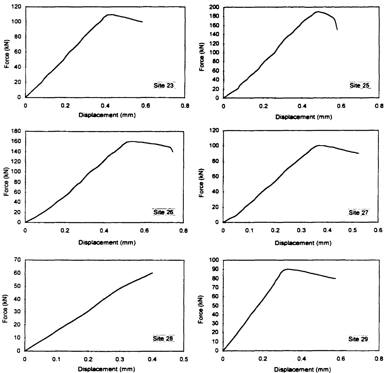
Figure F-4: Force versus displacement plot (Sites 23-29)
