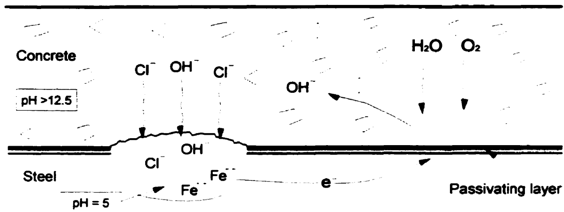
Figure 2-8: Schematic representation of pitting corrosion (in the presence of chlorides) [23]
