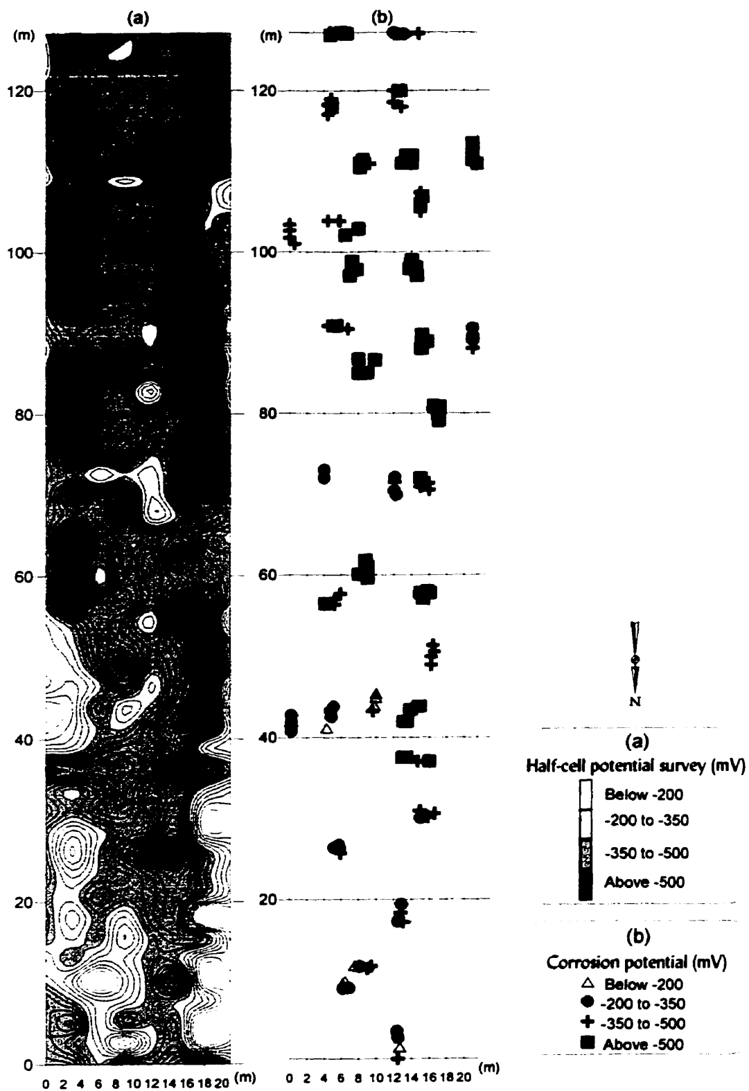
Figure 5-8: Half-cell potential and corrosion potential results
