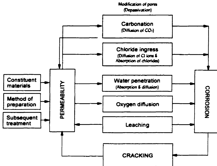
Figure 2-5: Corrosion-permeability interaction model [12, 14, 49]
