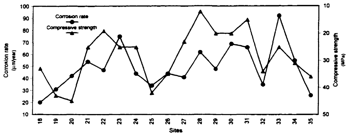
Figure 6-16: Dependence of concrete compressive strength on corrosion rate (west side of deck)
