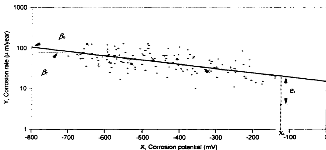
Figure 6-25: Y vs. X plot (Corrosion rate vs. corrosion potential)
