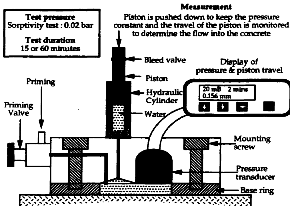
(a) Method of operation for sorptivity test
