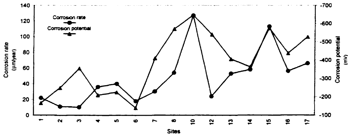
Figure 6-1: Dependence of potential on corrosion rate (east side of deck)
