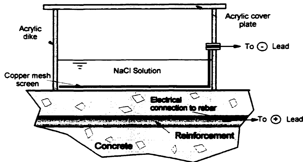
Figure 3-18: Applied voltage apparatus used on slab specimens [80, 81]
