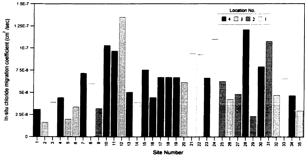
Figure A-6: In-situ chloride migration coefficient values
