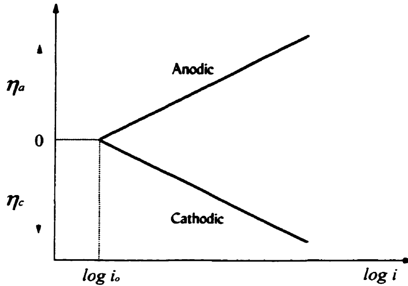
Figure 3-3: Polarization curves [53]
