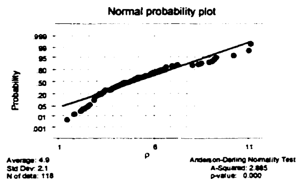
Figure G-16: Analysis 2 for resistivity of concrete (entire deck)
