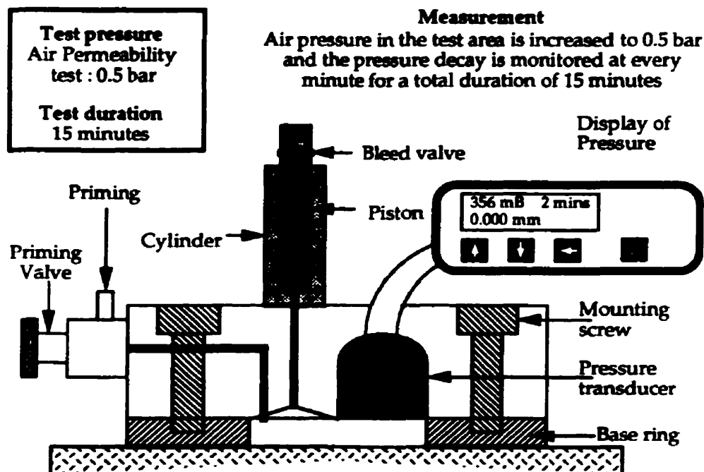
(b) Method of operation for air permeability test
