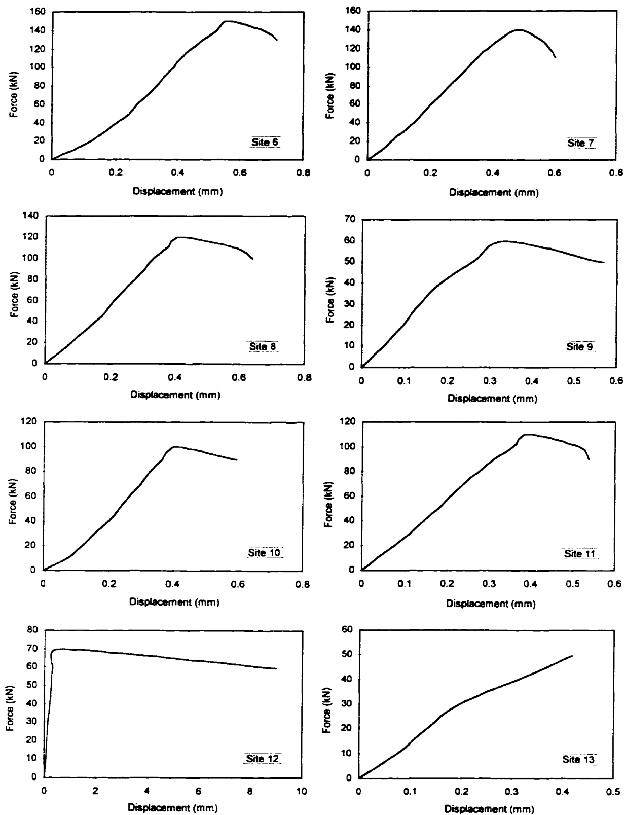
Figure F-2: Force versus displacement plot (Sites 6-13)
