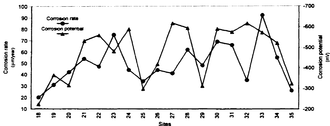
Figure 6-2: Dependence of potential on corrosion rate (west side of deck)
