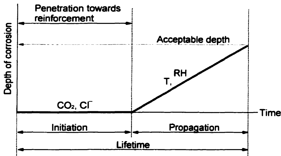
Figure 2-1: Schematic sketch of steel corrosion sequence in concrete [22]
