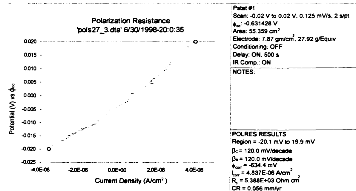
Figure B-11: Polarization resistance plot (Site 27, location 3)
