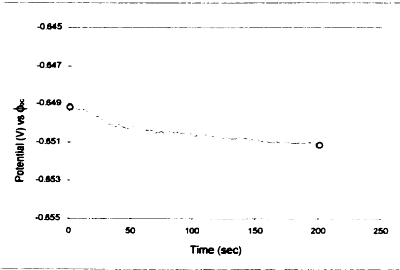
Figure 4-10: Stabilizing of open circuit potential (Site 10, location 1)
