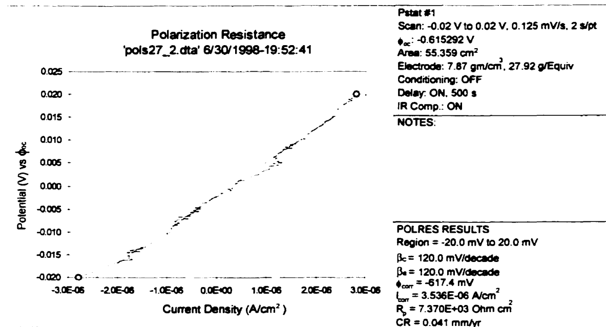
Figure B-10: Polarization resistance plot (Site 27, location 2)
