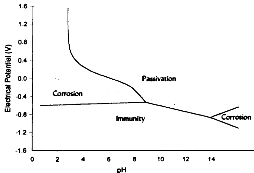
Figure 2-4: Simplified Pourbaix diagram for iron [25]
