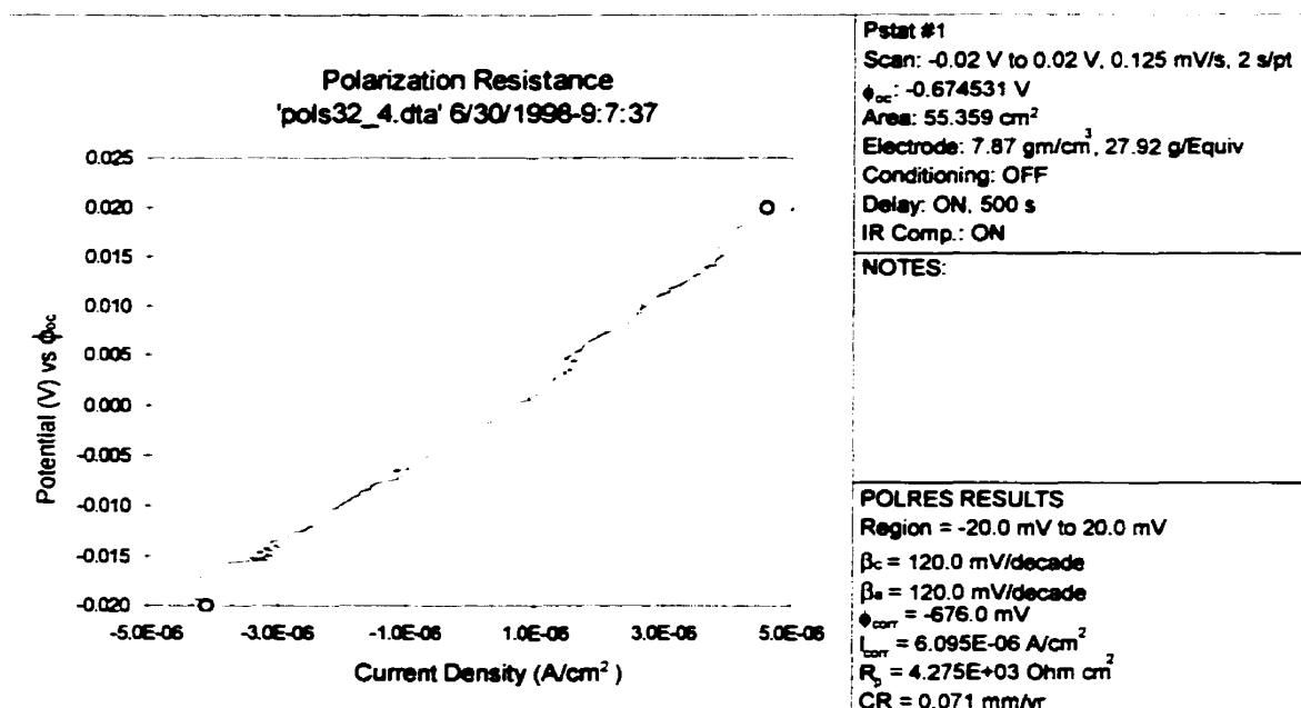
Figure B-16: Polarization resistance plot (Site 32, location 4)
