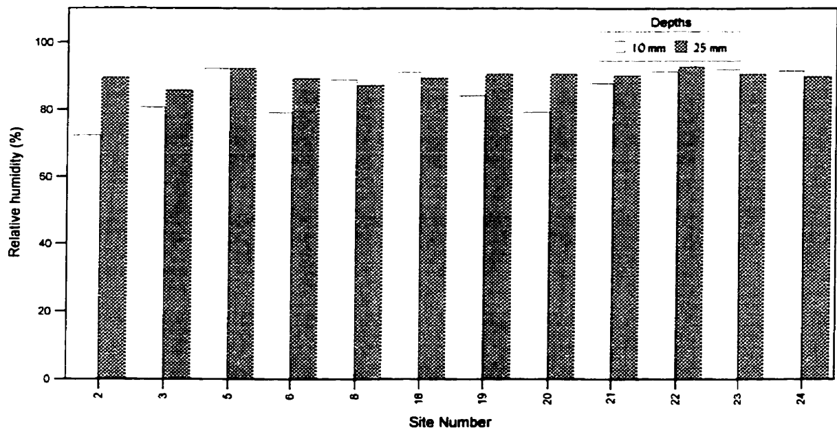
Figure A-9: Relative humidity readings
