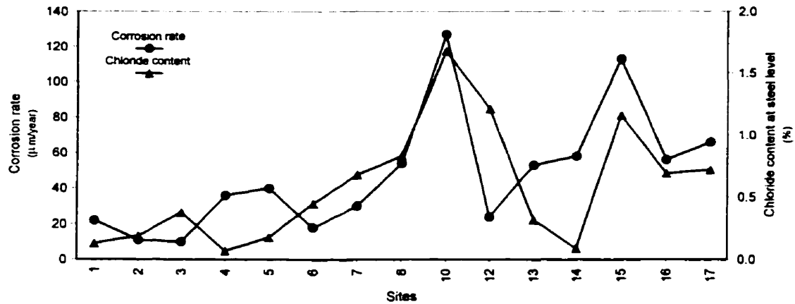
Figure 6-9: Dependence of chloride content at steel level on corrosion rate (east side of deck)
