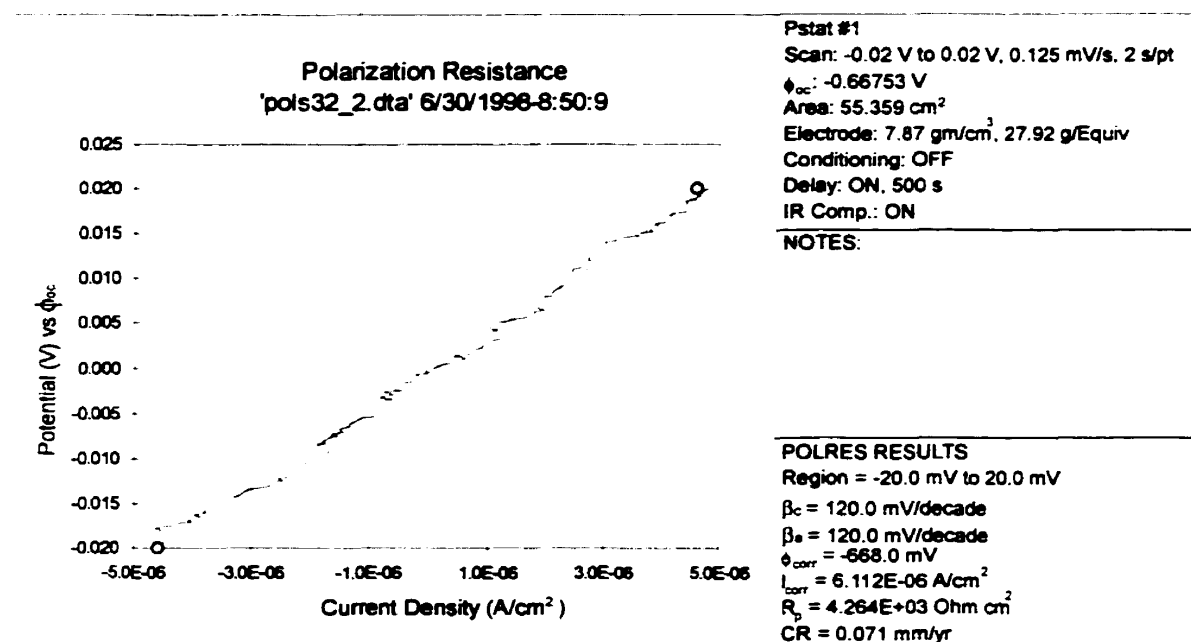
Figure B-14: Polarization resistance plot (Site 32, location 2)
