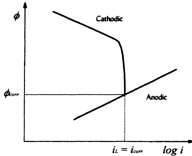
Figure 3-4: Concentration potential curve [56]
