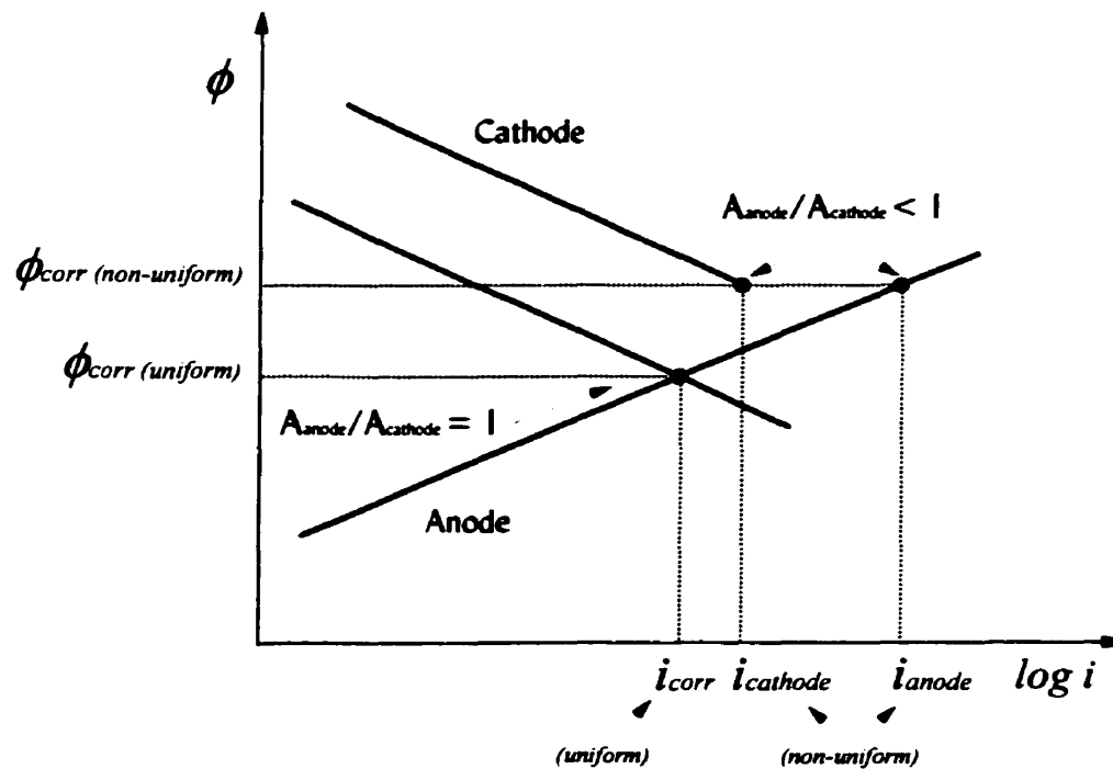
Figure 3-9: Effects of anode/cathode surface area ratio on corrosion reaction [55, 56]
