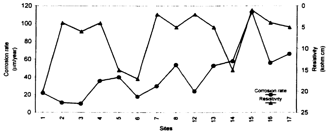
Figure 6-13: Dependence of resistivity of concrete on corrosion rate (east side of deck)
