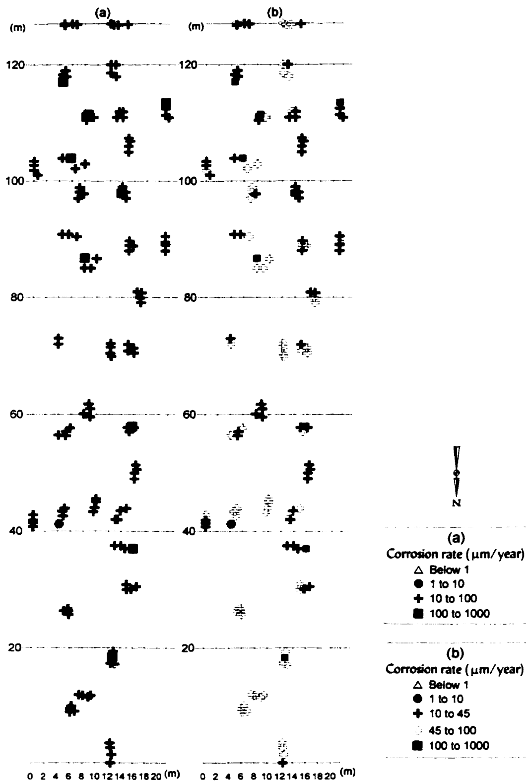
Figure 5-9: Corrosion rate results
