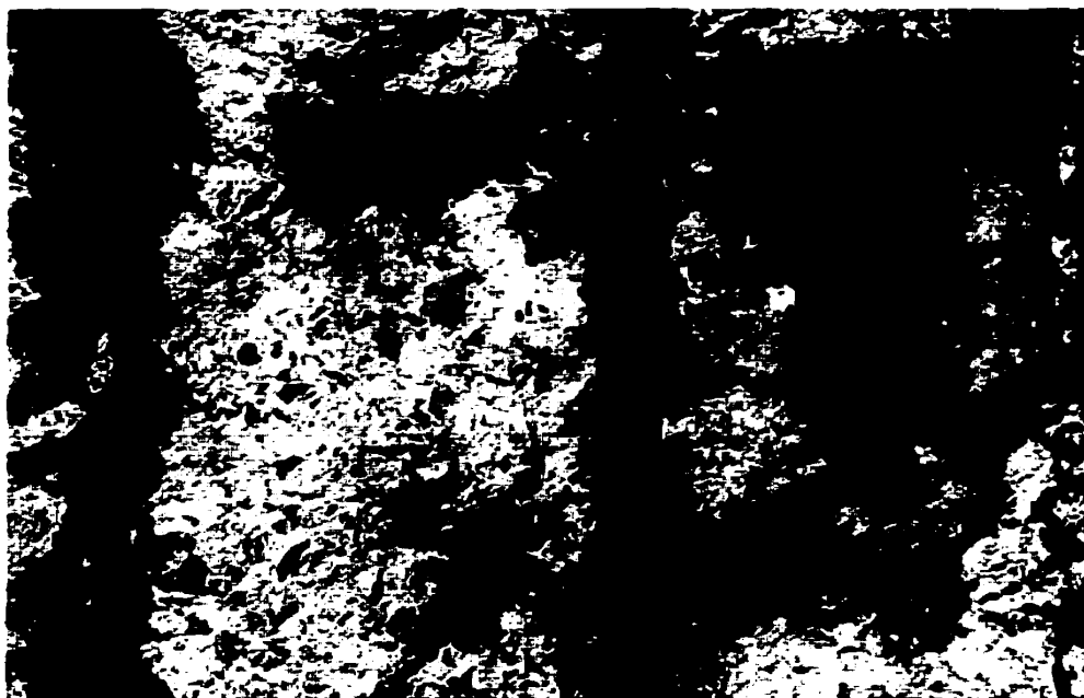
Figure 5-2: Corrosion of reinforcing steel and spalling of concrete cover (Site 11)
