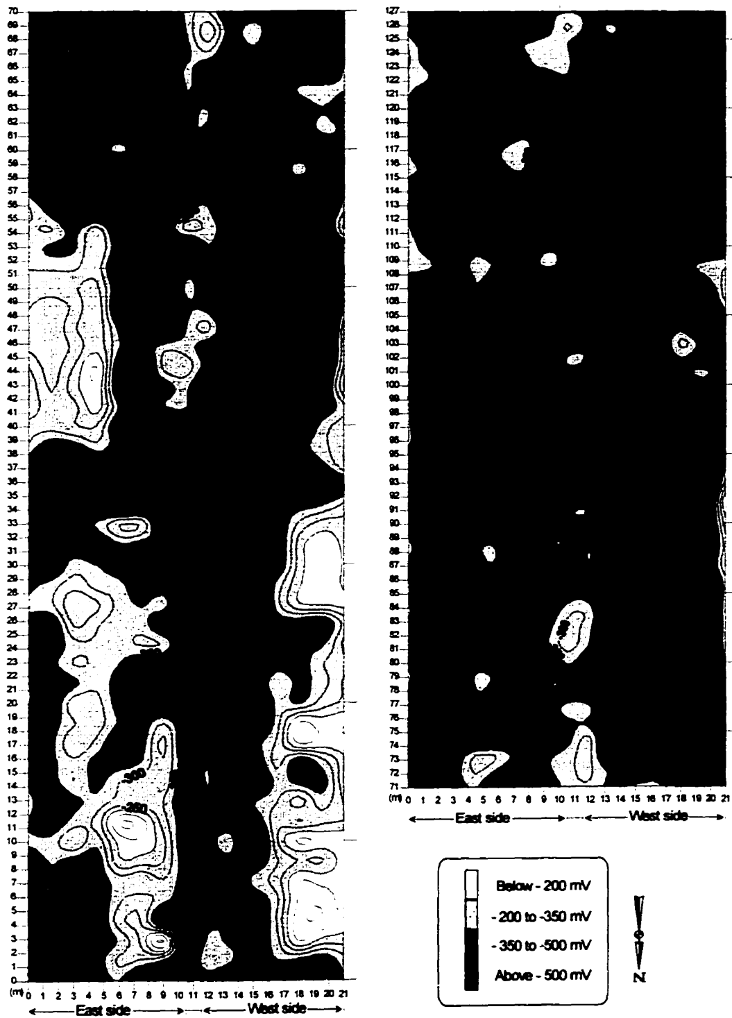
Figure 4-5: Half-cell potential survey of the northern portion of the bridge deck
