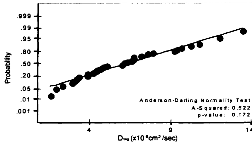
Figure 6-24: Normal probability plot for D_{mig} values (Analysis 1)
