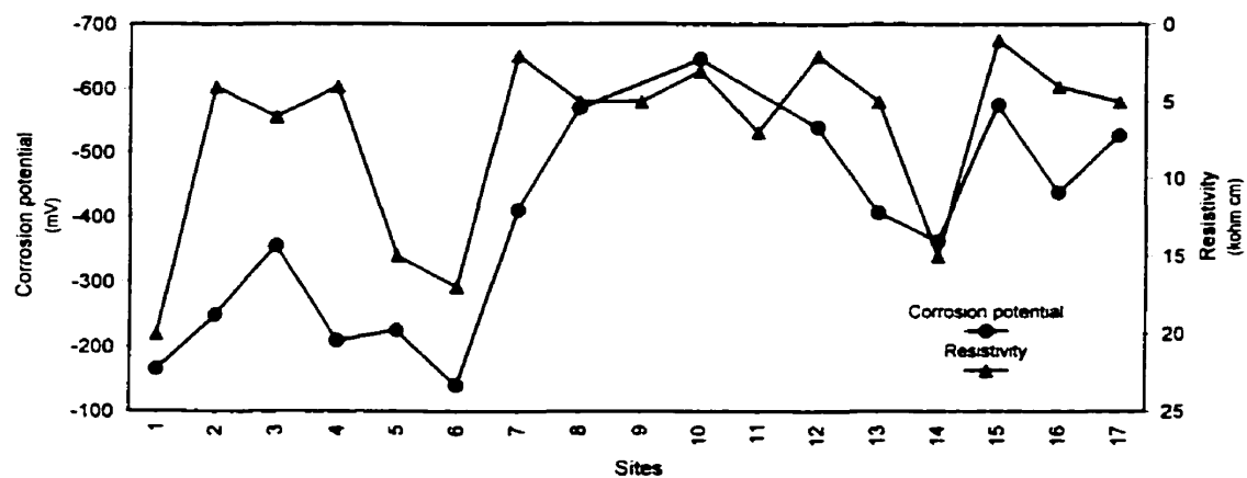
Figure 6-11: Dependence of resistivity of concrete on corrosion potential (east side of deck)
