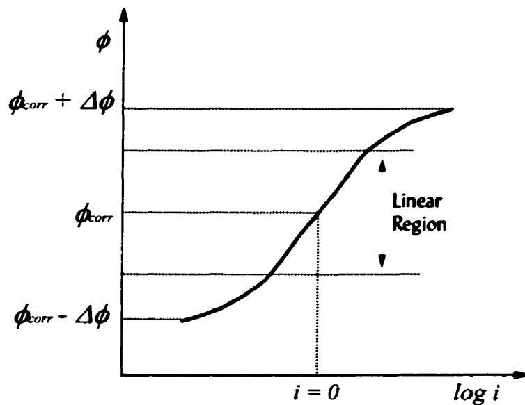
Figure 3-12: Linear polarization curve [66]
