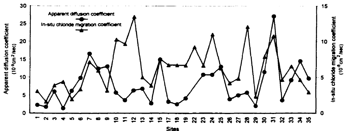
Figure 6-19: Dependence of in-situ migration coefficient on apparent diffusion coefficient (entire deck)
