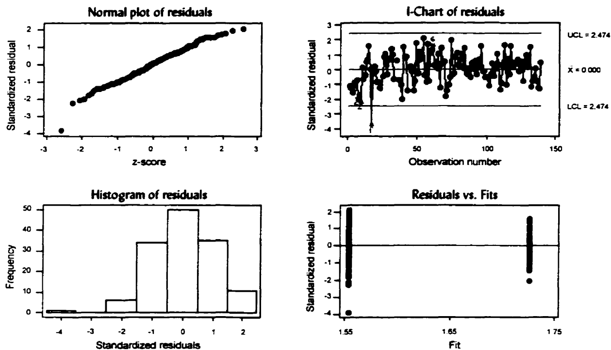
Figure H-2: Standardized residual model diagnostics for 'Delam' (entire deck)
