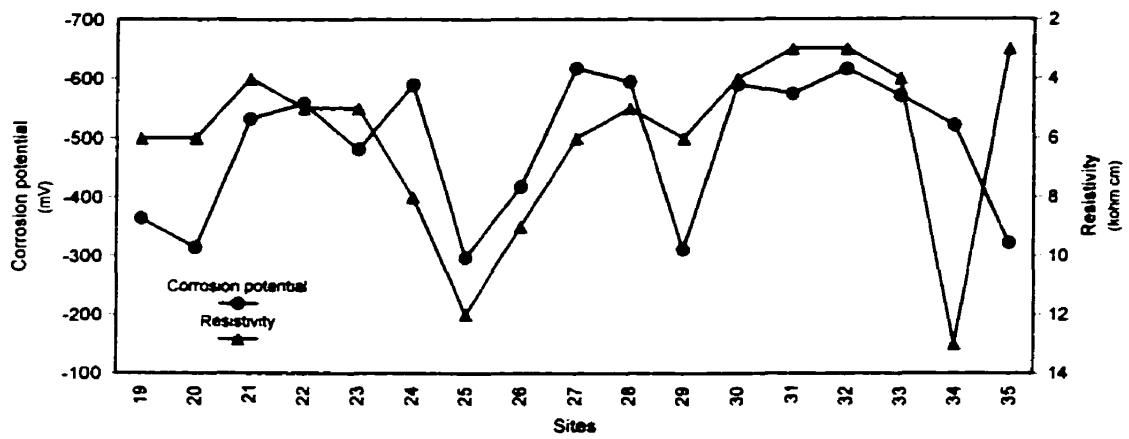
Figure 6-12: Dependence of resistivity of concrete on corrosion potential (west side of deck)
