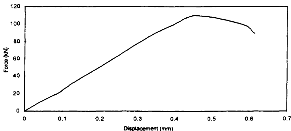
Figure 4-26: Force versus displacement plot (Site 24)
