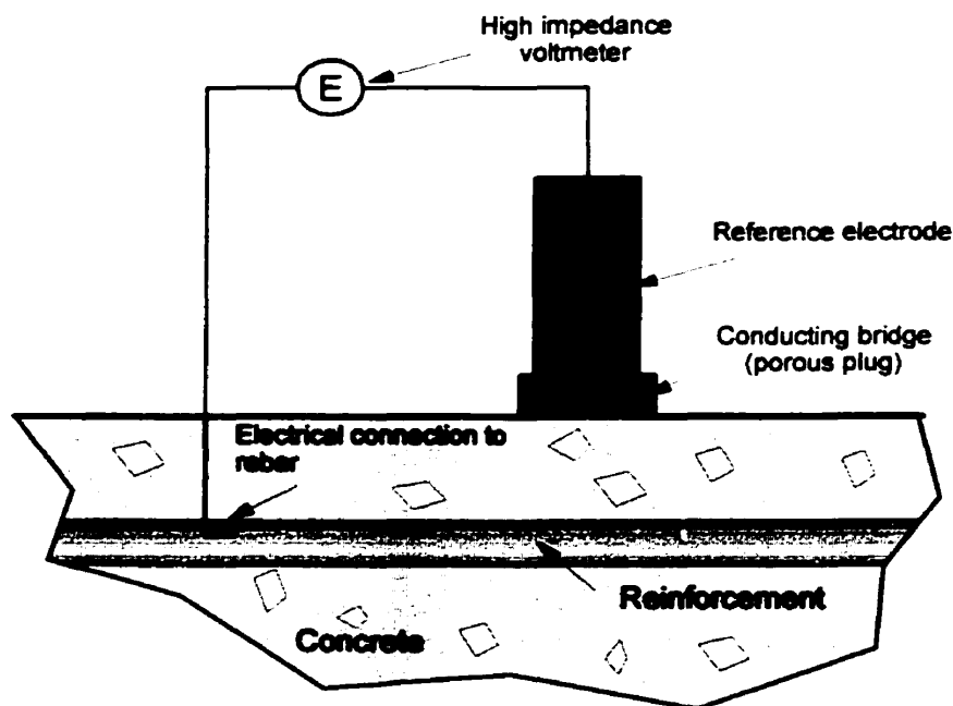
Figure 3-11: Electrical circuit for measuring half-cell potentials [62, 63]
