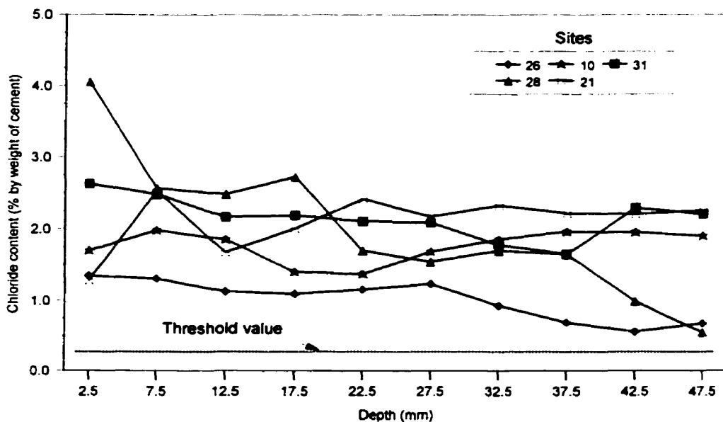
Figure D-3: Chloride profiles (Sites 10, 21, 26, 28 and 31)
