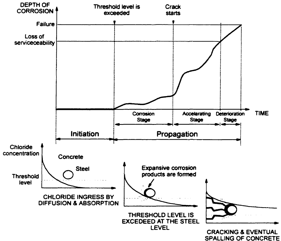
Figure 2-6: Corrosion stages [54]
