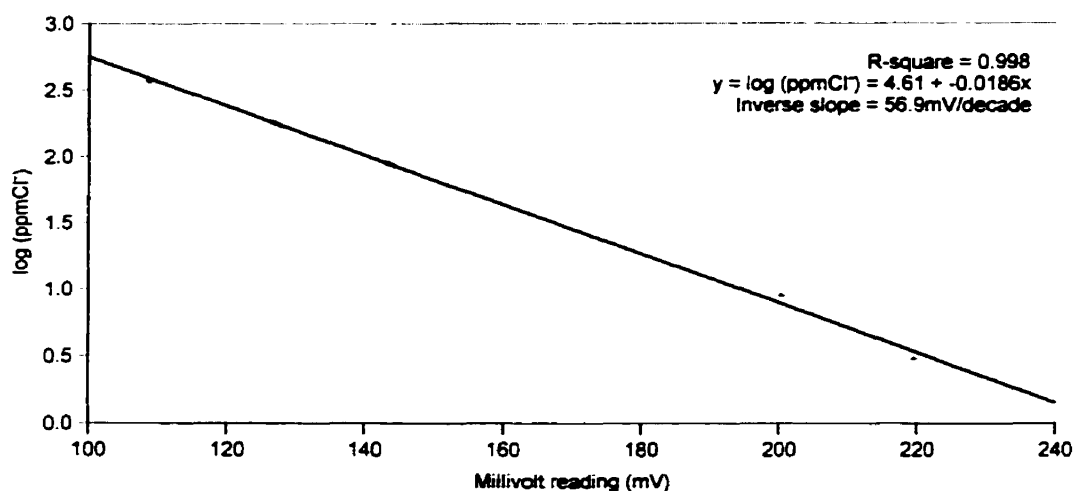
Figure 4-19: Typical calibration curve
