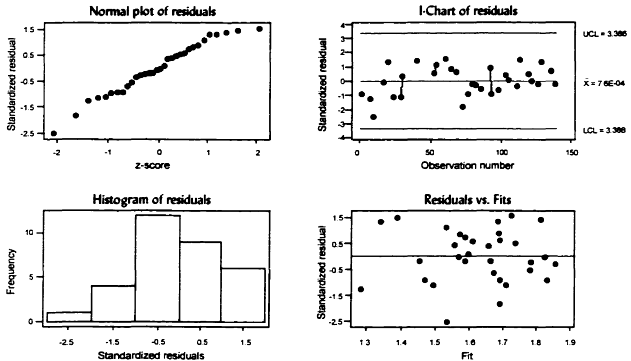
Figure 6-26: Standardized residual model diagnostics for 'LogD mig ' (entire bridge deck)
