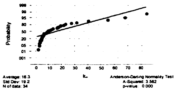
Figure G-18: Analysis 1 for coefficient of permeability (entire deck)
