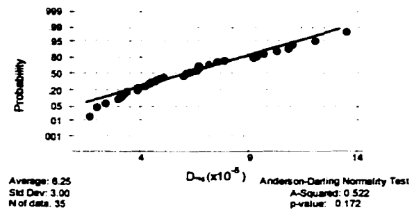
Figure G-12: Analysis 1 for in-situ chloride migration coefficient (entire deck)
