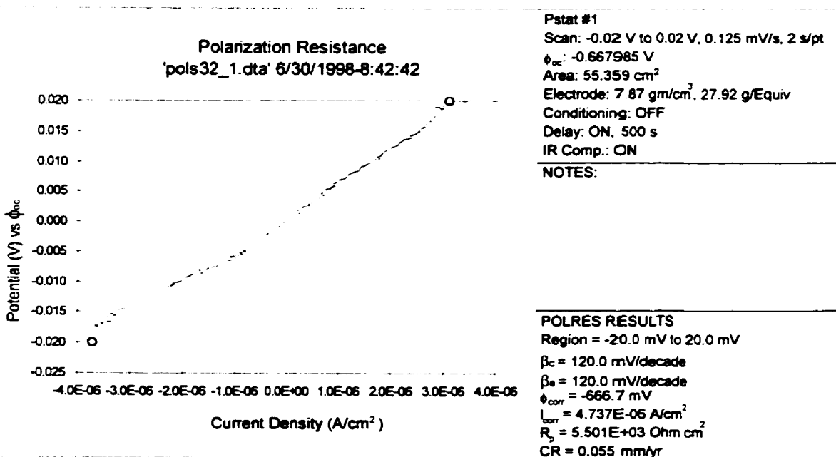
Figure B-13: Polarization resistance plot (Site 32, location 1)
