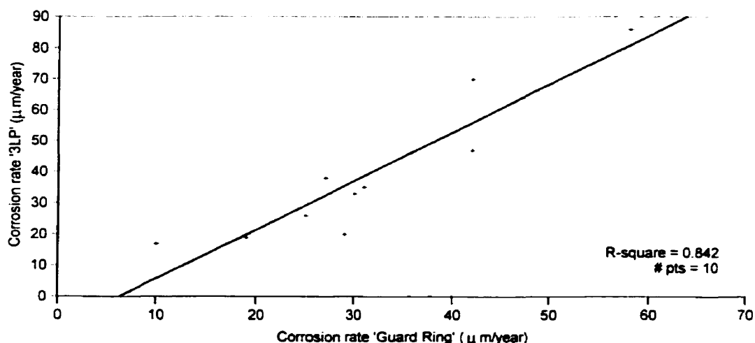
Figure 4-12: Comparison of corrosion rate values obtained with different probes
