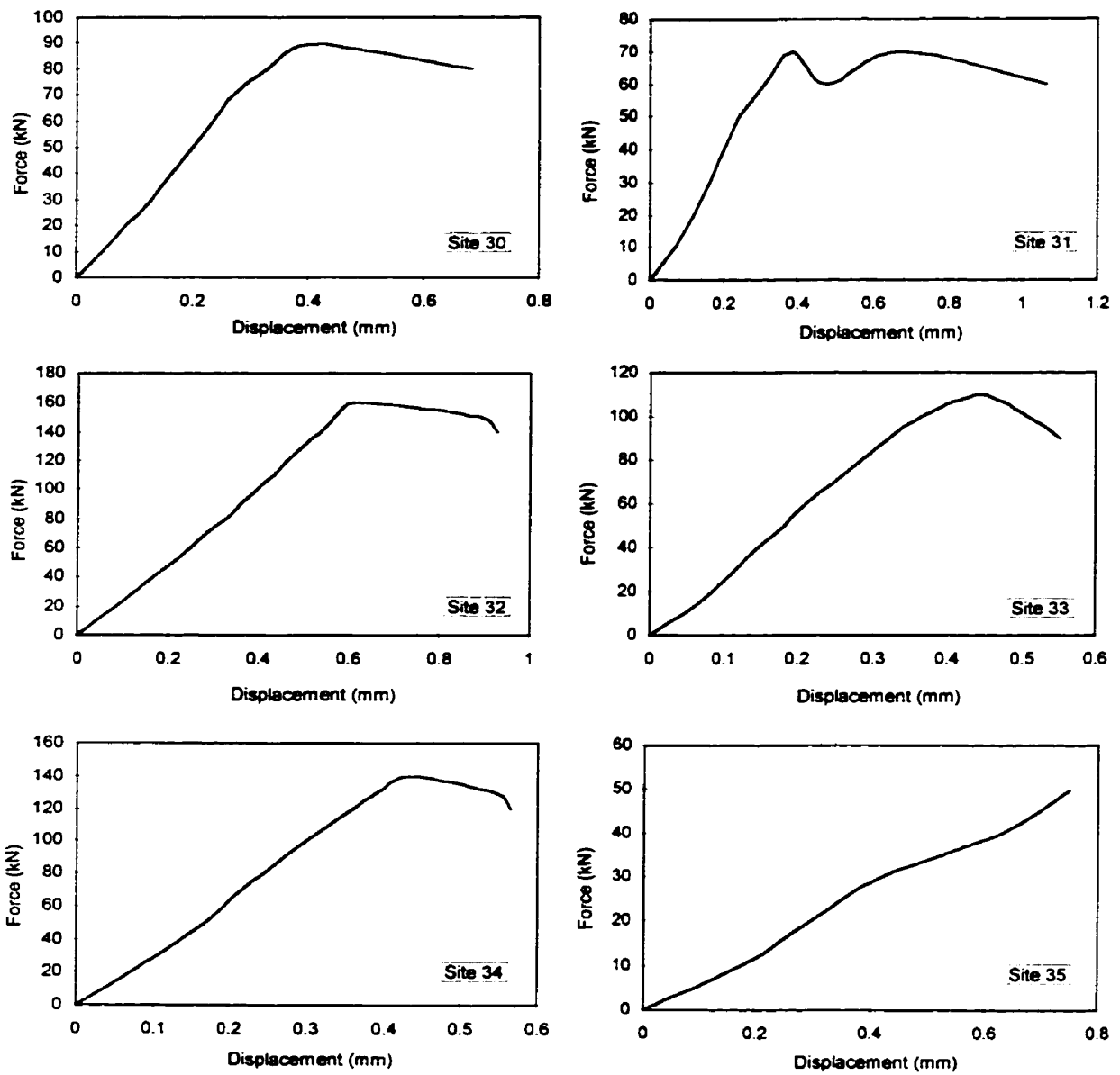
Figure F-5: Force versus displacement plot (Sites 30-35)
