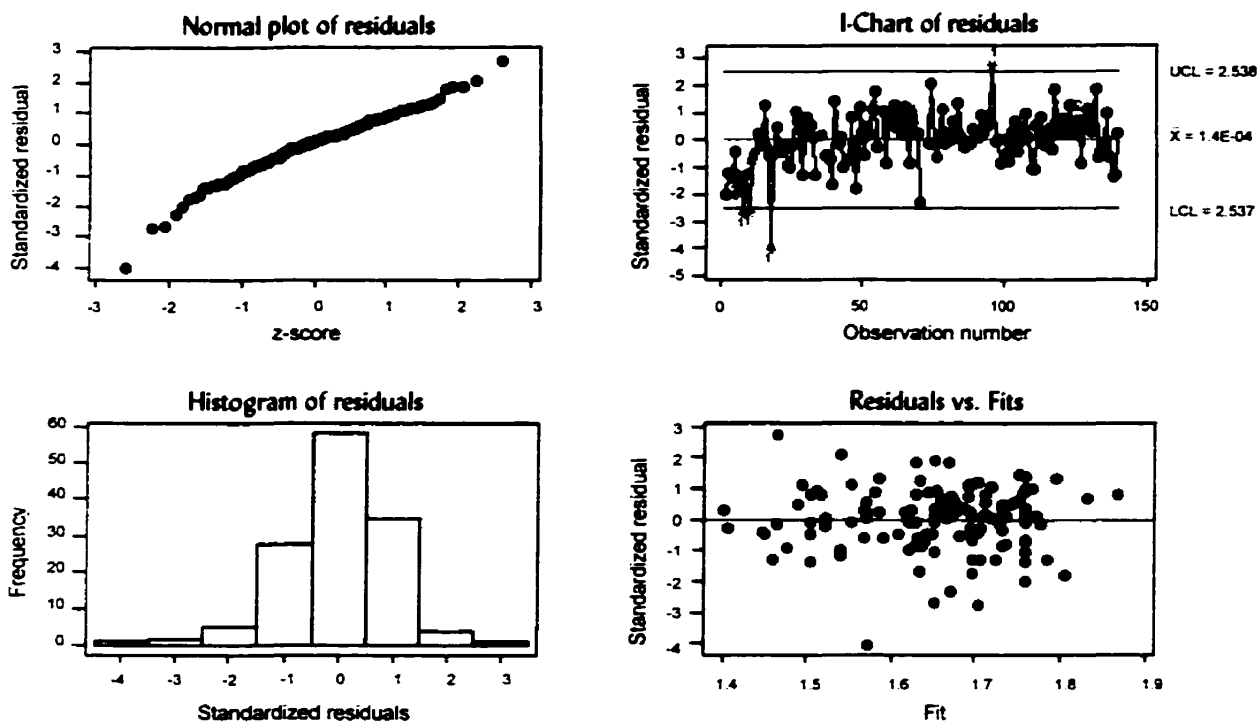
Figure H-6: Standardized residual model diagnostics for 'Logp'(entire deck)
