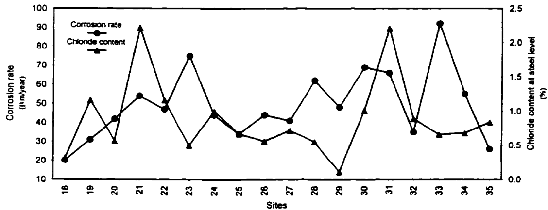
Figure 6-10: Dependence of chloride content at steel level on corrosion rate (west side of deck)
