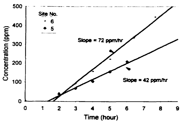
Figure C-1: Steady state slope of concentration vs. time graphs (Sites 1-3, 5-7, 18-22 and 24)
