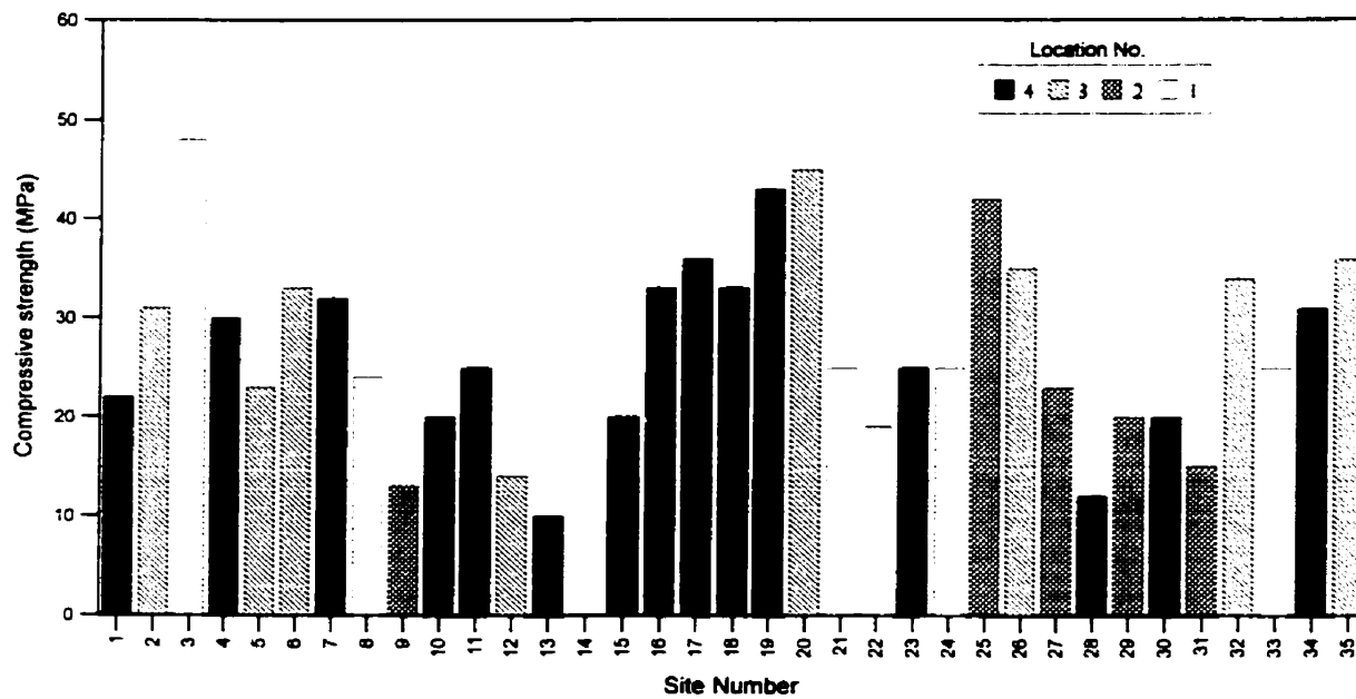
Figure A-12: Concrete compressive strength values
