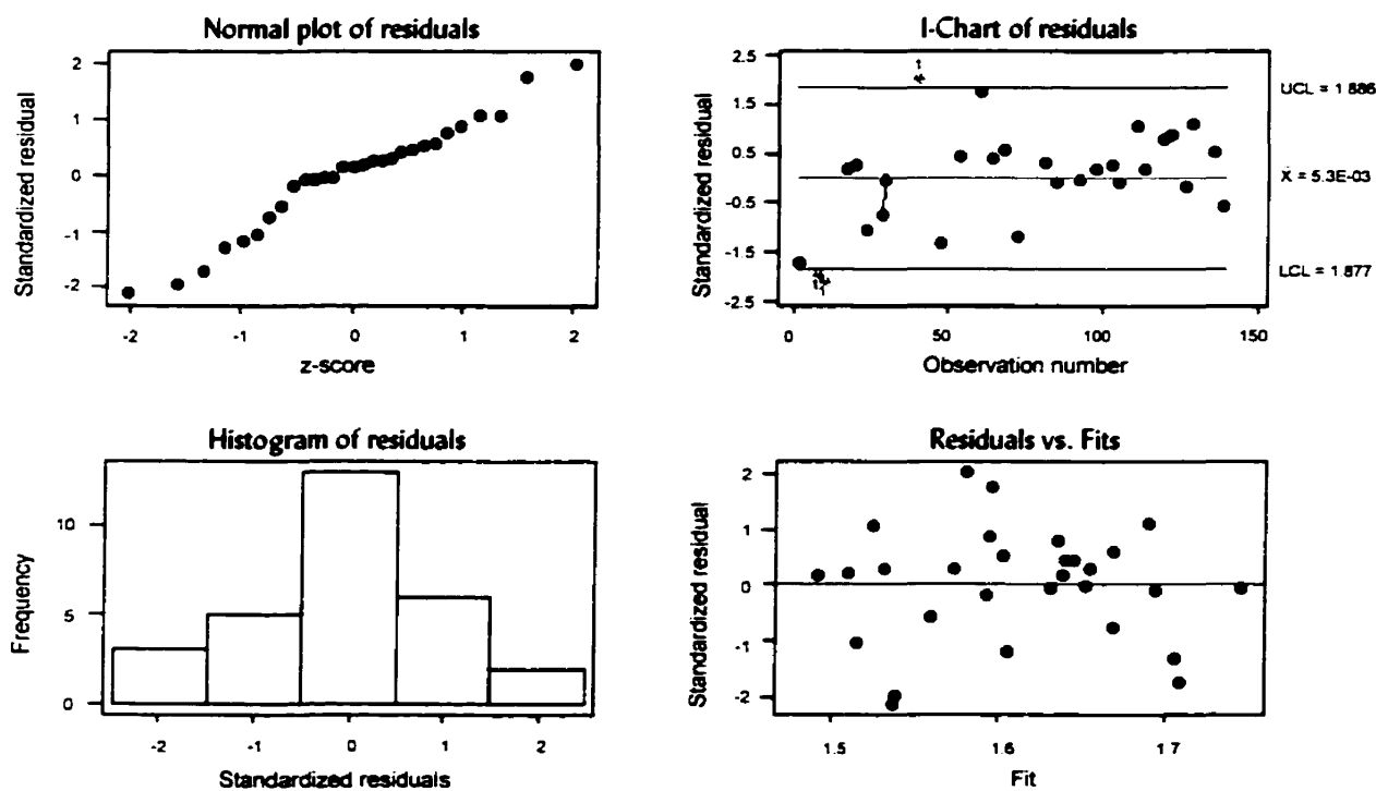
Figure H-7: Standardized residual model diagnostics for 'Logk w '(entire deck)
