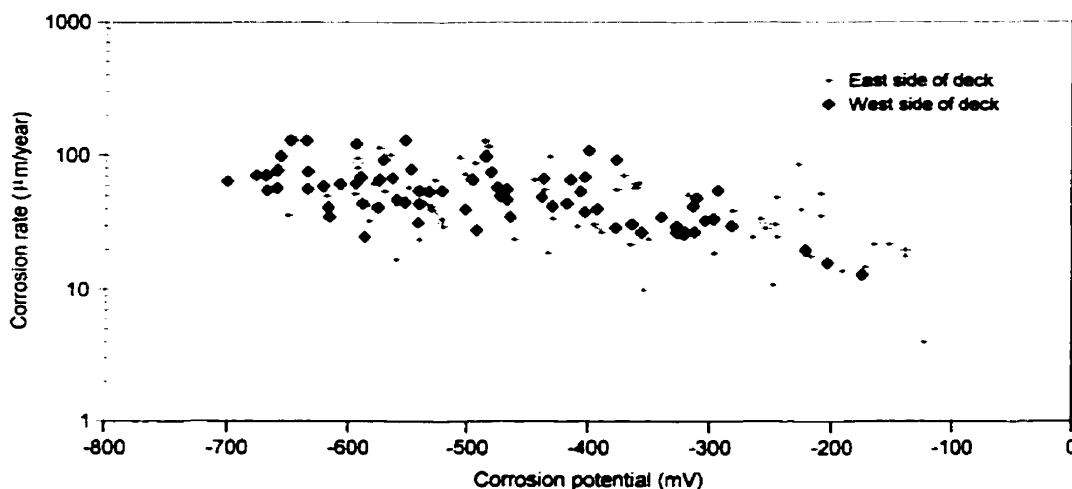
Figure 6-27: Corrosion rate vs. corrosion potential
