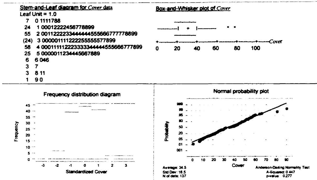
Figure G-5: Analysis 1 for concrete cover thickness (entire deck)
