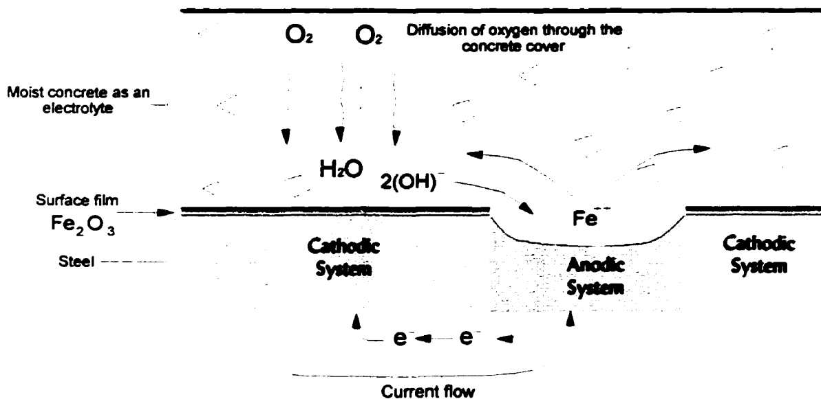
Figure 2-7: Corrosion process [48]
