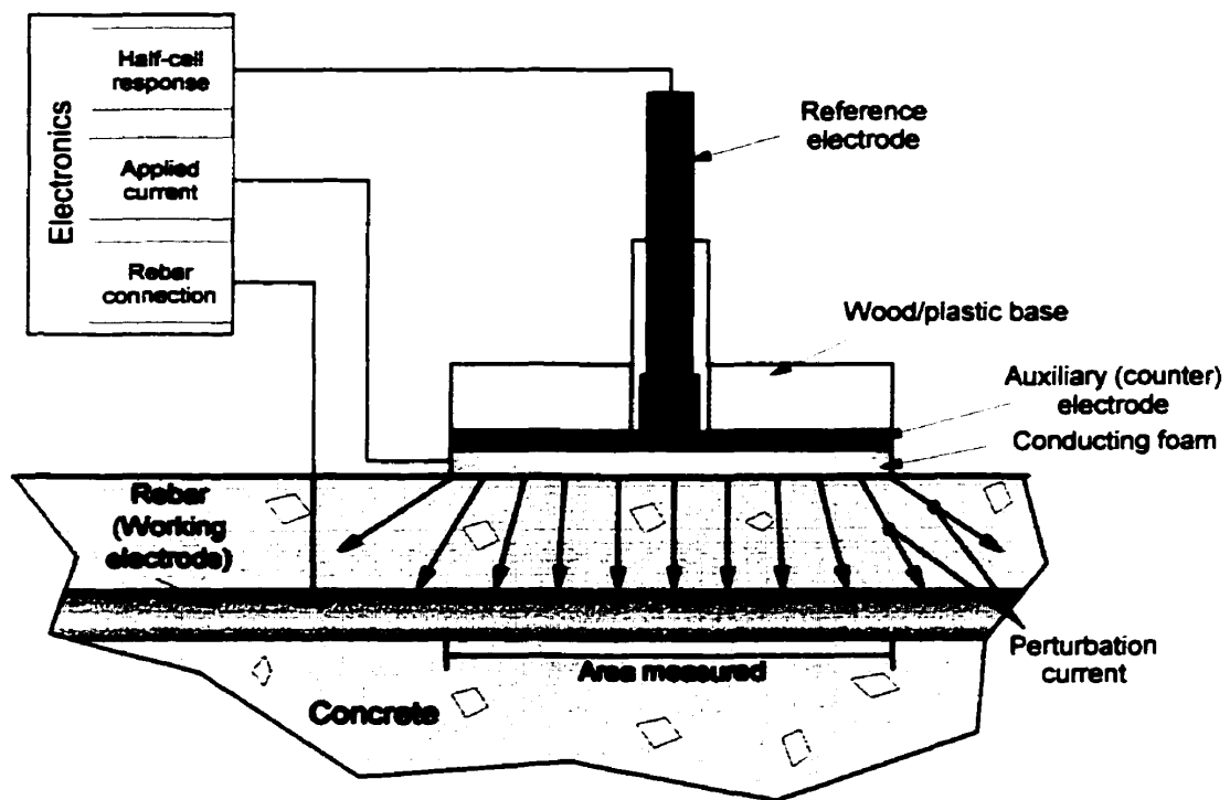
Figure 3-14: Schematic of the setup for linear polarization [33, 65]
