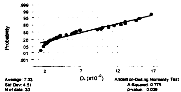
Figure G-10: Analysis 2 for apparent chloride diffusion coefficient (entire deck)
