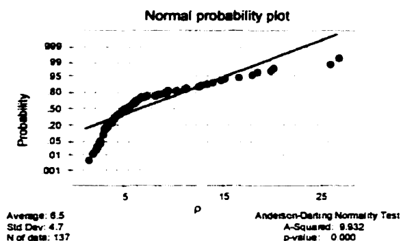
Figure G-15: Analysis 1 for resistivity of concrete (entire deck)
