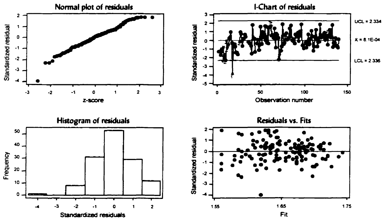
Figure H-3: Standardized residual model diagnostics for 'Cover' (entire deck)
