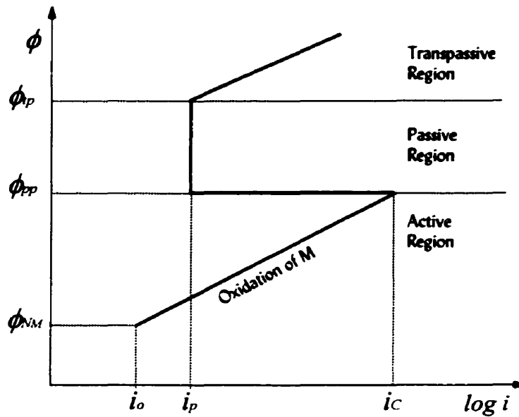
Figure 3-10: Polarization diagram of a metal exhibiting passivity [55, 56]
