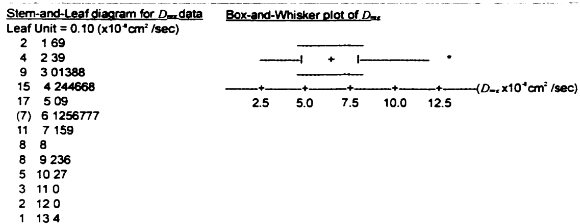
Figure 6-22: Stem-and-leaf diagram and box-and-whisker plot for D_{mg} (Analysis 1)
