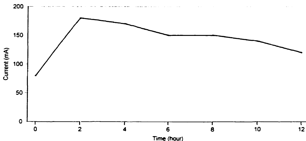
Figure 4-17: Current versus time plot for Site 15 (12-hour test duration)
