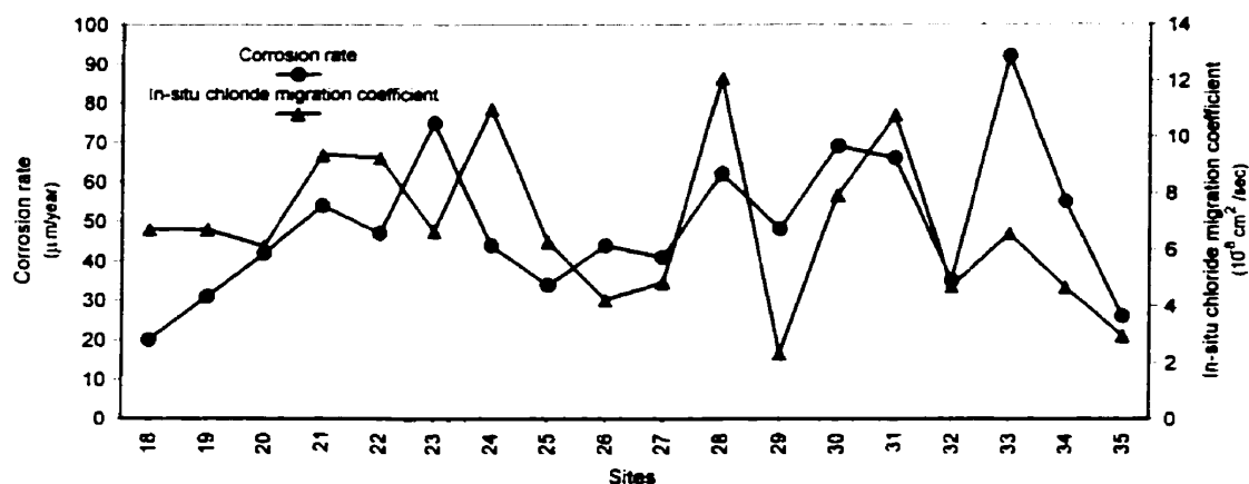
Figure 6-6: Dependence of in-situ chloride migration coefficient on corrosion rate (west side of deck)
