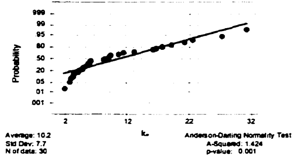
Figure G-19: Analysis 2 for coefficient of permeability (entire deck)
