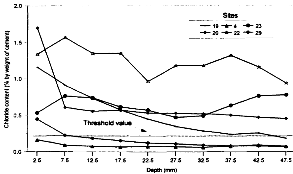
Figure D-4: Chloride profiles (Sites 4, 19, 20, 22, 23 and 29)
