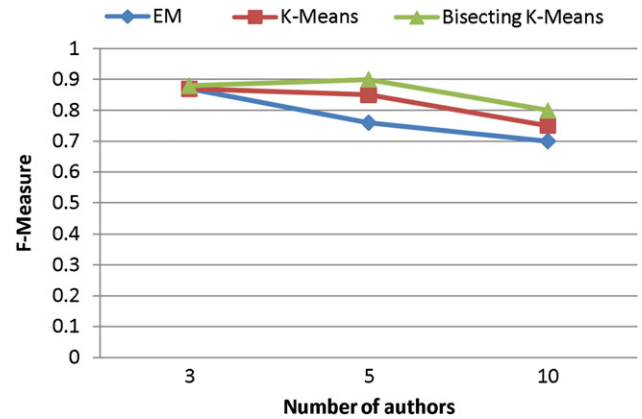
Fig. 4 – F-Measure vs. Number of authors and Clustering Algorithms (Messages = 100, Features = T_1 + T_2 + T_3 + T_4 ).
