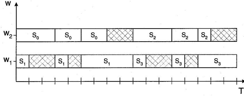
Fig. 3.4 Example 1: Allocation schedule of two available wavelengths (shown by two different colors) achieved by SEQSAM. S_i denotes the source node i . The schedule length in this example is 17 time slots.
