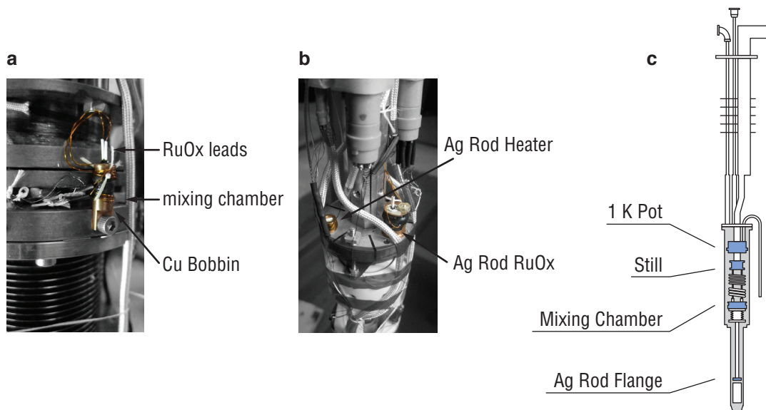
Figure 3.6: a : A view of the standard mounting scheme for a RuOx thermometer encased in a Cu bobbin and heat sunk to the mixing chamber. b : The Ag Rod tail showing a heater and thermometer. c : The locations of the four resistance thermometers on the fridge.
