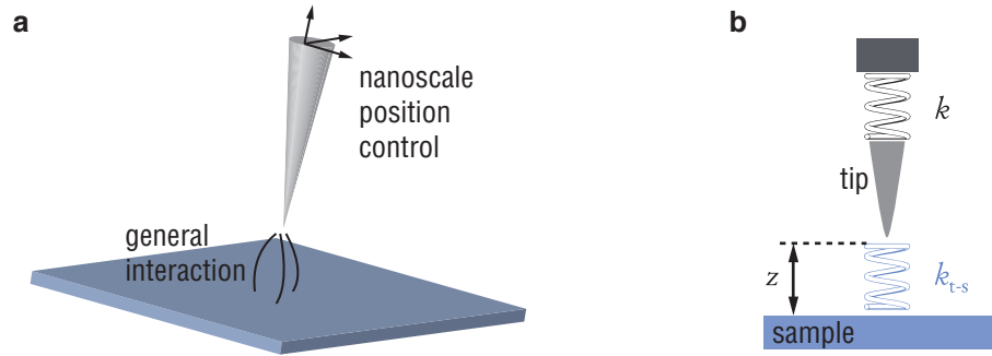
Figure 1.1: a: A generalized interaction between a generalized tip and sample. The interaction strength depends on position and the tip is capable of nanoscale motion in all three dimensions. b: The effective, distance dependent spring constant k_{t-s} created by the tip-sample interaction.
