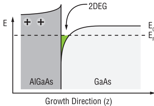
Figure 5.1: Energy diagram of the modulation doped AlGaAs/GaAs heterojunction showing the region where the 2DEG forms as the conduction band, E_C bends below the Fermi level, E_F .
