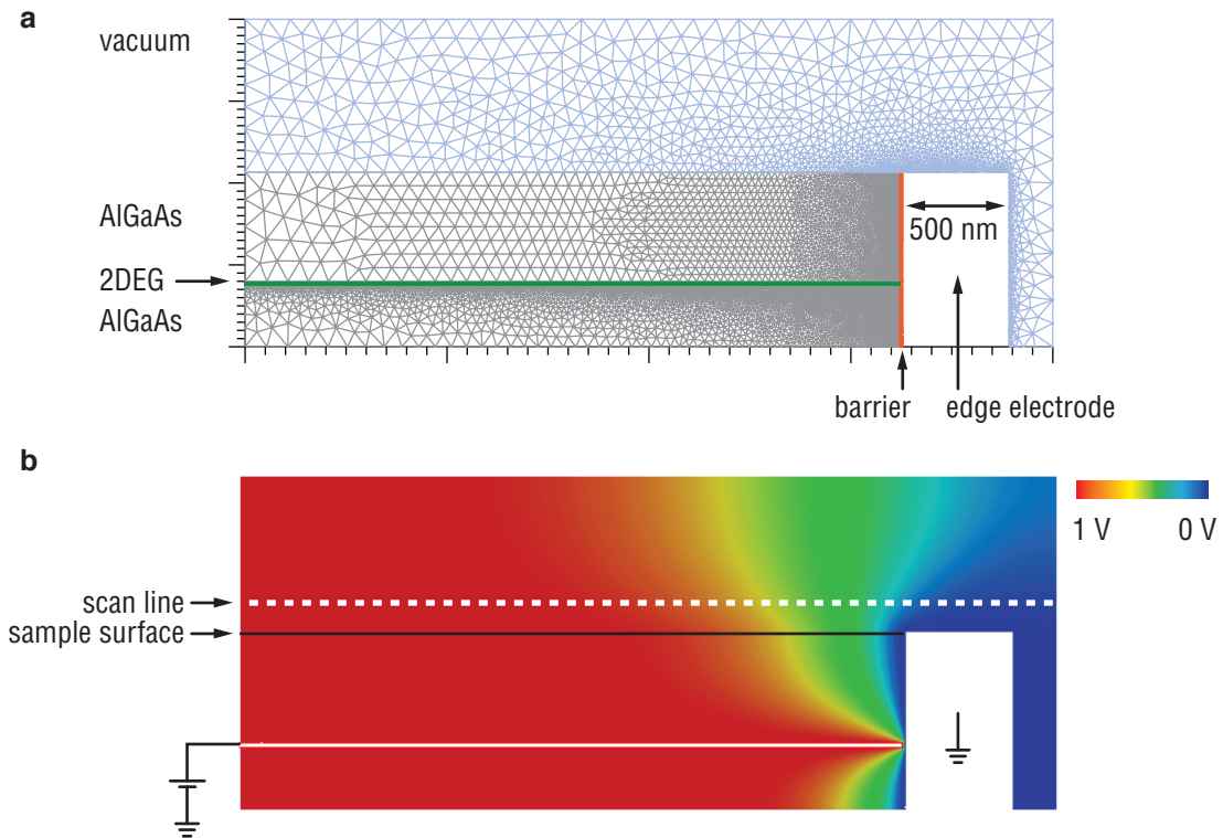
Figure 5.19: a: The mesh of the sample geometry. b: Resulting potentials when a voltage is applied to the 2DEG and the edge electrode is grounded. A dotted white line indicates the location of the tip during a pass over the edge ( \sim 100 nm above the surface)
