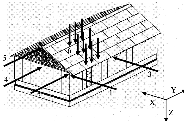
Figure 5: Applied load tests (see Table 1)
