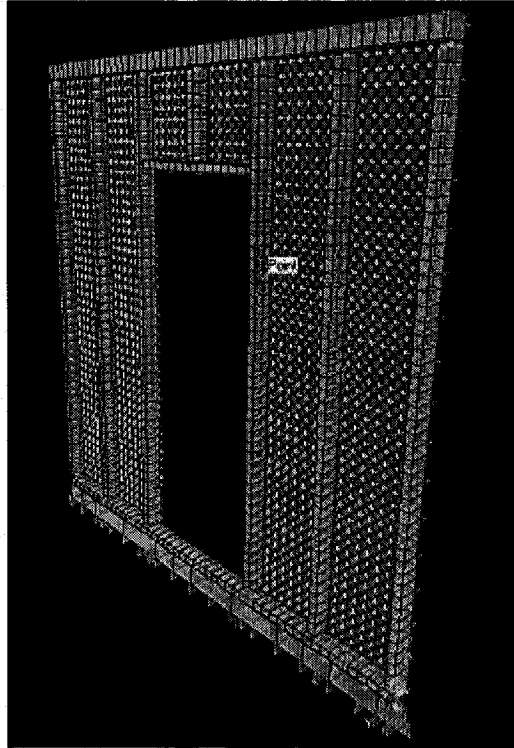
Figure 10. Example of mesh showing detailed modeling of all physical elements of shear Wall No. 4
