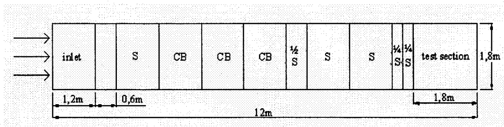
Figure 6: Upstream roughness panel set-up for wind tunnel testing
