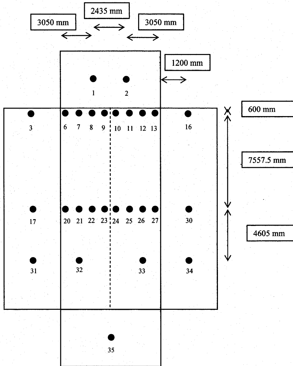
Figure 3: Distribution of pressure taps on the test house
