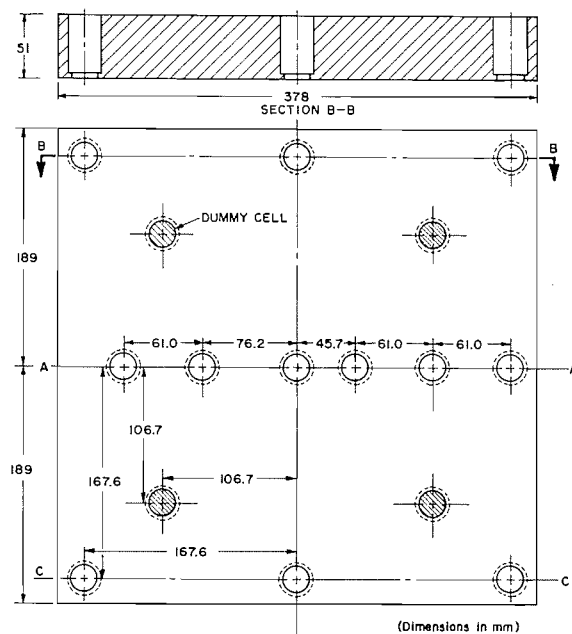
FIG. 5. The test plate and a configuration of contact stress transducers.
