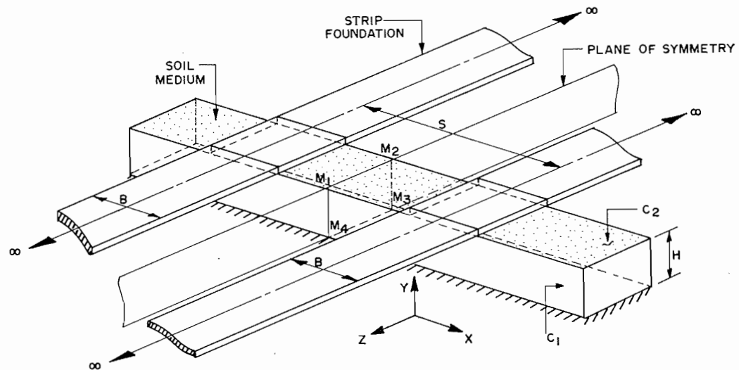
FIG. 3. Modelling of the problem of two interfering strip foundations (plane strain problem).
