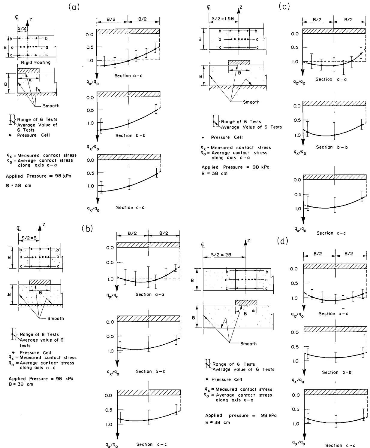
FIG. 10. Contact stress distribution beneath one of two interfering rigid strip foundations. (a) Spacing ratio S/B = 1 . (b) Spacing ratio S/B = 2 . (c) Spacing ratio S/B = 3 . (d) Spacing ratio S/B = 4 .
