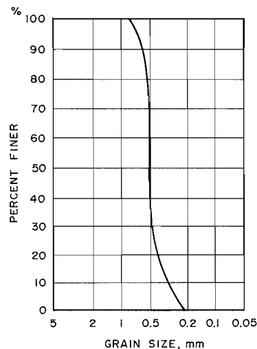
FIG. 6. Particle size distribution for the Ottawa sand.
