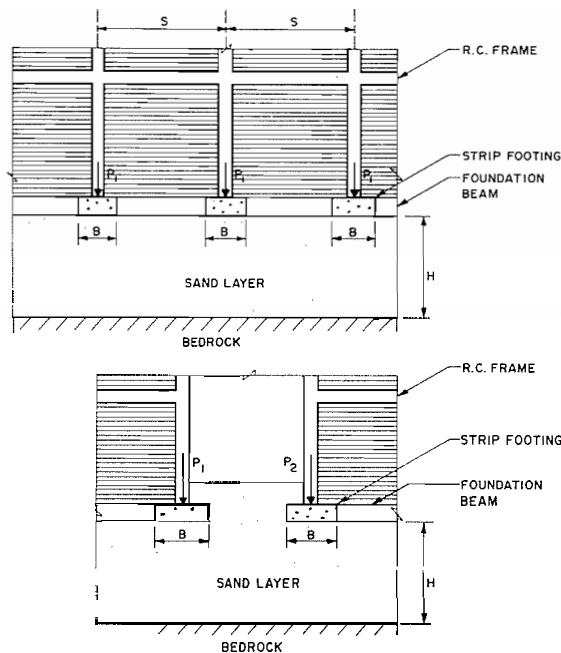
FIG. 1. Examples of mutual interference between strip foundations.
