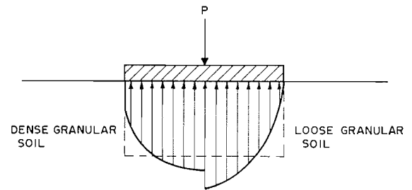
FIG. 11. Probable influence of soil density on the contact stress distribution.
