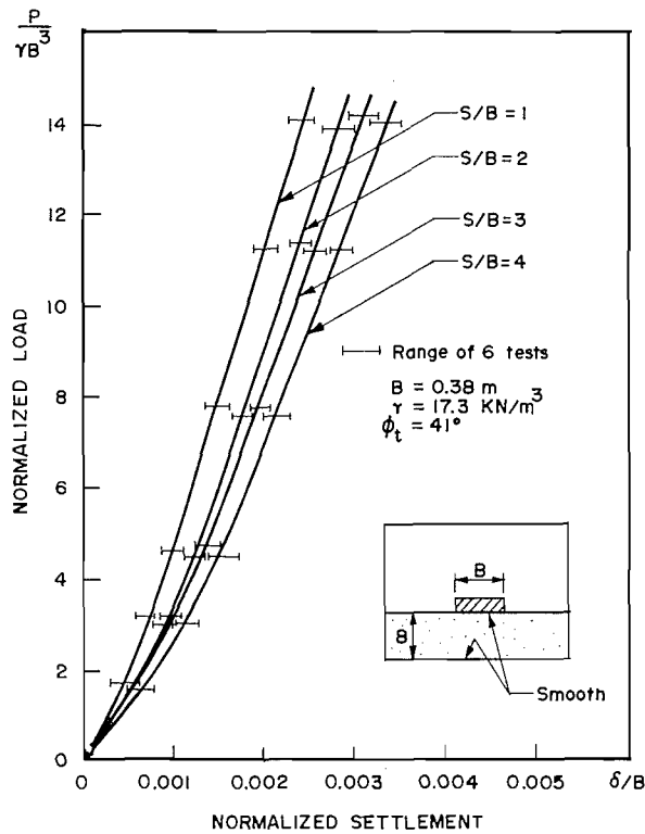
FIG. 8. Load-settlement curves of two interfering rigid strip foundations resting on a layer of sand and underlain by a rigid base.
