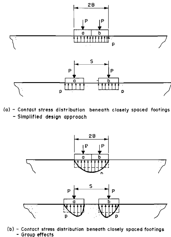
FIG. 2. Contact stress distribution beneath closely spaced footings. Comparison between the simplified design and group effect approaches.
