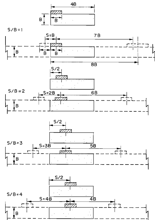
FIG. 12. Test plate and its counterpart.
