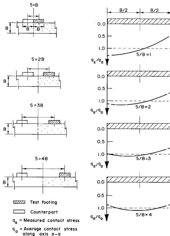
FIG. 13. Effect of spacing on the contact stress distribution.
