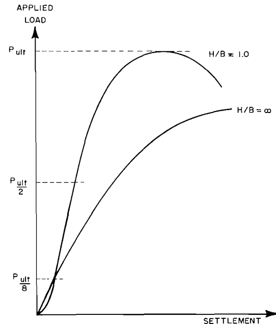
FIG. 9. Probable influence of rough rigid base on the load-settlement curve for a loaded footing - plane strain problem.
