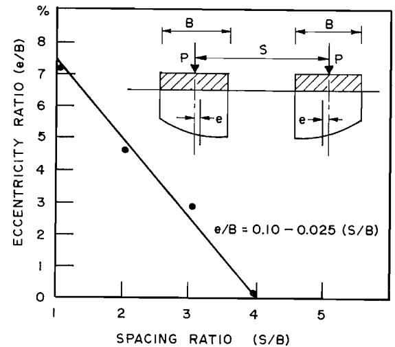
FIG. 14. Relationship between spacing and eccentricity due to interference of two rigid strip foundations.
