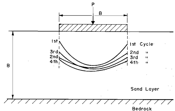
FIG. 7. Influence of the load cycling on the contact stress distribution beneath a rigid strip foundation resting on a granular soil underlain by a rigid base.
