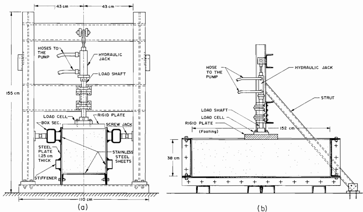
FIG. 4. The plane strain apparatus. (a) Cross section; (b) longitudinal section.
