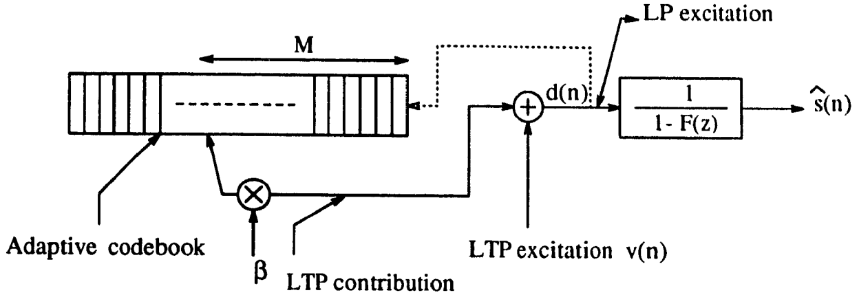
Figure 3.1: Single-tap pitch predictor; adaptive codebook illustration.
