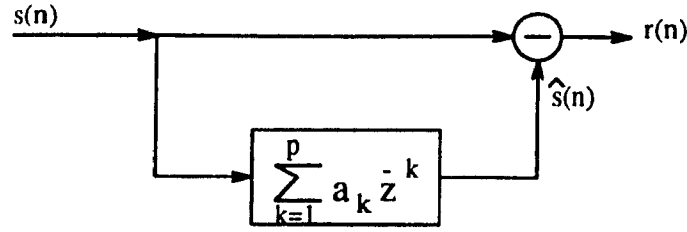
Figure 2.1: Formant Prediction.
