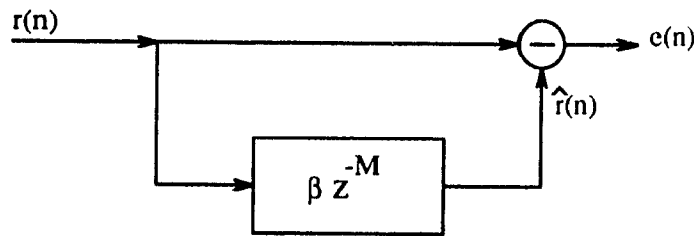
Figure 2.2: Pitch Prediction.
