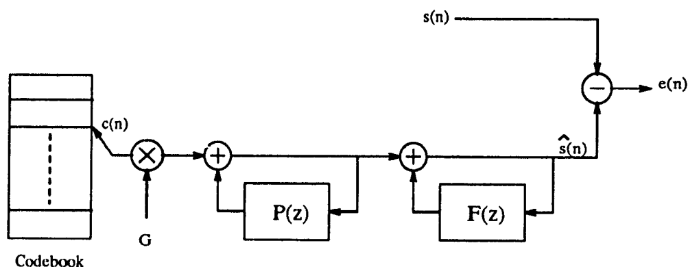
Figure 2.5: Analysis-by-synthesis coder.
