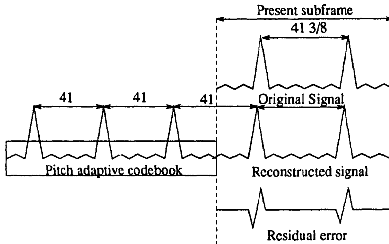
Figure 4.7: Motivation for time scaling.
