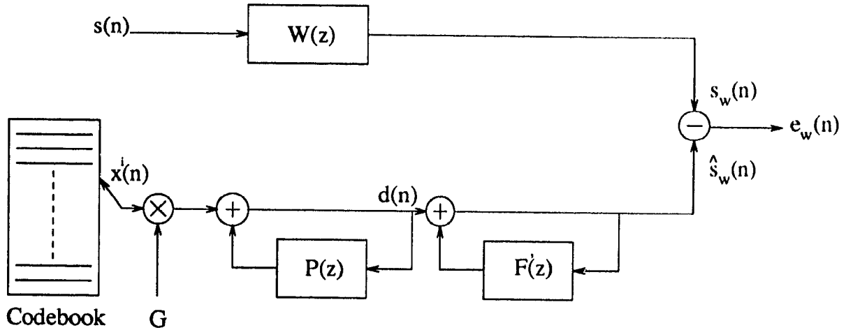
Figure 2.6: Basic CELP configuration.
