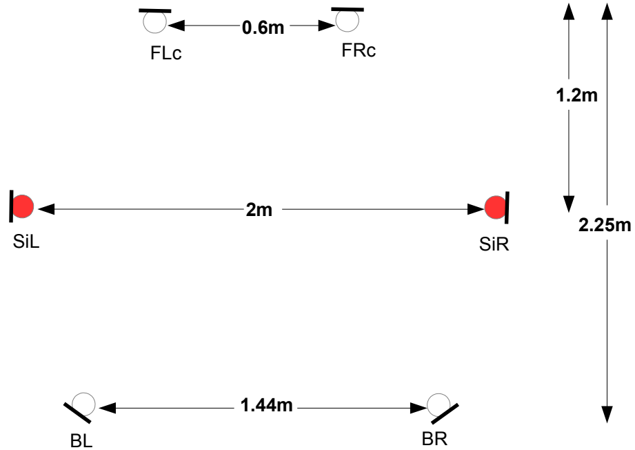
Main microphone array
