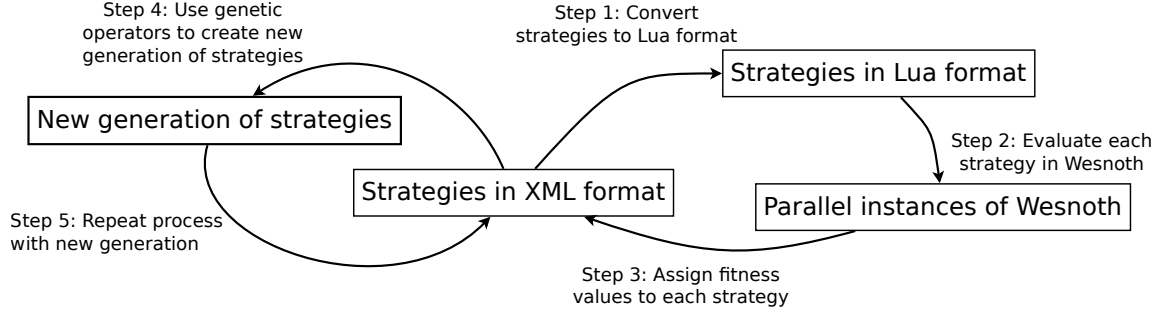
Figure 6.1: Diagram of evolutionary algorithm
