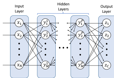
Figure 4-11 A general MLP diagram showing the input layer, the hidden layers and the interconnected hidden units, and the output layer.
