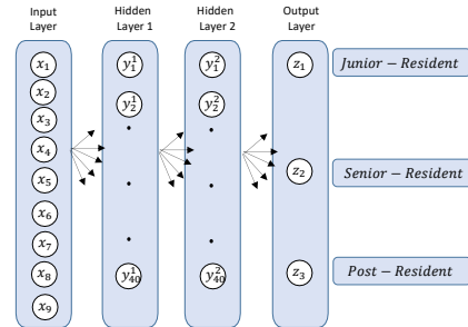
Figure 4-12 Pre-trained model architecture
