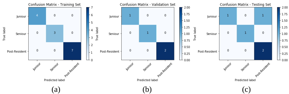
Figure 4-7 Confusion matrices highlighting the performance of the trained model on the: (a) training set, (b) validation set, and (c) testing set.
