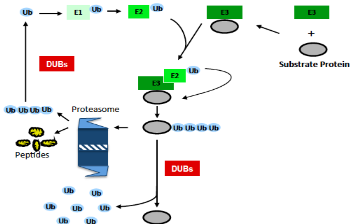
Figure II: The Ubiquitin Proteasome System (UPS). Three enzymatic steps mediate Ubiquitin conjugation: E1 (ubiquitin activating enzyme) activates and transfers ubiquitin to E2 (ubiquitin conjugating enzyme), which then functions with a E3 (ubiquitin ligase) to mediate ubiquitination. The E3 provides substrate recognition and specificity. The linkage of ubiquitin can be reversed through the catalytic action of deubiquitinating enzymes (DUBs).
