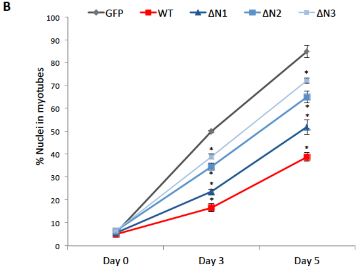
Figure 5: Deletion of USP19 N-terminal domains diminishes its ability to modulate muscle cell fusion. C2C12 myoblasts were infected with adenovirus expressing GFP control or USP19 WT, \Delta N1, \Delta N2, or \Delta N3 to yield similar levels of overexpression and induced to differentiate for five days. The cells were fixed, stained and visualized under a light microscope (10X) on the indicated days. Representative samples of cell morphology on day 0, 3 and 5 of differentiation are shown in (A). (B) The fusion index was determined by counting the nuclei from three randomly selected images per group per day and calculating the proportion of nuclei in myotubes (defined as cells with \geq 2 nuclei). Means that are statistically significant compared to GFP on the same day with * P < 0.001 (2-way ANOVA).
