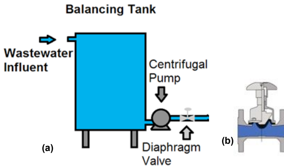
Figure 4. (a) Closer view of balancing tank, along with centrifugal pump and diaphragm value. (b) Detailed picture of the diaphragm valve while open.
