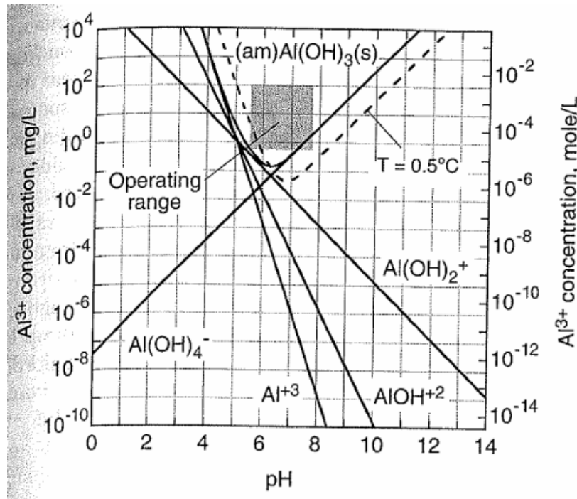
Figure 12: Graph showing the effect of pH on the solubility and precipitation of aluminum sulfate, with an ideal operating range existing between a pH of 5.5 and 7.5. Source: https://awwoa.ab.ca .
