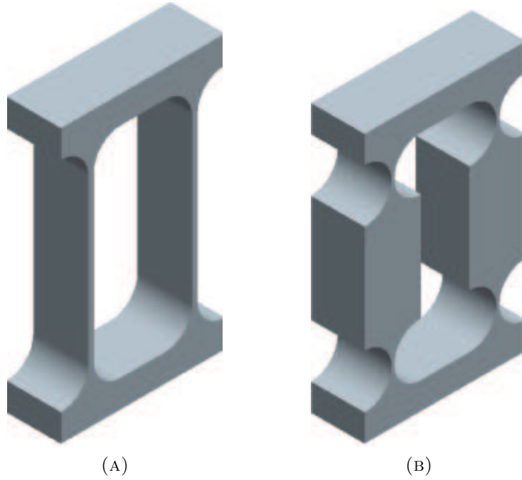
FIGURE 2.4. Compliant realization of the II-joint: (a) with a pair of constant cross-section beams; and (b) with four notched beams
