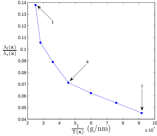
FIGURE 5.8. Pareto frontier
