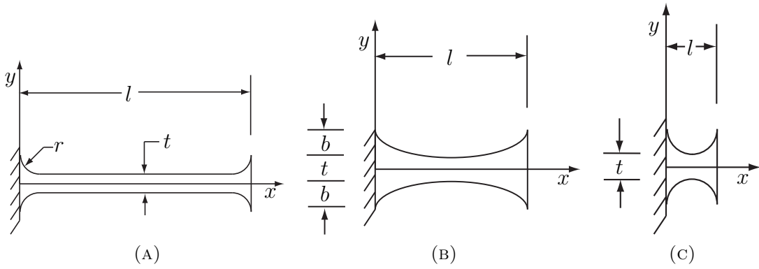
FIGURE 2.2. Compliant Hinge: (a) corner-filletted hinge; and (b) elliptic flexural hinge; and (c) notched-beam flexural hinge
