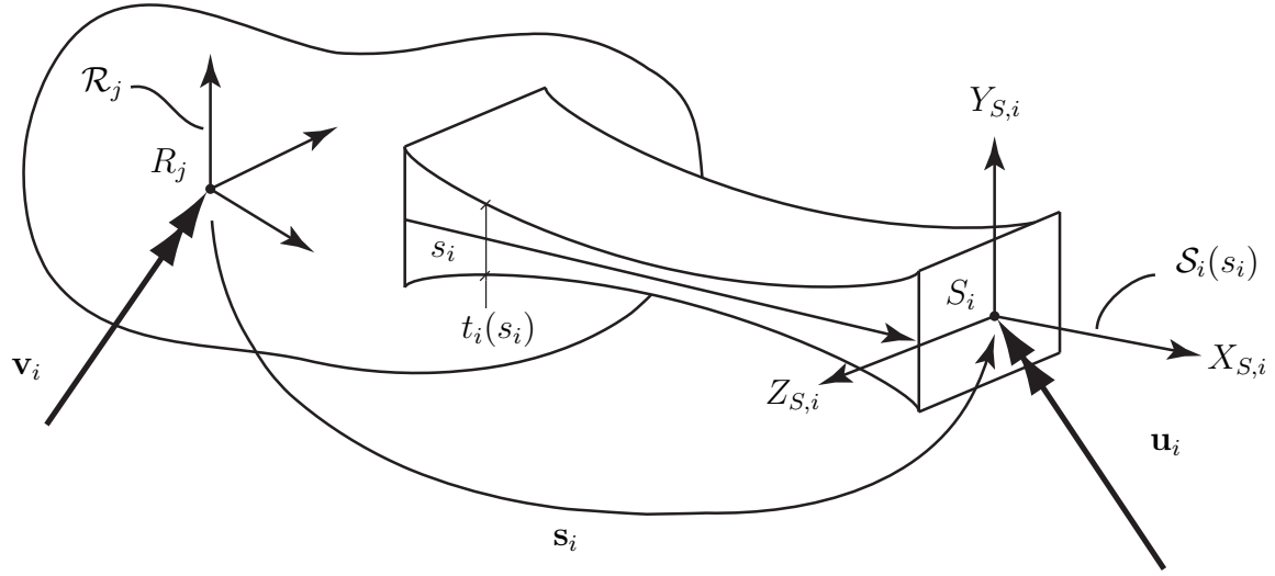
FIGURE 3.1. The i th compliant link attached to the j th rigid link: (a) layout; (b) detail of the definition of \mathcal{S}_i(s_i)
