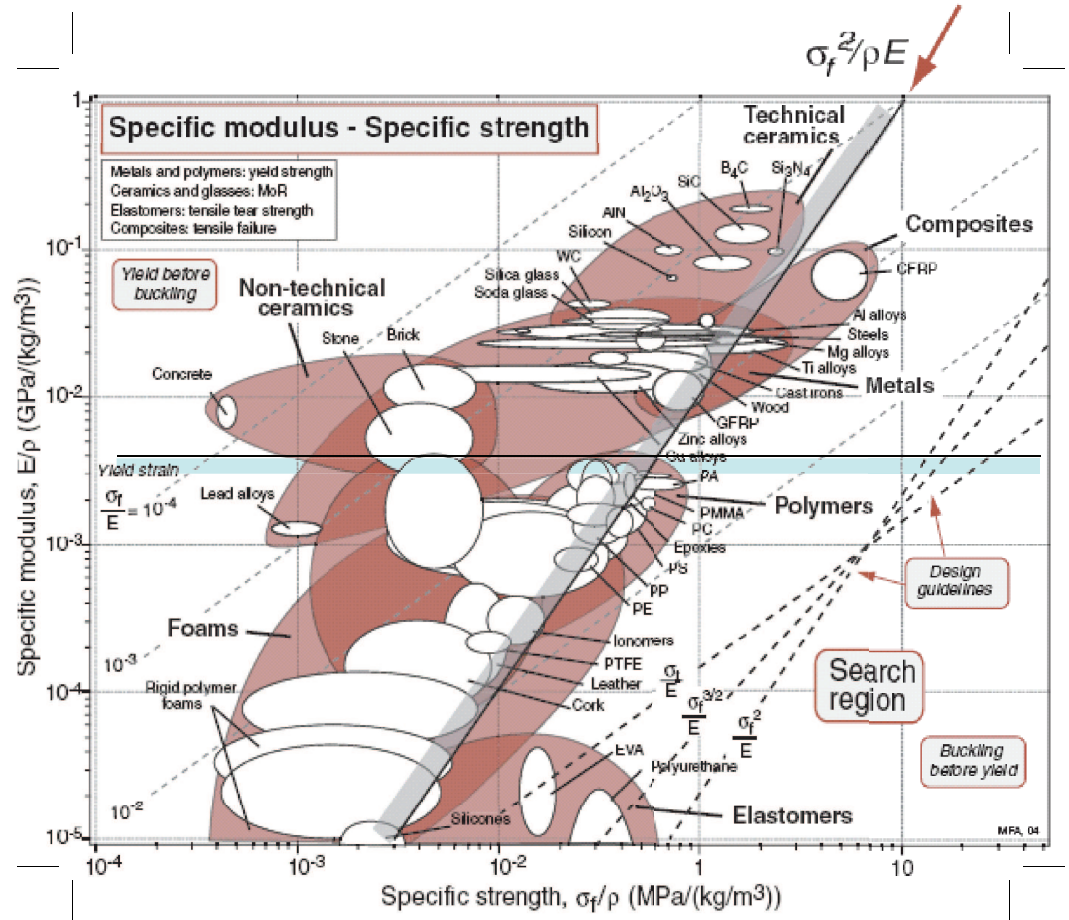
FIGURE 2.9. The S_y/\rho - E/\rho chart (Ashby, 2005)
