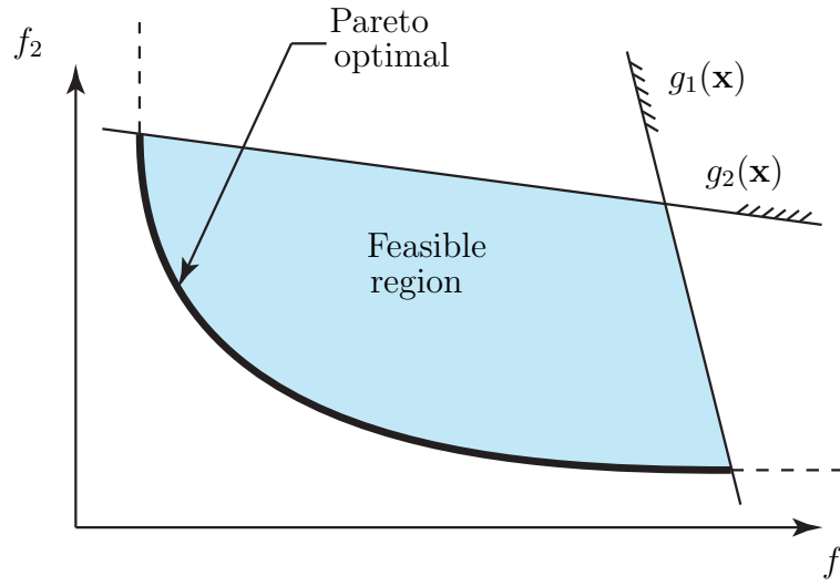
FIGURE 5.5. Bi-objective design space
