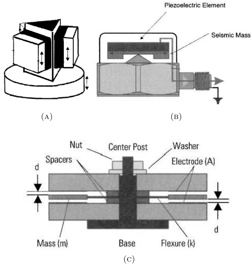
FIGURE 1.2. Example industrial accelerometers: (a) piezoelectric in shear mode, (b) piezoelectric in flexure mode; and (c) capacitive
