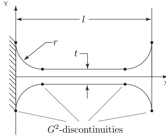
FIGURE 4.1. Corner filleted hinge
