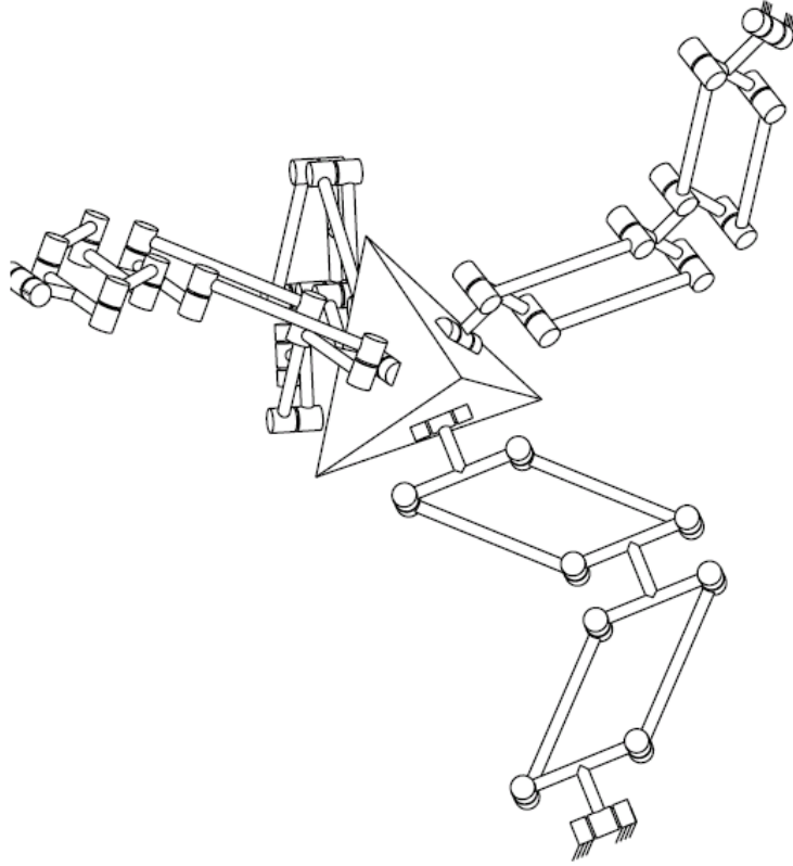
FIGURE 1.6. The simplicial 4RIIIIR triaxial accelerometer
