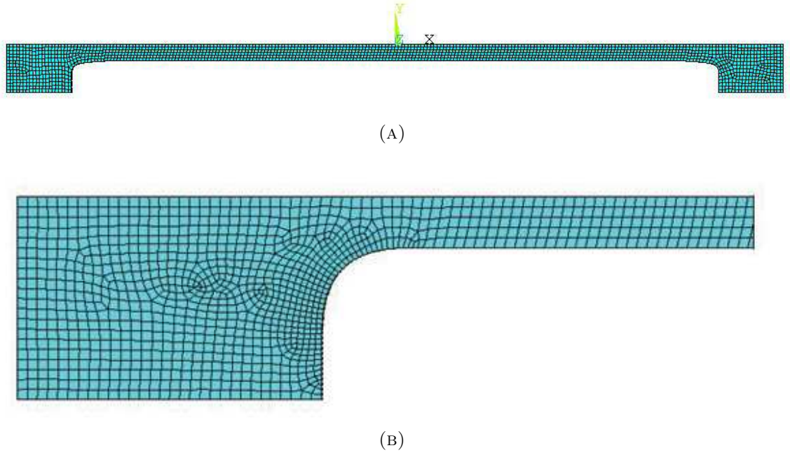
FIGURE 4.8. Meshing of the flexible beam: (a) front view; and (b) zoom-in on the fillet
