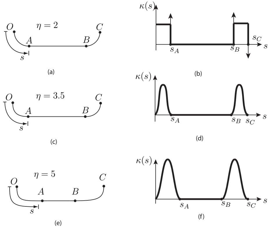
FIGURE 4.5. Flexible beam profiles and their corresponding curvature distributions: (a) (b) circular fillets; (c) (d) supercircular fillets; and (e) (f) superelliptical fillets
