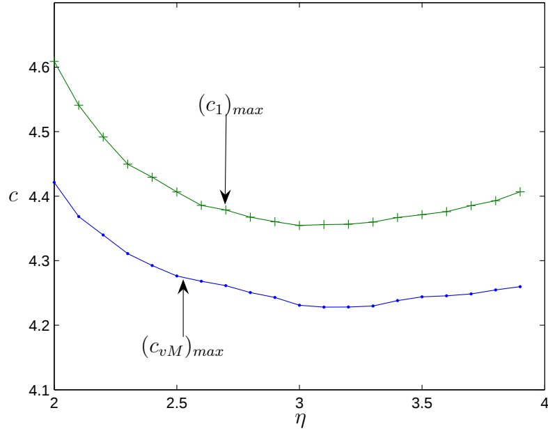
FIGURE 4.9. Stress concentration factor as a function of power \eta of a Lamé curve for supercircular fillet
