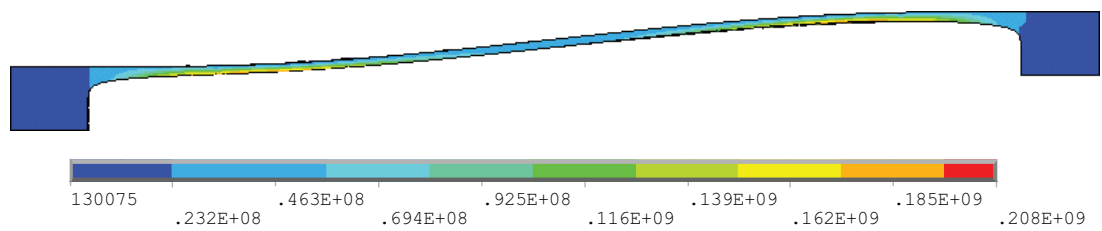
FIGURE 5.10. Von Mises stress distribution
