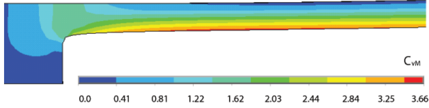
FIGURE 4.12. Von Mises stress concentration distribution of the optimum super elliptical fillet
