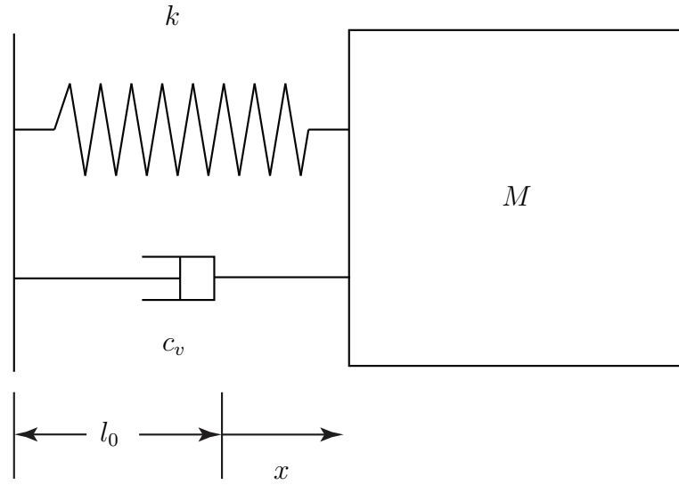
FIGURE 1.1. Mass-spring system of an accelerometer
