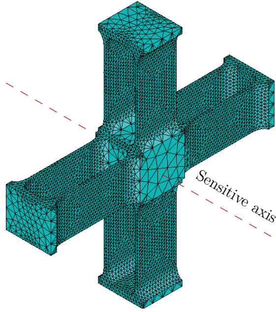
FIGURE 5.3. FE model of the accelerometer
