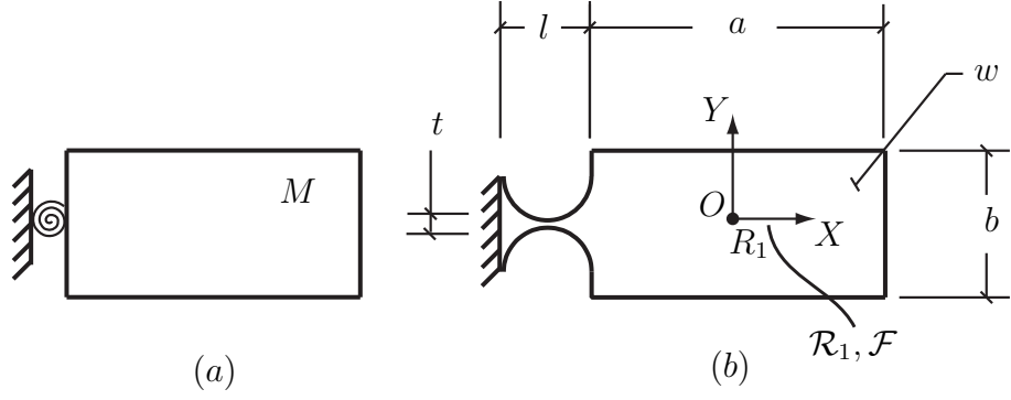
FIGURE 3.2. Notched beam: (a) Mass-spring representation; (b) compliant joint
