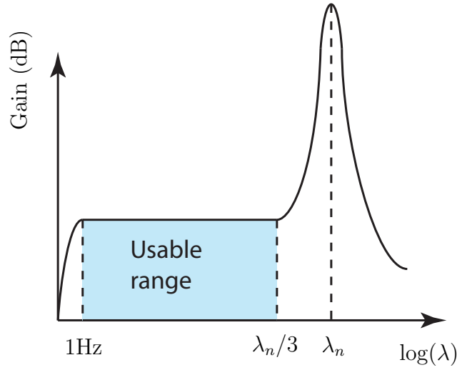
FIGURE 1.3. Frequency response
