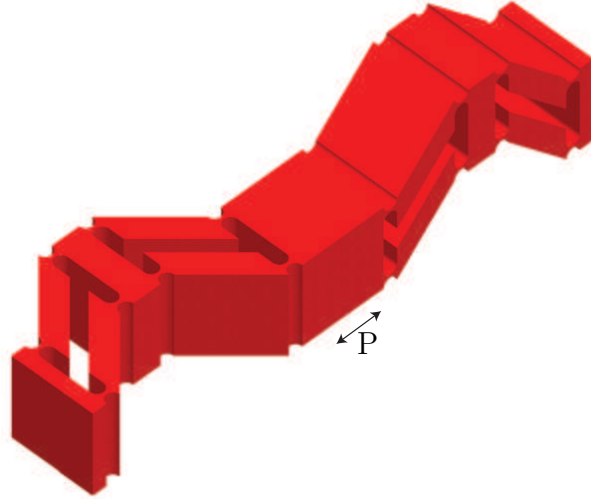
FIGURE 2.7. The Simplicial 2III Uniaxial Accelerometer
