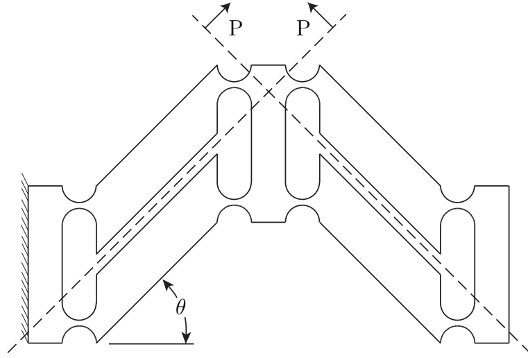
FIGURE 2.6. The compliant realization of the III-leg architecture
