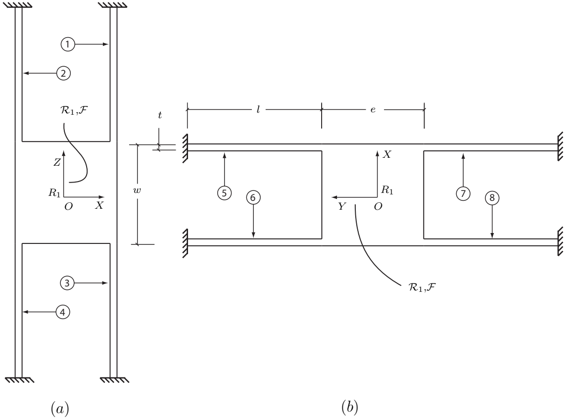
FIGURE 3.5. New layout of the uniaxial accelerometer: (a) left view; and (b) top view
