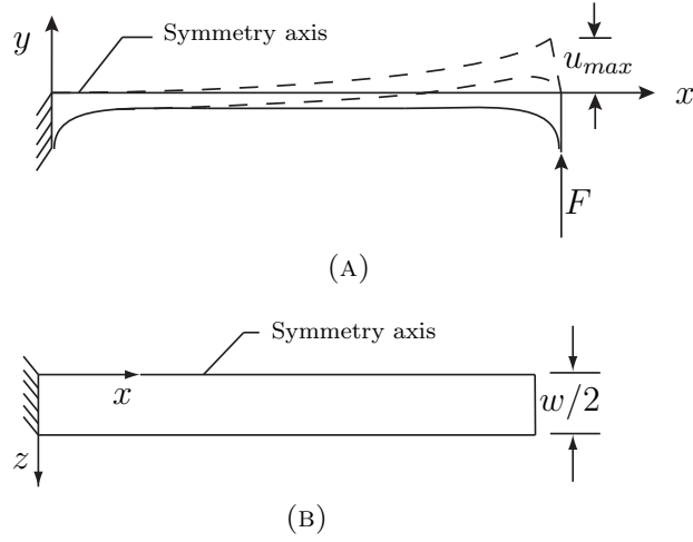
FIGURE 4.7. Structural model: (a) front view, (b) top view
