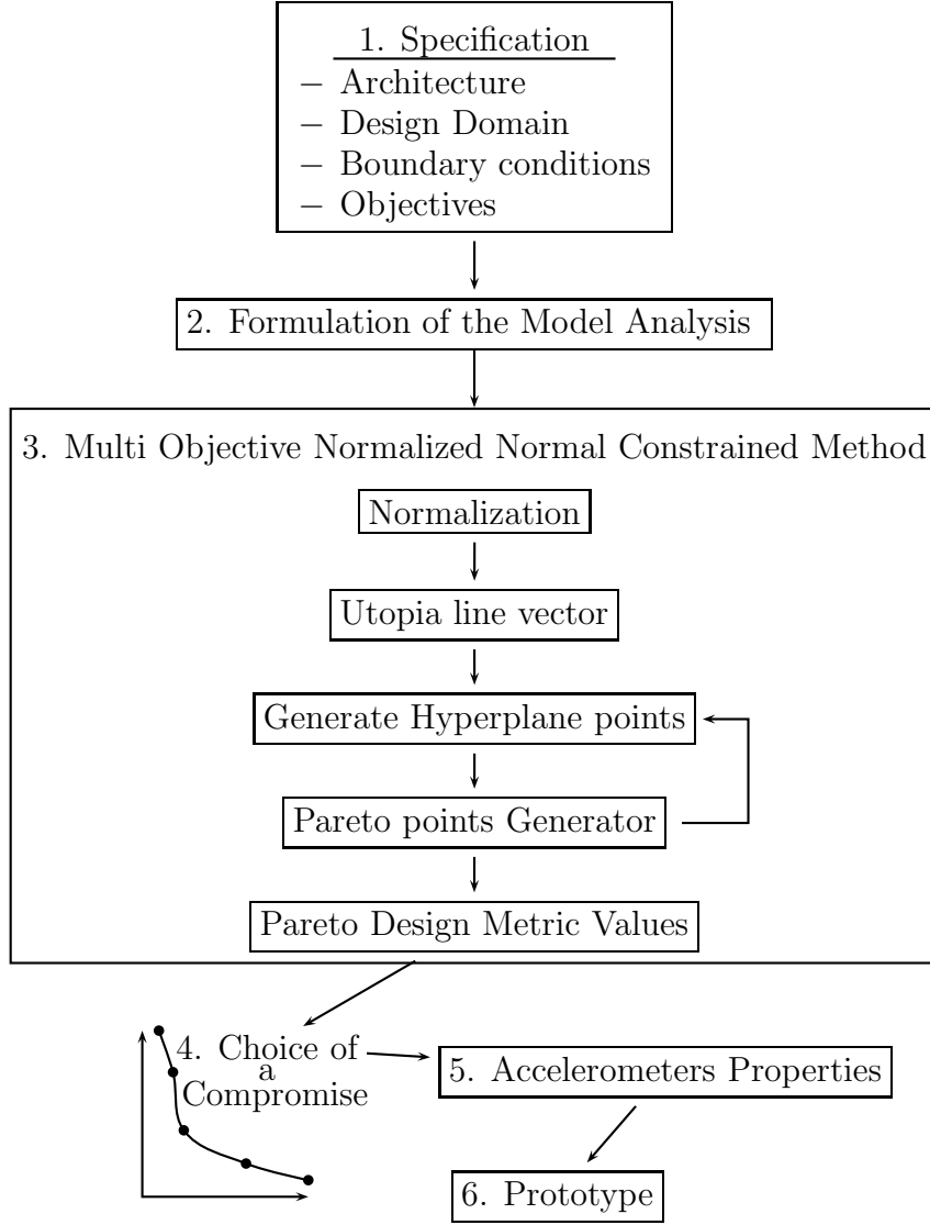
FIGURE 5.1. Methodology flow chart
