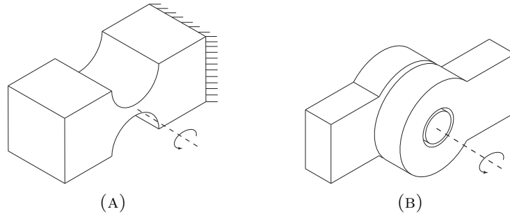
FIGURE 2.1. Revolute joint: (a) notched beam joint; and (b) standard mechanical revolute joint
