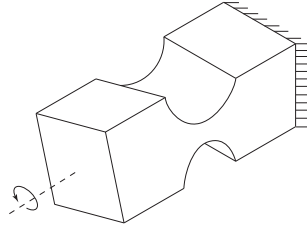
FIGURE 2.3. Revolute compliant hinge subjected to torsional loading
