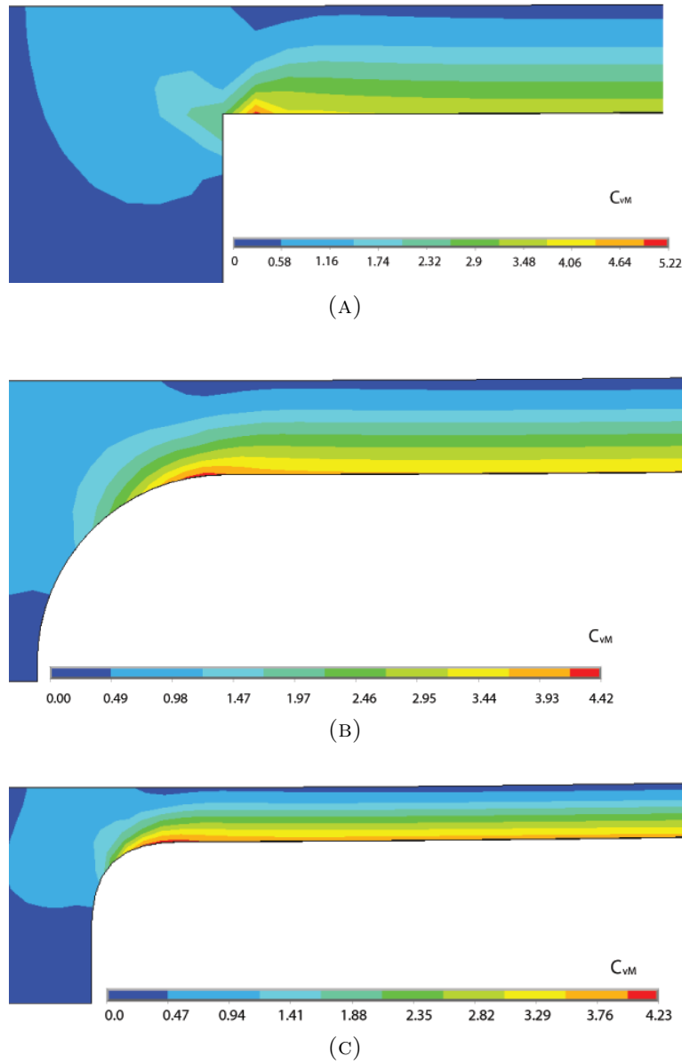
FIGURE 4.10. Von Mises stress distribution with (a) no fillet; (b) circular fillet; and (c) optimum supercircular fillet with \eta = 3.2
