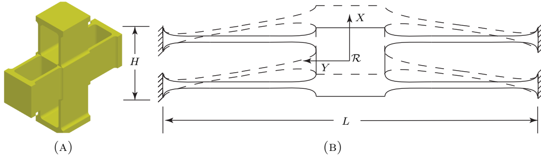
FIGURE 3.4. New layout: (a) CAD model; and (b) deformation along the sensitive axis
