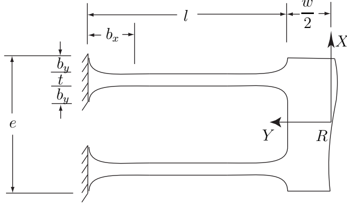
FIGURE 5.2. Parameterization of the cross-configuration mechanism
