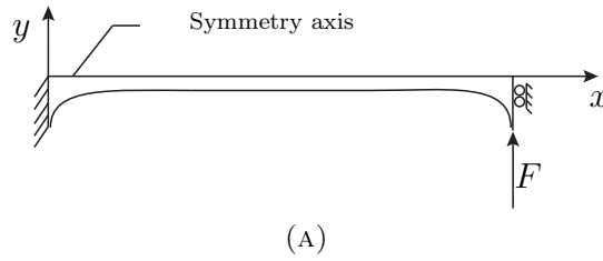
FIGURE 5.4. Structural model
