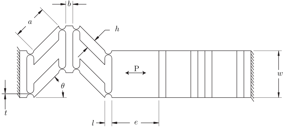
FIGURE 2.8. Parametrization of the 2III Configuration
