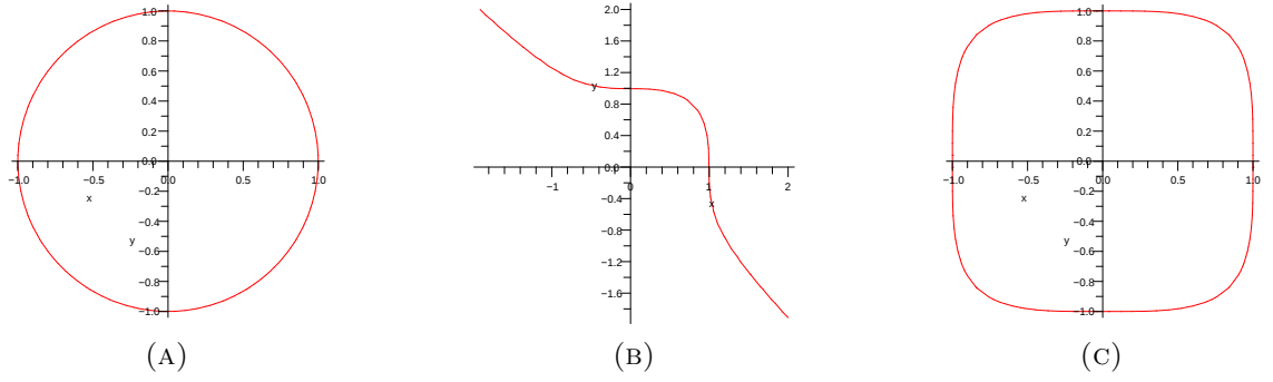
FIGURE 4.2. Lamé curves for: (a) \eta = 2 ; (b) \eta = 3 ; and (c) \eta = 4
