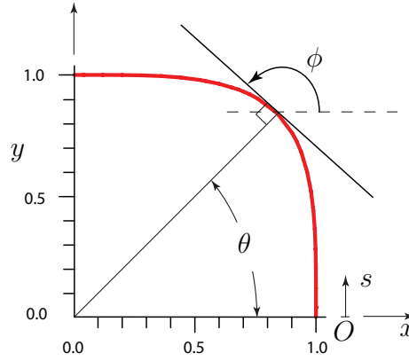
FIGURE 4.4. Lamé curves polar coordinate for \eta = 4
