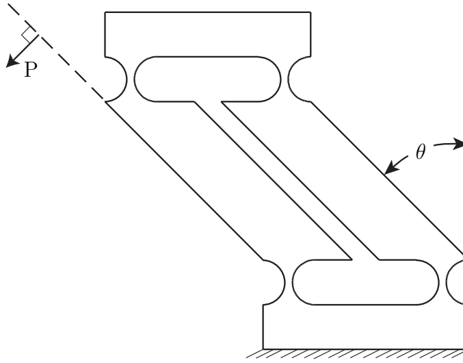
FIGURE 2.5. Compliant realization of the \Pi -joint in a \theta posture
