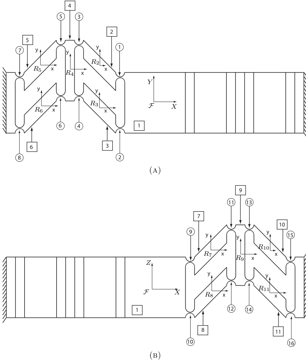
FIGURE 3.3. Uniaxial accelerometer: (a) front view; and (b) bottom view
