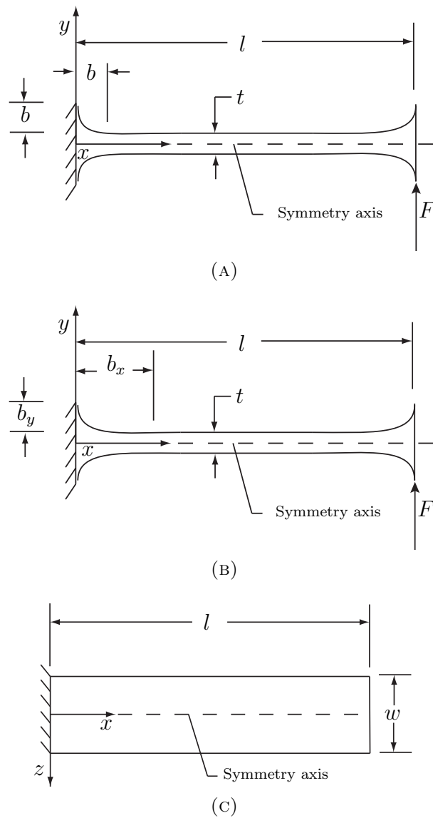
FIGURE 4.6. Geometry of a Lamé-filletted hinge: (a) supercircular filleted hinge; (b) superelliptical filleted hinge; (c) top view of both hinges
