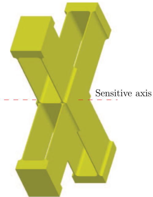
FIGURE 5.9. Optimum accelerometer
