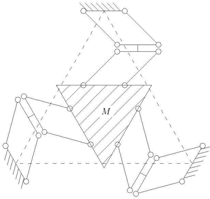
FIGURE 1.5. The simplicial 3III biaxial accelerometer
