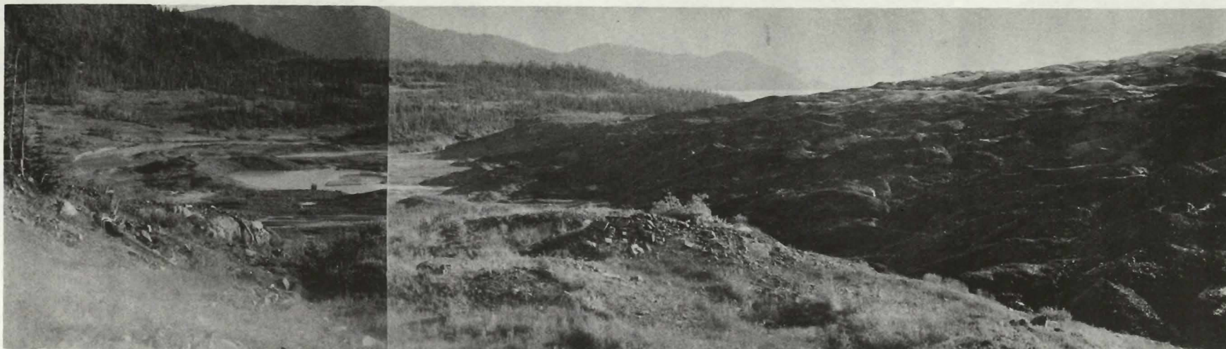
Columbia Glacier, east margin, 1935 from Station 22 Photos f-35-446, 447 by Wm. O. Field
