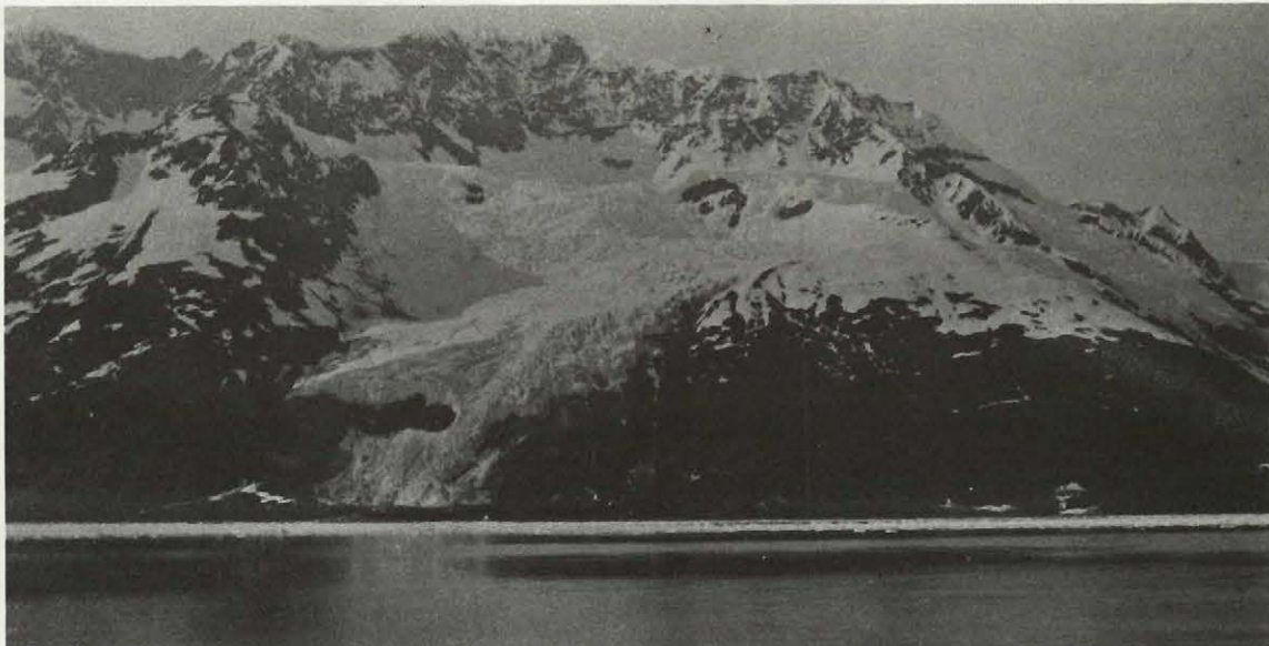
Baker Glacier, 1909, from Station F (Harriman) Photo 9-2 (198) by U.S. Grant
