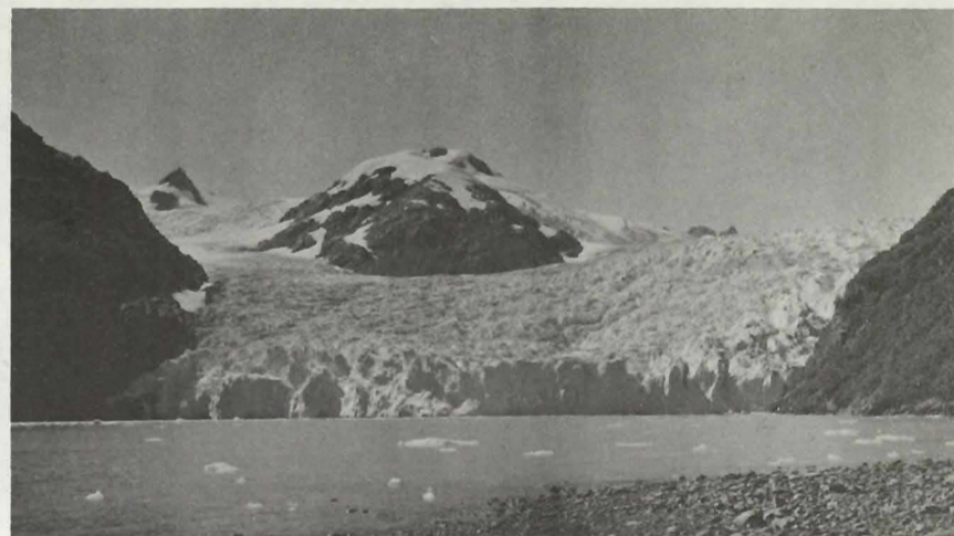
Tiger Glacier from Station B, 1957 Photo M-57-SG19 by M.T. Millett
