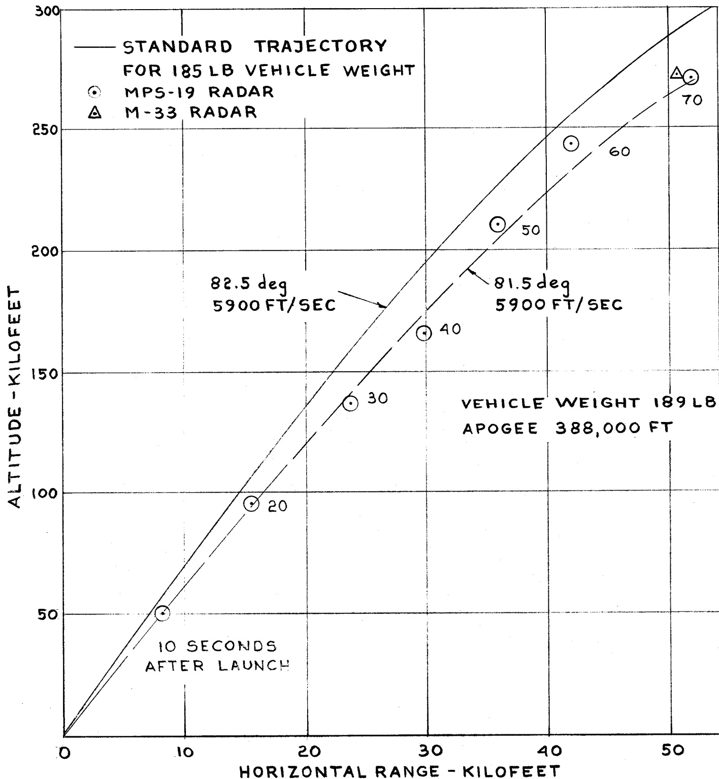
FIG.13c MARTLET 2C SHOT LUCRETIA ALTITUDE VS RANGE
