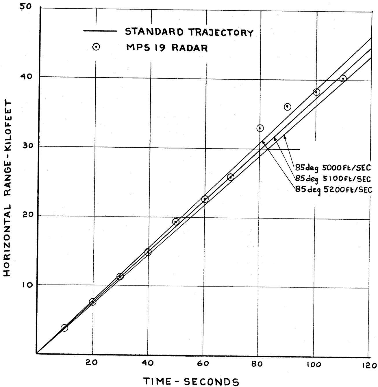
FIG.3b MARTLET 2A SHOT APPIUS RANGE VS TIME
