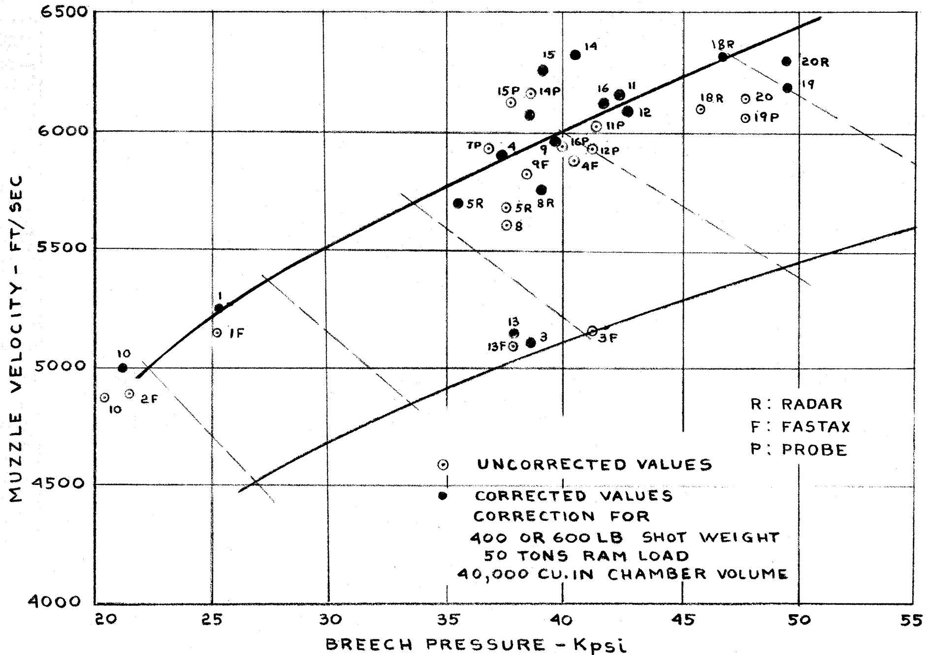
FIG.29 BALLISTIC PERFORMANCE OF M8M.220 IN 16.4" GUN WITH 51 FT MUZZLE EXTENSION
