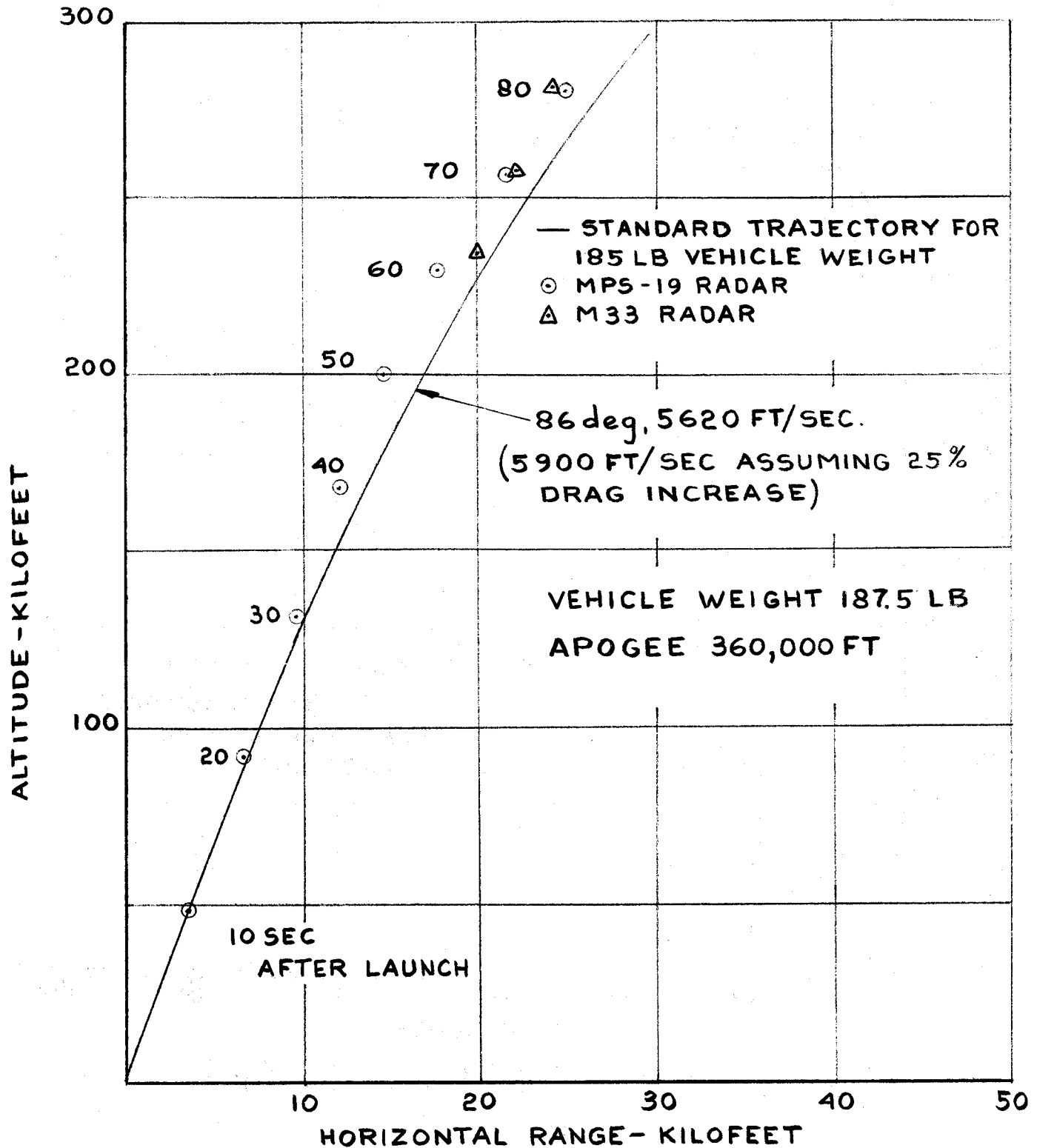
FIG. IIc. MARTLET 2C SHOT FABIUS ALTITUDE VS RANGE
