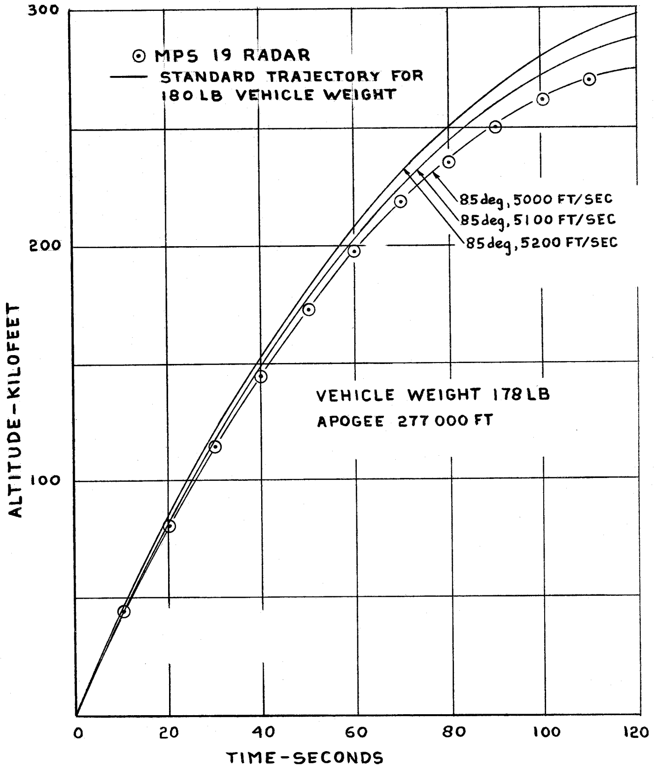
FIG.3a MARTLET 2A SHOT - APPIUS ALTITUDE VS TIME
