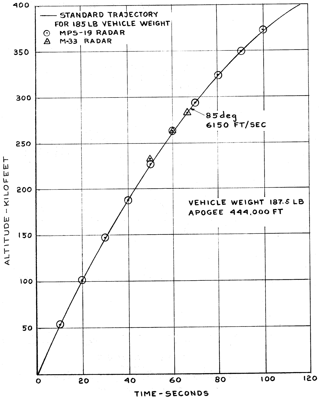
FIG 18 a MARTLET 2C SHOT QUINTUS ALTITUDE VS TIME
