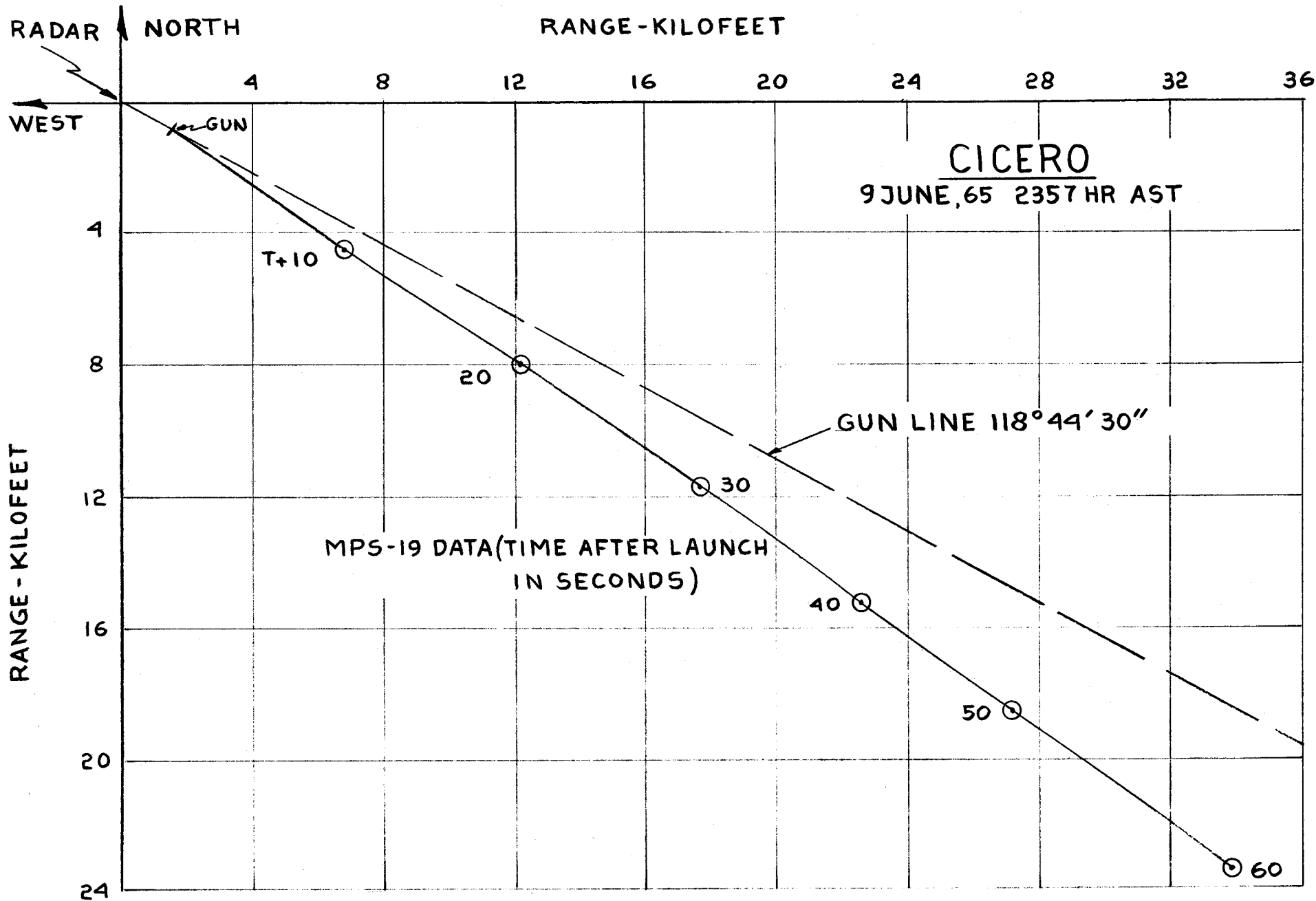
FIG.15 d PLAN VIEW OF MARTLET 2C CICERO TRAJECTORY
