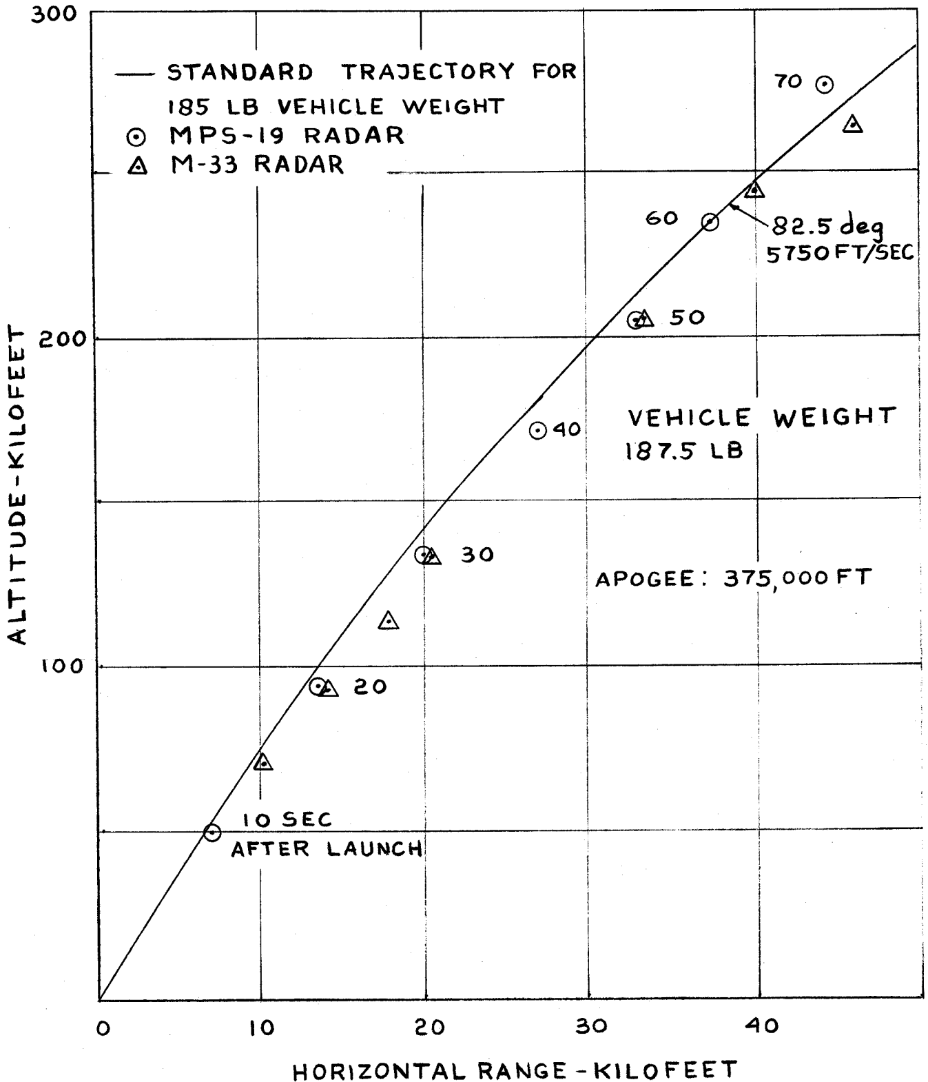
FIG.12c MARTLET 2C SHOT GRACCHUS ALTITUDE VS RANGE
