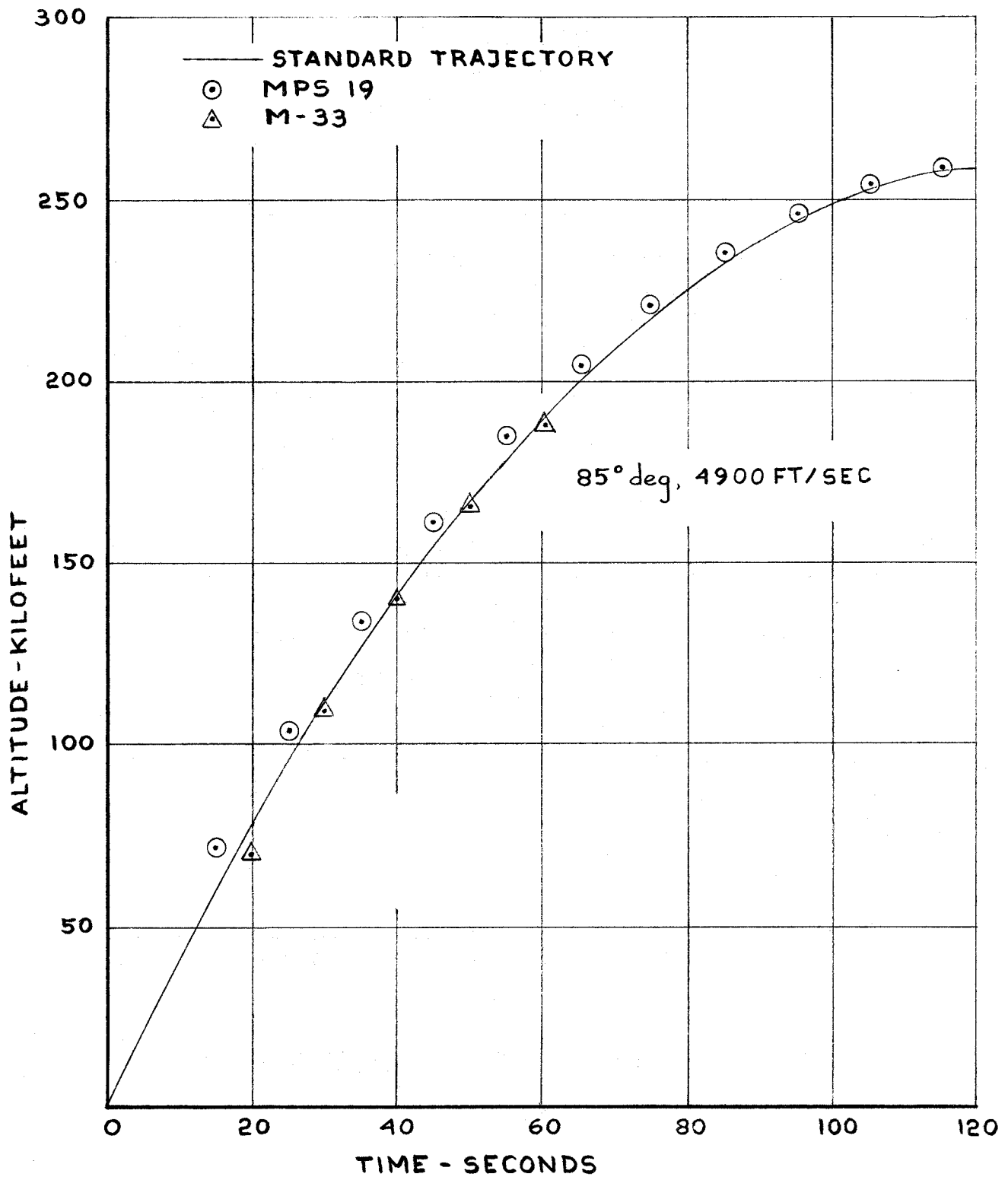
FIG. 4a MARTLET 2A SHOT-RUFUS ALTITUDE VS TIME
