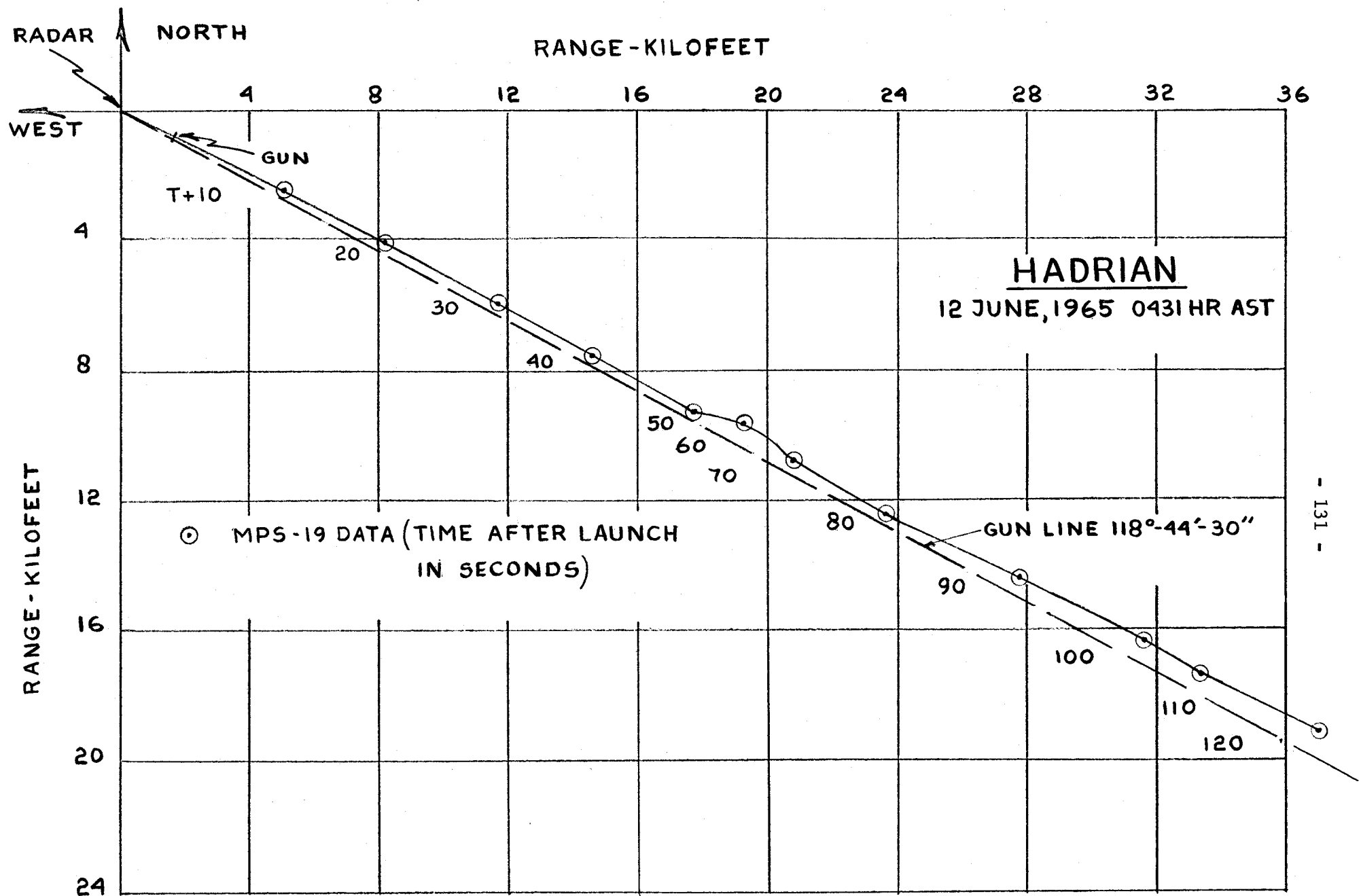
FIG.19d PLAN VIEW OF MARTLET 2C HADRIAN TRAJECTORY
