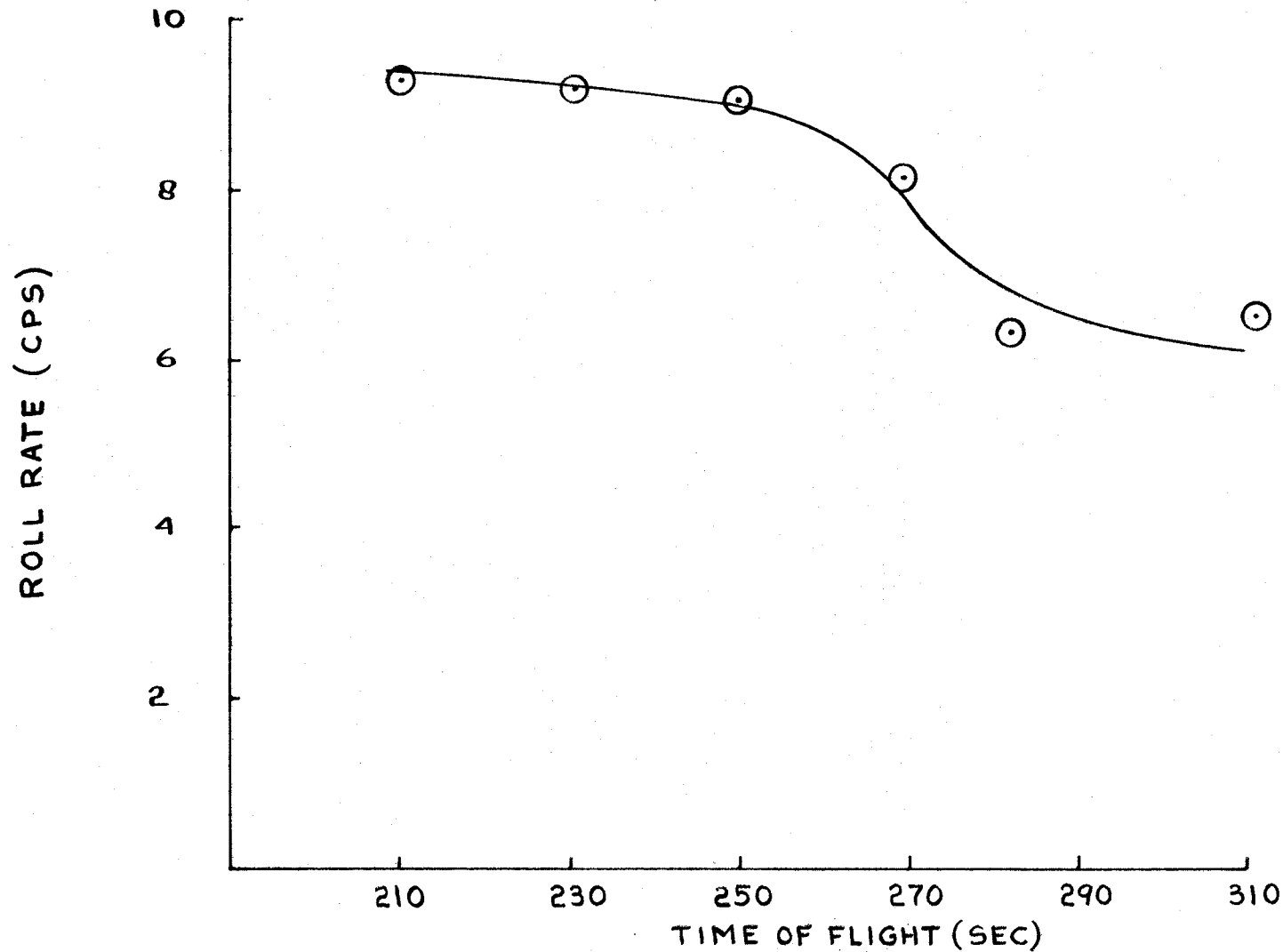
FIG.46 ROLL RATE VS FLIGHT TIME
