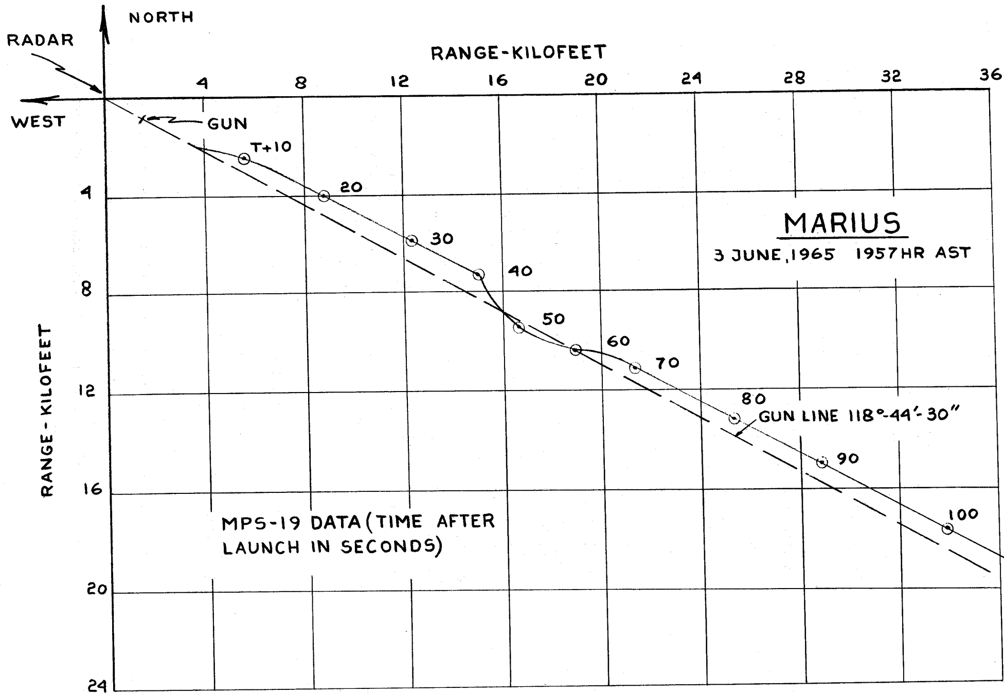
FIG. 8d PLANVIEW OF MARTLET 2C - MARIUS TRAJECTORY
