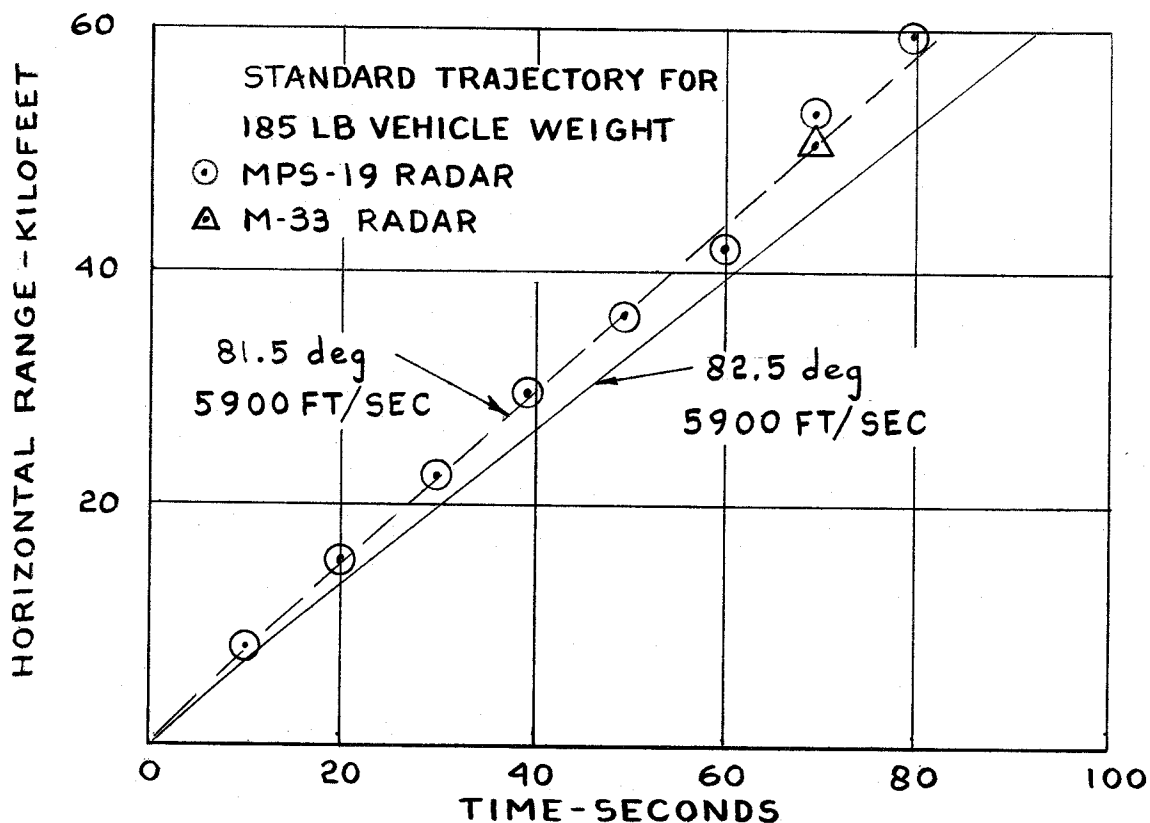
FIG.136 MARTLET 2C SHOT LUCRETIA RANGE VS TIME
