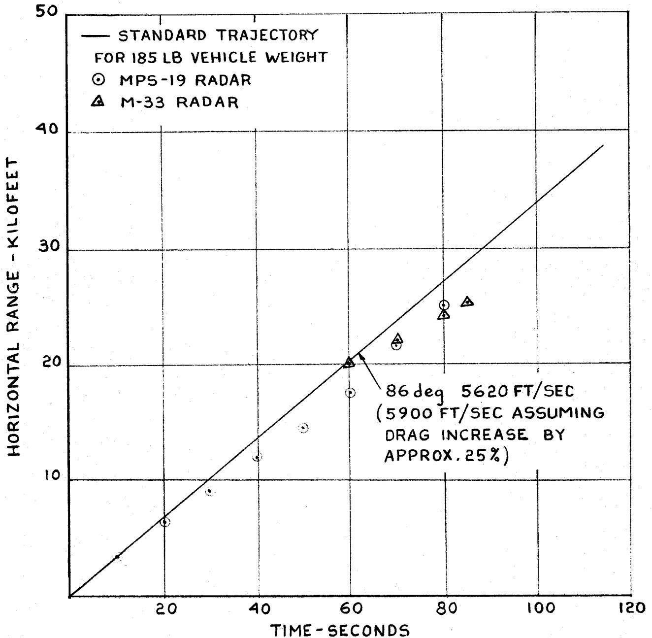
FIG.IIb MARTLET 2C SHOT FABIUS RANGE VS TIME
