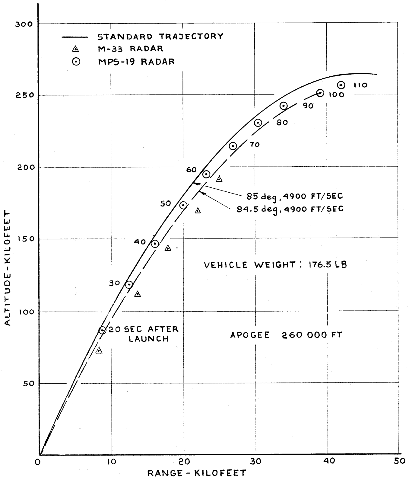
FIG. 4c MARTLET 2A SHOT- RUFUS ALTITUDE VS RANGE
