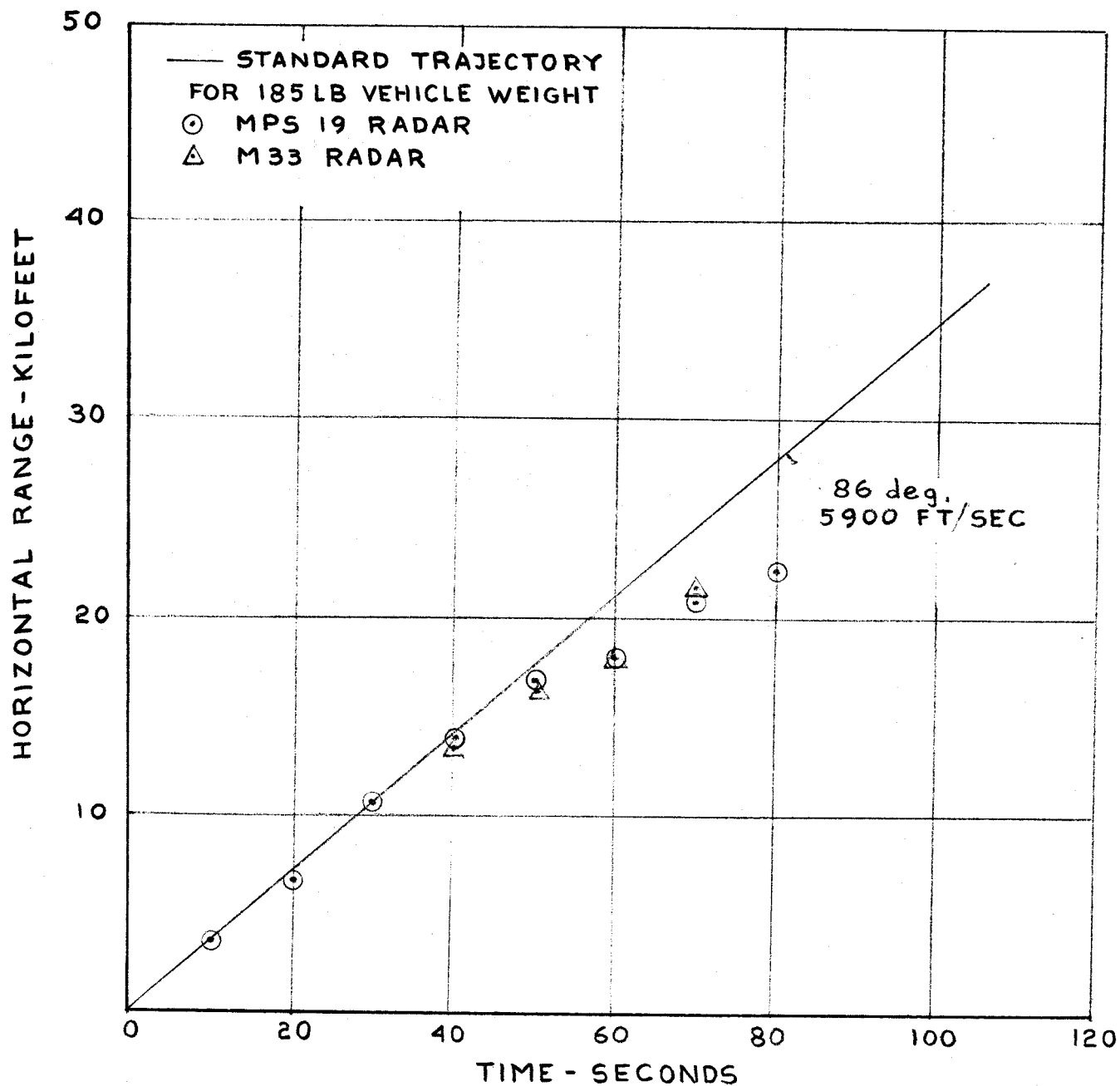
FIG. 10b MARTLET 2C SHOT ELAGABULUS RANGE VS TIME
