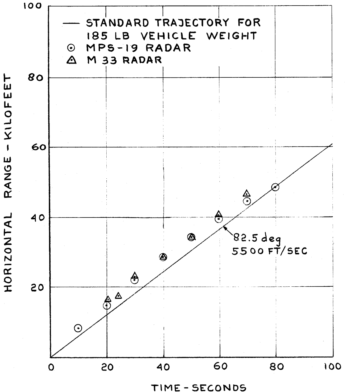
FIG. 146 MARTLET 2C SHOT OVID RANGE VS TIME
