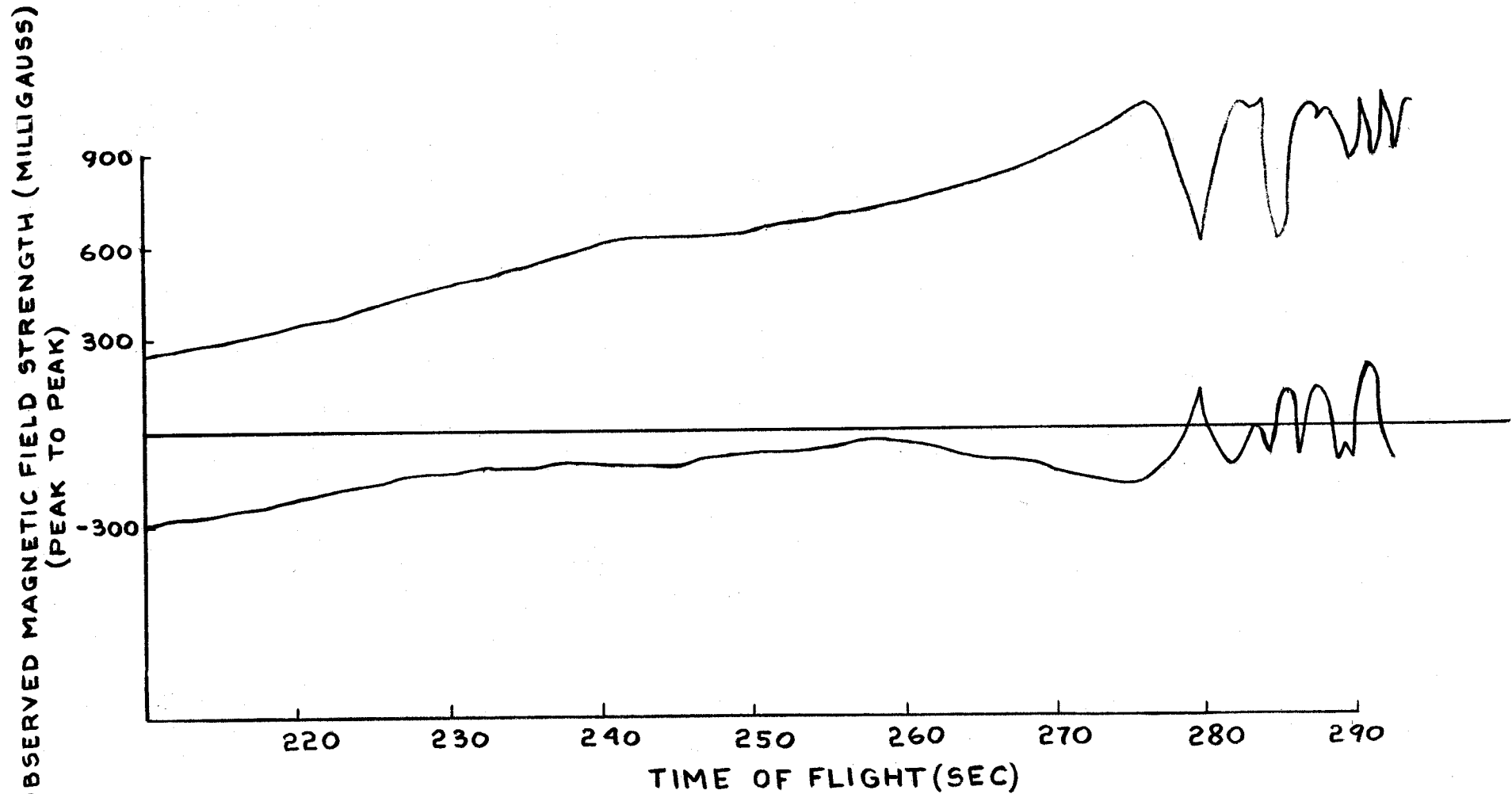
FIG.42 MAGNETIC FIELD STRENGTH VS FLIGHT TIME
