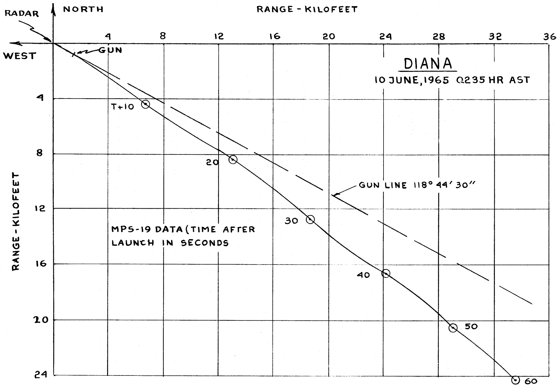
FIG.16d PLAN VIEW OF MARTLET 2C DIANA TRAJECTORY
