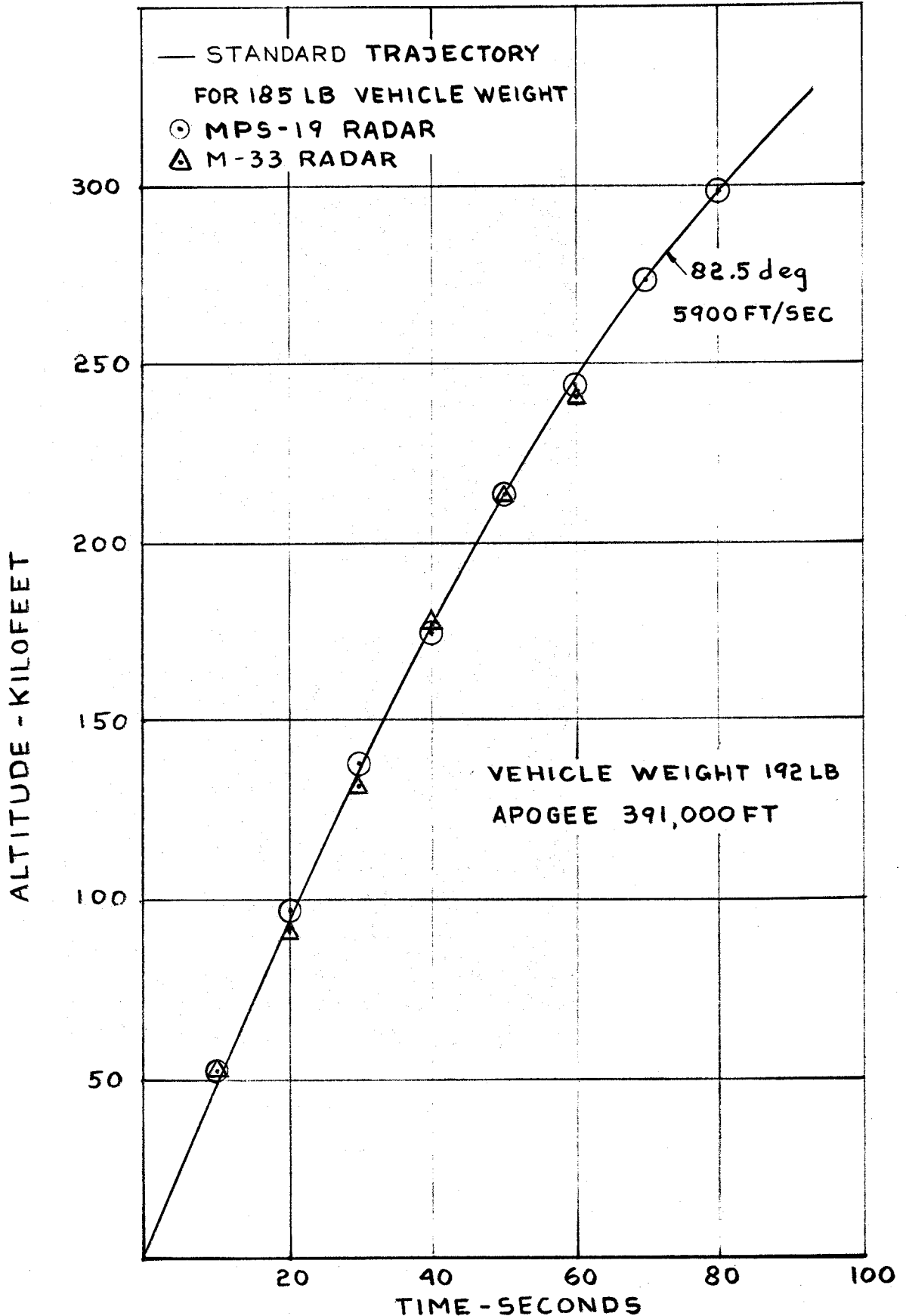
FIG. 22a MARTLET 2C SHOT BRUTUS ALTITUDE VS TIME
