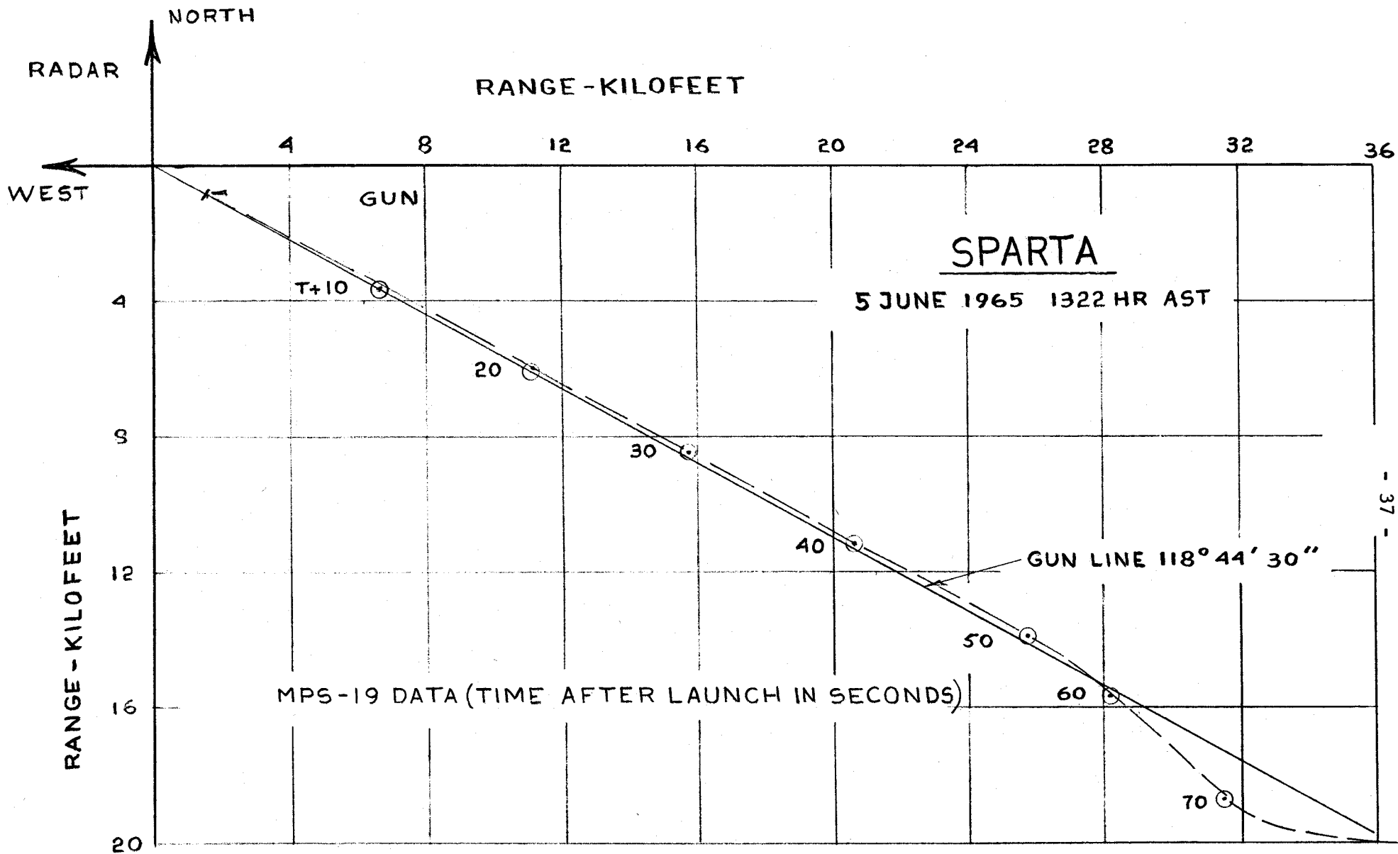
FIG.5d PLAN VIEW OF MARTLET 2A - SPARTA TRAJECTORY
