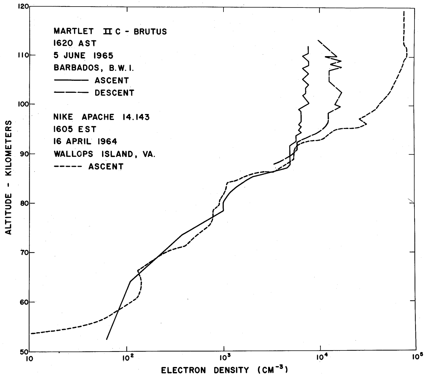
FIG.52 GUN PROBE MEASUREMENTS OF IONOSPHERIC ELECTRON DENSITY
