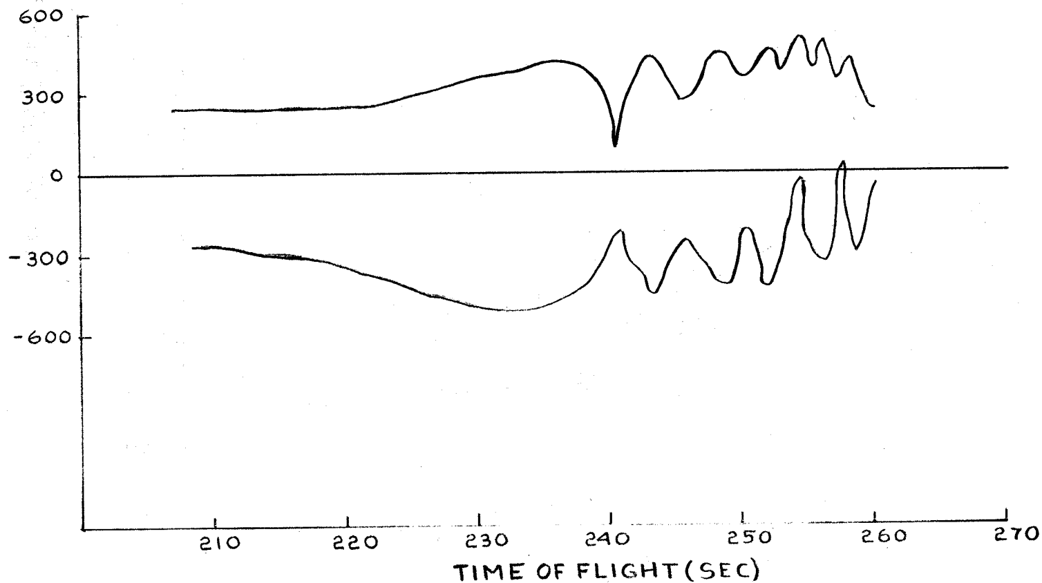
FIG.45 MAGNETIC FIELD STRENGTH VS FLIGHT TIME
