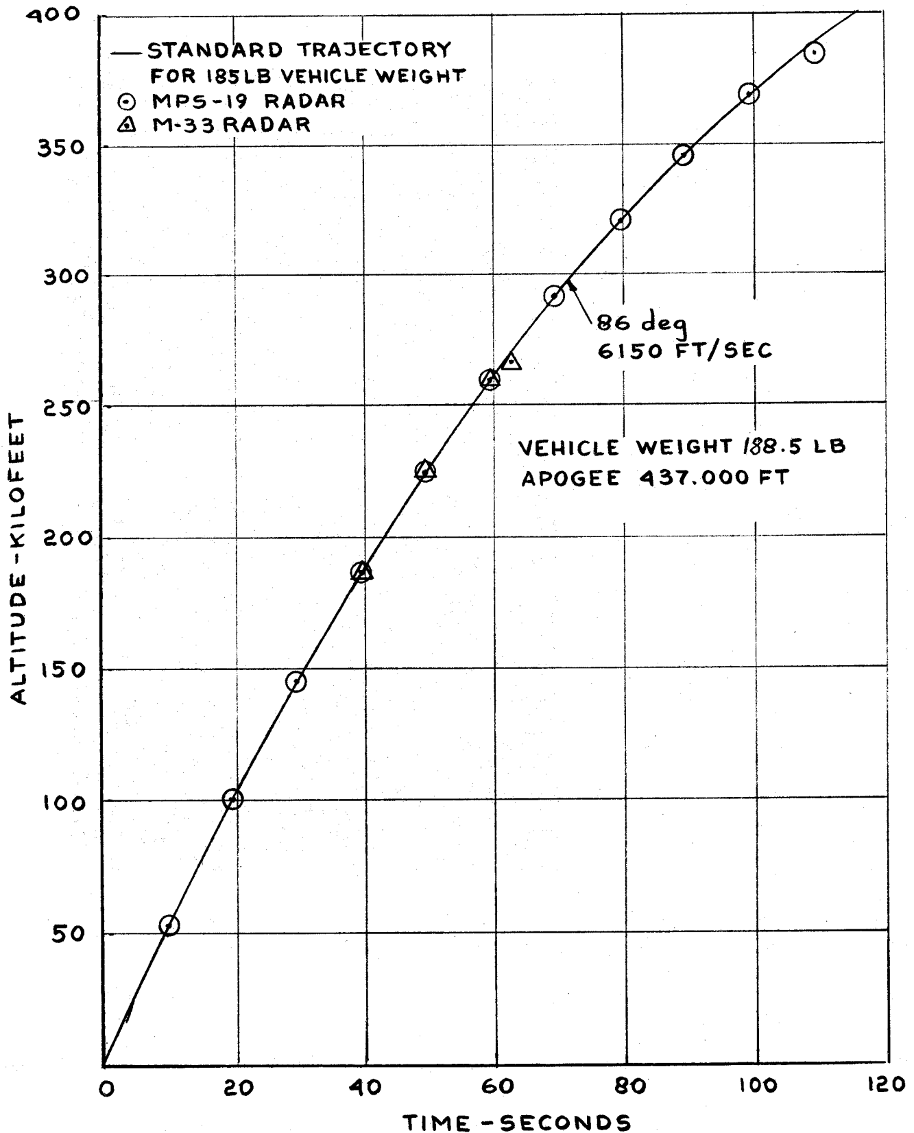
FIG.19a MARTLET 2C SHOT HADRIAN ALTITUDE VS TIME
