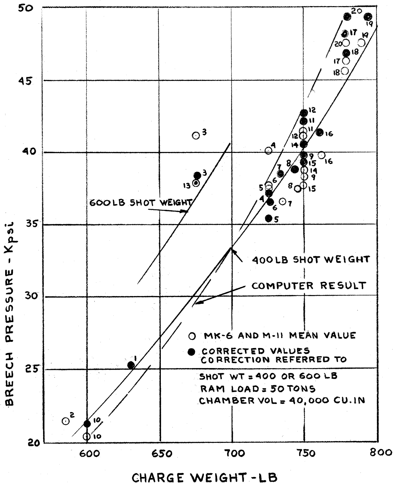
FIG.27 BREECH PRESSURE VS CHARGE WEIGHT
