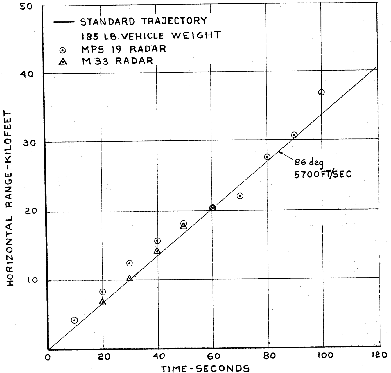
FIG. 8b. MARTLET 2C SHOT MARIUS RANGE VS TIME
