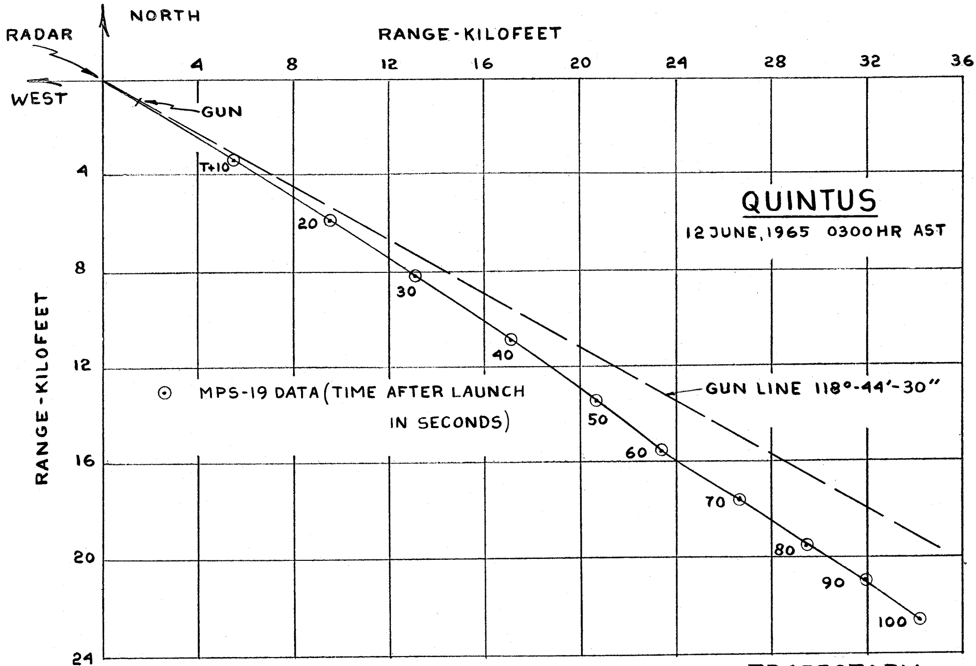
FIG.18d PLAN VIEW OF MARTLET 2C QUINTUS TRAJECTORY
