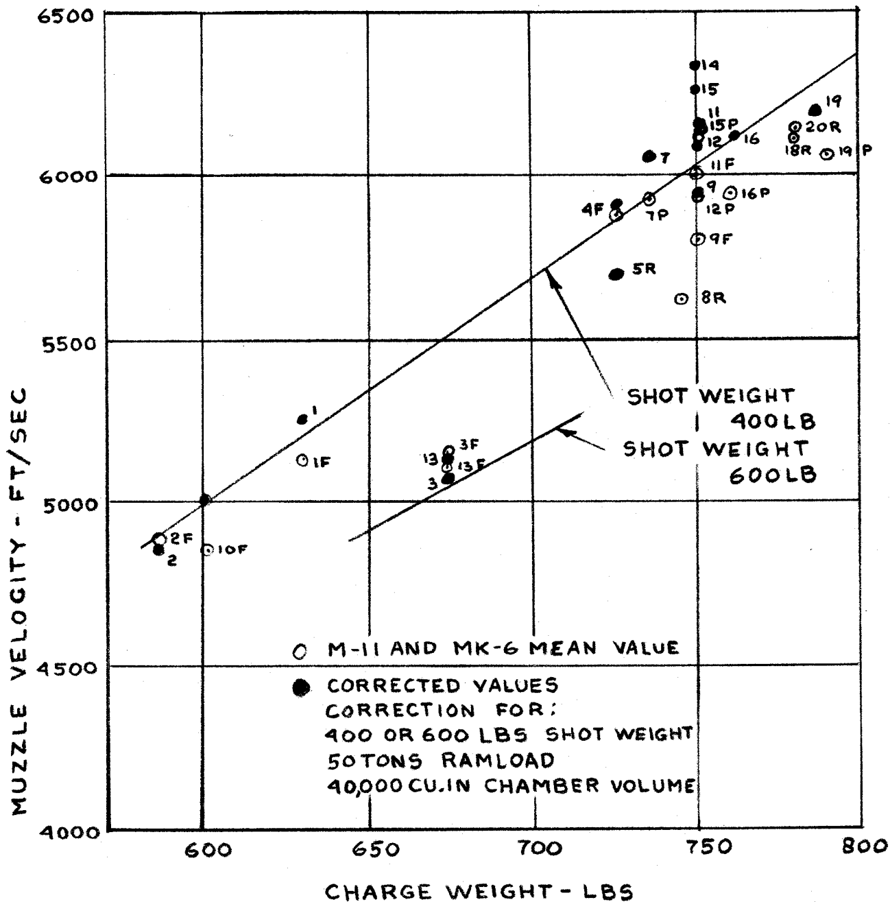
FIG.28 MUZZLE VELOCITY VS CHARGE WEIGHT
