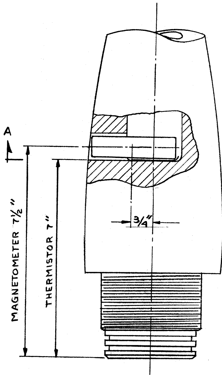
FIG.39 MARTLET 2C MAGNETOMETER AND THERMISTOR LOCATION
