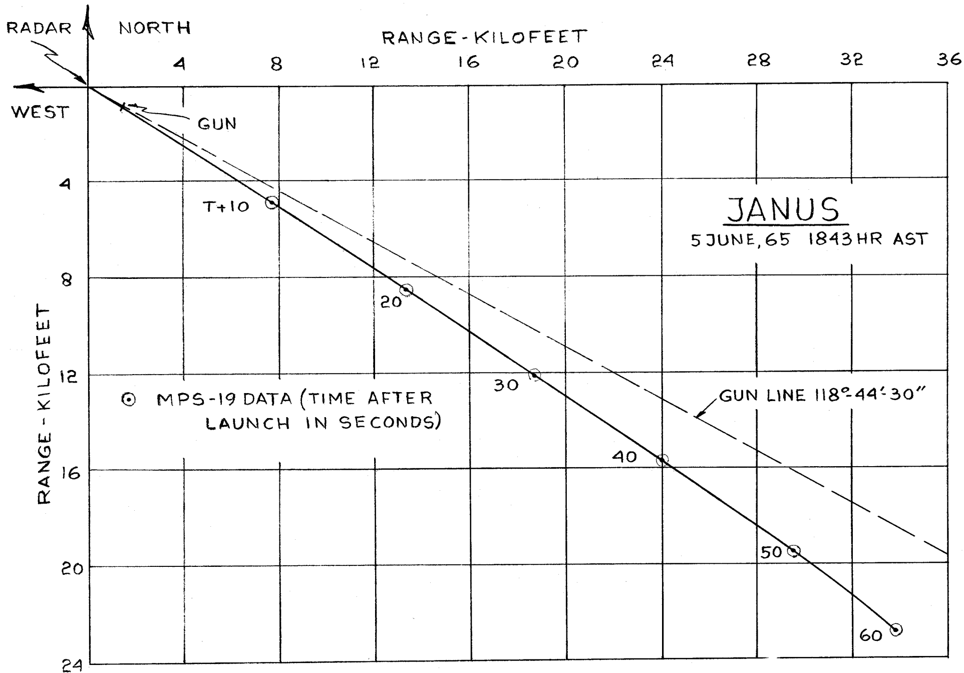
FIG.23d. PLAN VIEW OF MARTLET 2C- JANUS TRAJECTORY
