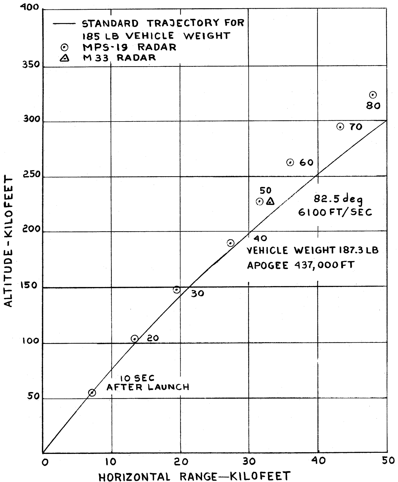
FIG.17c MARTLET 2C SHOT PLINY ALTITUDE VS RANGE
