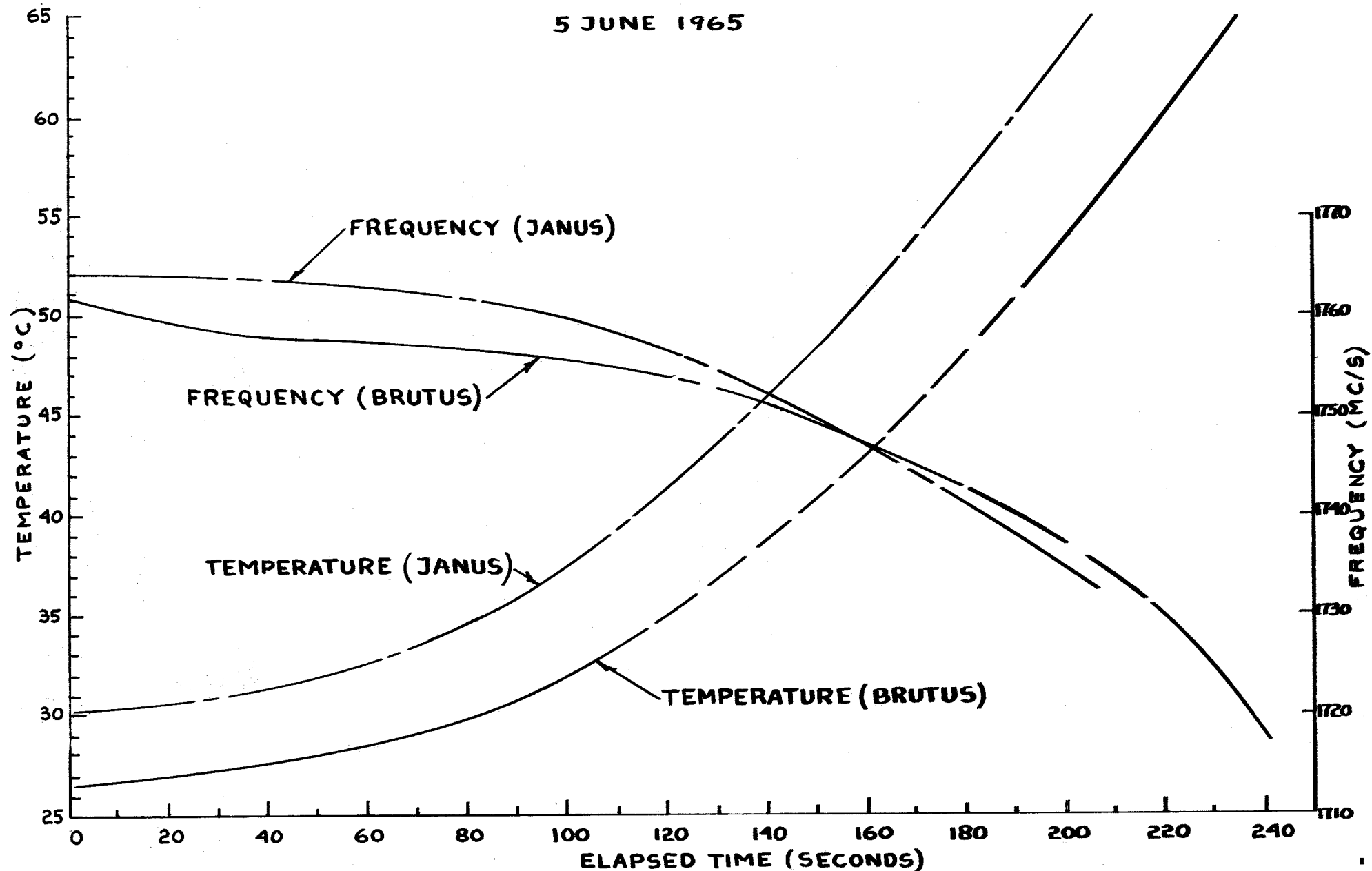
FIG.51 SHOTS BRUTUS AND JANUS, TRANSMITTER FREQUENCY AND TEMPERATURE VS ELAPSED TIME
