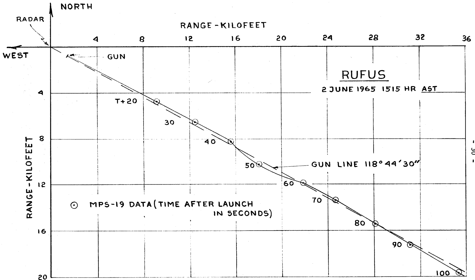
FIG.4d PLAN VIEW OF MARTET 2A -RUFUS TRAJECTORY
