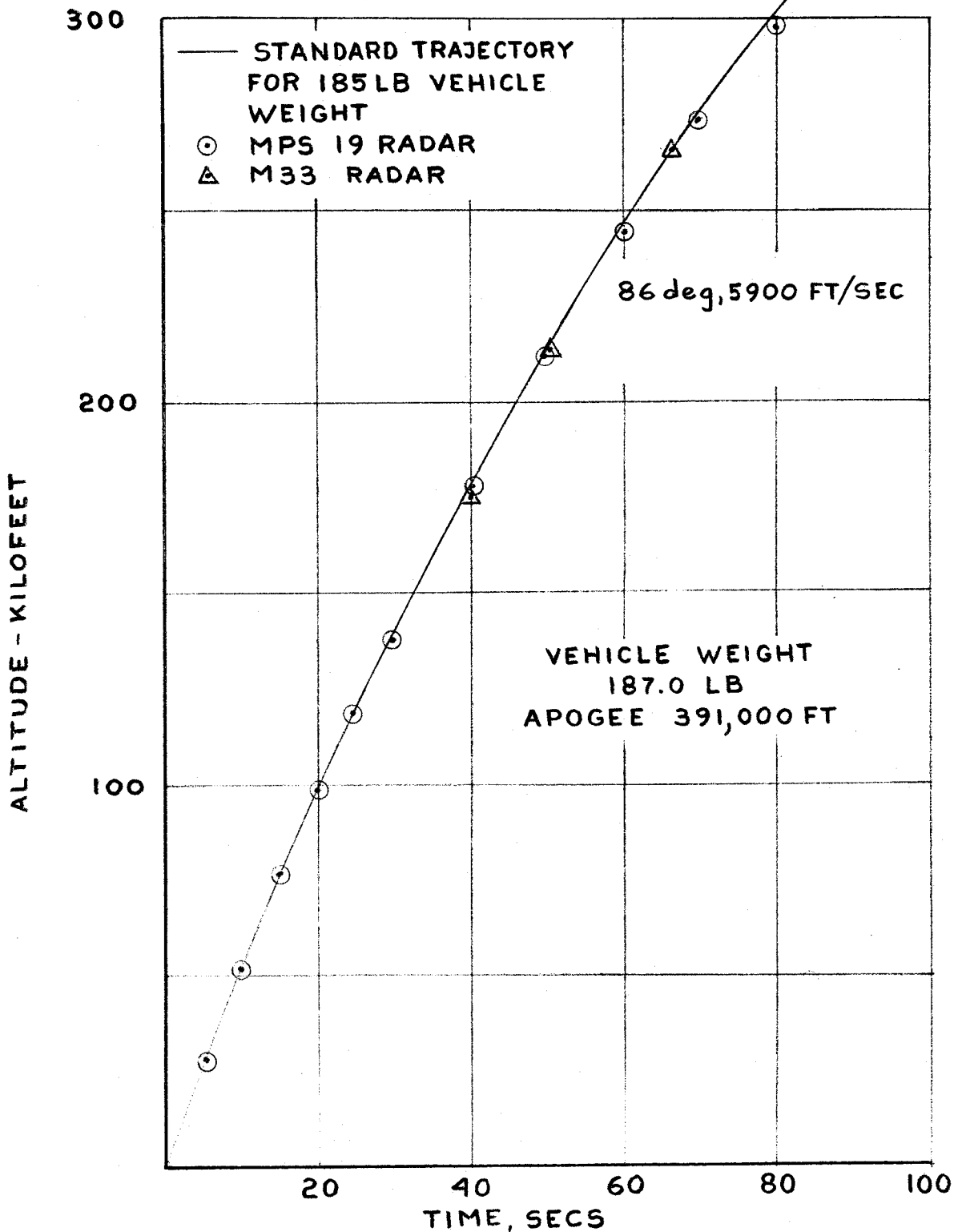
FIG.10a MARTLET 2C SHOT ELAGABULUS ALTITUDE VS TIME
