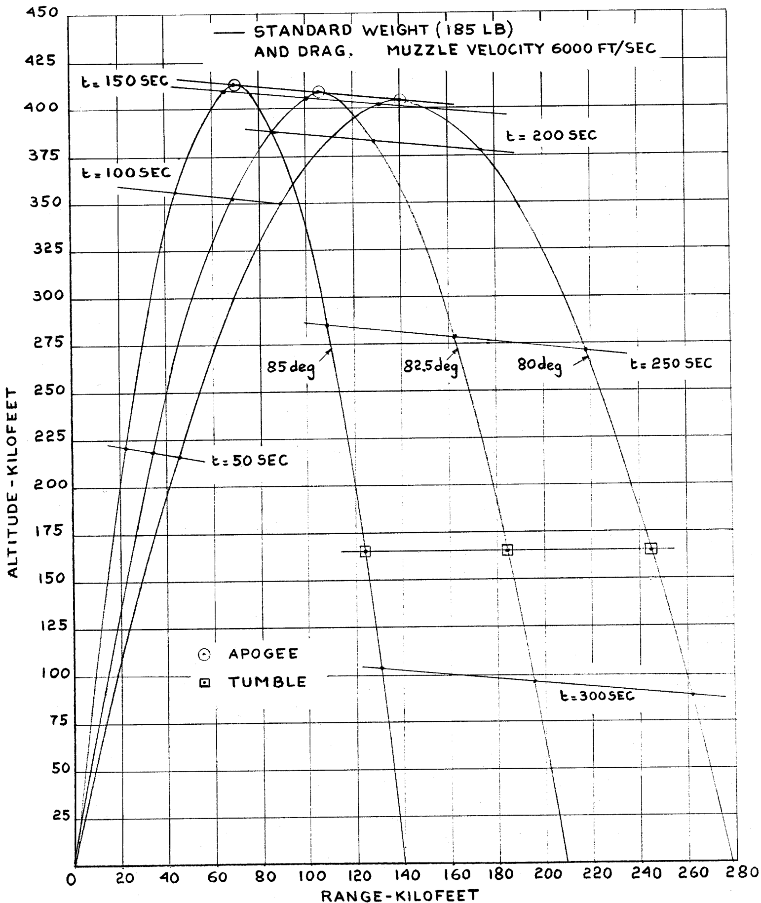
FIG. 7 MARTLET 2C TRAJECTORIES
