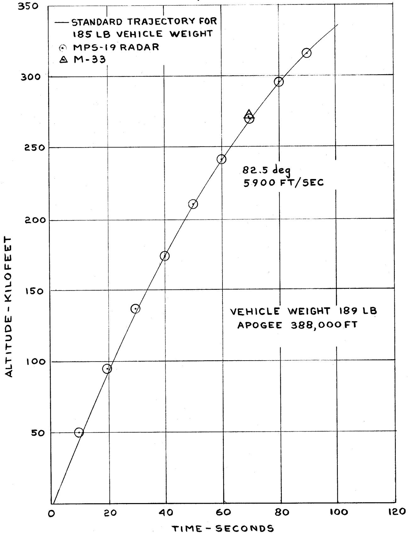
FIG.13a MARTLET 2C SHOT LUCRETIA ALTITUDE VS TIME
