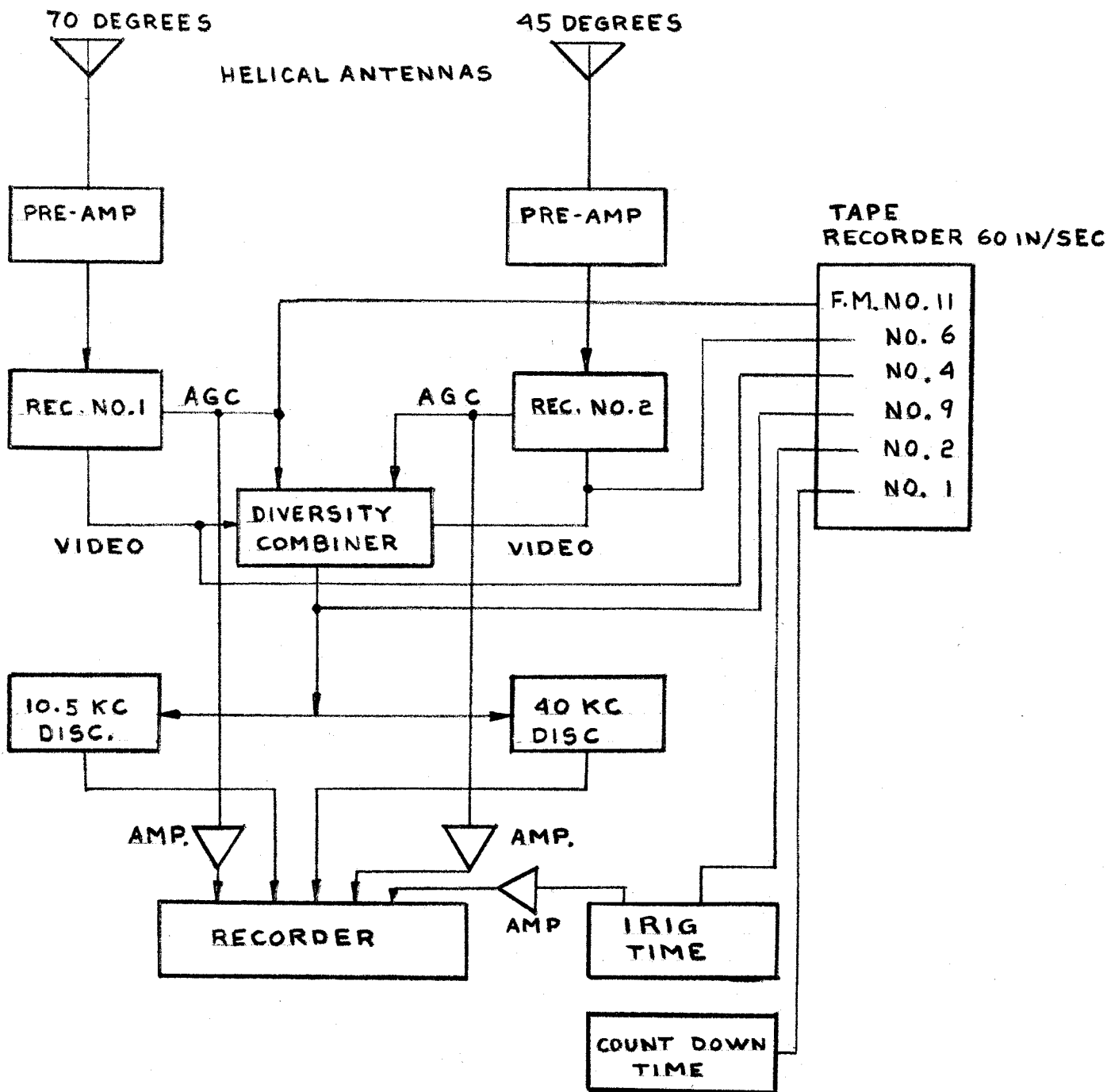
FIG. 41 BLOCK DIAGRAM FOR GROUND STATION TELEMETRY (PARAGON)
