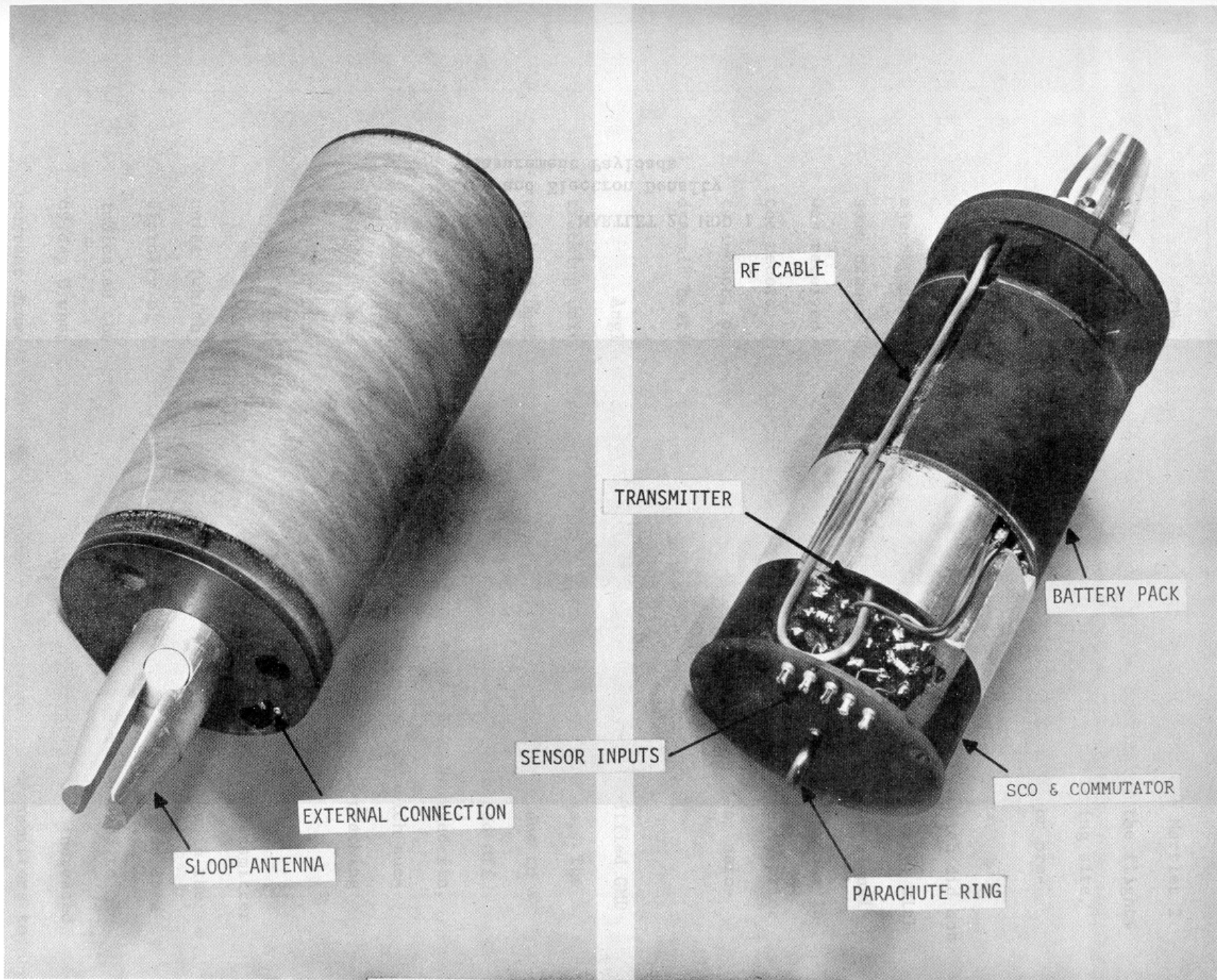
FIGURE 48 EJECTABLE - PARACHUTE PAYLOAD
