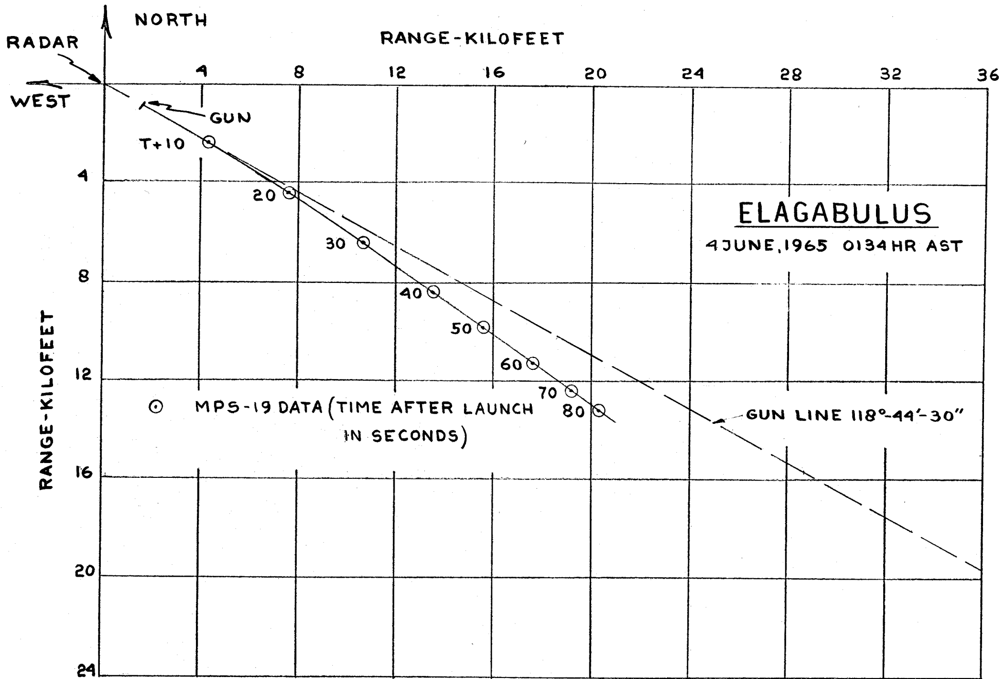
FIG.10d PLAN VIEW OF MARTLET 2C ELAGABULUS TRAJECTORY
