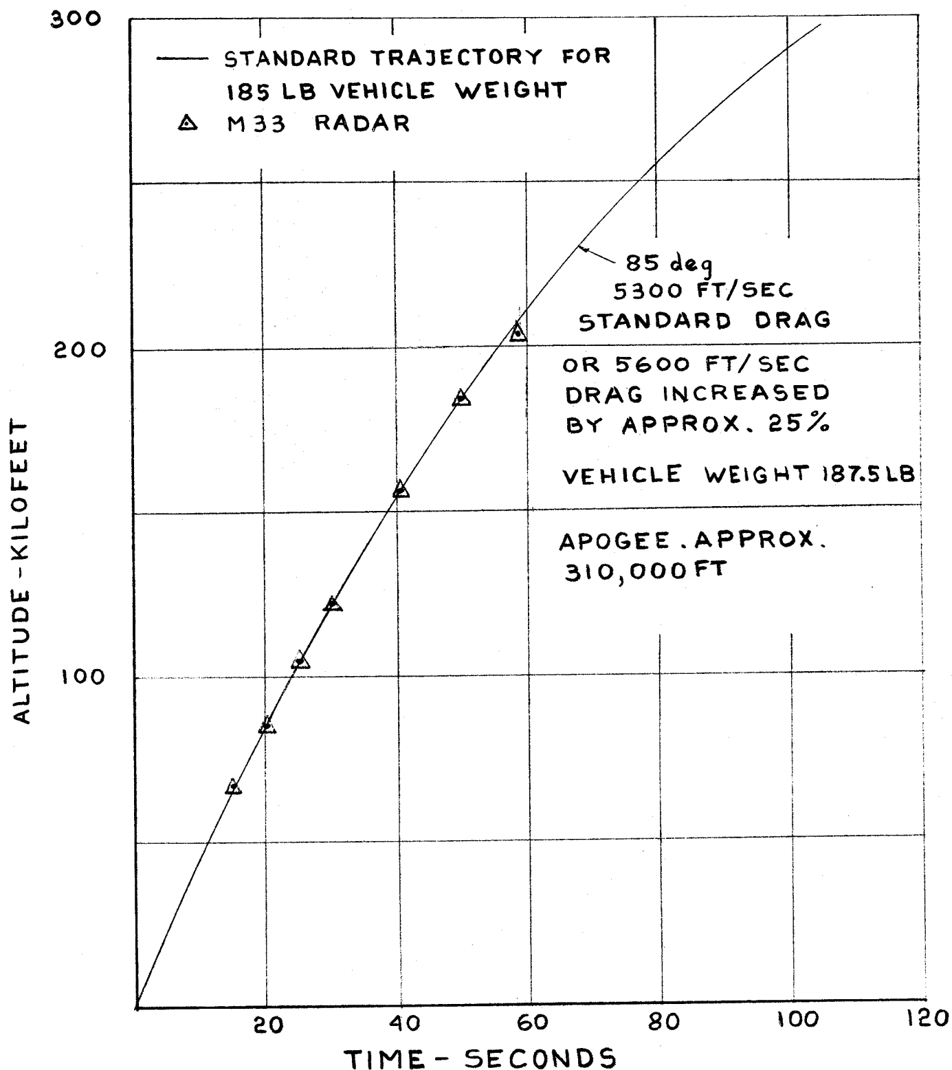
FIG. 9a MARTLET 2C SHOT NERO ALTITUDE VS TIME
