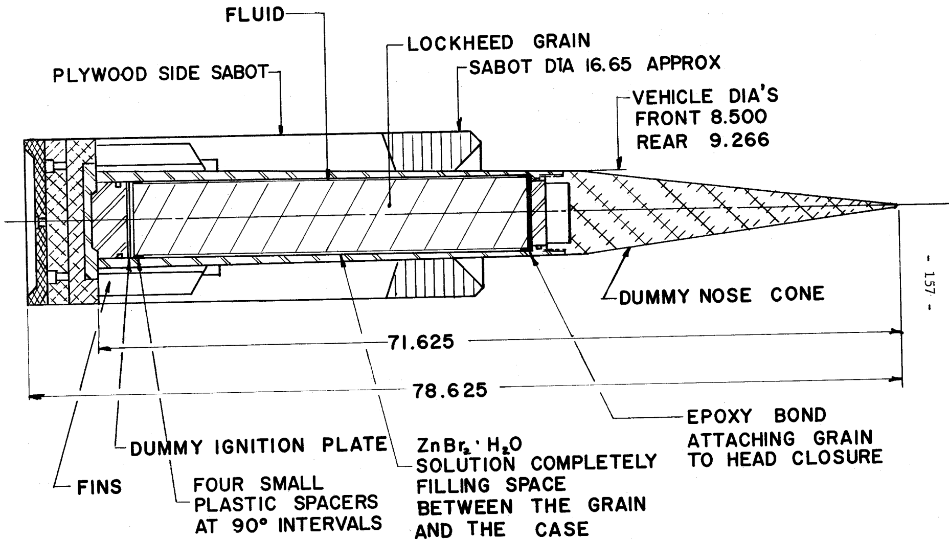
MARTLET 3B - LOCKHEED TEST CONFIGURATION # 2
