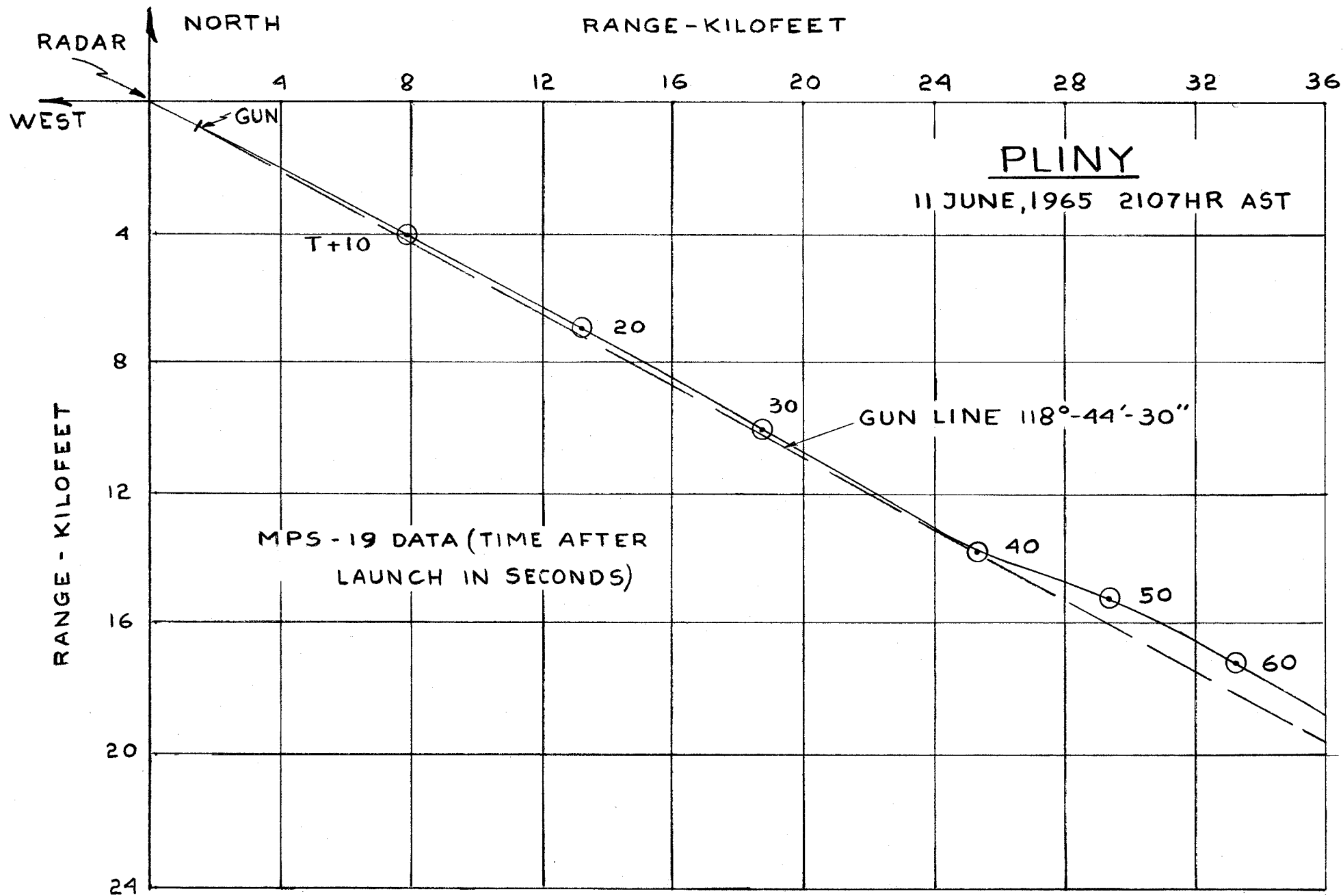
FIG.17d PLAN VIEW OF MARTLET 2C PLINY TRAJECTORY
