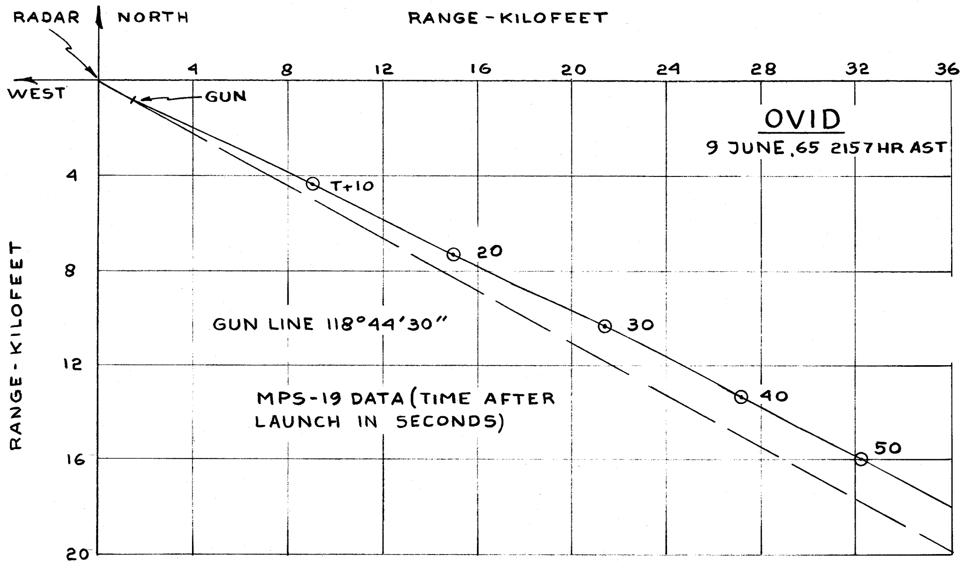
FIG.14d PLAN VIEW OF MARTLET 2C OVID TRAJECTORY
