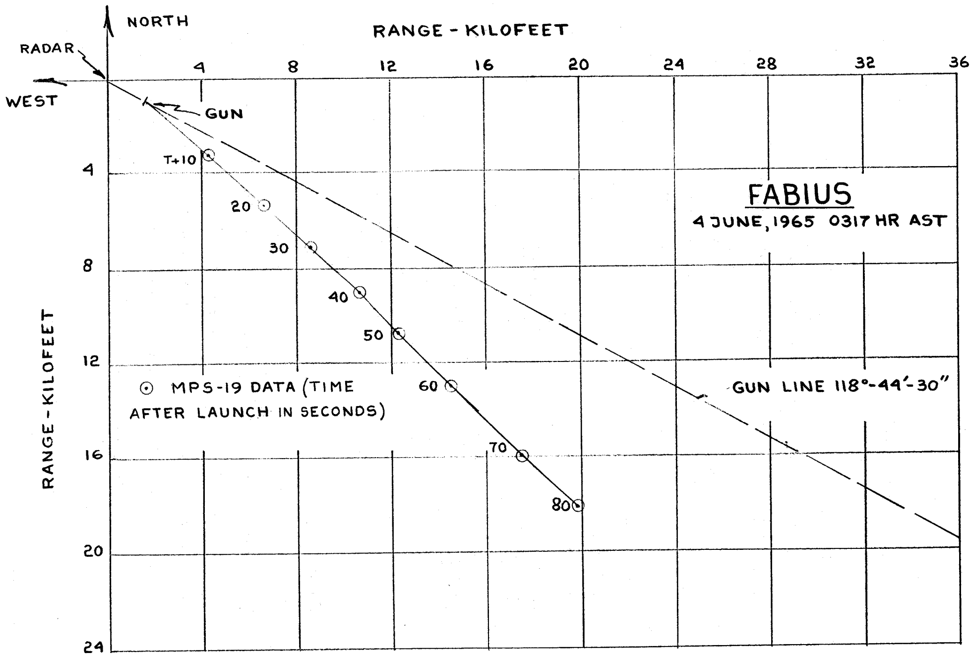
FIG.IId. PLAN VIEW OF MARTLET2C FABIUS TRAJECTORY
