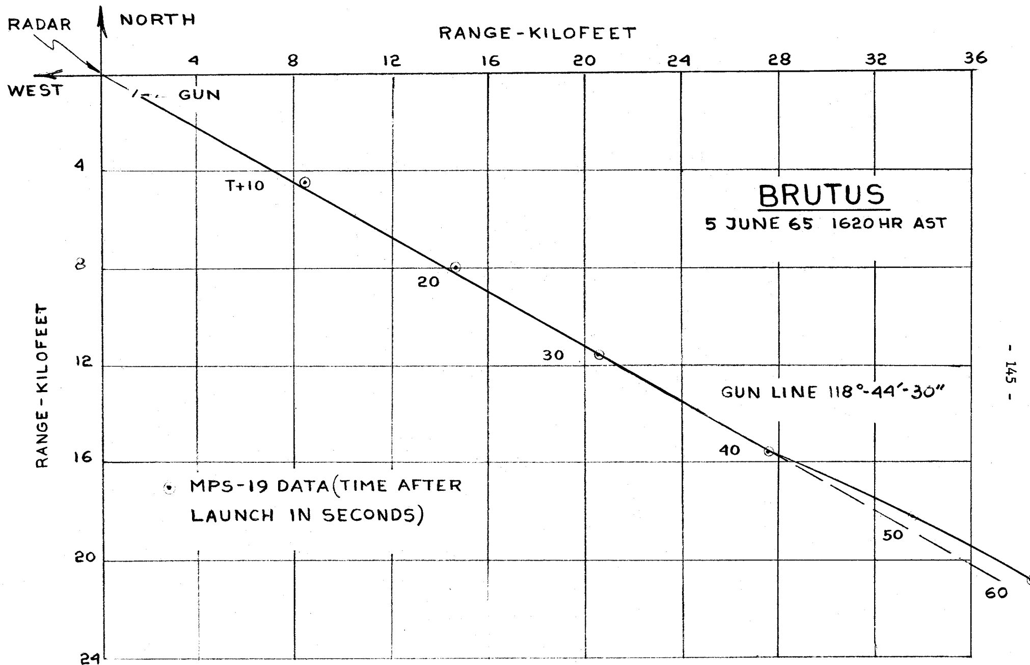
FIG.22d PLAN VIEW OF MARTLET 2C-MODEL BRUTUS TRAJECTORY.
