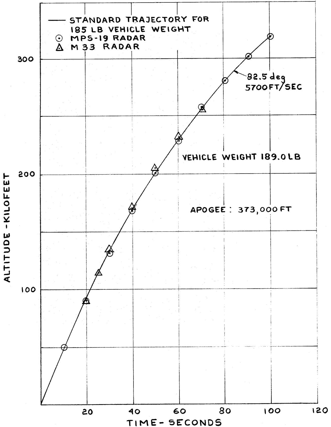
FIG.16a MARTLET 2C SHOT DIANA ALTITUDE VS TIME
