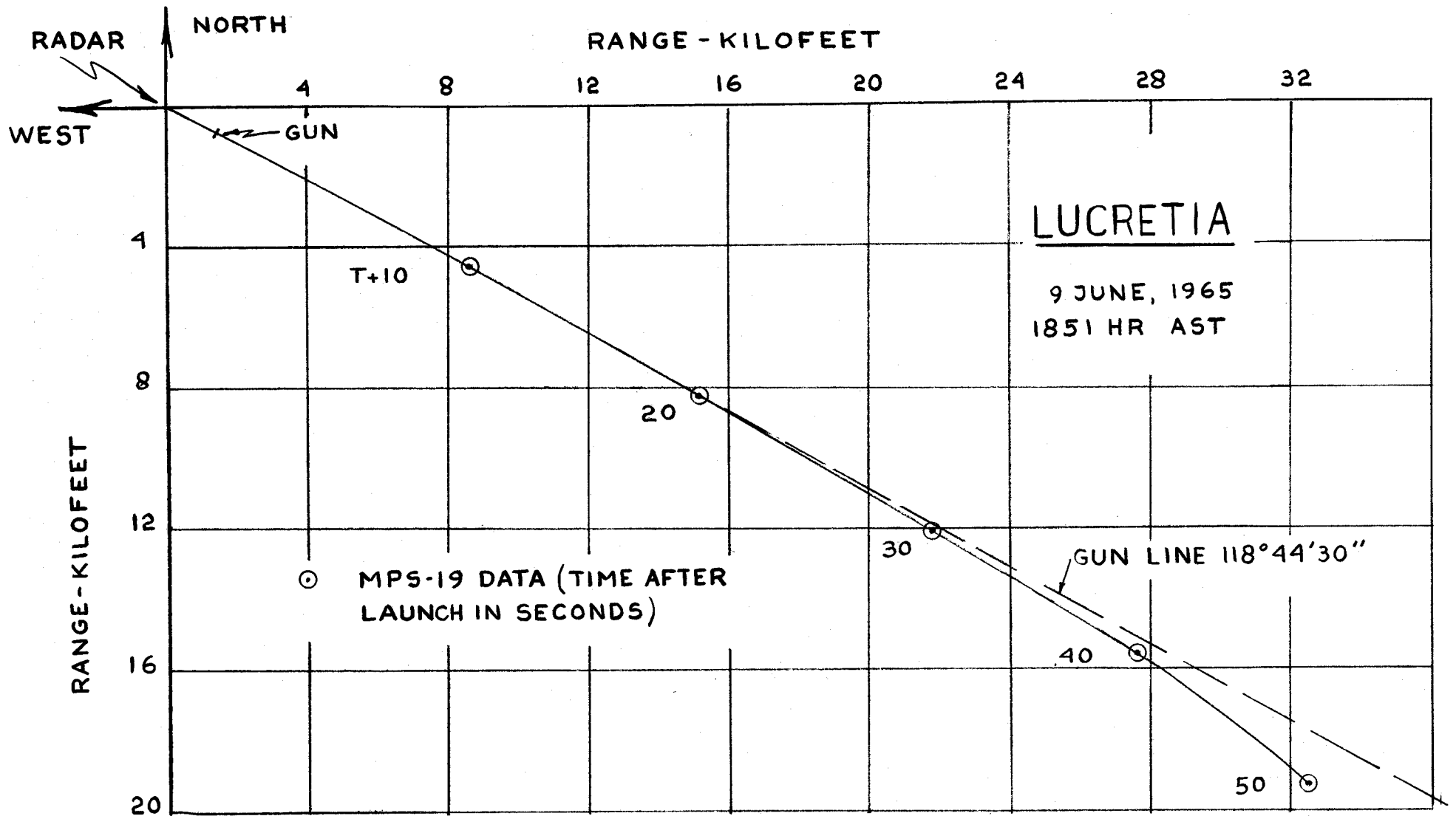
FIG.13d PLAN VIEW OF MARTLET 2C LUCRETIA TRAJECTORY
