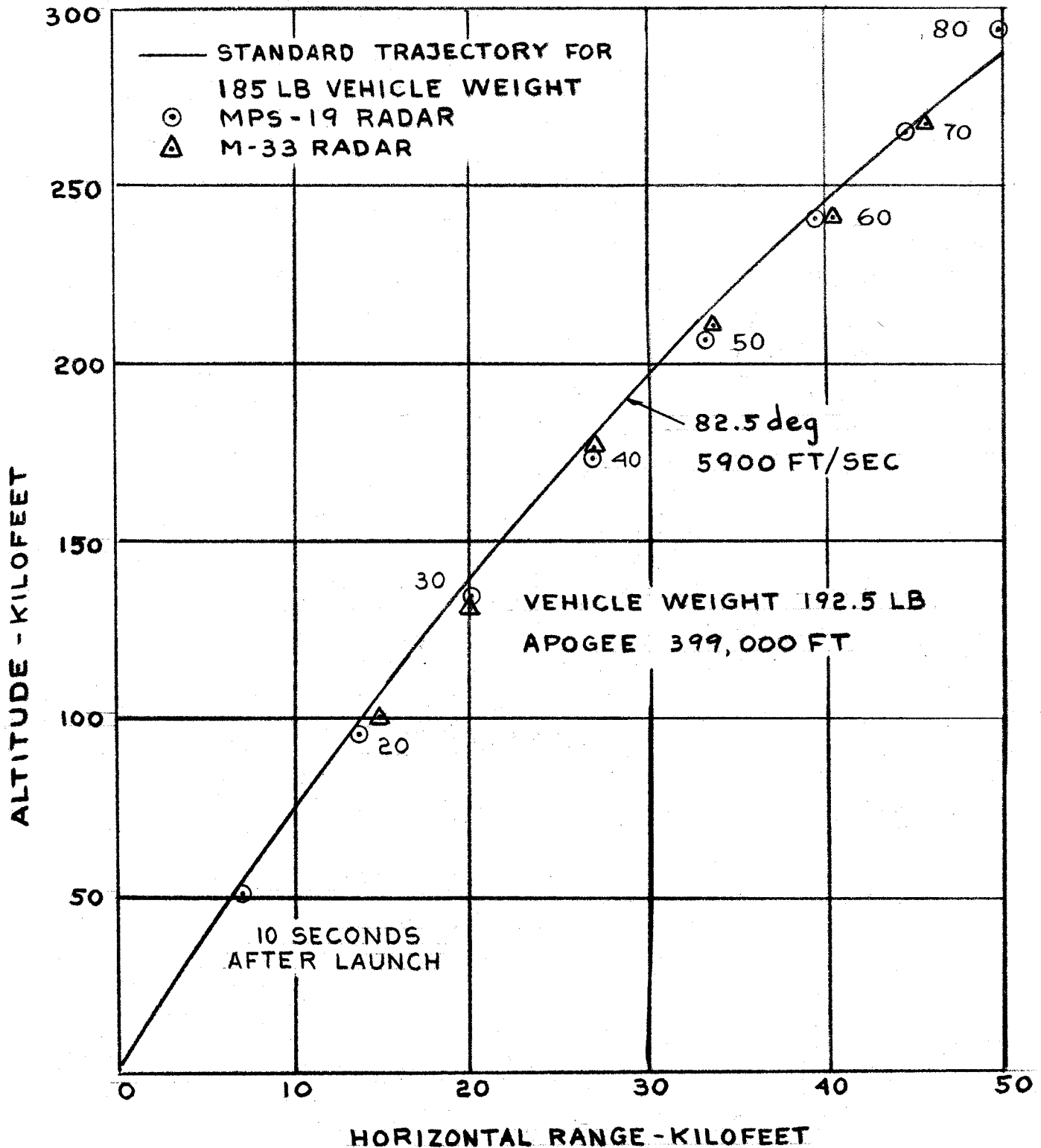
FIG.23c MARTLET 2C SHOT JANUS ALTITUDE VS RANGE
