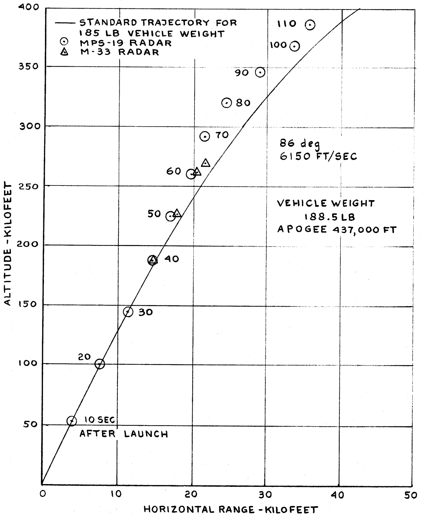
FIG.19c MARTLET 2C SHOT HADRIAN ALTITUDE VS RANGE
