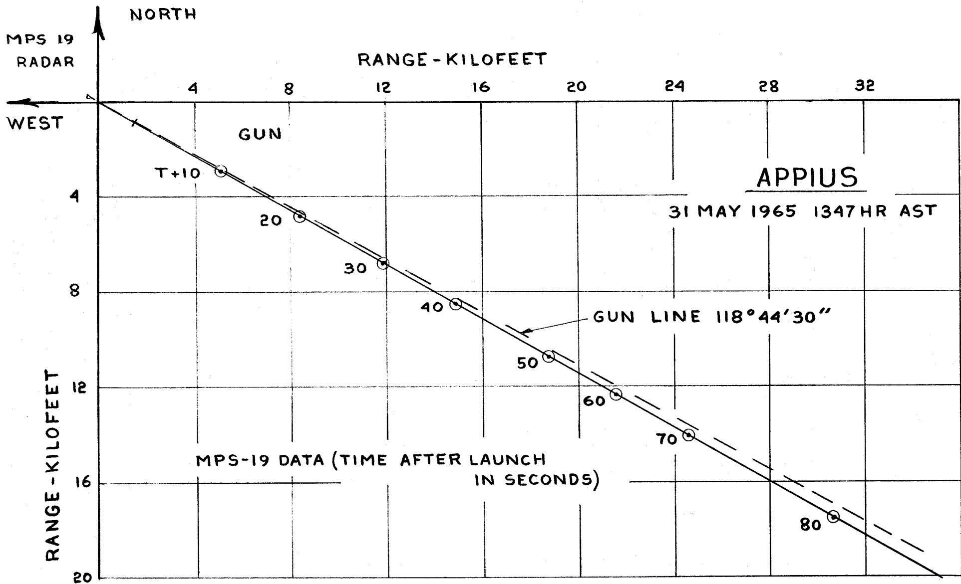
FIG.3d PLAN VIEW OF MARTLET 2A-APPIUS TRAJECTORY
