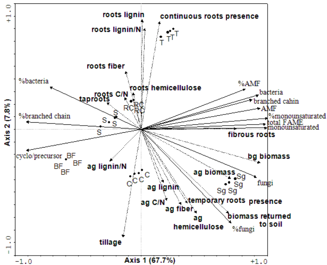
Figure 3.3: Redundancy analysis (RDA) biplot of FAME data for the different cropping systems, using 12 FAME groups as species and 18 explanatory variables. The cropping systems C, Sg, S, RC, T and BF refer to corn, sorghum, soybean, red clover, timothy and bare fallow respectively. ag: above-ground; bg: below-ground.
