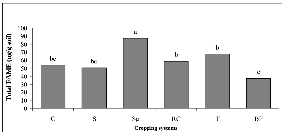
Figure A.2: Total fatty acid methyl ester (FAME) extracted from soil under the different cropping systems after 3 growing seasons. The cropping systems referred to as C, Sg, S, RC, T and BF involve corn, sorghum, soybean, red clover, timothy and bare fallow respectively. FAME values followed by the same letter are not significantly different ( P=0.05 ) according to Bonferroni (n=4).
