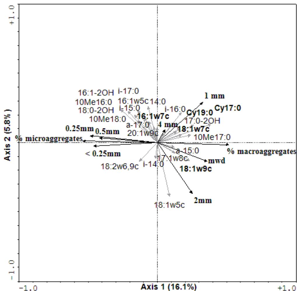
Figure 4.1: Redundancy analysis (RDA) exploring the relationship between FAME profiles and change in soil structure variables from 3 days until 28 weeks after amendments addition to soil. The 29 FAMEs given in Table 4.2 were used as explanatory variables and change in soil structure variables as species variables. Percentages represent the amount of variability explained by the axis.
