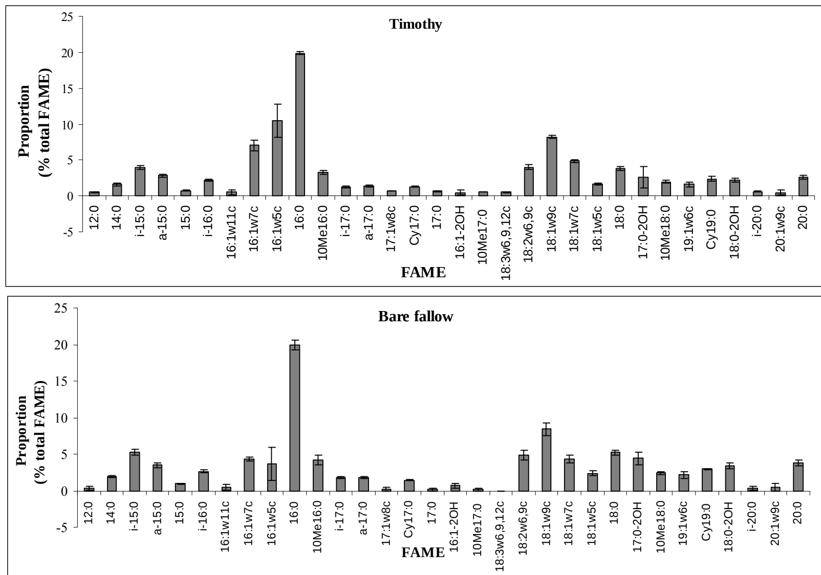
Figure A.3: Fatty acid methyl ester (FAME) profiles under the different cropping systems after three growing seasons. The vertical bars represent 2 x SE mean (n=4).
