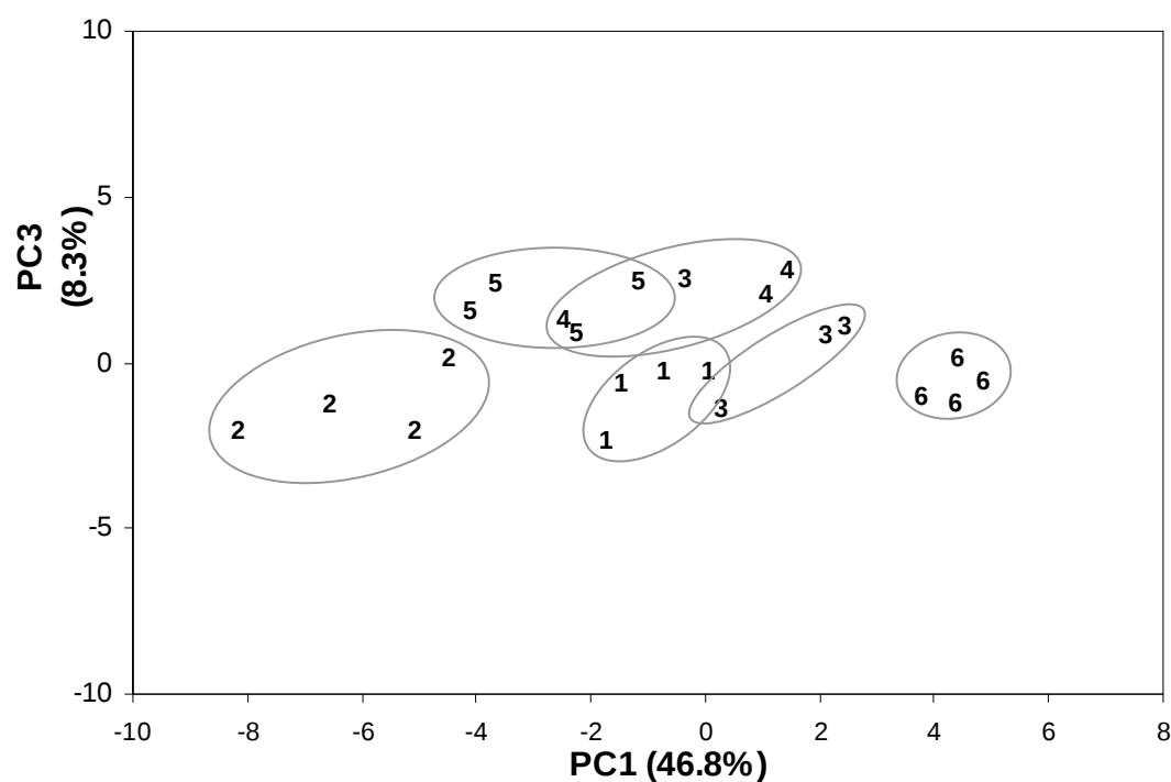
Figure 3.2: Two dimensional plot of the six cropping systems on the first and third principal components (PC1 and PC3) after principal component analysis of their fatty acid profiles. PCA was conducted with 32 fatty acids (percentage of total FAME) that were present in all the samples. 1: corn, 2: sorghum, 3: soybean, 4: red clover, 5: timothy, and 6: bare fallow.
