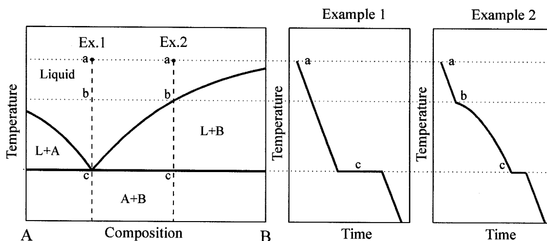
Figure 2-6 - Determination of phase transformations using the cooling curve technique. 6
