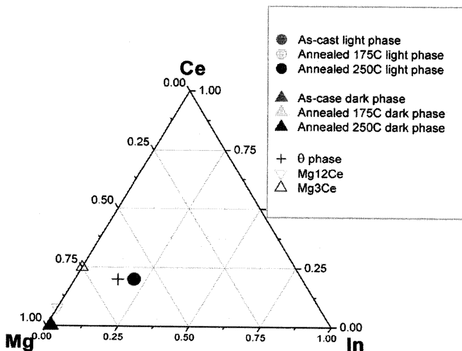
Figure 4-25 - \text{Mg}_{90}\text{Ce}_5\text{In}_5 phase compositions as-cast and annealed
