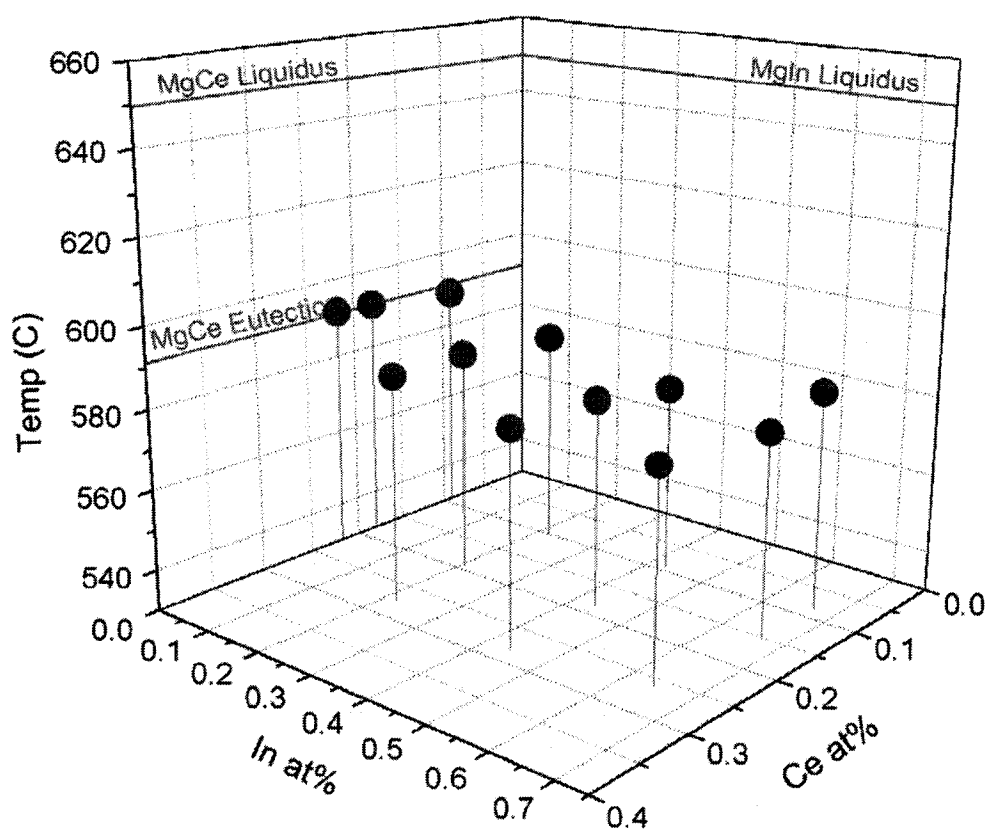
Figure 4-7 – Ternary eutectic values obtained from cooling curve analysis of dilute alloys
