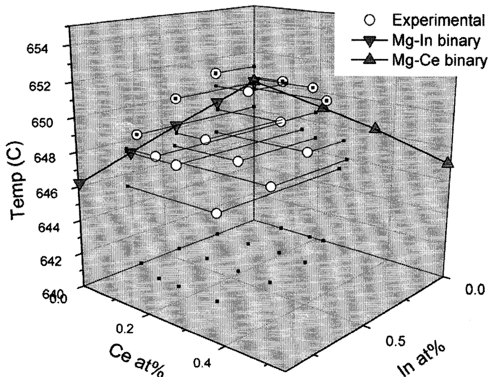
Figure 4-4- Liquidus temperatures vs. element concentration.
