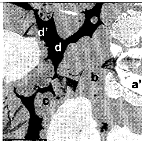
Figure 4-20 - \text{Mg}_{62}\text{Ce}_{21}\text{In}_{17} annealed 175°C microstructure.
