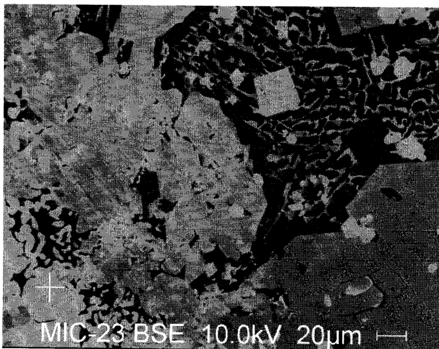
Figure 4-26 - \text{Mg}_{84}\text{Ce}_6\text{In}_{11} alloy microstructure.
