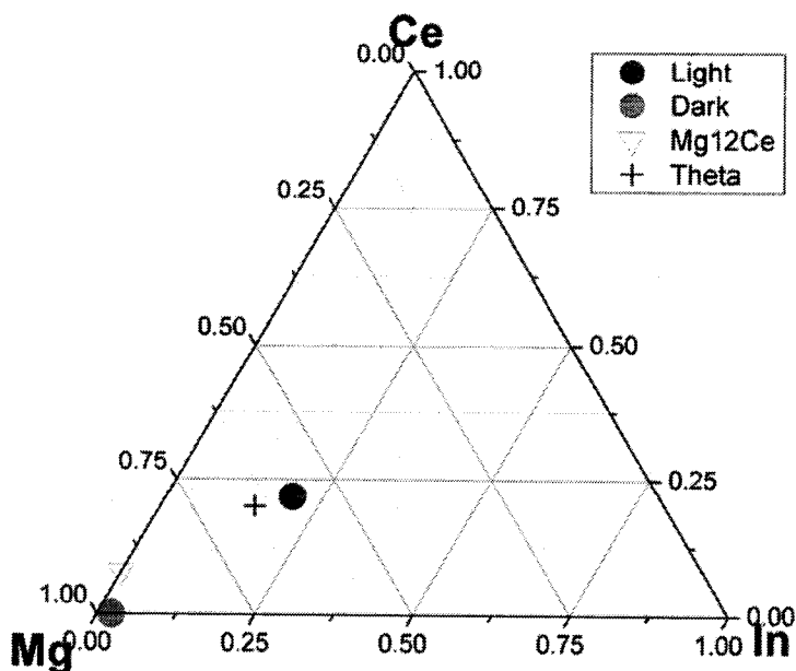
Figure 4-27 - Compositions of some phases in \text{Mg}_{84}\text{Ce}_6\text{In}_{11} .
