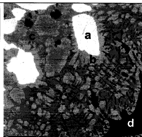
Figure 4-19 - \text{Mg}_{62}\text{Ce}_{21}\text{In}_{17} as-Cast microstructure.
