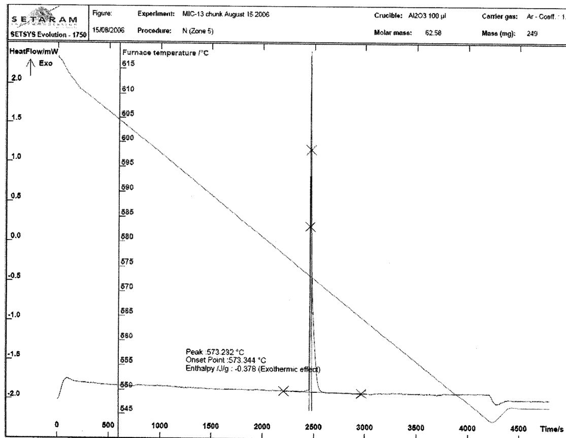
Figure 4-28 - Sample DSC graph from Setaram.
