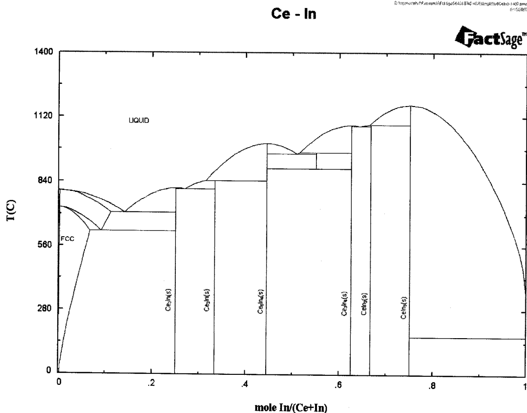
Figure 4-38 - Ce-In binary equilibrium phase diagram generated by FactSage.
