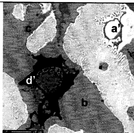
Figure 4-21 - \text{Mg}_{62}\text{Ce}_{21}\text{In}_{17} annealed 250°C
