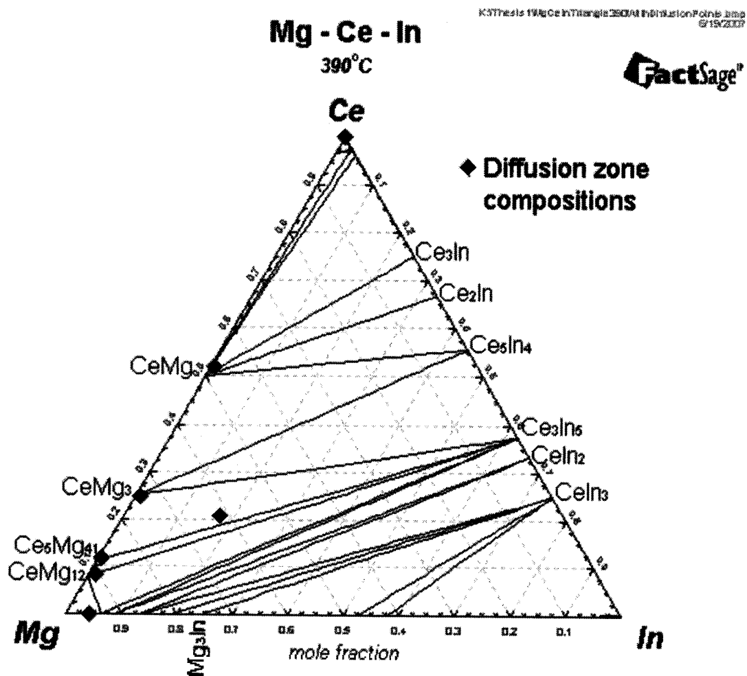
Figure 4-42 - Calculated Mg-Ce-In isotherm at 390°C
