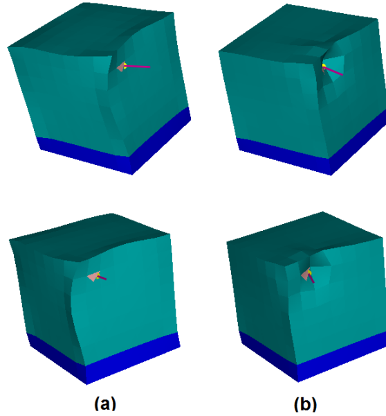
Figure 6–2: Reduced dynamic deformations vs reduced dynamics with statics: The cube model is deformed considering only reduced dynamic deformations (a) whereas the model in (b) also involves the high-frequency static deformations; hence the local deformations in the vicinity of the virtual finger. The pink line segment shows the response force. Note that in both solvers 30 modes out of 1152 modes are picked for computing the low-spatial-frequency dynamics.
