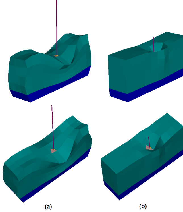
Figure 1–2: Comparison of (a) reduced low-spatial-frequency dynamic deformations, which show the global deformation, and (b) reduced dynamics coupled with high-spatial-frequency statics, which show the local deformations in the vicinity of the virtual finger. The model is fixed at the bottom, and the pink line segment represents the response force. In both solvers, 30 modes out of 660 modes are picked for computing the low-spatial-frequency dynamics.
