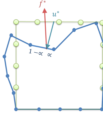
Figure 3–2: Contact at an interpolated point within an edge: The red arrow labeled as f_* represents the response force, and the blue arrow labeled as u_* corresponds to the imposed displacement from the rest pose.
