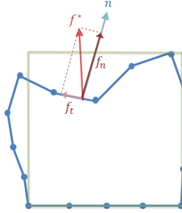
Figure 4–1: A 2D model which is deformed due to a single contact. Note that n shows the surface outward-pointing normal at the point of contact, f_n shows the response force in the normal direction and f_t shows the tangential component of the force.
