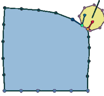
Figure 3–5: Shared point of contact: A node (the orange one) is involved in two contacts introducing an LLS problem. The blue and red line segments represent the computed contact forces and the black line segment which starts from the centre of the virtual stylus shows the total force response.
