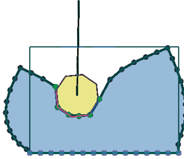
Figure 3–3: Types of multi-point contact: The object is deformed from its rest configuration using a virtual stylus (the octagon). The pink edges of the rigid stylus and the green nodes of the object show two types of contacts.
