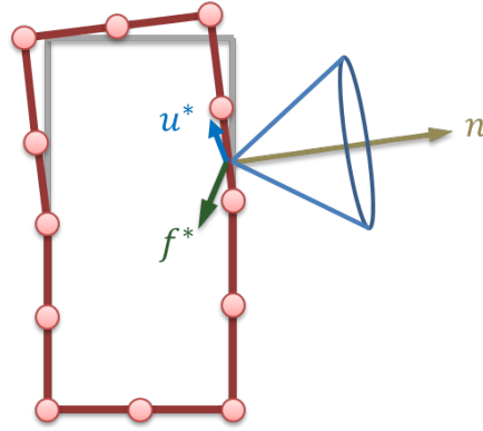
Figure 4–2: A 2D model is deformed due to a single contact. Note that n defines the surface outward-pointing normal at the point of contact. Sliding iteratively modifies the position of this point to decrease the ratio of the magnitude of the tangential force to the magnitude of the normal force, so that f^* falls inside the friction cone.
