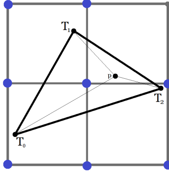
Figure 5–3: Collision with an embedded object: A mesh triangle is embedded in a 2D element grid, where each vertex lies in a different element. Note that although the contact point p lies in the upper right element, the corresponding nodes in the coarser grid are the other three elements' nodes (shown in blue).
