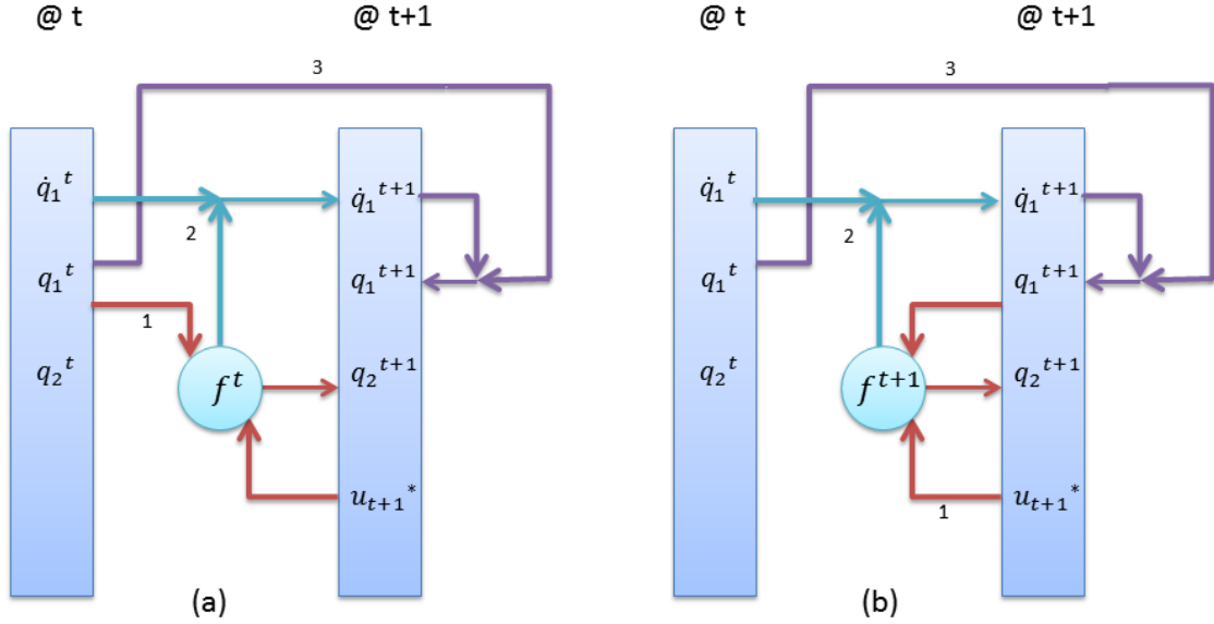
Figure 3–6: Our stepping methods for statics and dynamics coupling: Diagram (a) indicates the symplectic Euler integration (Section 3.3.1) and diagram (b) indicates the backward Euler integration (Section 3.3.2). The blue bars indicate the state of the system at each time-step. Step 1 (red) illustrates the evaluation of the response force along with the high-spatial-frequency static deformations. Steps 2 (blue) and 3 (purple) show the integration of the low-spatial-frequency dynamics.
