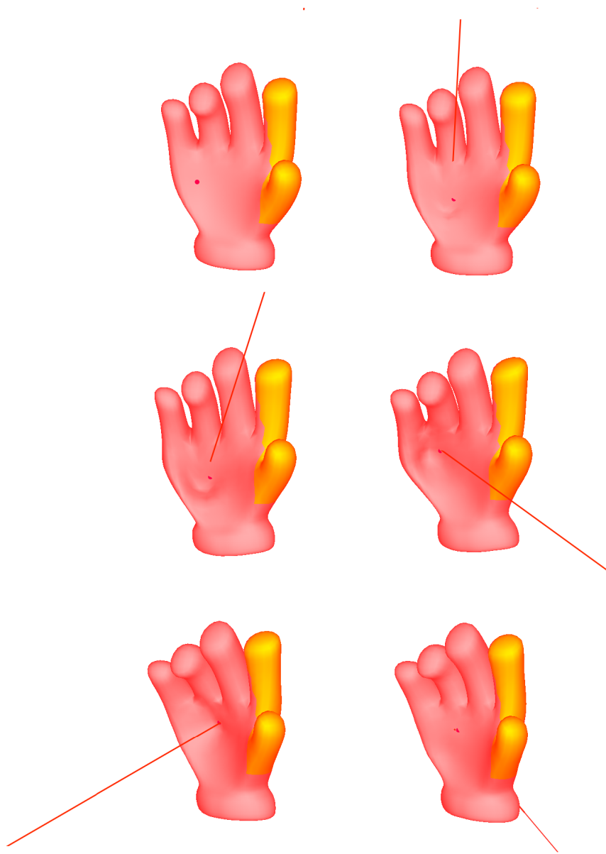
Figure 6–3: Simulation snapshots of the coupled deformations: The hand model is deformed by the user interaction. The user comes into contact with the model, imposes some deformations, and lets go of the model (last snapshot). The orange region of the mesh contains the fixed nodes. The red dot shows the position of the virtual stylus and the line segment represents the response force. In the coupling solution 15 low-spatial-frequency modes out of 1368 modes are selected for the dynamics and the remaining modes are left for constructing the high-resolution-static basis.
