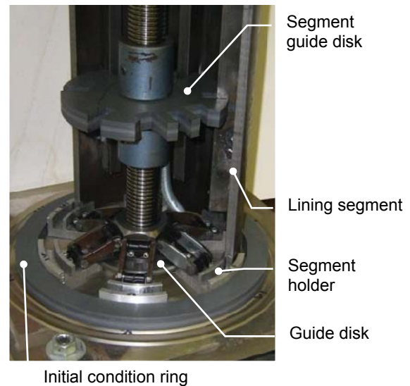
Figure 2. Details of the mechanical adjustable system
