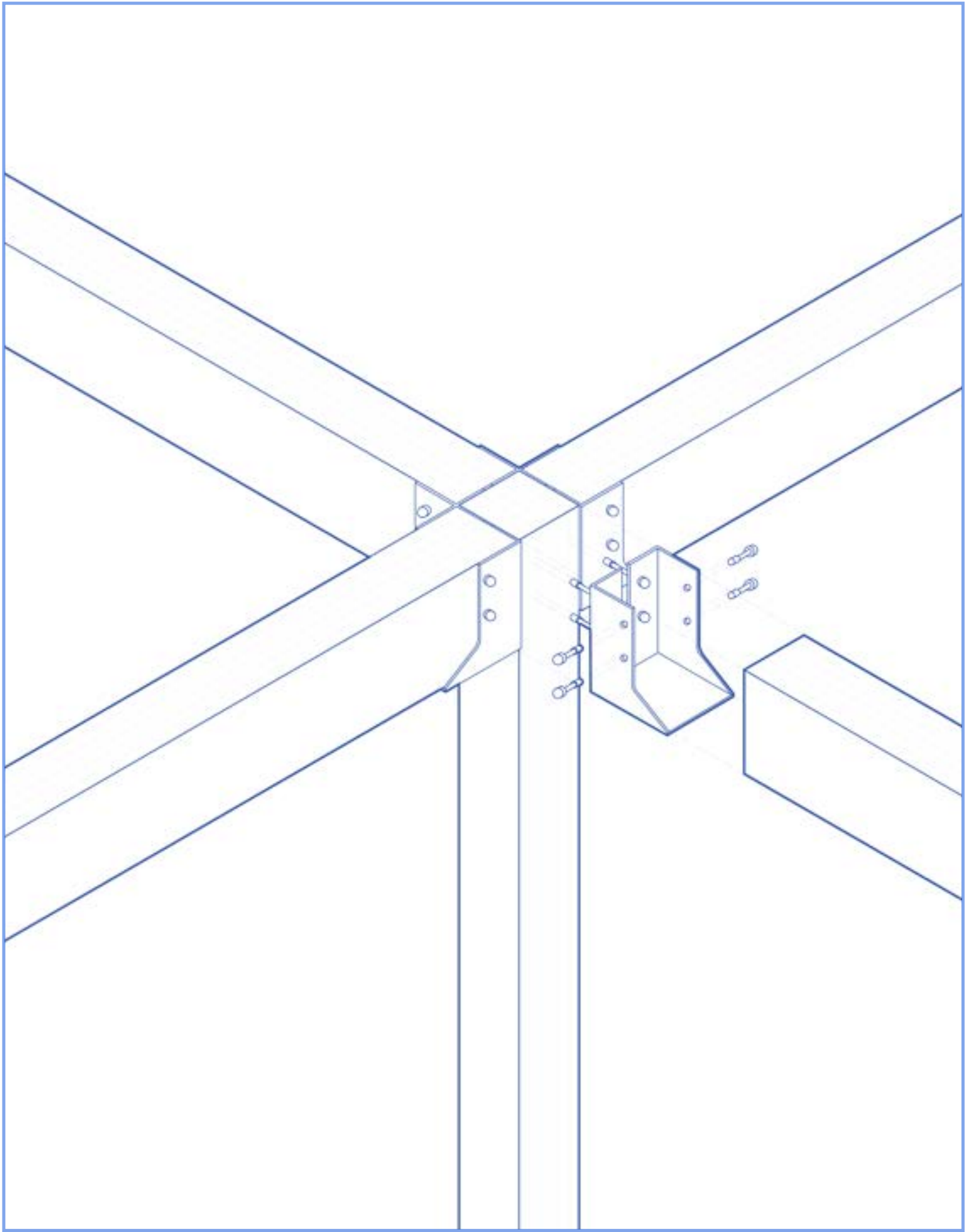
structural detail 1:20
