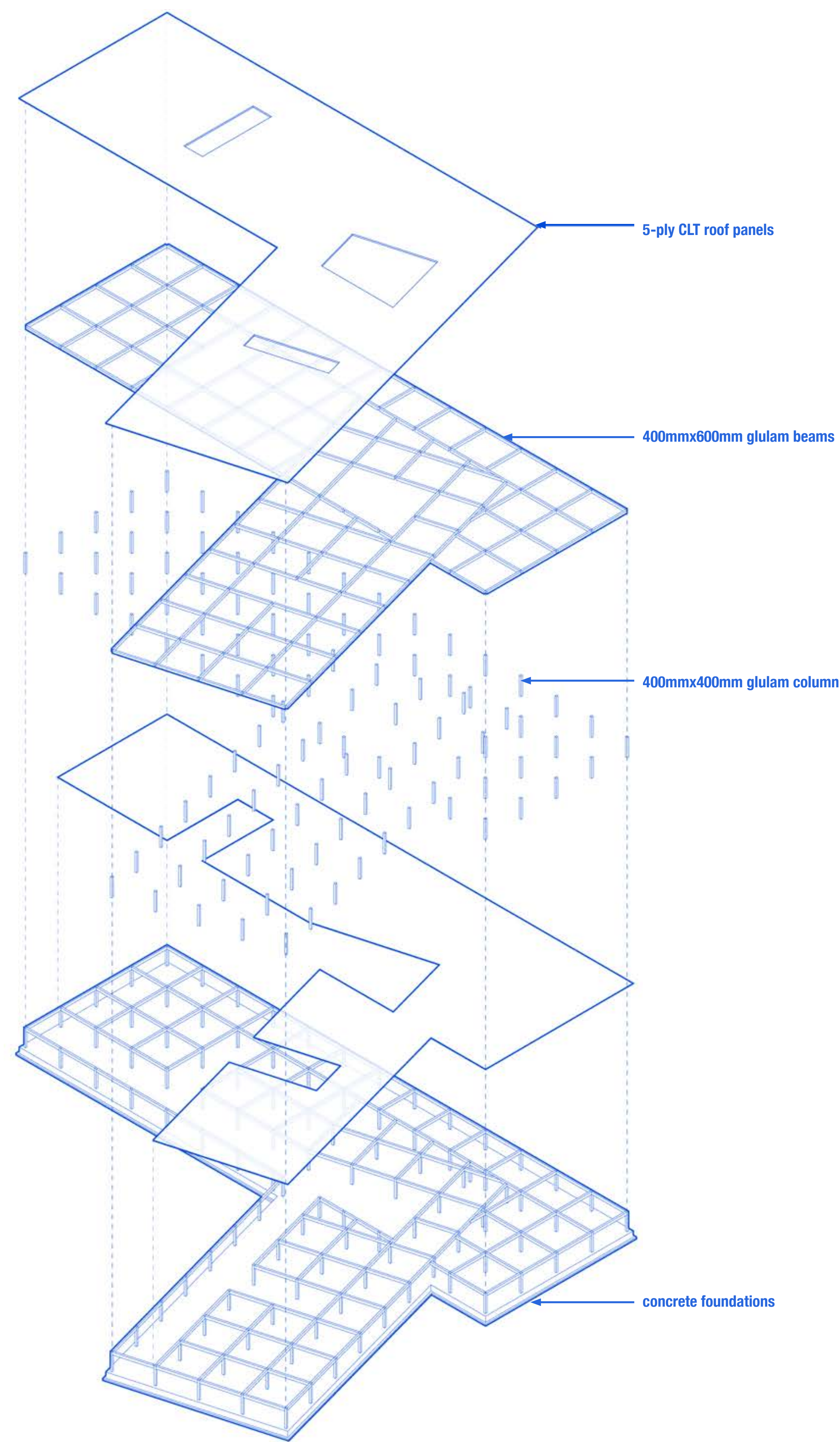
structural axonometric 1:500
