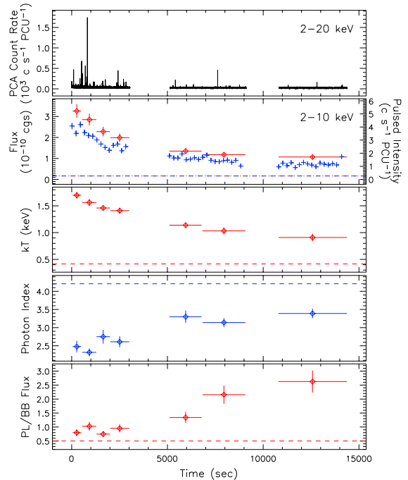
FIGURE 3. Light curve and time evolution of persistent and pulsed emission during the burst observation [22]. Top panel: 2–20 keV RXTE /PCA light curve for 1E 2259+586 on June 18, 2002, at 125 ms resolution. The gaps are Earth occultations. 2nd panel: Unabsorbed persistent (diamonds) and pulsed (crosses) fluxes in the 2–10 keV band. The vertical scale of each parameter has the same relative range to show the lower pulsed fraction within this observation relative to the pre-burst value. The horizontal dashed (dotted) lines denote the quiescent (pre-burst) levels of each parameter. 3rd panel: Blackbody temperature of the persistent and pulsed emission spectrum assuming a two-component model consisting of the blackbody and a power law. The same spectral fits show that the blackbody radius remained at \sim 1 km throughout. 4th panel: Power-law photon index of the persistent and pulsed emission spectrum for same model as in the 3rd panel. 5th panel: Ratio of the unabsorbed 2–10 keV power-law flux and the bolometric blackbody flux.
