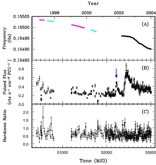
FIGURE 1. (A) Long-term frequency history of 1E 1048–5937 from RXTE monitoring [after 14, ; Gavril & Kaspi, in preparation]. The heavy lines pre-2002 represent intervals over which phase-coherent timing was possible. After 2002, observations began weekly. (B) Pulsed flux in the 2–6 keV band. We have detected clear flux variations in this AXP. The two arrows indicate the epochs of the bursts reported by Gavril et al. [17]. (C) Hardness ratio computed for the energy range (2 – 4 keV)/(6 – 10 keV). There are no significant variations in spite of the frequency and pulsed flux variations.
