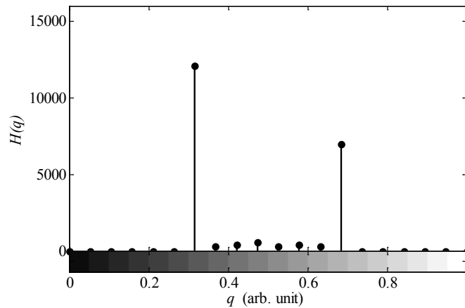
Figure 4.2. Image histogram
