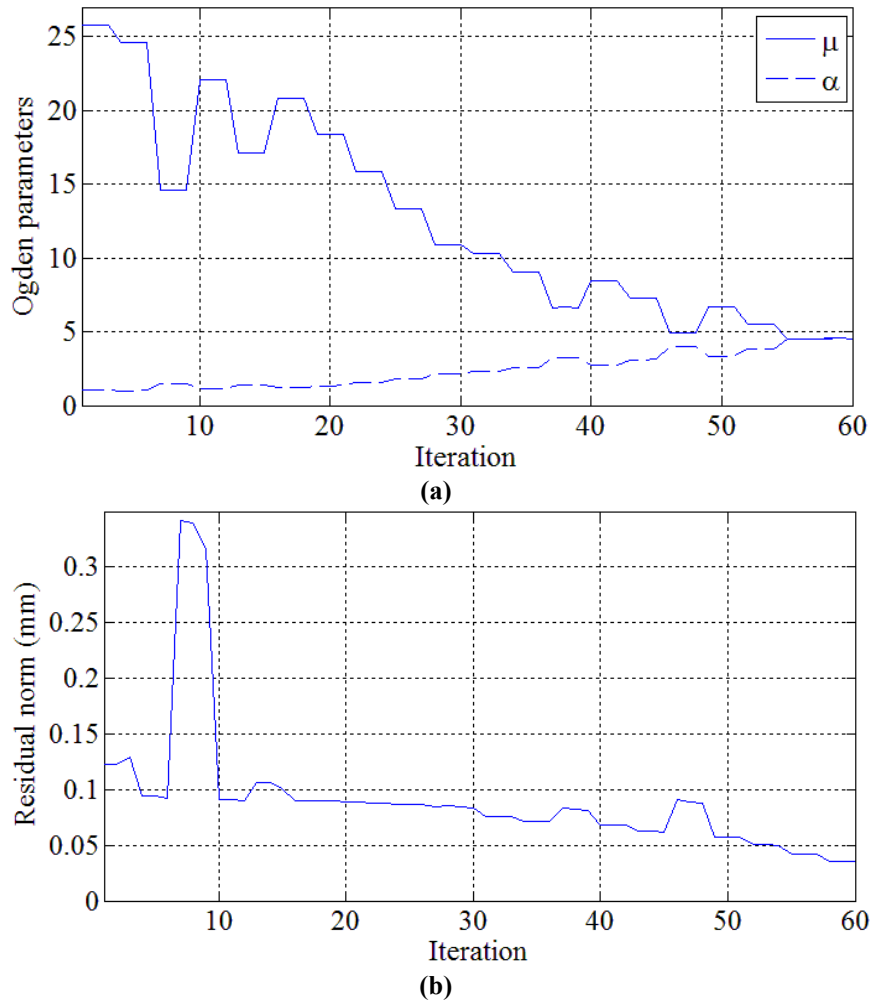
Figure 9.3. Ogden parameters (a) and the residual error (b) during optimization
