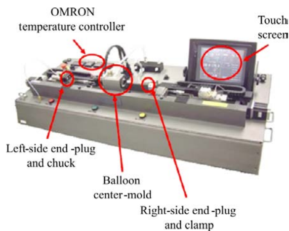
Figure 7.2. The balloon forming machine (9810-H, Interface Catheter Solutions)
