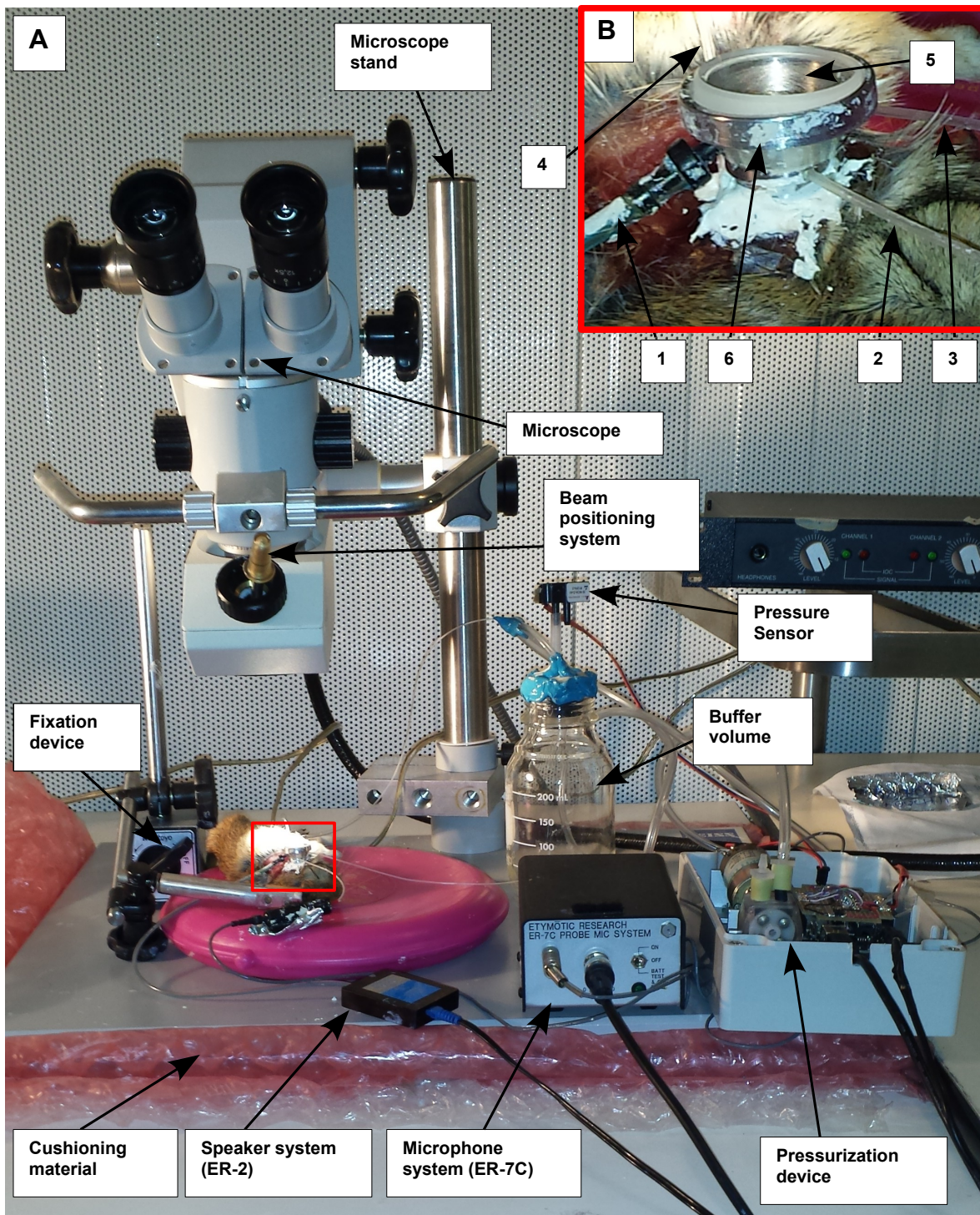
Figure 4.4: A. Experimental setup. B. Close up of the preparation. (1) Tubeophone (ER-2) tube. (2) Probe microphone (ER-7C) tube. (3) Ventilation tube of coupler. (4) Ventilation tube of middle ear. (5) Glass window. (6) Acoustic coupler secured to the bulla with dental cement.
