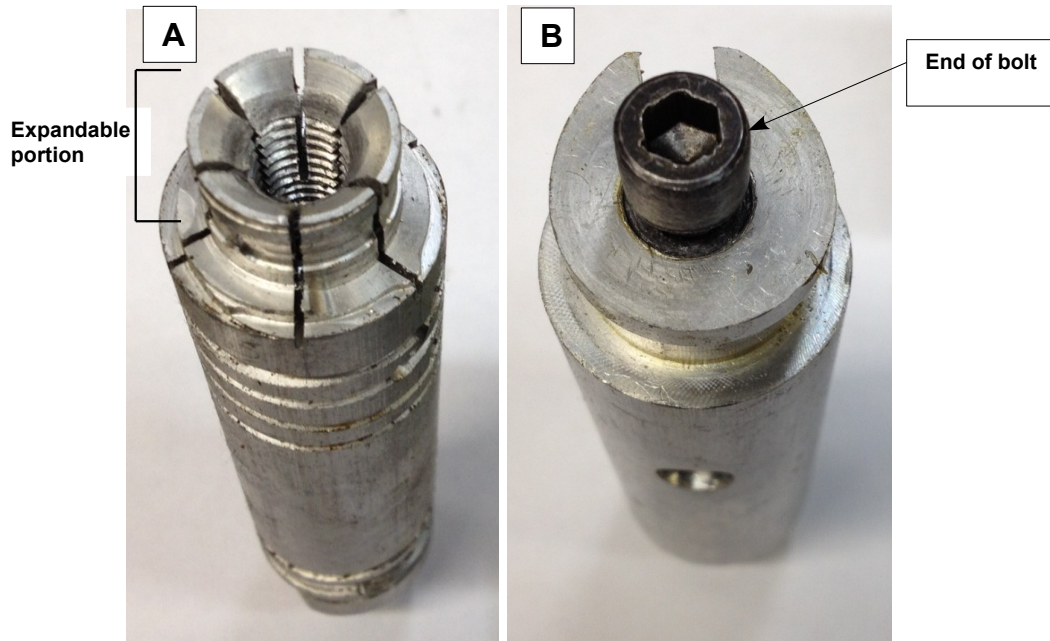
Figure 4.19: A. Top view of the specialized chuck or collet used to hold the coupler during milling operations. The coupler is mounted around the top expandable portion. B. Bottom view of the collet. A bolt is tightened to expand the upper walls.
