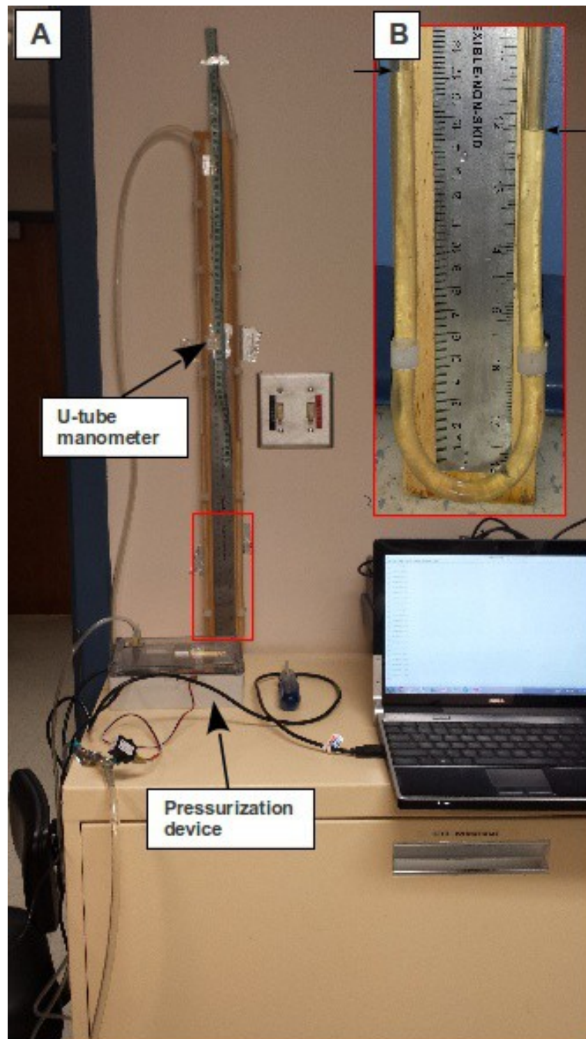
Figure 4.26: A. Pressurization device calibration setup. B. Close-up of the U-tube manometer. The arrows correspond to the water levels used to calculate the pressure in the system.
