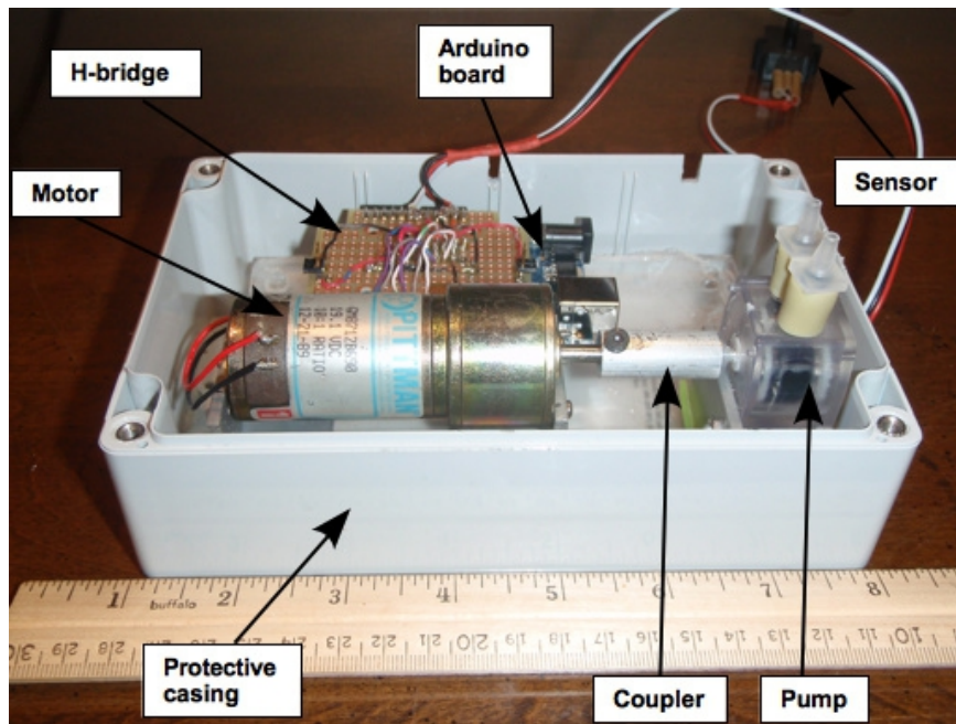
Figure 4.20: Pressurization device including sensor, controller, motor and pump.
