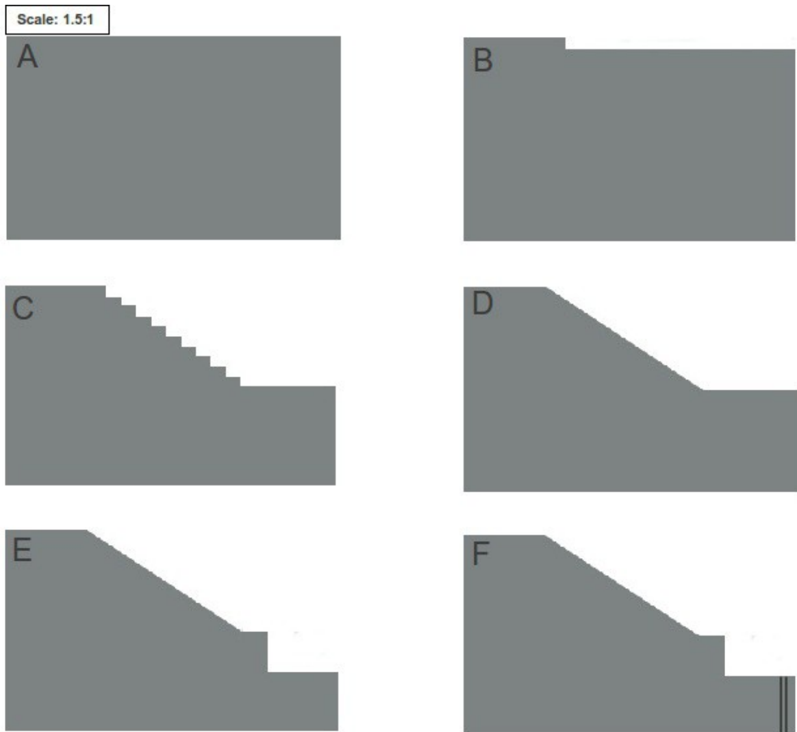
Figure 4.15: Schematic diagrams of the workpiece at various stages of the CNC lathe operation (side view) A. Aluminum cylindrical workpiece after the facing pass. B. Workpiece following the first pass with the roughing tool. C. Workpiece following several passes with the roughing tool. After each pass the tool is translated a small distance to the right, resulting in a series of steps. D. Workpiece following multiple passes with the finishing tool, used to smooth the steps. E. Workpiece following the machining of a cylindrical rim at the base of the coupler. F. Workpiece following the machining of threads.
