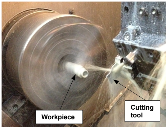
Figure 4.16: The roughing tool approaches the workpiece as it spins very rapidly about its long axis. Cutting fluid is applied to the cutting tool and workpiece continuously during the machining process.
