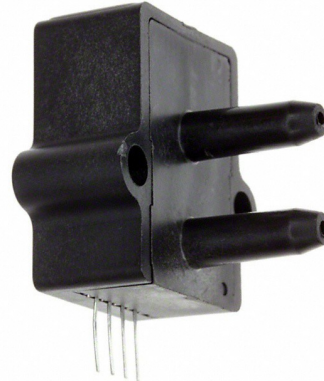
Figure 4.23: 20 INCH-D-4V amplified low-pressure sensor (Source: http://www.allsensors.com , retrieved 2012 June 1)
