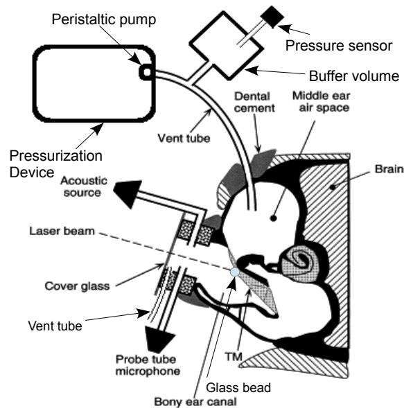
Figure 4.1: Schematic illustration of the gerbil middle ear and the experimental preparation. (After Lee and Rosowski 2001)
