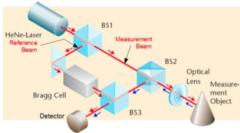
Figure 4.29: Schematic diagram of the operation of the laser Doppler vibrometer. Beam splitters BS1, BS2, BS3 split and recombine the HeNe-laser beam travelling towards the detector. (After polytec.com)
