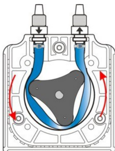
Figure 4.24: Schematic diagram of a peristaltic pump (Source: http://www.blwwhite.com , retrieved 2013 December 1)
