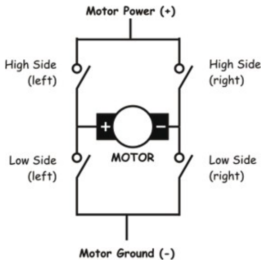
Figure 4.22: Simplified schematic diagram of an H-bridge (Source: http://www.mcmanis.com , retrieved 2013 December 1)
