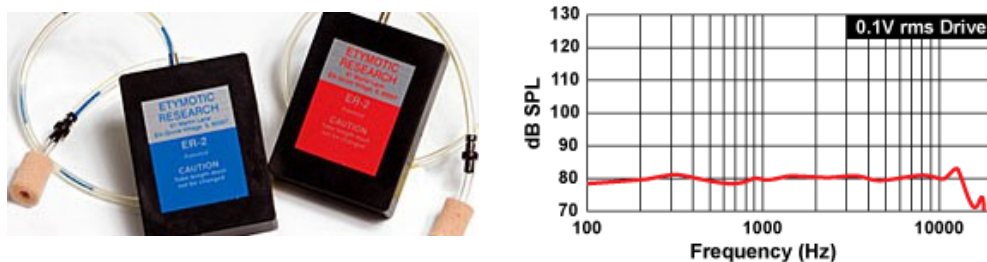
Figure 4.5: ER-2 Tubeophone, and its frequency response.
