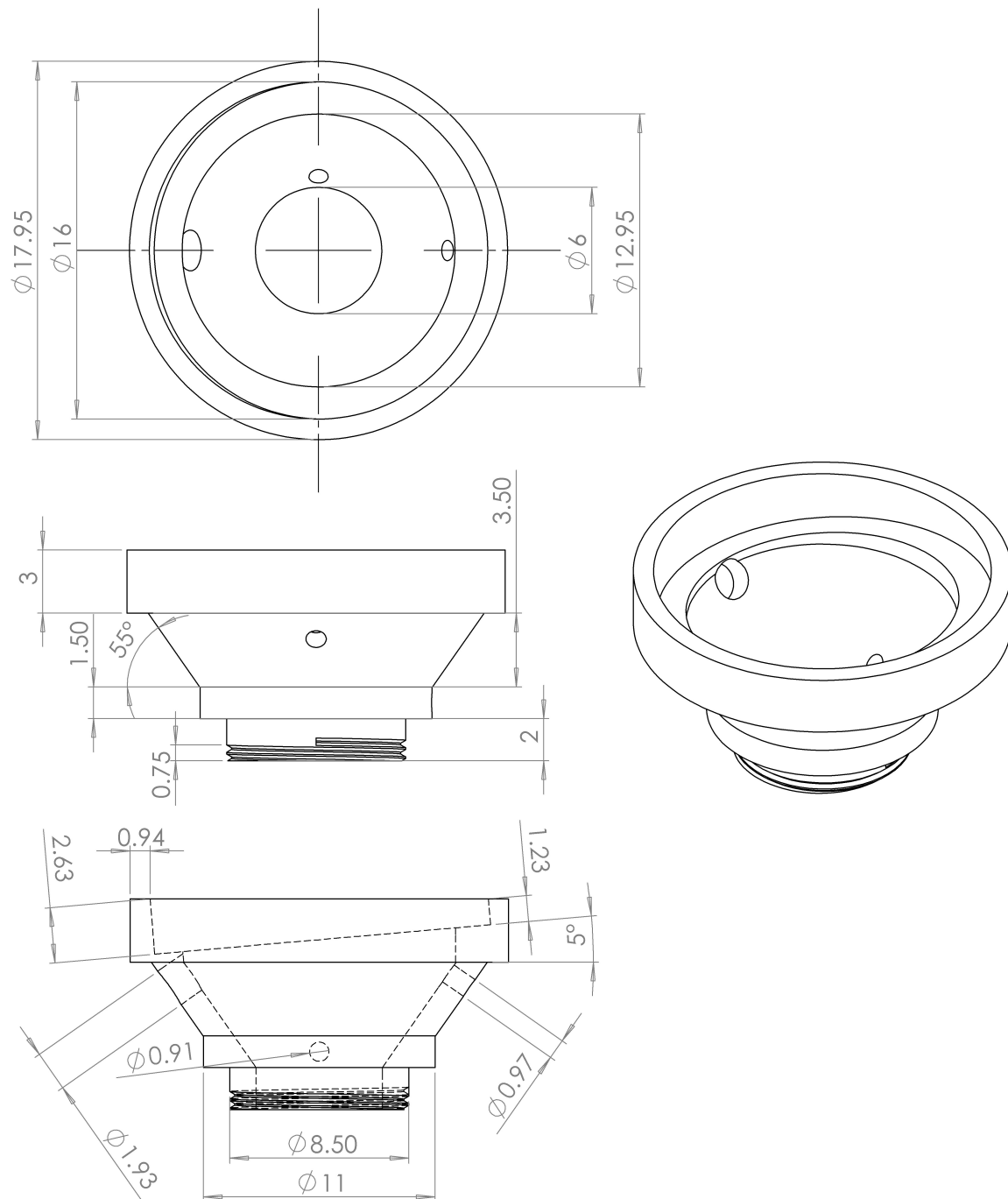
Figure 4.10: Engineering drawing of the coupler designed and manufactured for use in this study. All linear dimensions shown are in millimetres.
