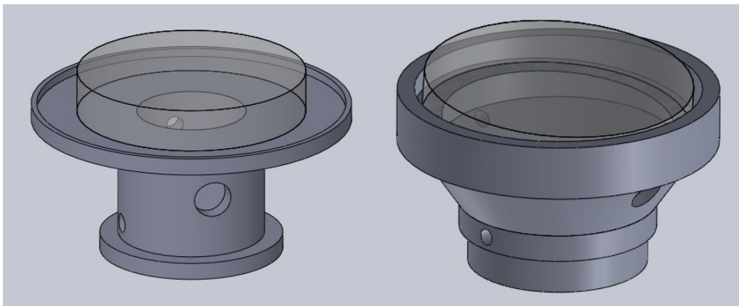
Figure 4.9: 3-D CAD models of the previous coupler and washer (left) and the newly designed coupler and washer (right) used in this study. Details of the new coupler and washer are shown in the engineering drawings of Figures 4.10 and 4.11, respectively.
