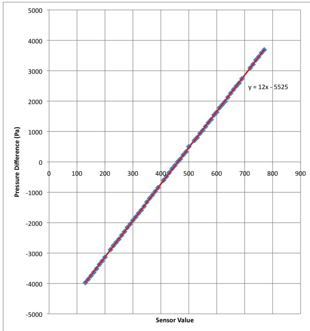
Figure 4.27: Pressurization device calibration data and fitted straight-line.
