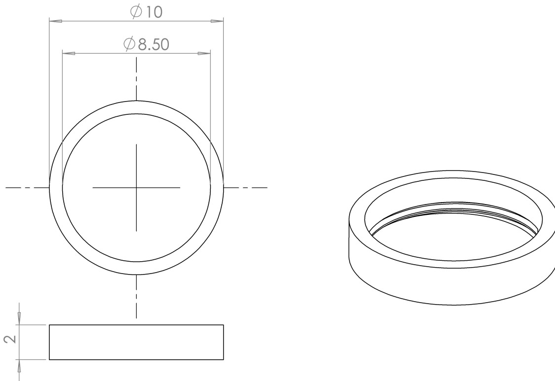
Figure 4.11: Engineering drawing of the washer designed and manufactured for use in this study. All dimensions shown are in millimetres. Threads are on the inside, at the bottom.
