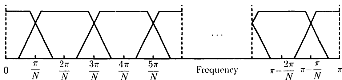
(c) Filter responses for systems T1 and T3
