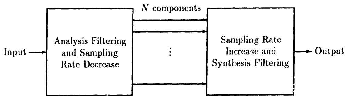
Fig. 1.3 General illustration of a subband system
