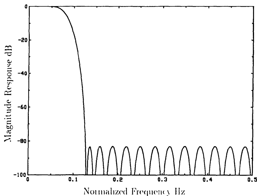
Fig. 4.2 Magnitude response of the Nyquist filter. Example 1
