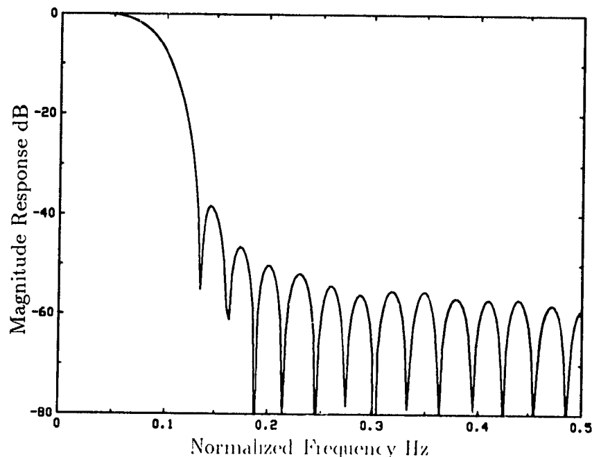
Fig. 5.1 Magnitude response of the lowpass filter for system T1. The weighting factors are (\gamma_1, \gamma_2, \gamma_3, \gamma_4) = (100, 1, 1, 0.01) .
