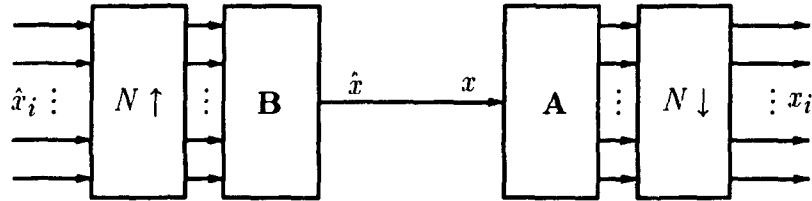
(c) Identity transmultiplexer
