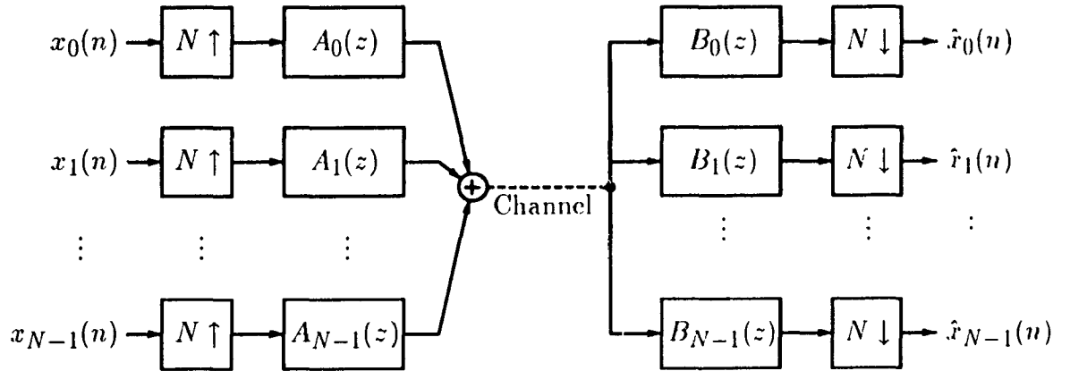
Fig. 2.1 A transmultiplexer system
