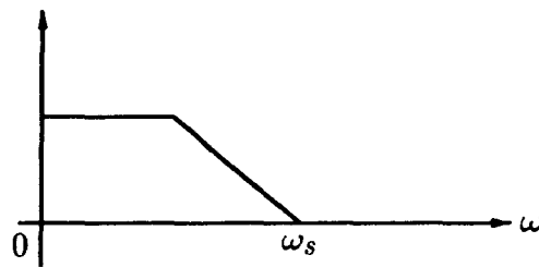
Fig. 2.5 Frequency characteristic of a general bandlimited lowpass prototype
