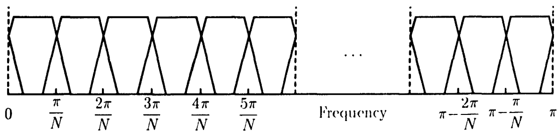
(e) Filter responses for systems T1 and T5
