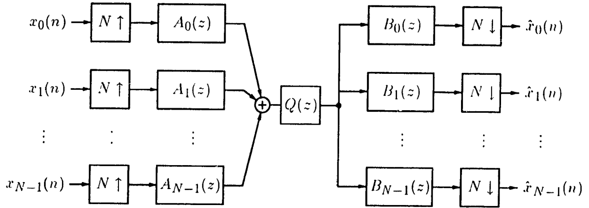
Fig. 6.1 Channel distortion in a transmultiplexer
