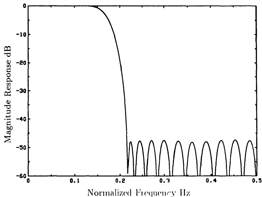
Fig. 4.5 Magnitude response of the minimum phase part of the Nyquist filter designed with the same parameters as in [29]
