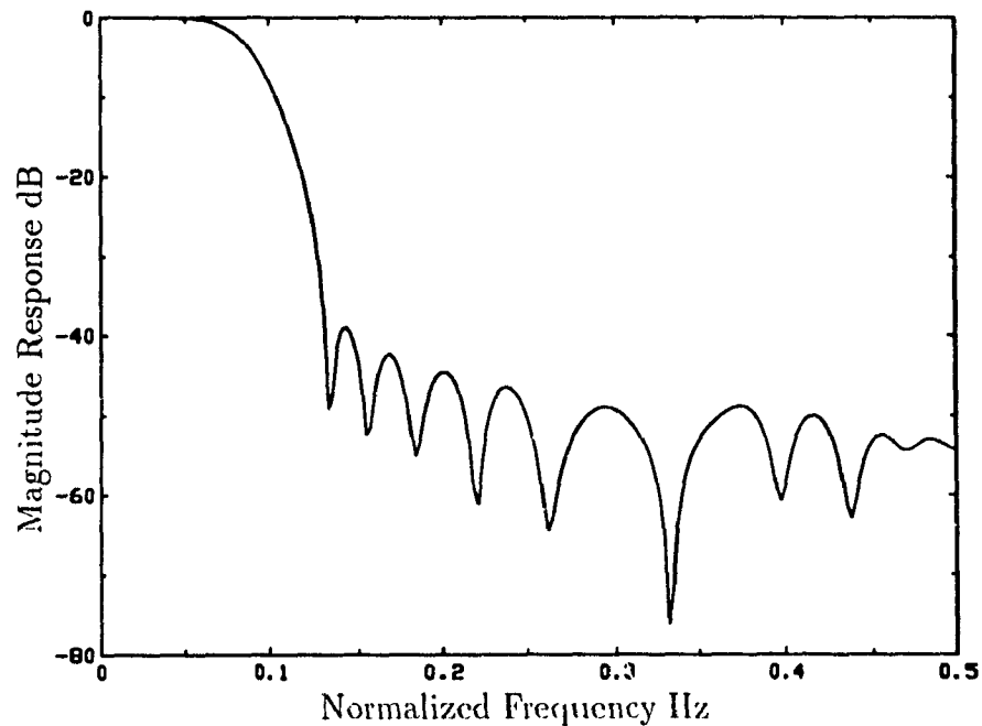
Fig. 5.2 Magnitude response of the lowpass filter for system T3. The weighting factors are (\gamma_1, \gamma_2, \gamma_3, \gamma_4) = (100, 1, 1, 0.01) .
