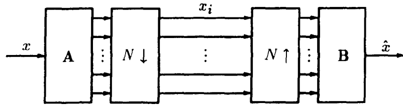
(a) Identity subband system
