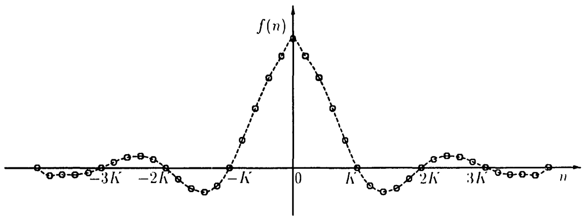
Fig. 4.1 Typical Nyquist response f(n) (shown for K = 5 , M = 39 and \beta = 0.2 )
