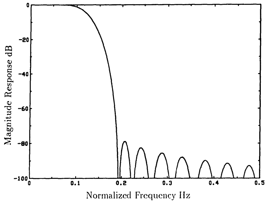
Fig. 4.3 Magnitude response of the Nyquist filter: Example 2
