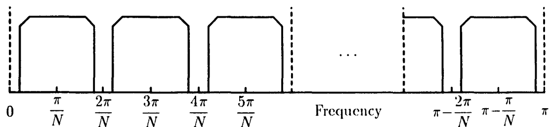
(b) Spectrum of input signal multiplied by (-1)^n after sampling rate expansion
