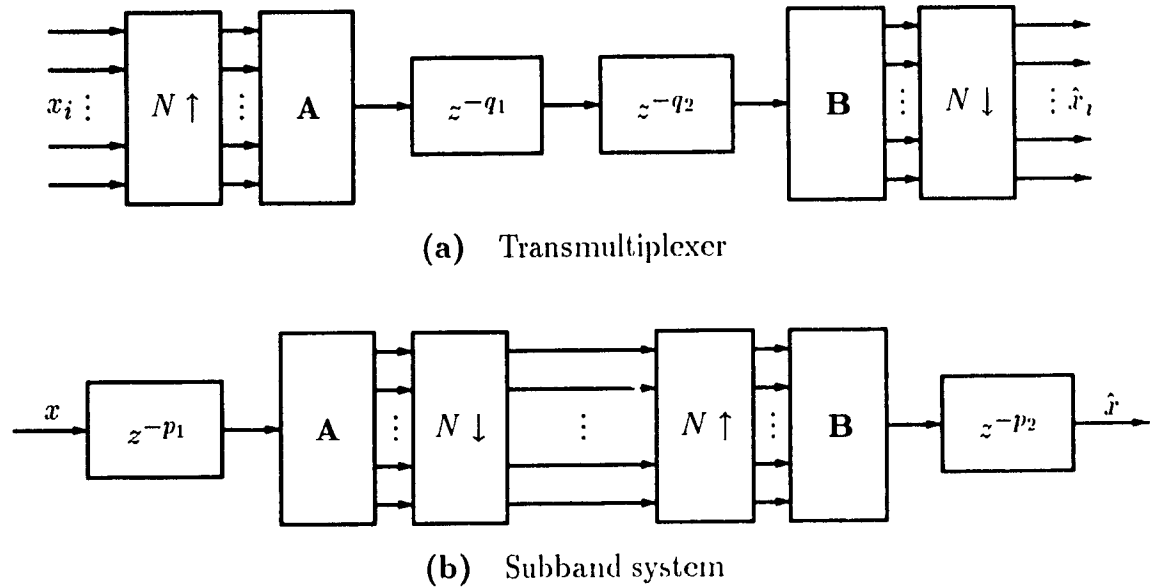
Fig. 2.4 Application of delay factors
