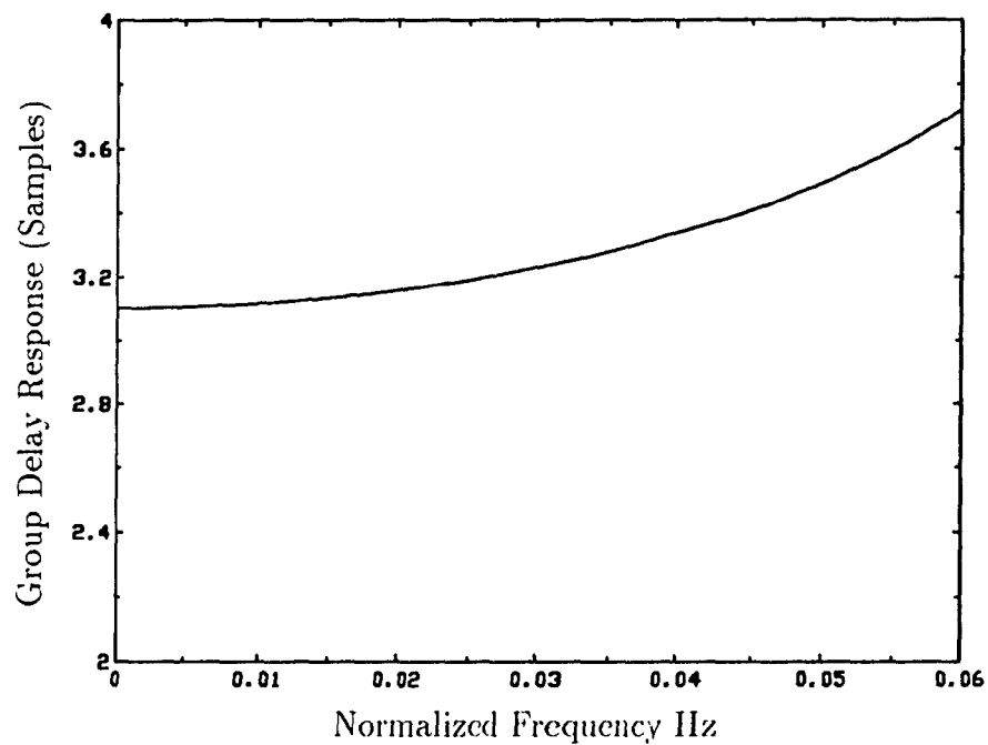
Fig. 4.4 Group delay response of the minimum phase part: Example 2
