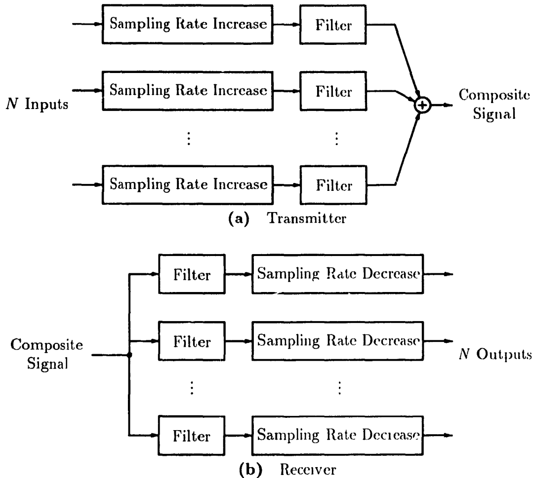
Fig. 1.1 General transmultiplexer structure
