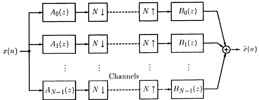
Fig. 2.2 A subband system
