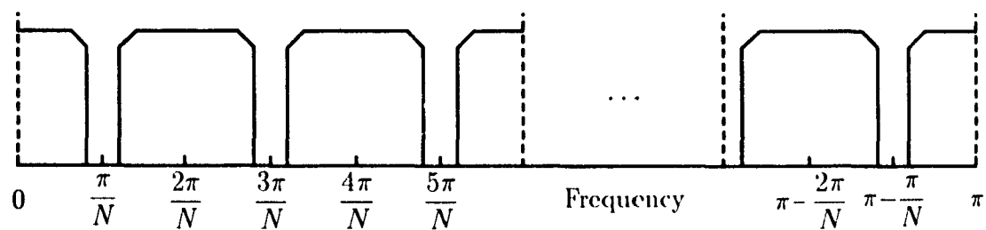
(a) Input signal spectrum after sampling rate expansion
