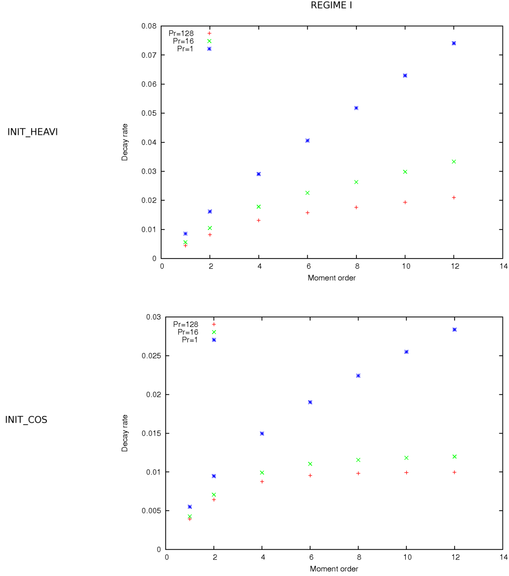
Figure 4-2: Top: exponential decay of the various moments \langle |\phi|^n \rangle for 1 \leq n \leq 12 in the first exponential decay (regime I, 25T \lesssim t \lesssim 60T ) for INIT_HEAVI (top) and INIT_COS (bottom). We show Pr = 1; 16; 128 . Pr = 1 is given to show a different situation where the decay is essentially controlled by diffusion. The vertical scale is not the same for the two plots.
