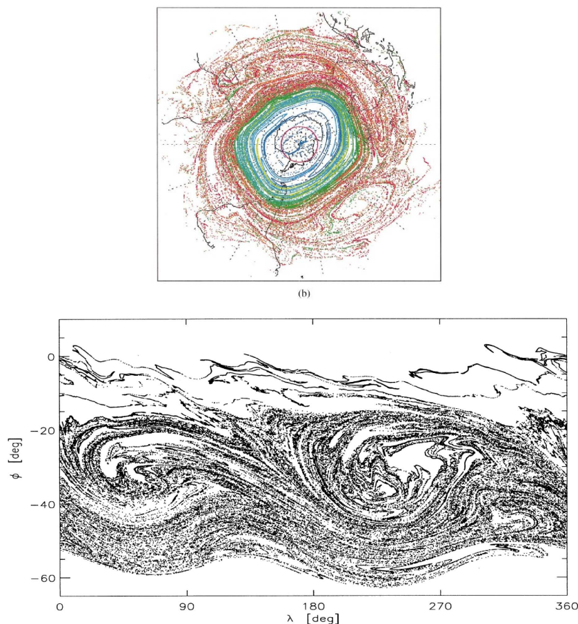
Figure 1-6: On the top are shown the results of trajectory calculations on the 450\text{ K} isentrope ( 20\text{ km} ) during one month in the northern hemisphere winter ( Shepherd , 2000). At the bottom, it is the same but on the 1000\text{ K} isentrope corresponding to the upper stratosphere ( Ngan and Shepherd , 1999a). The winds are calculated with the Canadian Middle Atmosphere Model (CMAM). The cat's eye structures are clearly visible. There are four at 450\text{ K} and two at 1000\text{ K} . This reduction is due to the fact that only the largest scale waves reach the upper stratosphere. The transport barriers (polar vortex and tropical pipe) are clearly visible.
