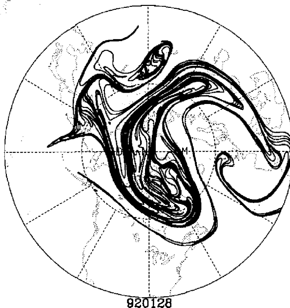
Figure 1–2: Contour advection with surgery (from Waugh and Plumb (1994)) in the stratosphere on the 450 K isentrope in January 1992 in the Northern Hemisphere (altitude around 20 km). The contours are circular at the initial time and the advection is run during two weeks. The length of the contours grows exponentially.
