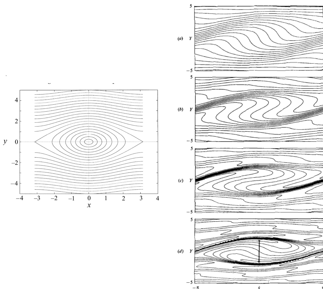
Figure 1–5: On the left is shown the SWW solution for weakly nonlinear Rossby waves critical layers (Kelvin Cat’s eye), from Ngan and Shepherd (1997a). With x the zonal coordinate and Y a rescaled meridional coordinate, the streamfunction is given by -\frac{1}{2}Y^2 + \cos x . Formally this is the equivalent of the phase space of a simple pendulum without friction with the angle in x and the acceleration in y . On the right is shown the advection of potential vorticity as predicted by the SWW theory (from Killworth and McIntyre (1985)). The potential vorticity is a passive tracer at the leading order (however one can note the rotation of the cat’s eye).
