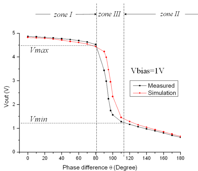
Figure 2.8 Measured response of phase detector when V_{bias} = 1.0 V
