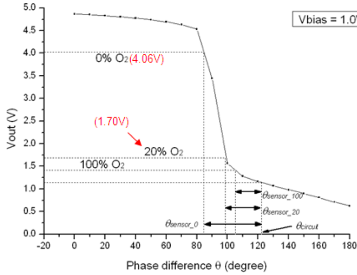
Figure 2.11 Calibration of phase detector with V_{bias} = 1.0\text{ V}
