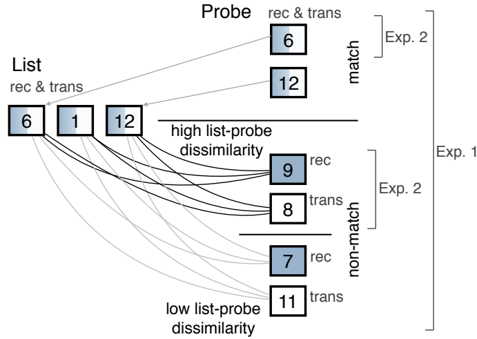
Fig. 7.1 Illustration of the construction of list-probe sequences. Digits refer to individual sounds (#1–14), blue boxes to recordings, white boxes to transformations, half blue/half white boxes to numbers that are instantiated by both materials. Per list, there were two matching probes, equally selected from all three serial positions across the different trials (see Table 7.1). Non-matching probes were selected such that both materials’ lists had a probe with high, and another with low list-probe dissimilarity (and the distribution of dissimilarities did not differ across material). Exp. 2 only used a subset of trials.
