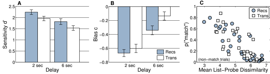
Fig. 7.2 Exp. 1: d' scores (A), response biases (B), and proportion of match responses as a function of mean dissimilarity of list and probe items for non-match trials (C). Error bars depict standard errors of the mean.
