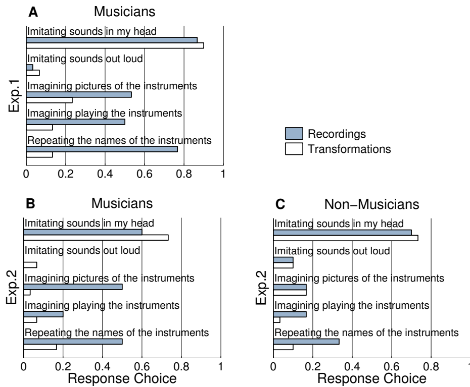
Fig. 7.7 Self reports from post-experiment questionnaires for (A) musicians from Exp. 1, (B) musicians from Exp. 2, (C) non-musicians from Exp. 2. Participants indicated which of the five strategies they had used to accomplish the memory task. Proportion of response choices displayed on the x-axis.
