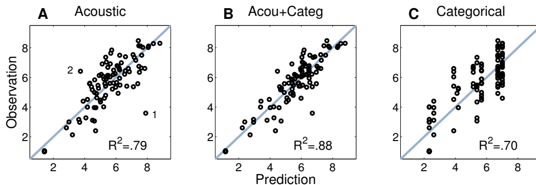
Fig. 6.5 Mean pairwise dissimilarity ratings for Set 1 (observations; y axis) and predictions based upon acoustic descriptors (A), audio and categorical predictors combined (B), and category membership of the instruments (C). Data points 1 and 2 in the left panel are discussed in the text.
