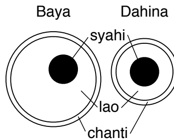
Fig. 5.1 Schematic drawing of the tabla drum surface including the outer ring ( chanti ), the inner surface head ( lao ), and the patch ( syahi ). The Baya is usually played with the left hand, the Dahina with the right hand.
