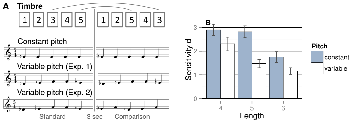
Fig. 4.3 (A) Schematic of pitch variability in Exps. 1 and 2 for an exemplary 5-item sequence. Although pitch sequences are identical for standard and comparison in Exp. 1, they differ in Exp. 2. (B) d' scores for the factors sequence length and pitch variability. Error bars indicate 95% confidence intervals.
