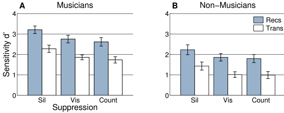
Fig. 7.5 Exp. 2: d' scores for musicians (A) and non-musicians (B) in the suppression conditions of silence, visual suppression, and articulatory suppression (counting).
