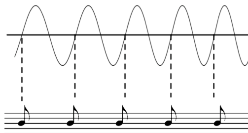
Example 8-1. Zero-crossings, at 0^\circ phase, mapped to note onset.
