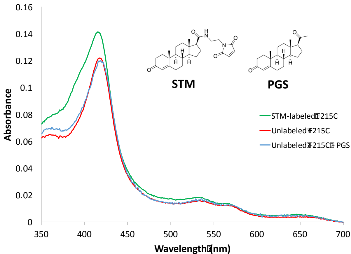
Figure 2. Absorbance spectra of the ligand-free unlabeled, STM-labeled, and PGS-treated F215C mutant of CYP3A4. To demonstrate that unconjugated STM was likely removed during the washing step and is not responsible for the high-spin shift (390 nm peak), a mock-bioconjugation control experiment was performed by treating the F215C mutant with non-modified progesterone (PGS, a good mimic of STM) under similar conditions. As evident from the absorbance spectra, the PGS-treated CYP3A4 spectrally resembles the untreated P450. Thus, the high spin shift in STM-labeled CYP3A4 is induced by the attached steroid rather than the trace amounts of non-conjugated STM that might be present in the sample.
