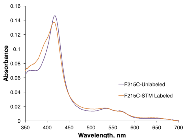
Figure 4. Absorbance spectra of the purified STM-labeled and unlabeled CYP3A4 C215 mutant. Both enzymes are predominantly in the low-spin state (418 nm peak), but the STM-labeled mutant has the larger high-spin content (a pronounced shoulder at 386 nm). The high spin content in STM-bioconjugated CYP3A4 (~15%) was estimated based on the absorbance spectra of the ligand-free (100% low-spin) and bromoergocriptin-bound protein (100% high-spin conversion) samples.
