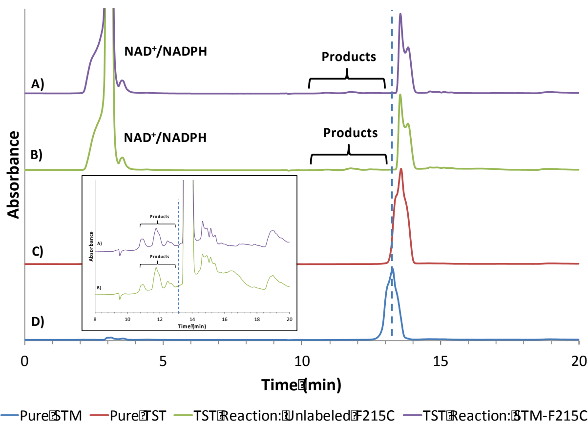
Figure 3. HPLC-UV chromatograms of the testosterone (TST) oxidation reaction by STM-labeled or unlabeled mutant F215C. A) Oxidation of TST by STM-labeled mutant F215C consisting of P450, CPR, SOD, excess TST and excess NADPH. The location of the 4 products is shown by the bracket. B) Oxidation of TST by unlabeled mutant F215C consisting of P450, CPR, SOD, excess TST and excess NADPH. The location of the products is shown by the bracket. C) Pure TST with a retention time of 13.4 min. D) Pure STM with a retention time of 13.1 min. The dashed blue line is drawn to demonstrate the expected location of STM in chromatograms A and B. The inset is zoomed in to show the product peaks in samples A and B.
