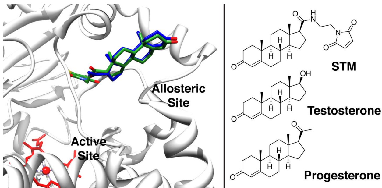
Figure 1. A modified X-ray crystal structure image showing steroid-maleimide (STM) conjugated to C215 of a CYP3A4 mutant. STM (in green) is superimposed on the existing, co-crystallized progesterone (in blue). STM and C215 were built into the allosteric site of CYP3A4 using the USCF Chimera package[35], PDB structure 1W0F[5] and the Persistence of Vision ™ Raytracer. Chemical structures of the steroids and STM are shown for comparison.
