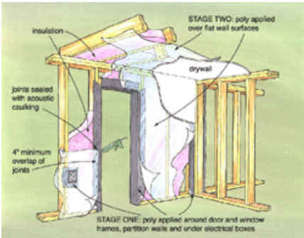
Figure 1.2 Window and frame insulation
