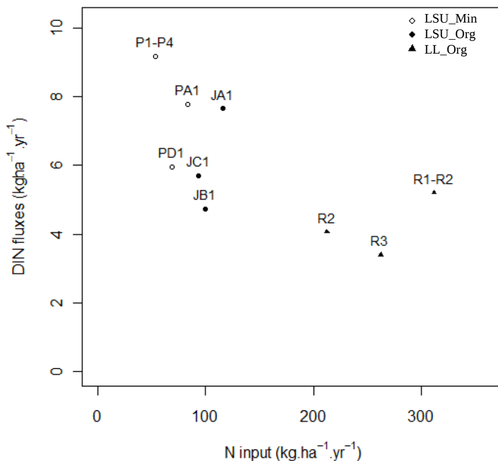
Figure 3.5. Nutrient inputs as fertilizers and nutrient fluxes exported to streams in industrial oil palm plantation watersheds. a/ N inputs vs. dissolved inorganic N (DIN) fluxes exported. LSU_Min: Mineral fertilized watersheds located on loamy-sand uplands; LSU_Org: Organic fertilized (empty fruit bunch only) watersheds located on loamy-sand uplands; LL_Org: Organic fertilized watersheds (mainly palm oil mill effluent) located on loamy lowlands. The R3 outlet is located downstream from the mill.
