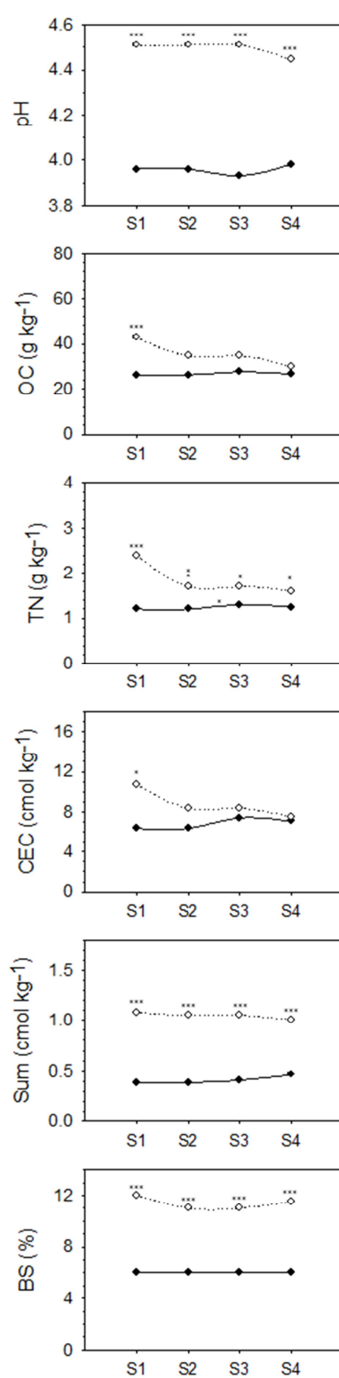
Loamy-sand uplands
