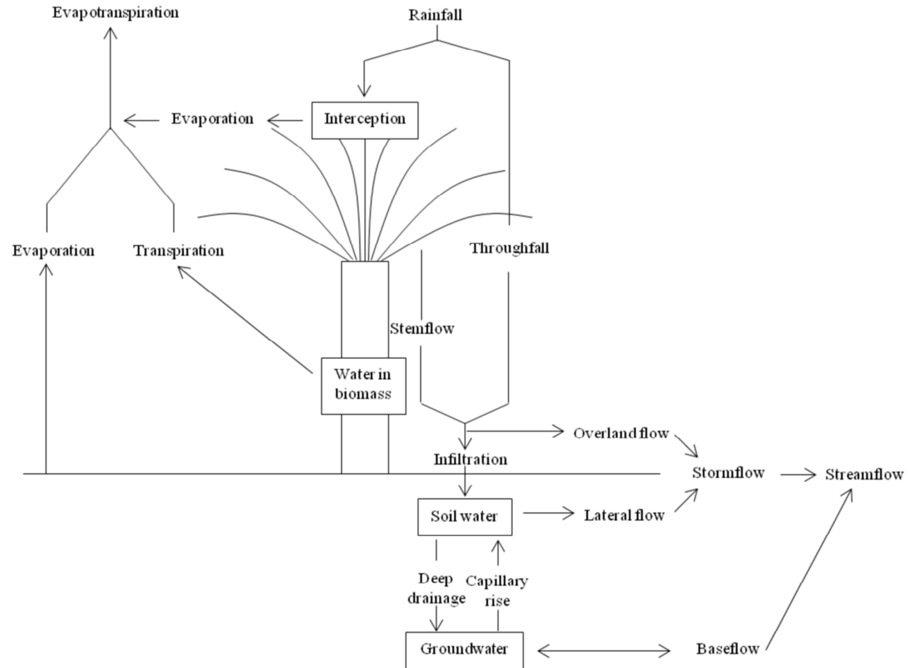
Figure 1.4. The hydrological cycle in oil palm plantation. Boxes indicate storage pools, arrows indicate fluxes.
