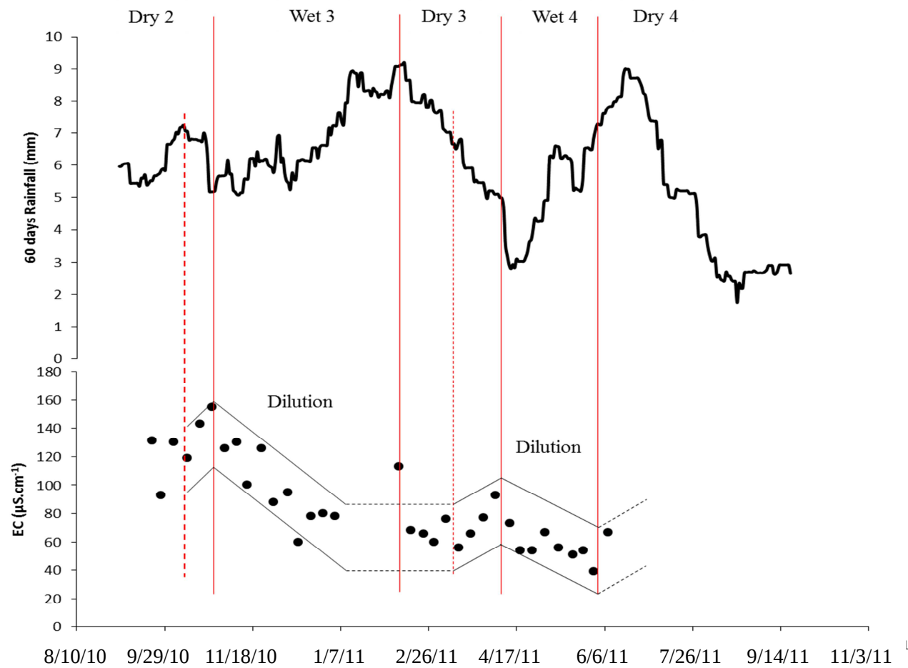
Figure 3.2. Electrical conductivity (EC) values in groundwater and 60 days-averaged rainfall pattern from September 1 st , 2010 to June 6 th , 2011 (EC values measured in the piezometer SP-P0 are shown as illustration).
