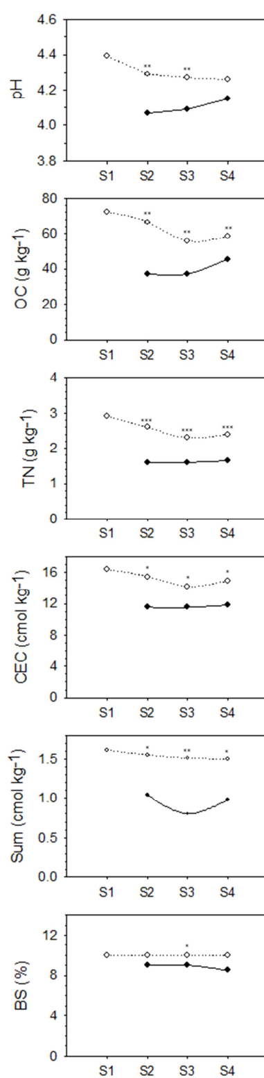
Loamy lowlands
