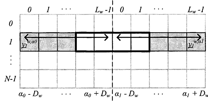
Fig. 3.5 Splitting temporal erasure bursts: The temporal erasure burst is split along the middle so that y_l^{w,\alpha_0} and y_l^{w,\alpha_l} are each used to reconstruct half the samples. The heavy frame delineates the temporal erasure burst, and the dashed line separates the two frames under analysis. Double-sided arrows specify the two temporal codevectors under analysis, and we highlight the available samples in both codevectors. Upper column labels specify the frame-relative time indices; bottom column labels specify the time index n ; row labels specify subband indices.
