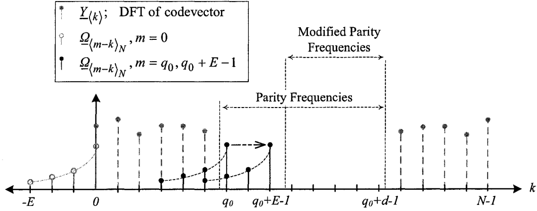
Fig. 2.1 Error detection with erasures using the modified codevector: Circularly convolving the erasure locator coefficients \underline{\Omega}_{\langle m-k \rangle_N} with the entries \underline{y}_{\langle k \rangle} of the original codevector eliminates the E parity frequencies at k = q_0, \dots, q_0 + E - 1 . Note the signal shapes where chosen strictly for illustrative purposes. (Adapted from Rath and Guillemot [8].)
