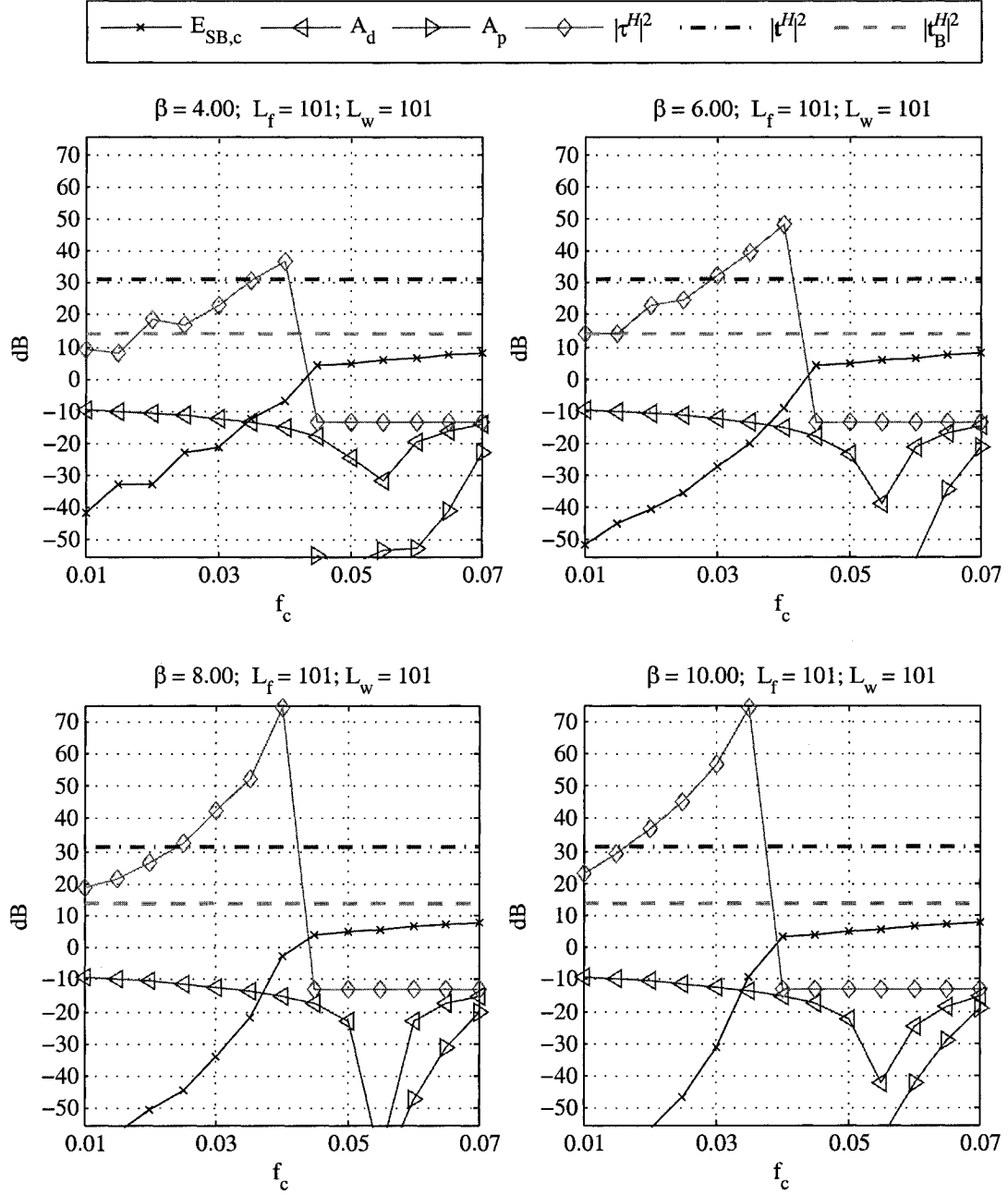
Fig. 5.9 TFBD code design (Kaiser, L_f = 101 ; Hanning, L_w = 101 ): Filterbank amplitude distortion ( A_d ) and aliasing power ( A_p ), vs. minimax stop-band component ( E_{SB,c} ) and maximum row magnitudes of reconstruction matrices for temporal code ( |\tau^H|^2 ), subband code ( |t^H|^2 ), and benchmark DFT code ( |t_B^H|^2 ). A burst length of E = 4 was used in all cases.
