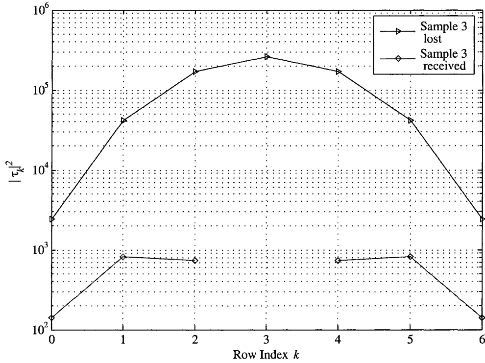
Fig. 4.1 Pivot effect on row-magnitudes of reconstruction matrix: Row magnitudes |t_k^T| of reconstruction matrix T for a (25, 11) DFT code. In the first case, T corresponds to a burst of size E = 7 erasures; the second case ( E = 6 ) is that when the sample at position k = 3 (along erasure vector, position e_3 of temporal codevector) is available. Quantization power is normalized to unity. Horizontal axis labels correspond to the erasure vector index (also the row-indices of T ).
