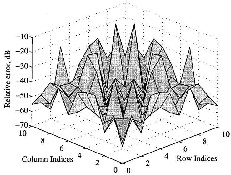
Fig. 5.2 Simulated vs. derived stopband correlation matrix, relative error: The relative error is shown as a surface plot, where the element at the k -th row and l -th column is given by \mathbf{R}_{s\Delta\langle k,l\rangle} in (5.1). The theoretical correlation matrix \mathbf{R}_s , and the simulated version \mathbf{R}_{s,sim} are the same as in Fig. 5.1. The maximum relative error is -12.5 dB.
