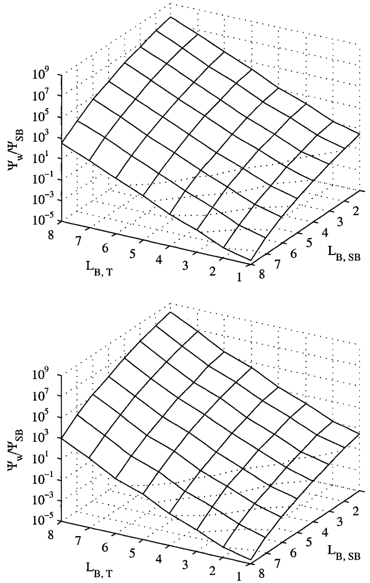
Fig. 5.14 Temporal code vs. benchmark DFT code, Hanning window: Ratio of \Psi_w of (15,10,7) TFB code to CSMSE of (15,7) DFT code at intersection of 2-D cross formation burst. L_{B,T} and L_{B,SB} are the length of the temporal and subband bursts, respectively. Contour lines drawn every 10^{-1} starting at unity. Setup as circled in Fig. 5.11. Top: single 2-D cross formation burst, with comparison sample at cross intersection (temporal position 150 and subband position 7). Bottom: same cross formation burst with 30 extra temporal erasures at positions 0,10,...,140, and 160,170,..., 300.
