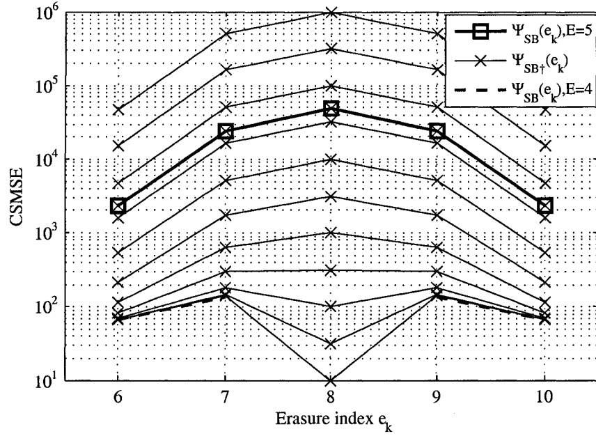
Fig. 4.3 Pivoting and the geometrical interpretation revisited: Plot of subband reconstruction CSMSE ( \Psi_{SB}(e_k) , E = 5 ) vs. pivoted reconstruction CSMSE ( \Psi_{SB+}(e_k) , as given by left hand side (4.33) with e_p = 8 ) for various values of pivot error; (15, 10, 7) TFBD code. The horizontal axis corresponds to the subband codevector indices e_k . The \Psi_{SB+}(e_k) curves decrease monotonically (over all samples e_k ) along with the pivot error up to a limit (heavy dashed line, \Psi_{SB}(e_k) , E = 4 ) corresponding to the case when the pivot sample was received.
