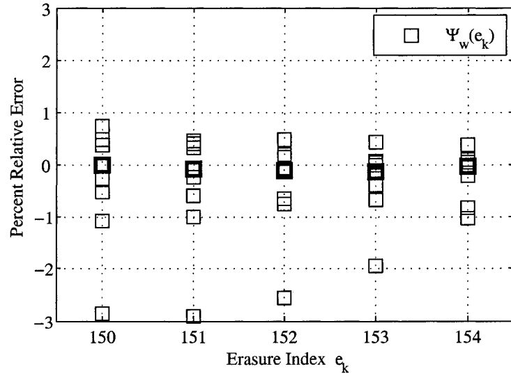
Fig. 5.3 Experimental evaluation of expression for temporal CSMSE: Temporal reconstruction error for (15, 10, 7)-TFBD Code, 1-D temporal burst.
