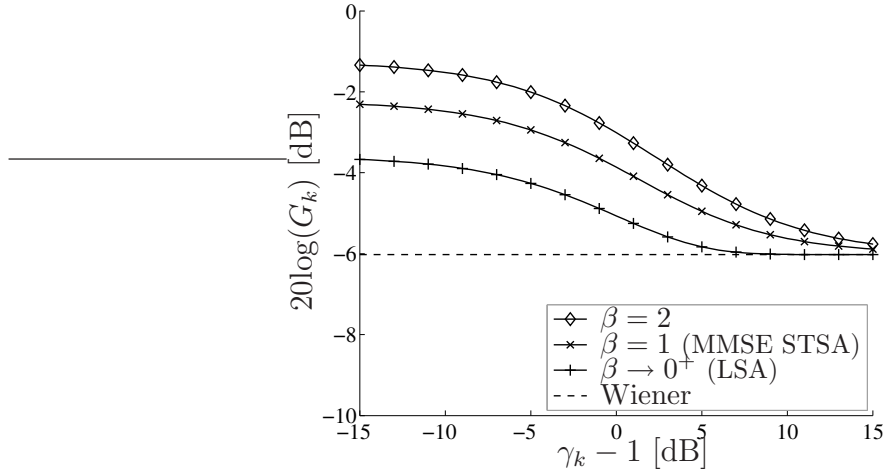
Fig. 3.4 \beta -SA estimator gain ( 20\log G_k ) versus instantaneous SNR, \gamma_k - 1 , for several \beta values ( \xi_k = 0 dB).
