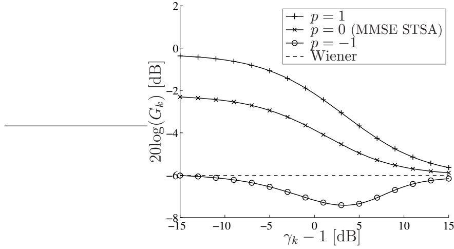
Fig. 3.5 WE estimator gain ( 20\log G_k ) versus instantaneous SNR, \gamma_k - 1 , for several p values ( \xi_k = 0 dB).
