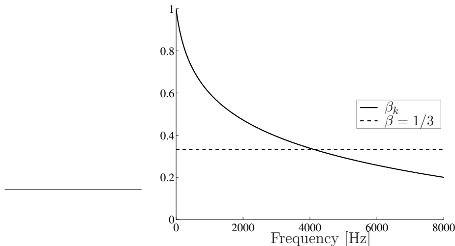
Fig. 5.3 Values of \beta_k and \beta = 1/3 versus frequency.
