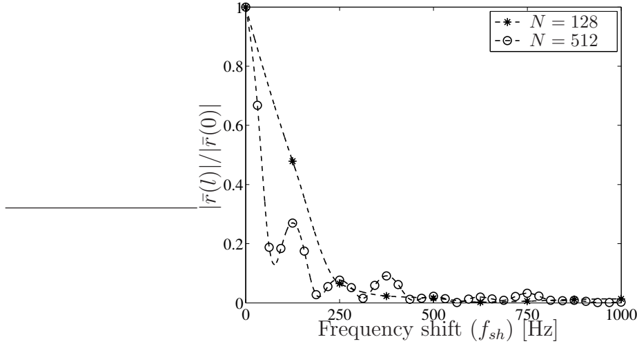
Fig. 7.1 Mean sample autocorrelation function |\bar{r}(l)|/|\bar{r}(0)| versus the physical frequency shift f_{sh} = lF_s/N in Hz for the vowel part of the male spoken word “hood”.
