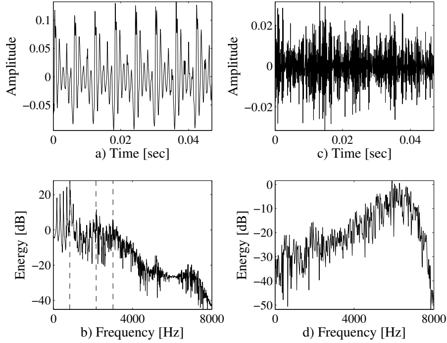
Fig. 2.2 (a) Time domain female uttered voiced phoneme (/ε/); (b) Frequency domain representation of (a); (c) Time domain female uttered unvoiced phoneme (/s/); (d) Frequency domain representation of (c).
