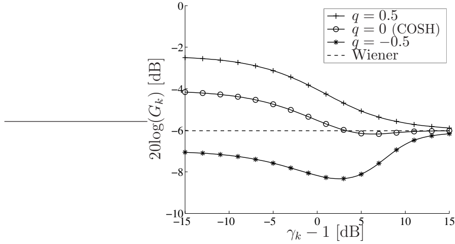
Fig. 3.6 WCOSH estimator gain ( 20\log G_k ) versus instantaneous SNR, \gamma_k - 1 , for several q values ( \xi_k = 0 dB).
