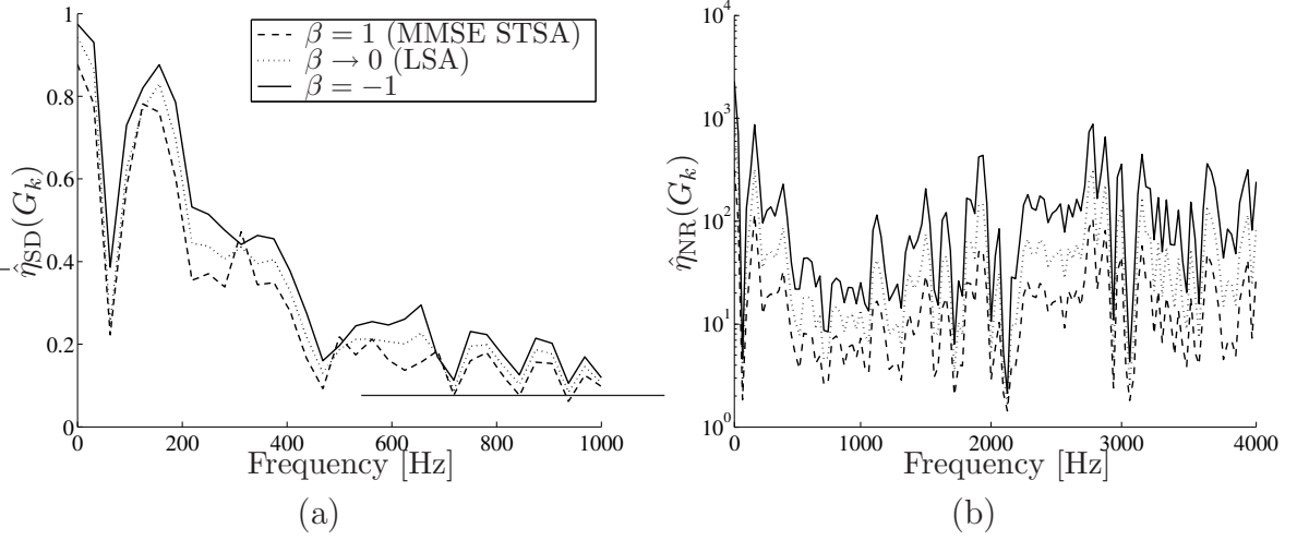
Fig. 4.2 (a) Speech distortion \hat{\eta}_{SD}(G_k) vs. frequency (0 - 1000 Hz) (b) Noise reduction \hat{\eta}_{NR}(G_k) vs. frequency (0 - 4000 Hz) (white noise, SNR = 0 dB).
