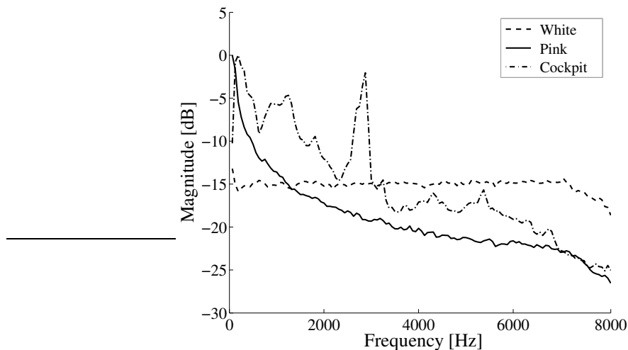
Fig. 8.1 Average noise spectrum magnitudes [dB] versus frequency [Hz] for white, pink and cockpit noises (16 kHz sampling frequency).
