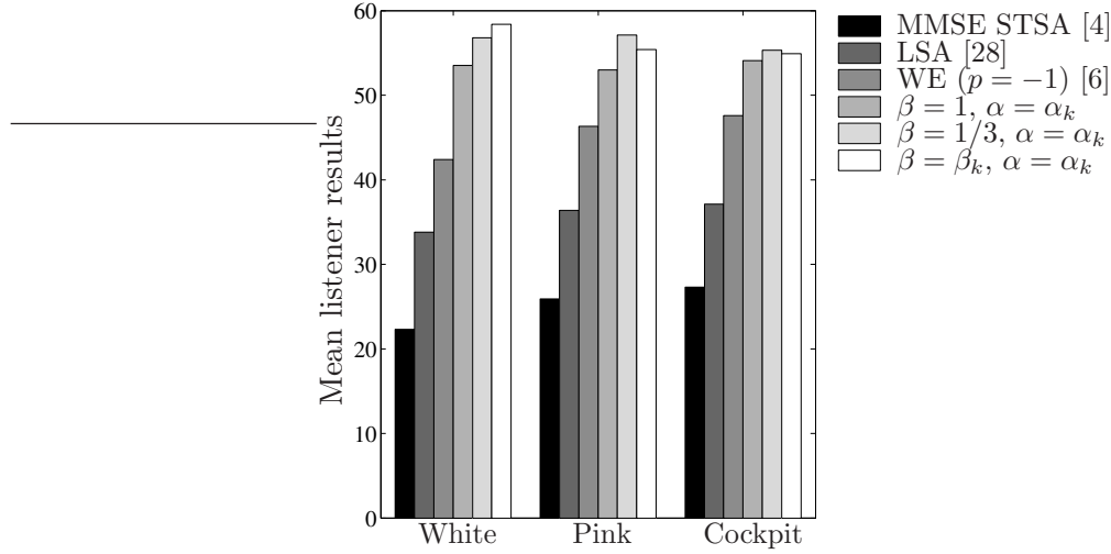
Fig. 8.4 Comparative subjective results for white, pink and cockpit noises (0 dB).
