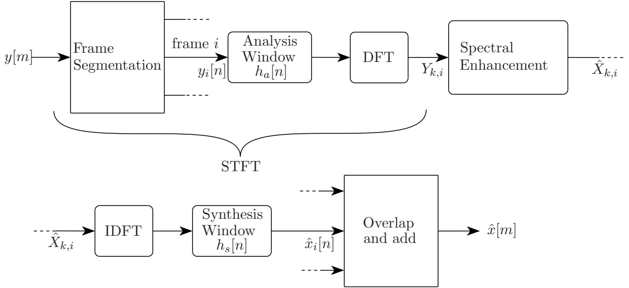
Fig. 3.2 STFT framework for single-channel speech enhancement.
