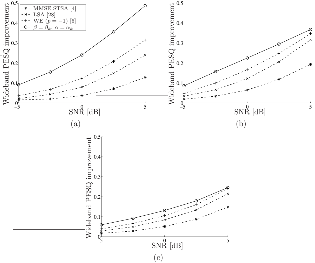
Fig. 8.3 Wideband PESQ improvement over noisy signal versus SNR for (a) white noise, (b) pink noise and (c) aircraft cockpit noise.
