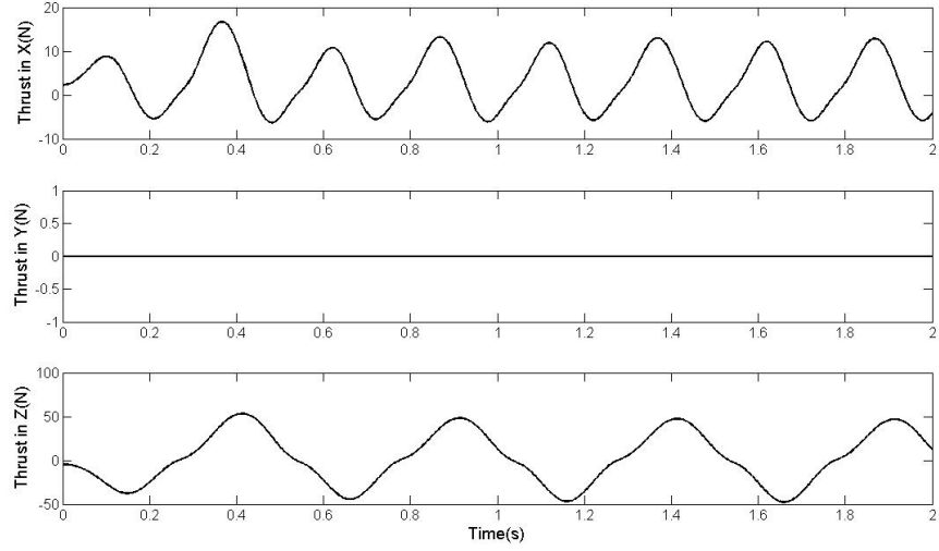
Figure 2-21: Thrust acting on centre of gravity of the robot
