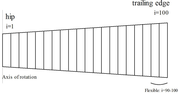
Figure 2-2: Top view of the flexible paddle, showing its discretization
