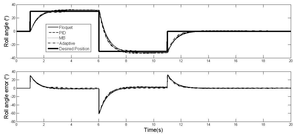
Figure 4-15: Simulation of the third roll maneuver
