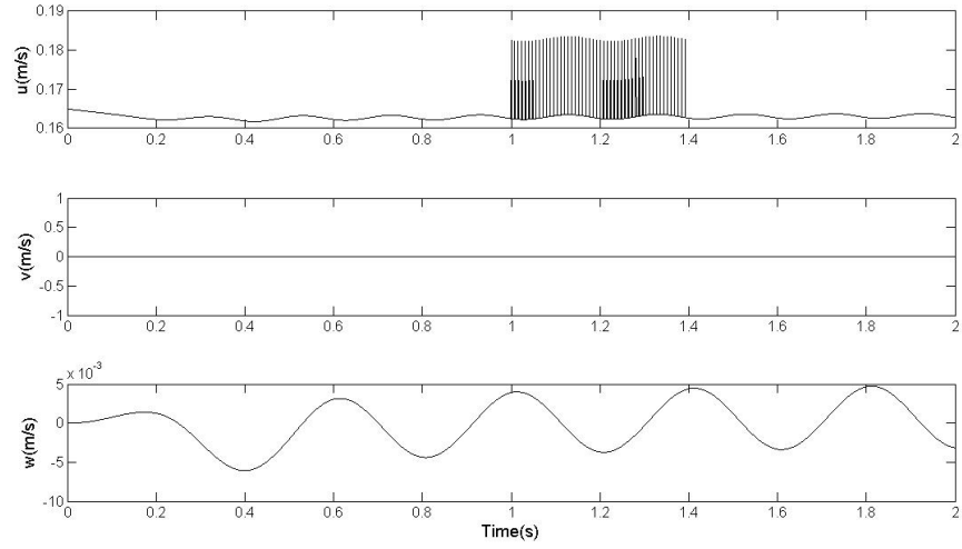
Figure 2–22: Disturbance in the surge velocity
