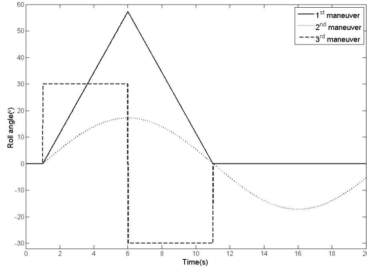
Figure 4-7: Roll trajectories
