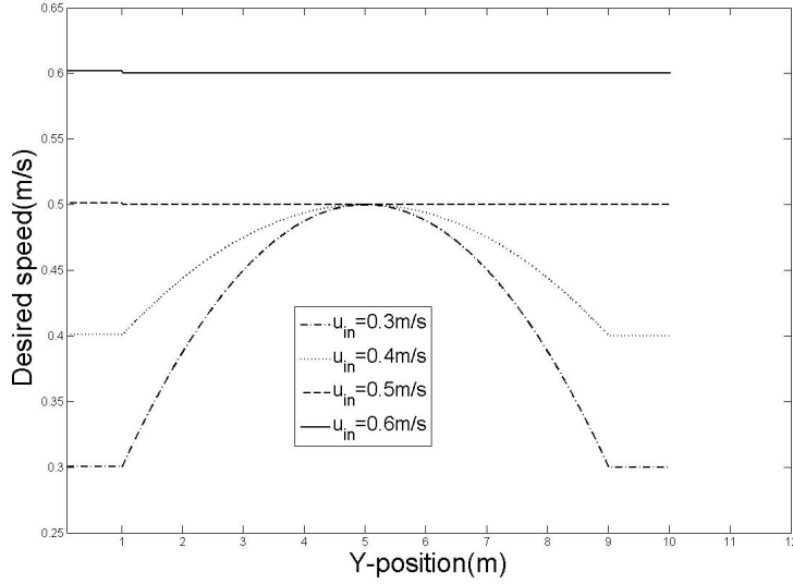
Figure 5-3: Desired speed of the vehicle, u_d , as a function of its y -position for D = 10\text{m} and R_{in} = 1\text{m}
