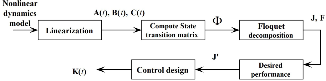
Figure 4–5: Flowchart of the process to obtain the gain matrix using Floquet theory
