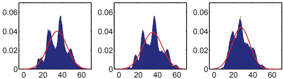
(c) Histograms and corresponding Gaussian density approximations for each of the three components of random vector \mathbf{y} ( n_0 = 8 ).
