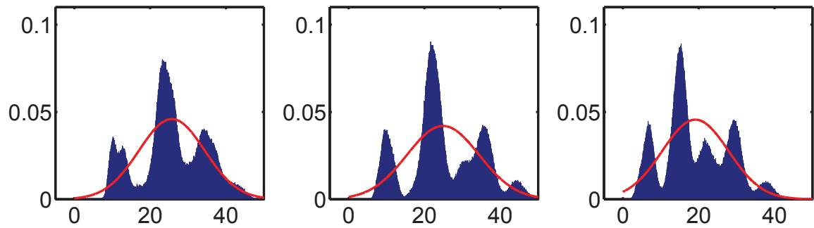
(b) Histograms and corresponding Gaussian density approximations for each of the three components of random vector \mathbf{y} ( n_0 = 6 ).
