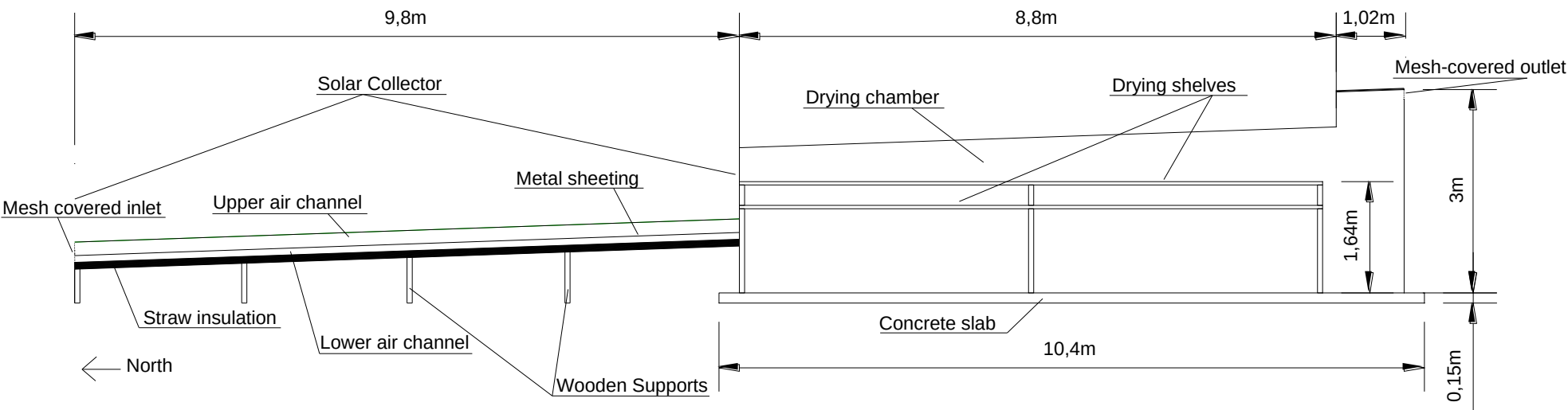
Solar Collector Inlet Details
