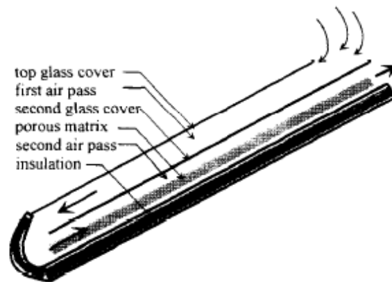
Figure 8: Example of Double Pass Solar Collector
