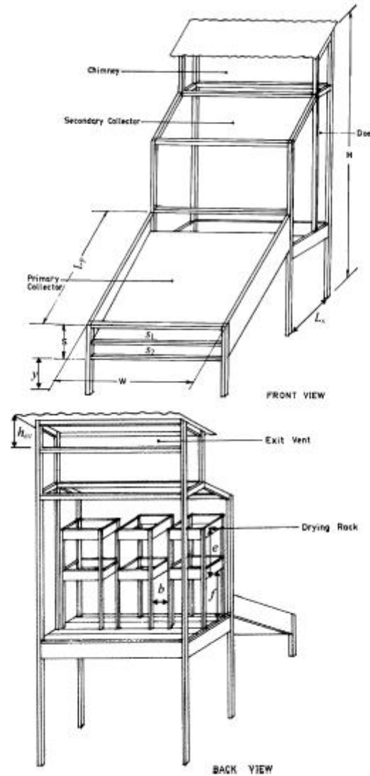
Figure 3: Schematic Views of the Mixed-Mode Natural Convection Solar Crop Dryer
