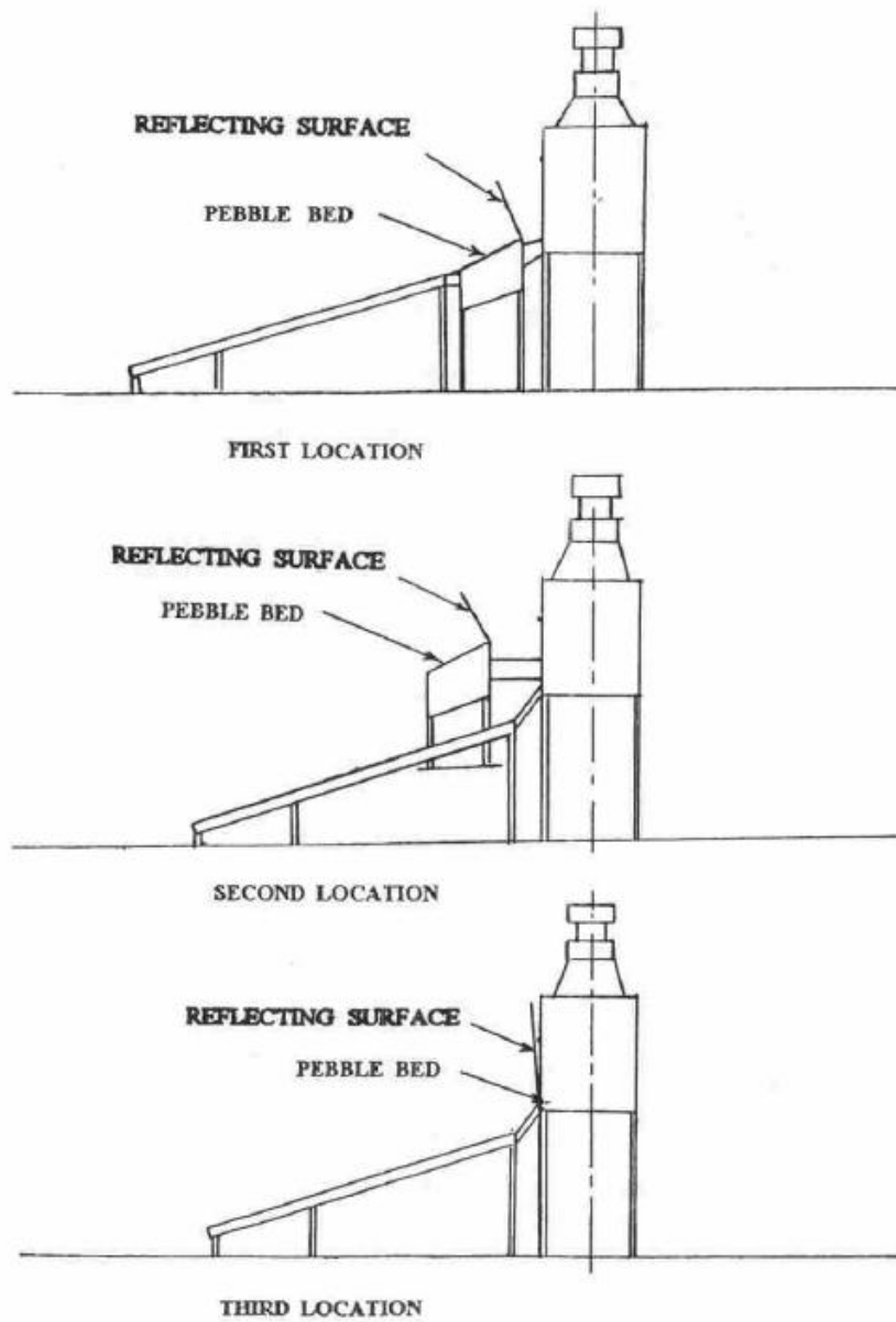
Figure 6: Pebble Bed Positions
