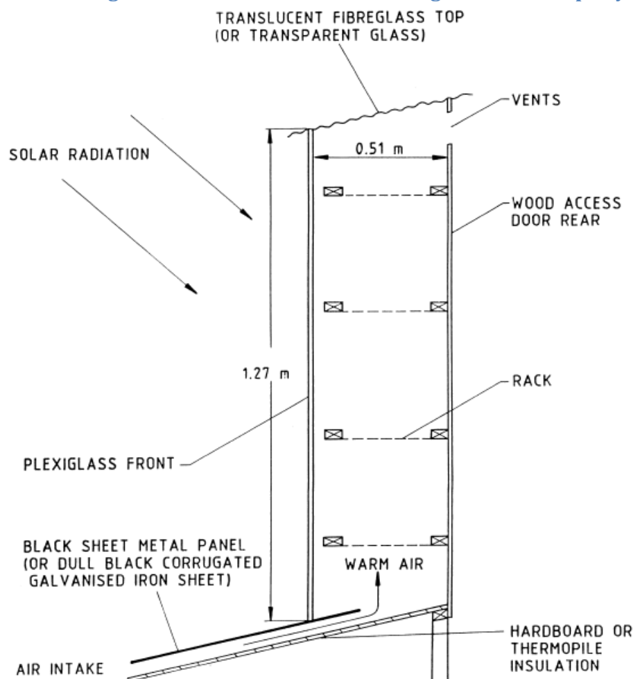
Figure 4: Lawand Multi-Stacked Design for Solar Crop Drying
