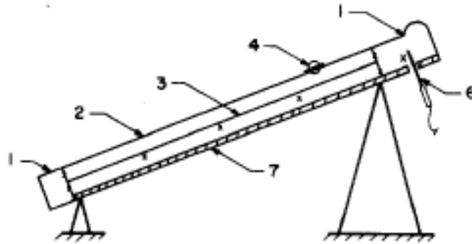
Figure 9: Solar collector setup: 1-Wind protection, 2- Glass cover, 3- Metallic absorber, 4- Radiometer, 6- Thermoanemometer, 7-Styrofoam insulation
