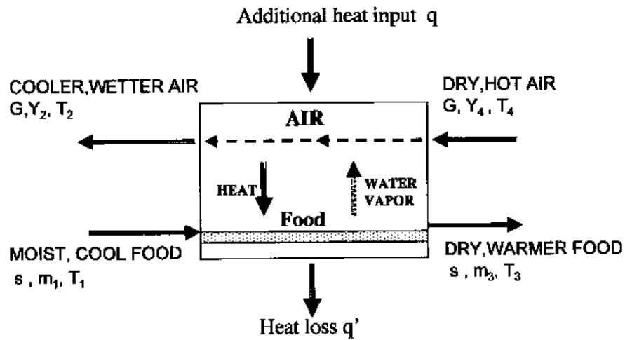
Figure 1: Schematic representation of material flows in a dryer.
