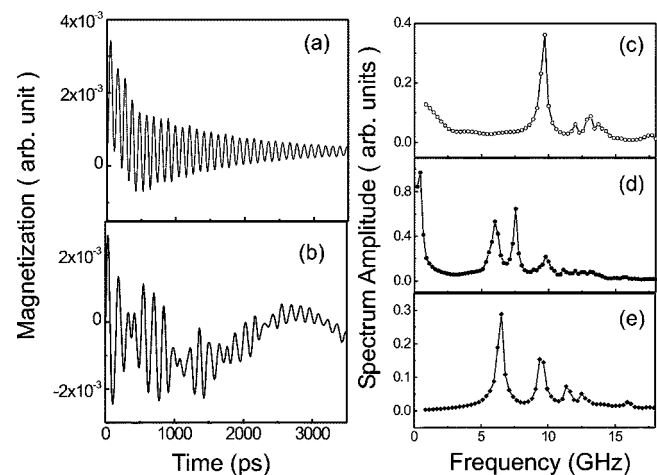
FIG. 3. Time-domain ferromagnetic resonance curves from micromagnetic simulation. FMR curve for pulsed magnetic field applied (a) perpendicular to the disk, and (b) parallel to the disk. (c)–(e) The spectrum amplitude as a function of frequency for the transient field applied (c) perpendicular to the disk, (d) parallel to the disk. (e) The simulation for the transient field in the plane of a wide ring (same outer diameter as the disk, with a 5-nm-diam central hole).
