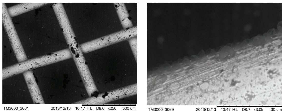
Figure S-3 Examples of back scattered electron images of gold grids from blank experiments (no Zn source).
