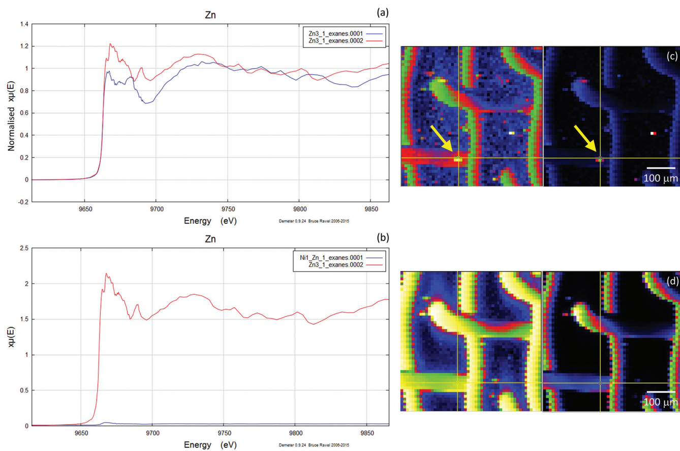
Figure S-5 Group b: (a) Zn K-edge XANES spectra of Zn precipitates, (b) comparison with background Zn (blue), (c) position of Zn hot spot 1 indicated by an arrow, (d) Au distribution of the gold mesh.
