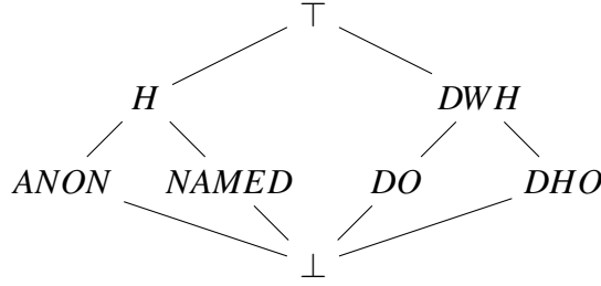
Figure 3.8 Handle propagation analysis abstract values.
