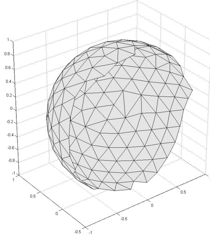
Fig. 3.2 Half of a sphere surface generated with Distmesh in 3D using tetrahedral mesh elements, after being processed by vol2surf
