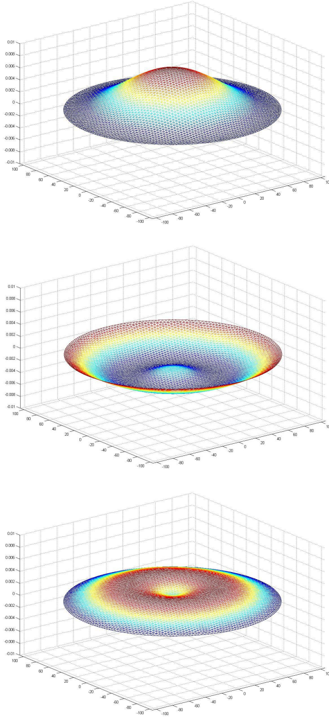
Fig. 3.5 Drum membrane modeled with a waveguide junction mesh adapted to an unstructured triangular topology, from top to bottom: timestep n=1 , 30, and 60
