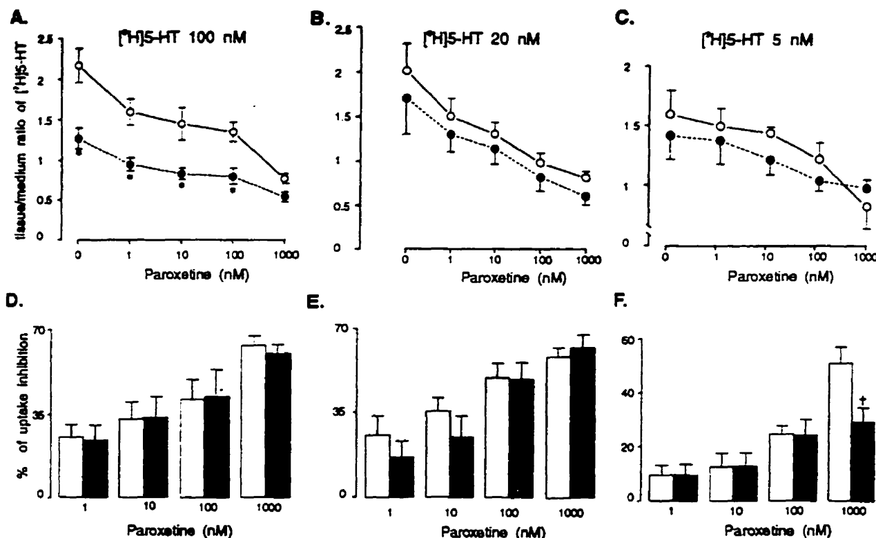
Figure 11. 3 H-5-HT reuptake activity (A–C) and effectiveness of paroxetine to inhibit 3 H-5-HT reuptake, expressed as percentage of uptake inhibition (D–F) in hippocampal slices from control ( n = 5 ; ○) and long-term paroxetine-treated rats ( n = 5 ; ●) (10 mg/kg/d. s.c. × 21 d + 48 h washout). *, p < 0.02 as compared to control values using nonpaired Student's t test; †, p < 0.05 as compared to control using nonpaired Student's t test.
