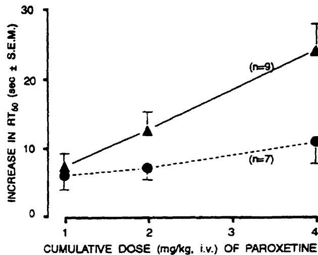
Figure 7. Effect of successive injections of paroxetine on the recovery time from 5 nA microiontophoretic applications of 5-HT in control rats ( \Delta ) and in rats treated with paroxetine (10 mg/kg/d, s.c. \times 21 d) following 48 hr washout ( \bullet ). Values are expressed as increase in RT_{50} (mean \pm SEM). p < 0.05 , comparing the two curves by ANOVA.
