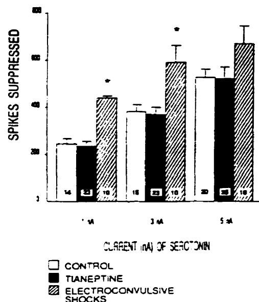
Fig. 4 Responsiveness, expressed as spikes suppressed (mean \pm SEM), of dorsal hippocampus pyramidal neurons to microiontophoretically-applied 5-HT in control rats, rats pretreated with tianeptine ( 20 \text{ mg/kg/day s.c.} \times 14 \text{ days} ) and in rats that had received six electroconvulsive shocks over a two week period. The number of neurons tested is indicated at the bottom of each column. * p < 0.001 using paired Student's t -test
