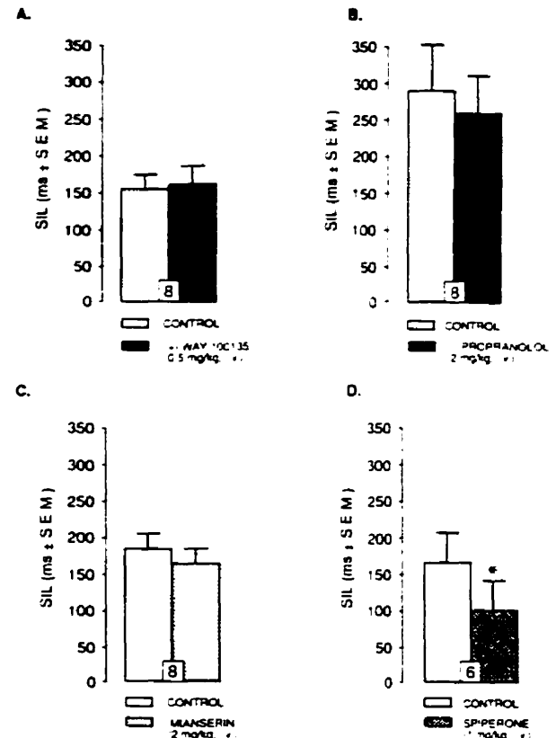
Fig. 4. Duration of the suppression of dorsal raphe 5-HT neuron firing activity produced by the stimulation of the 5-HT pathway prior to control and following the intravenous administration of (A) WAY 100135 (A), (B) propranolol (B), mianserin (C), and spiperone (D). The number of neurons tested (one per rat) is indicated at the bottom of each pair of columns. * P < 0.02 (paired Student's t test).
