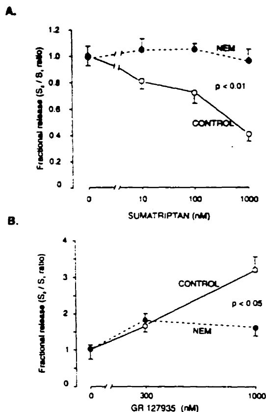
Fig. 2. Inhibition produced by the 5-HT 1D agonist sumatriptan (A) or enhancement produced by the 5-HT 1D receptor antagonist GR 127935 (B) of the evoked release of tritium elicited by electrical stimulation of preloaded midbrain control slices (open circles) or slices preincubated with NEM (solid circles). The experiments were carried out immediately after a 30 min incubation period with either Krebs alone or Krebs with NEM (30 \mu M). Ordinates: fraction of total tissue radioactivity released by 360 pulses (30 mA, 2 min, 3 Hz). Each point represents the mean \pm S.E.M. of the results obtained in experiments run in parallel for control and treated rats. Three to five pairs of rats were used per point. Statistical significance was calculated using two-way analysis of variance to compare the curves obtained in control and treated groups.
