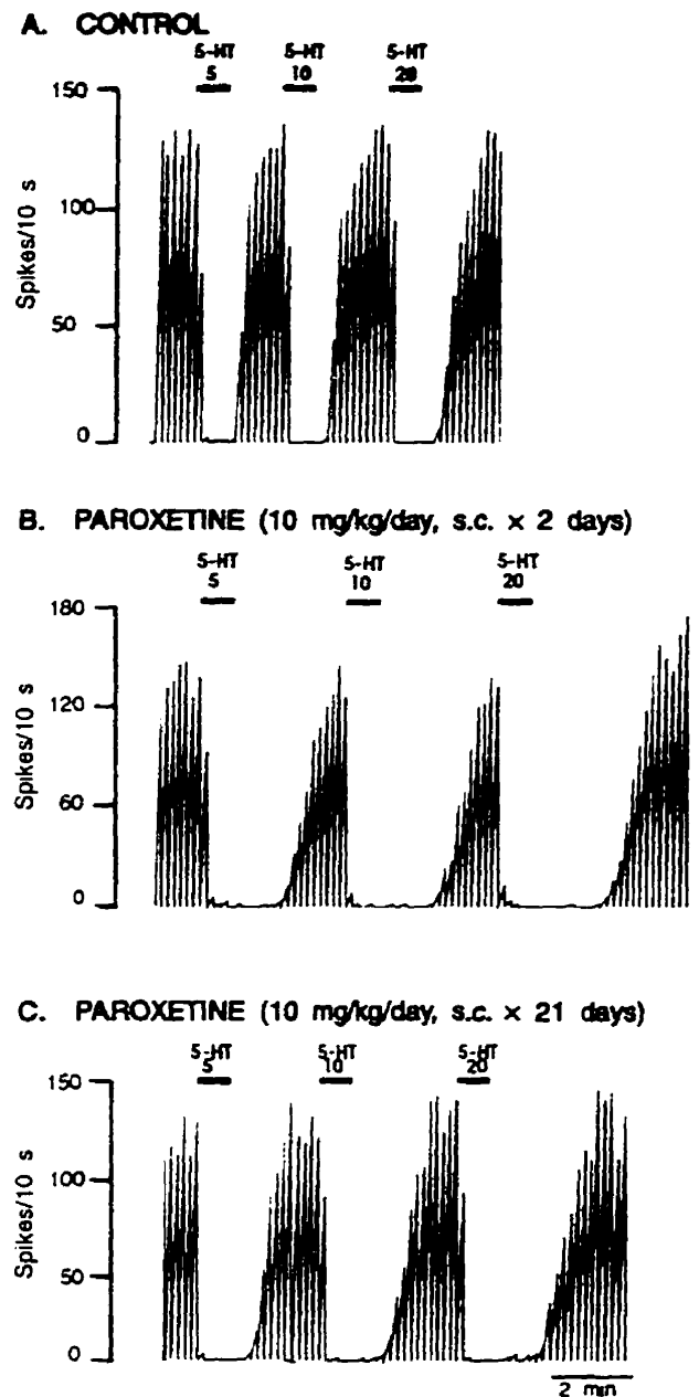
Figure 8. Integrated firing rate histograms showing the response of CA1 dorsal hippocampus pyramidal neurons to microiontophoretically applied 5-HT in a control rat (A) and in rats treated with paroxetine (10 mg/kg/d, s.c.) for 2 d (B) or 21 d (C). In B and C, the experiments were carried out with the minipump in place.
