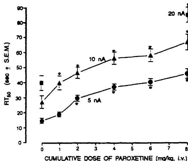
Figure 2. Effect of successive intravenous injections of paroxetine on the recovery time, expressed as RT_{50} values (means \pm SEM), from microiontophoretic applications of 5-HT with 5 nA ( \bullet ), 10 nA ( \blacktriangle ), and 20 nA ( \blacksquare ) ( N = 9 for all currents used). *, p < 0.001 , compared to preinjection value using the Student's paired t test.
