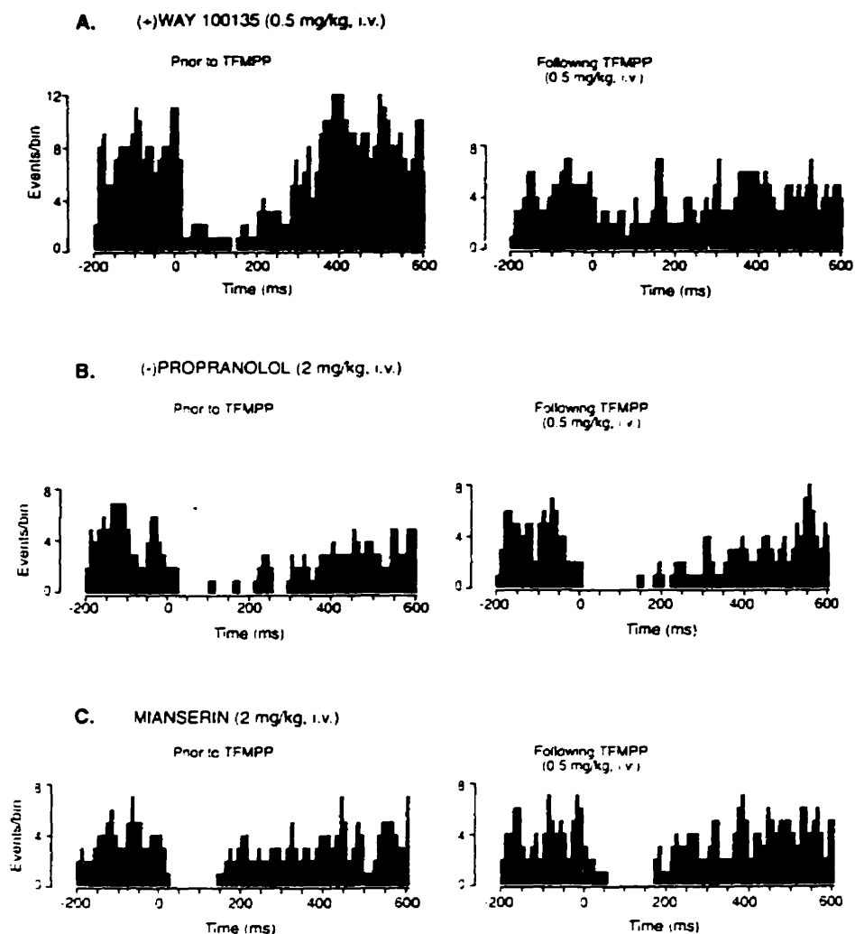
Fig. 5. Penstimulus time histograms obtained from dorsal raphe 5-HT neurons prior to and following the injection of TFMP in rats that had previously received (+)WAY 100135 (A), (-)propranolol (B) mianserin (C). Each histogram was constructed from 150–200 stimuli of 0.5 ms delivered at 1 Hz with an intensity of 300 \mu A. Bin width is of 10 ms. Stimulation pulse was delivered at time 0.
