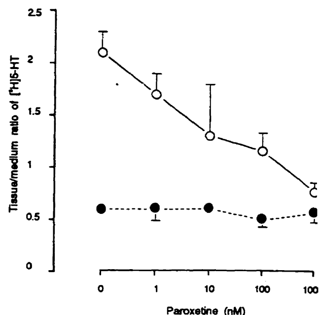
Figure 10. Effect of increasing concentrations of paroxetine on ^3H -5-HT uptake in hippocampal slices of control (O) and 5,7-DHT-lesioned rats (●). n = 3 in each group. p < 0.001 comparing both curves by ANOVA.
