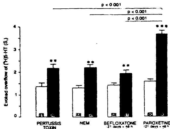
Fig. 3. Effect of G protein inactivation with pertussis toxin or NEM and of long-term administration of paroxetine or befloxadone on the electrically evoked release of tritium in midbrain slices preloaded with [ ^3 H]5-HT. Long-term treatments were administered using osmotic minipumps implanted subcutaneously and removed 48 hr before the experiments to allow drug elimination. Ordinates: fraction of the total radioactivity released by 360 pulses (30 mA, 2 min, 3 Hz) during the first period of stimulation before the introduction of any drug in the perfusate ( S_1 ). Experiments were always carried out in pairs of rats: a control and a treated one processed in parallel in the same experiment. Figures at the bottom of each column refer to the number of slices studied per group (five to eight rats per group). Statistical significance was calculated using nonpaired Student's t test to compare control and treated groups. ** P < .01 ; *** P < .001 .
