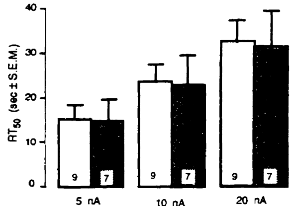
Figure 6. A , Integrated firing rate histograms illustrating the response of dorsal hippocampus CA 1 pyramidal neurons in a control and a long-term paroxetine-treated rat 48 hr after the removal of the osmotic pump. Each current is applied alternatively in the control rat and the paroxetine-treated rat. B , Recovery time expressed as RT 50 values (mean ± SEM) of dorsal hippocampus pyramidal neurons from microiontophoretically applied 5-HT in control rats and in rats treated with paroxetine for 21 d. Note that RT 50 values for the 5 nA current are significantly smaller than for the 20 nA current and this difference is maintained after long-term paroxetine administration ( p < 0.001). Number of neurons tested is given at the bottom of each column.
