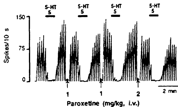
Figure 5. Integrated firing rate histograms showing the response of dorsal hippocampus CA 1 pyramidal neurons to microiontophoretic applications of 5-HT in a control rat ( A ) and a long-term paroxetine-treated rat ( B ), following successive intravenous injections of paroxetine at 10 min intervals. Rats were implanted subcutaneously with an osmotic minipump which delivered either vehicle or paroxetine. After 21 d the minipump was removed and a 48 hr washout period was allowed. Time scale applies to both traces.
