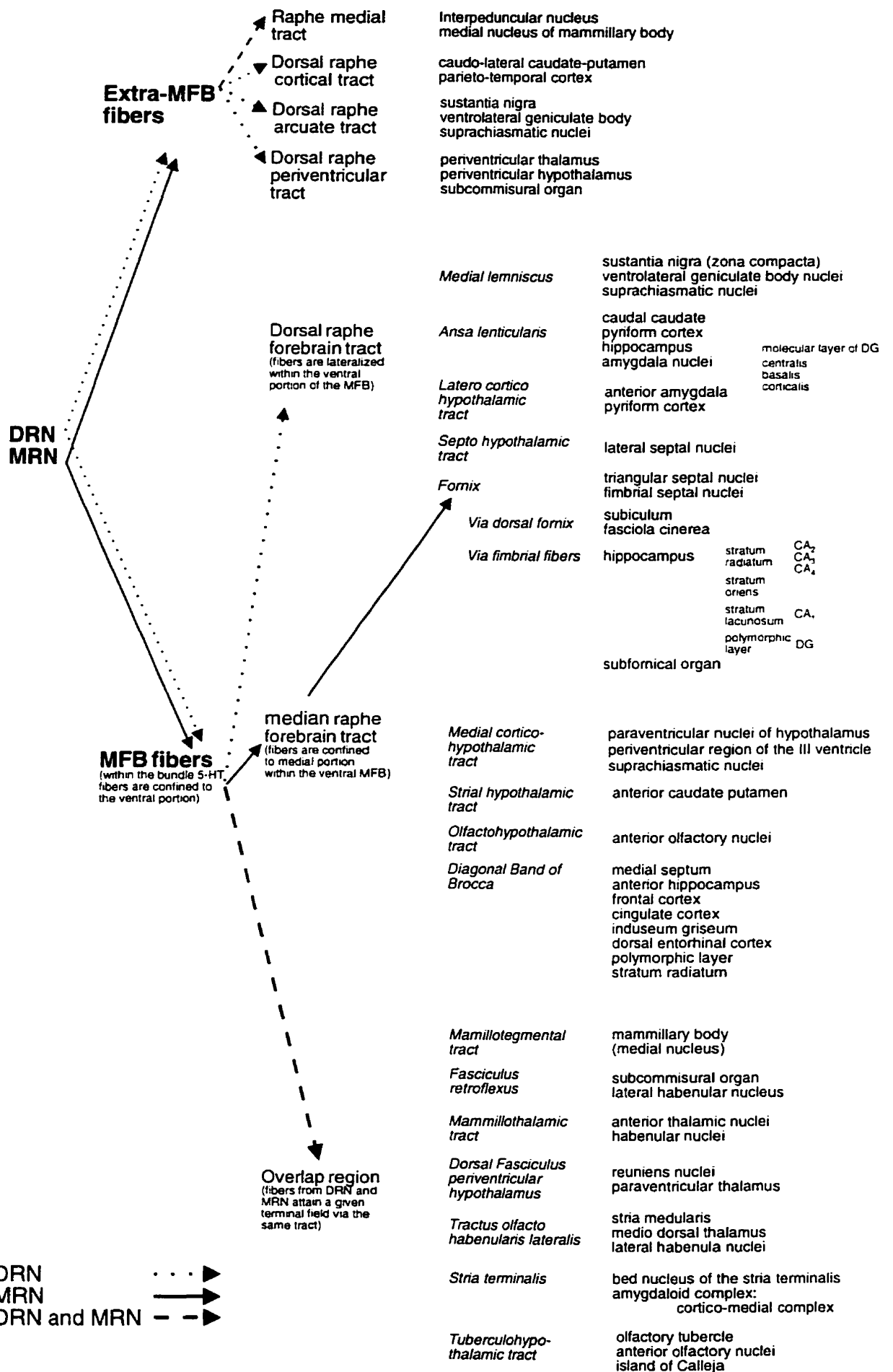
Figure 2. Differential projections from dorsal (DRN) and median (MRN) median raphe nuclei (see Azmitia and Segal, 1978).
