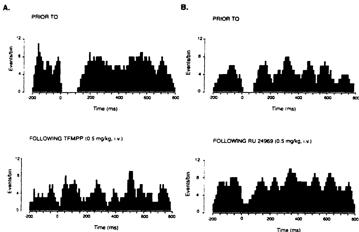
Fig. 2. Peristimulus time histograms obtained from a dorsal raphe 5-HT neuron prior to and following the intravenous administration of TFMPP (A) and RU 24969 (B). Each histogram was constructed from 150–200 stimuli of 0.5 ms delivered at 1 Hz with an intensity of 300 \mu A. Bin width is of 10 ms. Stimulation pulses were delivered at time 0.
