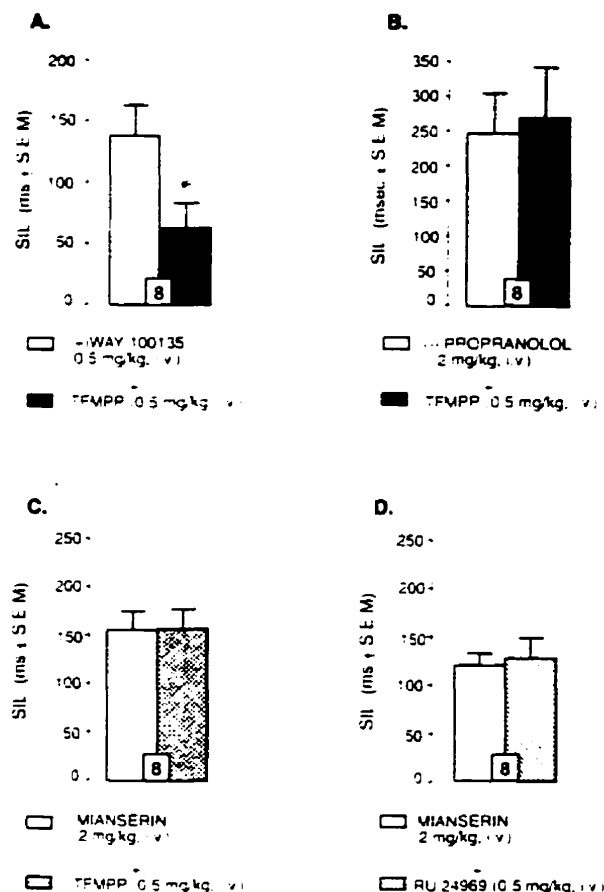
Fig. 6. Duration of the suppression of dorsal raphe 5-HT neuron firing activity produced by the stimulation of the 5-HT pathway in rats pretreated with (-)-WAY 100135 prior to and following the intravenous administration of TFMPP (A), in rats pretreated with (-)-propranolol prior to and following the intravenous administration of TFMPP (B), in rats pretreated with mianserin prior to and following the intravenous administration of TFMPP (C), in and rats pretreated with mianserin prior to and following the intravenous administration of RU 24969 (D). The number of neurons tested (one per rat) is indicated at the bottom of each pair of columns. * P < 0.02 (paired Student's t test).
