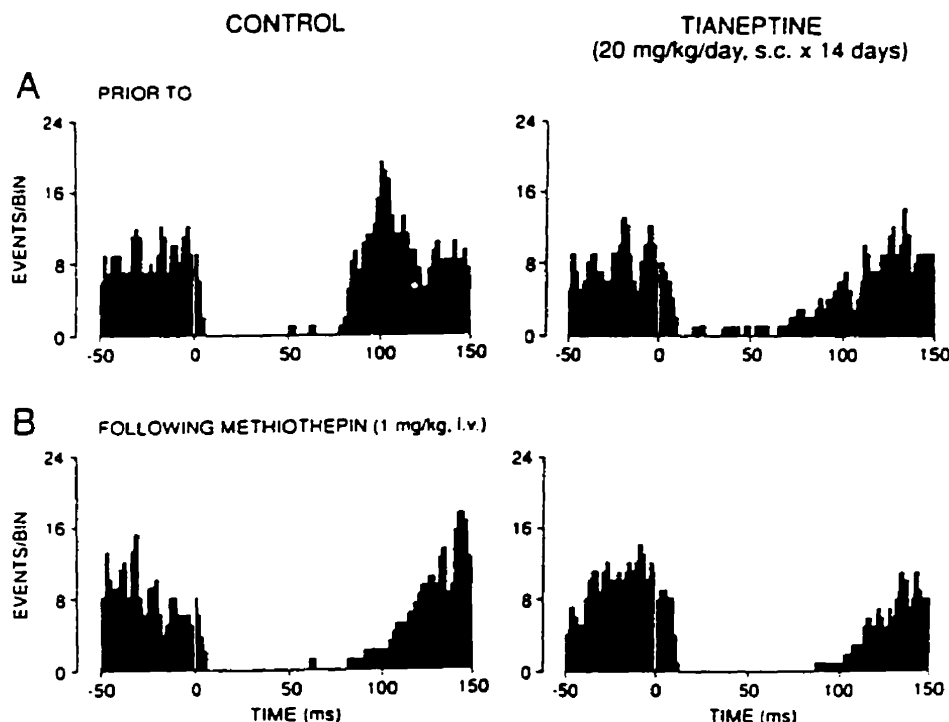
Fig. 6 Peristimulus time histograms showing the effect of the electrical stimulation of the ascending 5-HT pathway on the firing activity of two dorsal hippocampus pyramidal neurons, one recorded in a control rat and one in a rat treated with tianeptine, prior to (A) and following (B) the injection of methiothepin. Each peristimulus time histogram was constructed from 150 stimulations using 0.5 ms square pulses of 300 μA delivered at time 0. Bin width is 2 ms.
