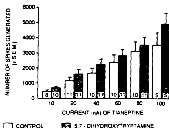
Fig. 2 Effect of tianeptine application onto CA 1 pyramidal neurons with different microiontophoretic currents in control and 5,7-dihydroxytryptamine treated rats. The number of neurons tested is given at the bottom of each column
