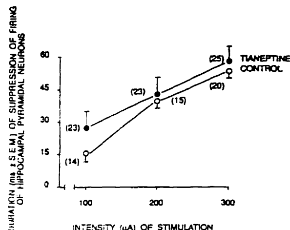
Fig. 7 Relationship between the duration of suppression of firing of CA 1 hippocampus pyramidal neurons and the intensity of the current used to stimulate the ascending 5-HT pathway in control rats (○) and in rats pretreated with tianeptine (20 mg/kg/day, s.c. x 14 days) (●). The number of neurons tested is given in parentheses.
