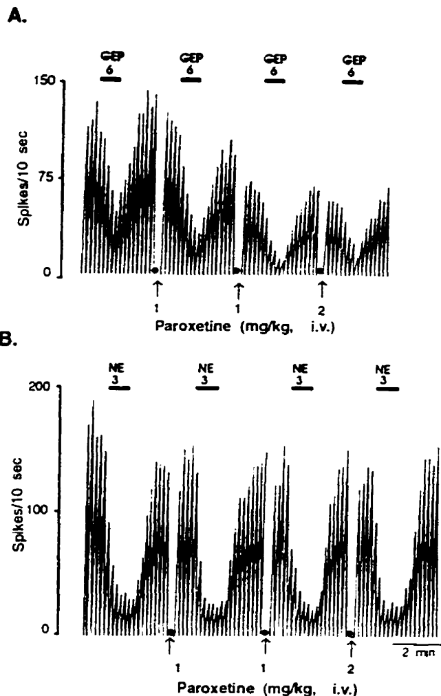
Figure 3. Integrated firing rate histograms of dorsal hippocampus CA1 pyramidal neurons showing the effect of successive injections of paroxetine at 10 min intervals on the response of a dorsal hippocampus pyramidal neuron to microiontophoretic application of gepirone ( A ) and NE ( B ). Dots at the bottom of each histogram represent periods of 10 min. Time scale applies to both tracings.
