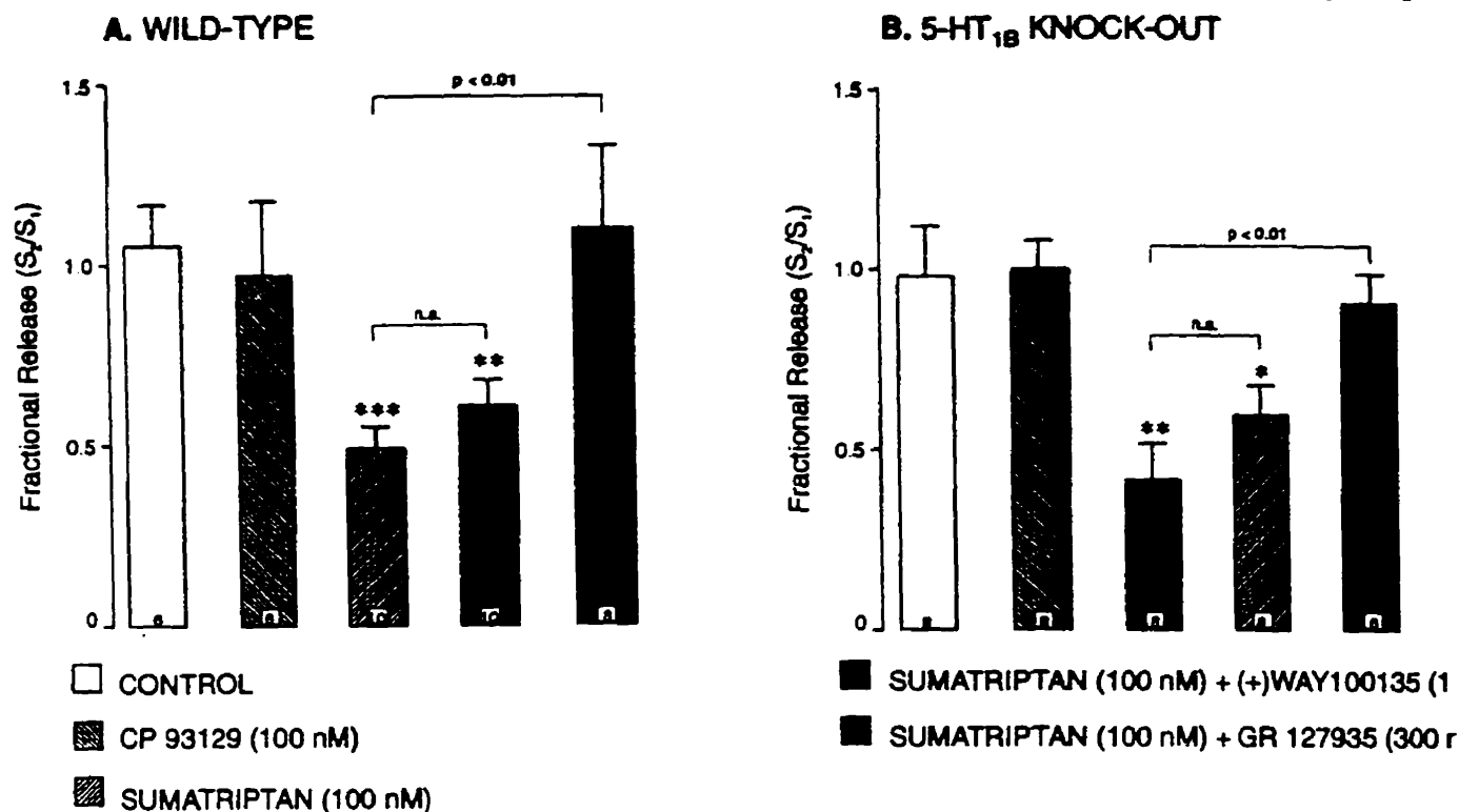
FIG. 3. Effect of different 5-HT 1 agonists and antagonists on the inhibition of electrically evoked release of [^3\text{H}]\text{5-HT} from preloaded midbrain raphe slices obtained from (A) wild-type and (B) 5-HT 1B knock-out mice. Agonists were introduced 20 min before S 2 and also remained present until the end of the experiment. The antagonists were introduced 20 min before S 1 . Values are expressed as means \pm s.e.m. for which the number of experiments per group is given at the bottom of each column. For each group, slices were obtained from two mice. The means were compared using Student's t -test. * p < 0.05; ** p < 0.01; *** p < 0.001.
